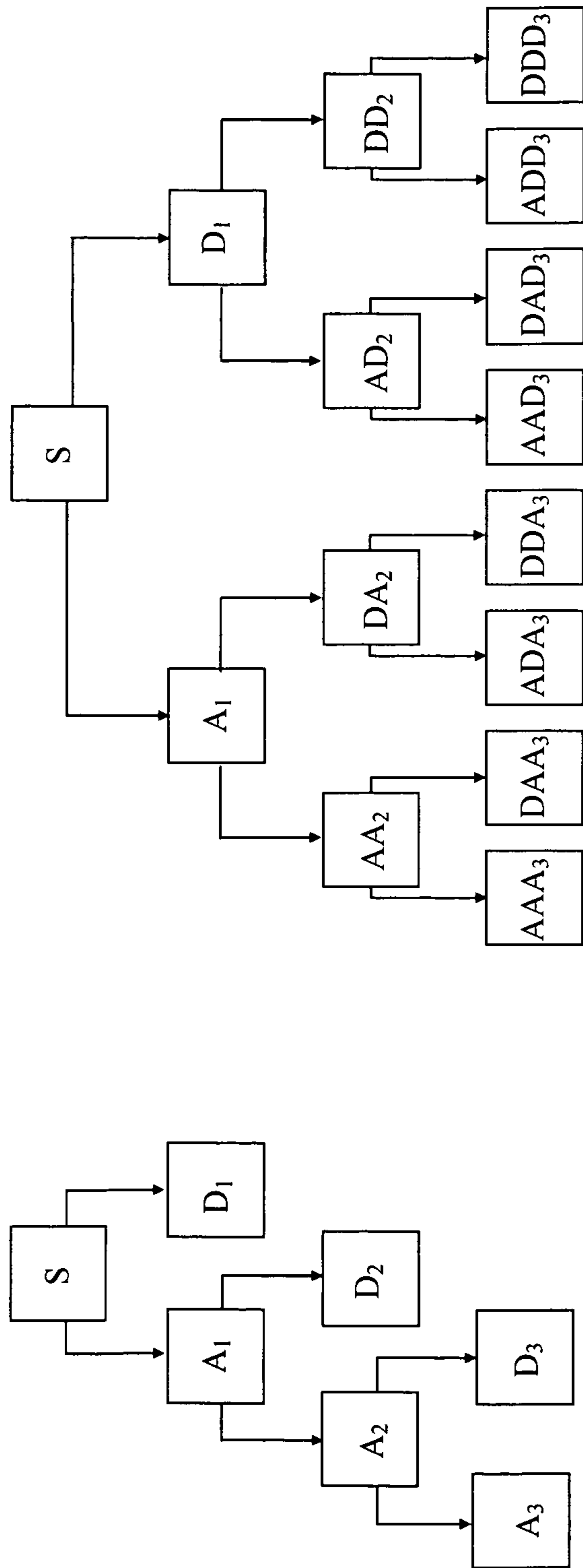
WAVELET PACKET
