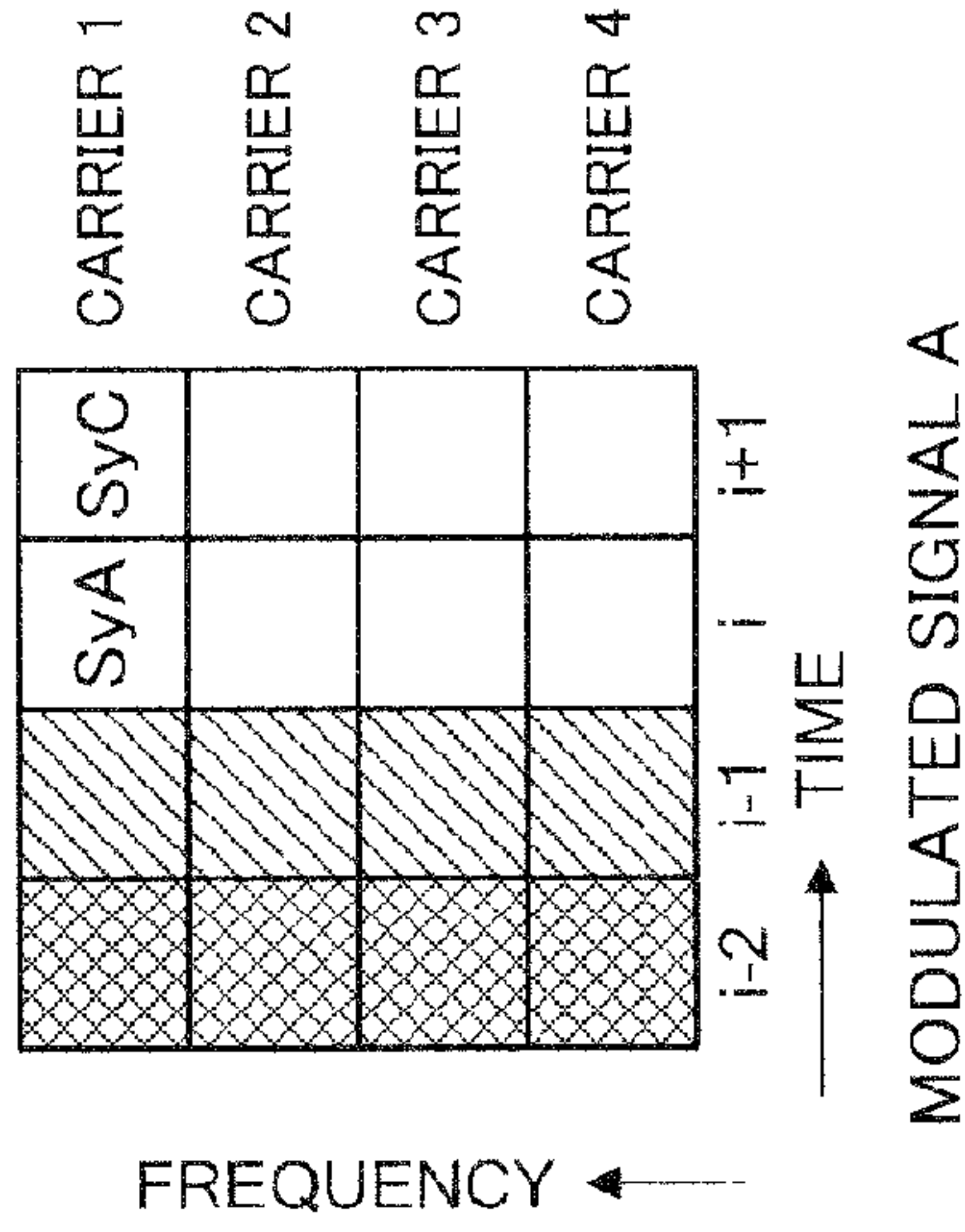
FIG.15B TRANSMISSION METHOD Y
