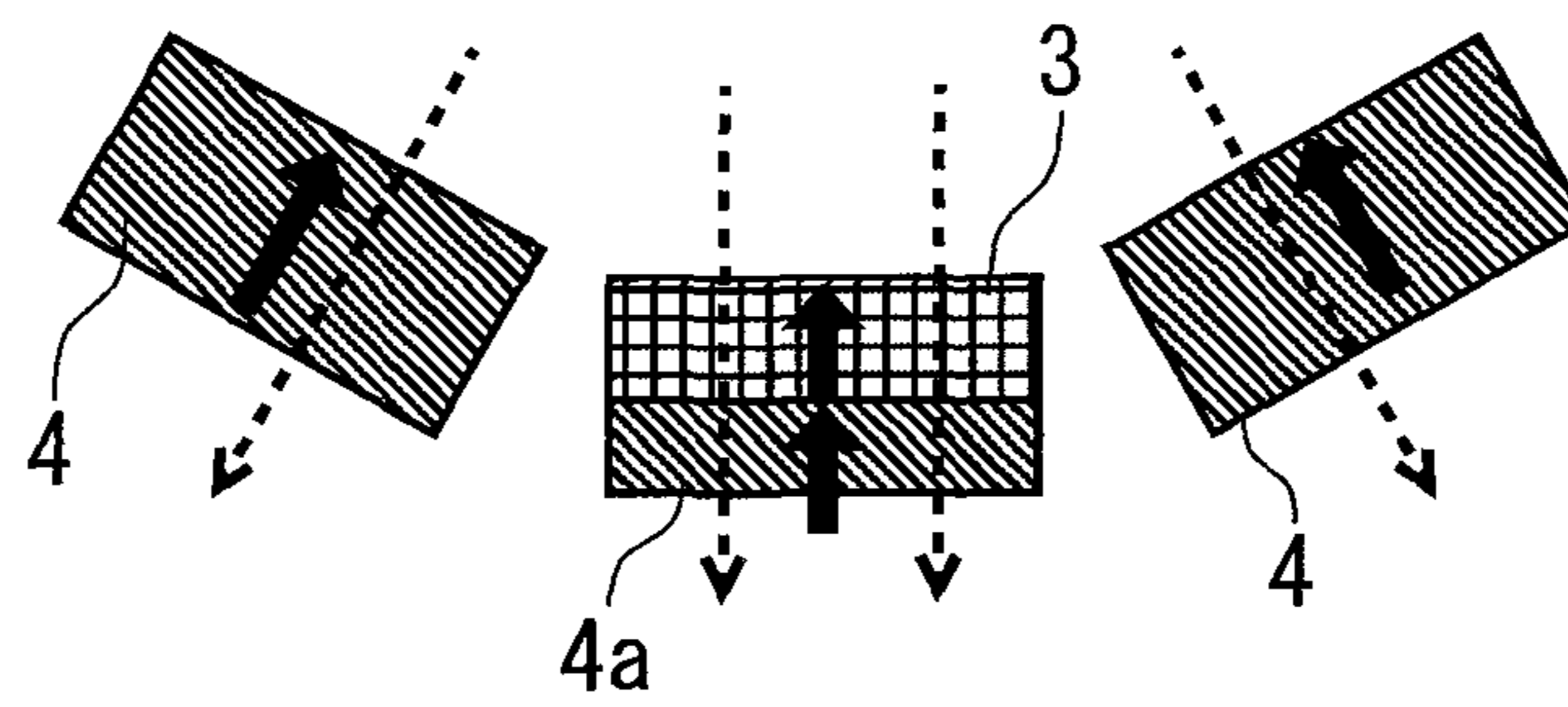
Decrease of the magnetic force of the variable magnet in the opposing magnetic field
