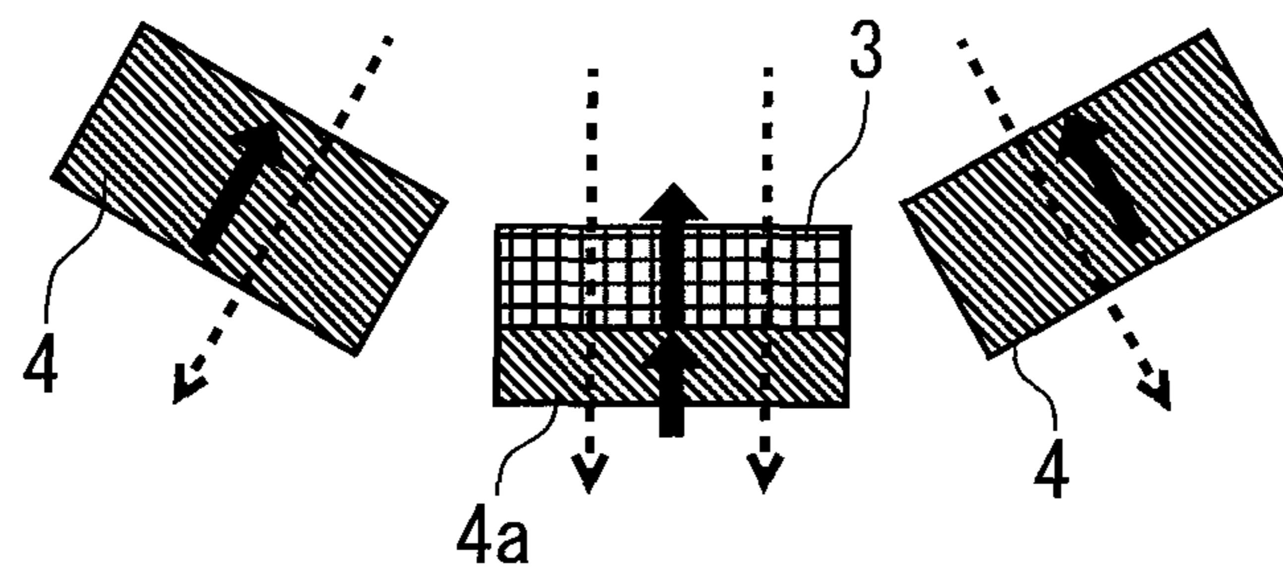
Generation of a magnetic field by the coil for decreasing the magnetic force of the variable magnet
