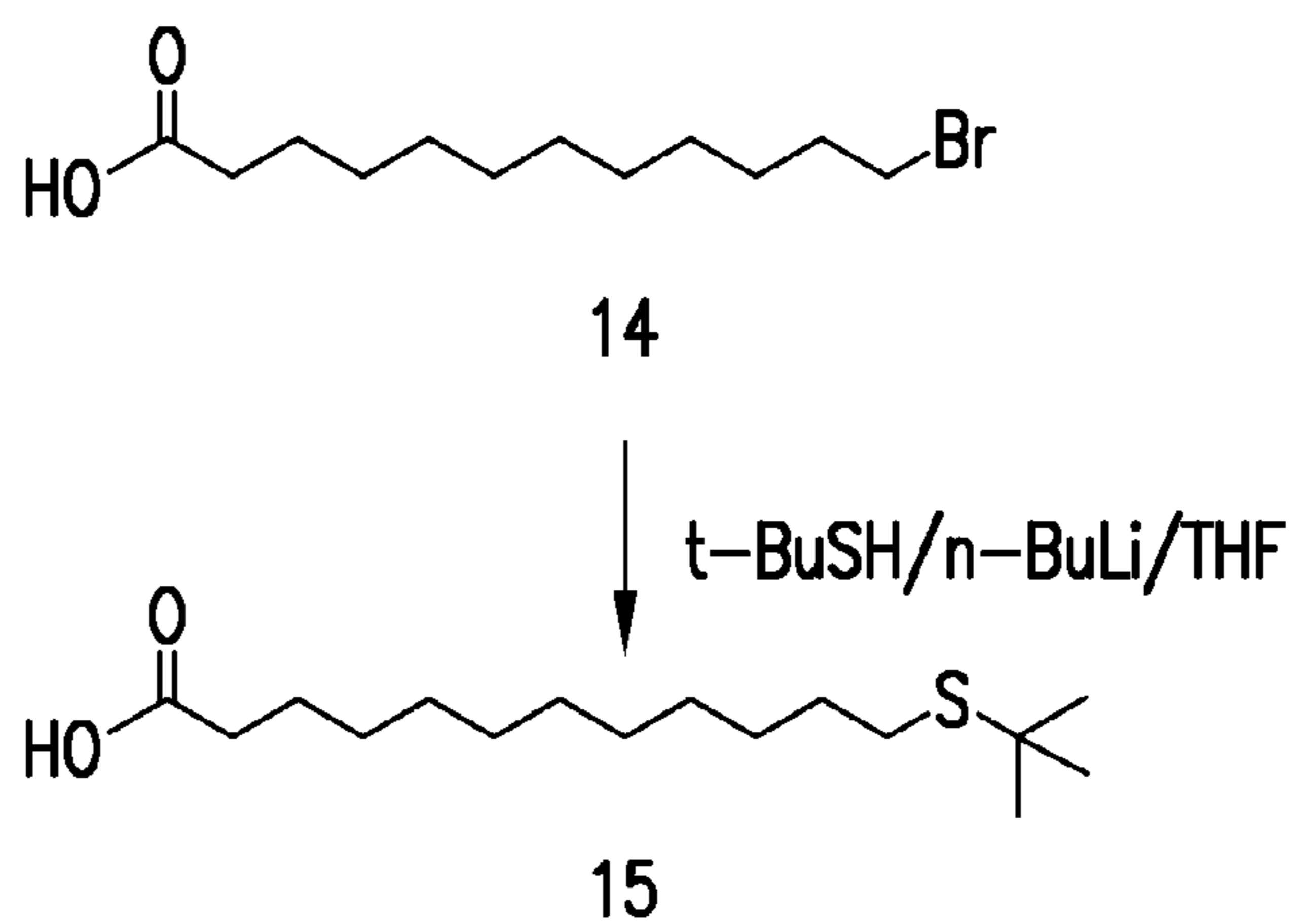
Synthesis of Typical Protected Thiolated Fatty Acid
