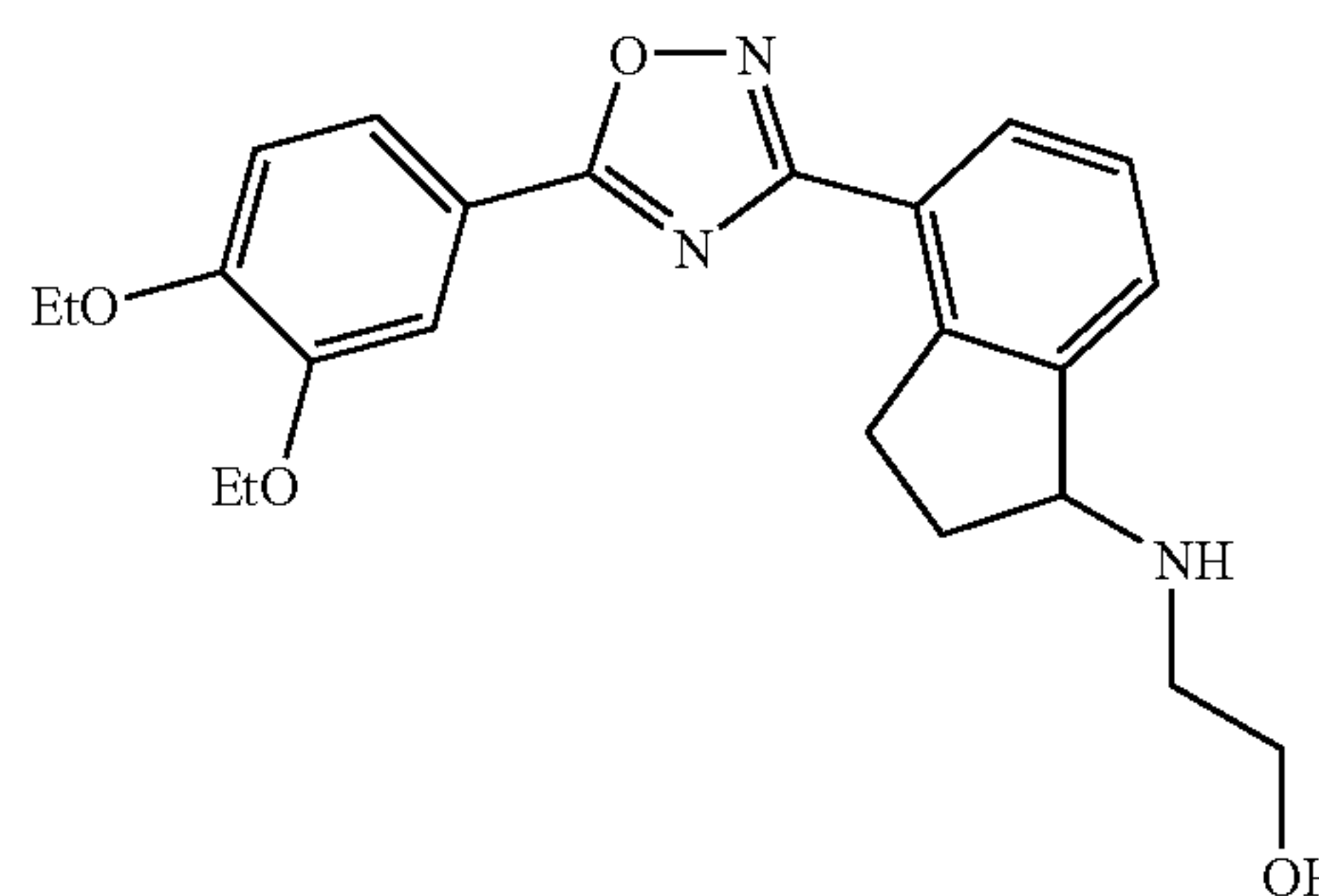
2-(4-(5-(3,4-diethoxyphenyl)-1,2,4-oxadiazol-3-yl)- 2,3-dihydro-1H-inden-1-ylamino)ethanol
