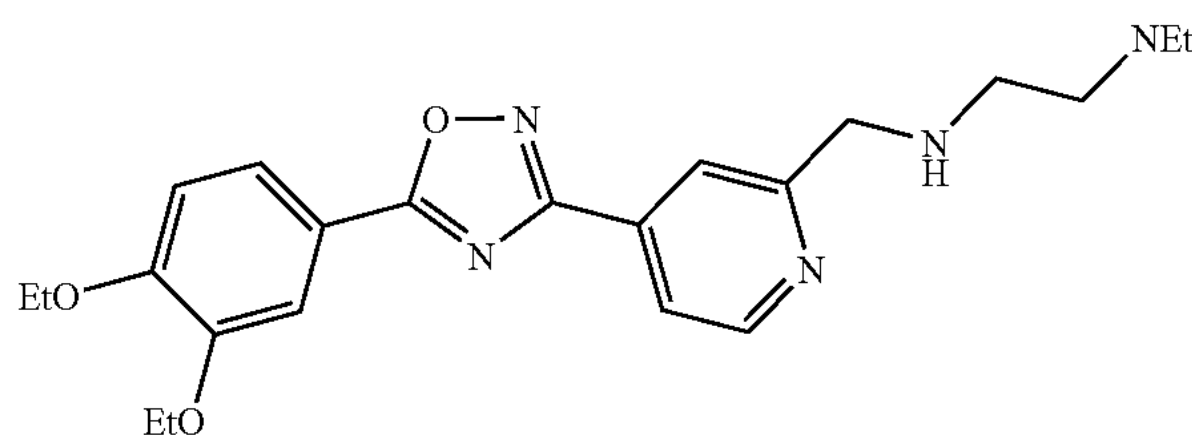
N1-((4-(5-(3,4-diethoxyphenyl)-1,2,4-oxadiazol-3-yl)pyridin-2-yl)methyl)-N2,N2-diethylethane-1,2-diamine
