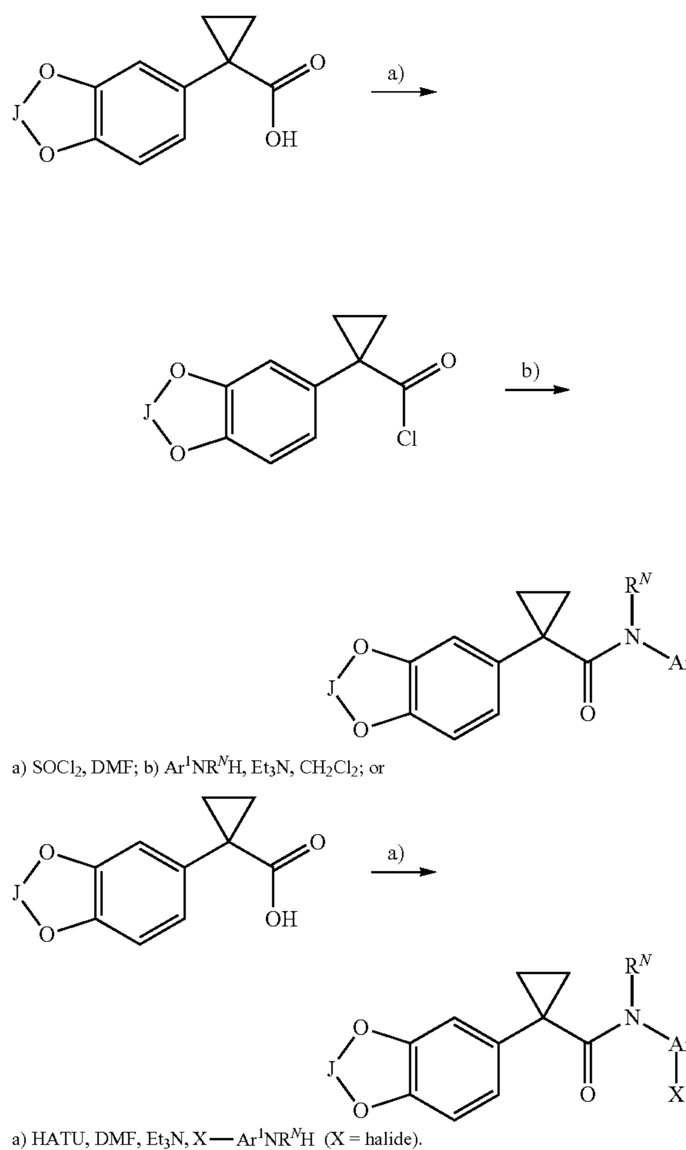
Scheme II - Amide coupling.
