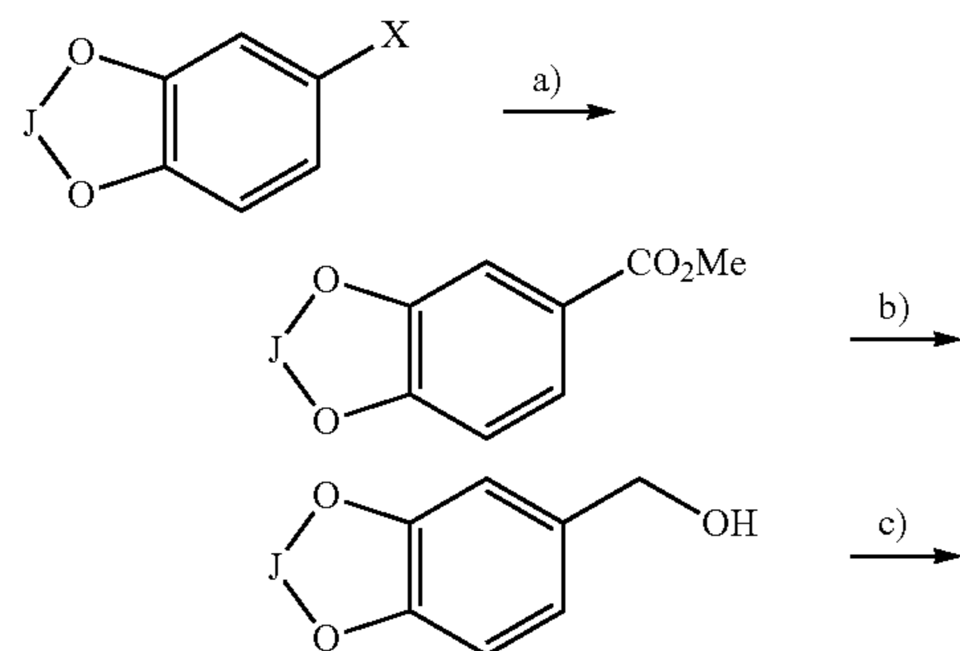
Scheme I - Preparation of cycloalkyl acids.
