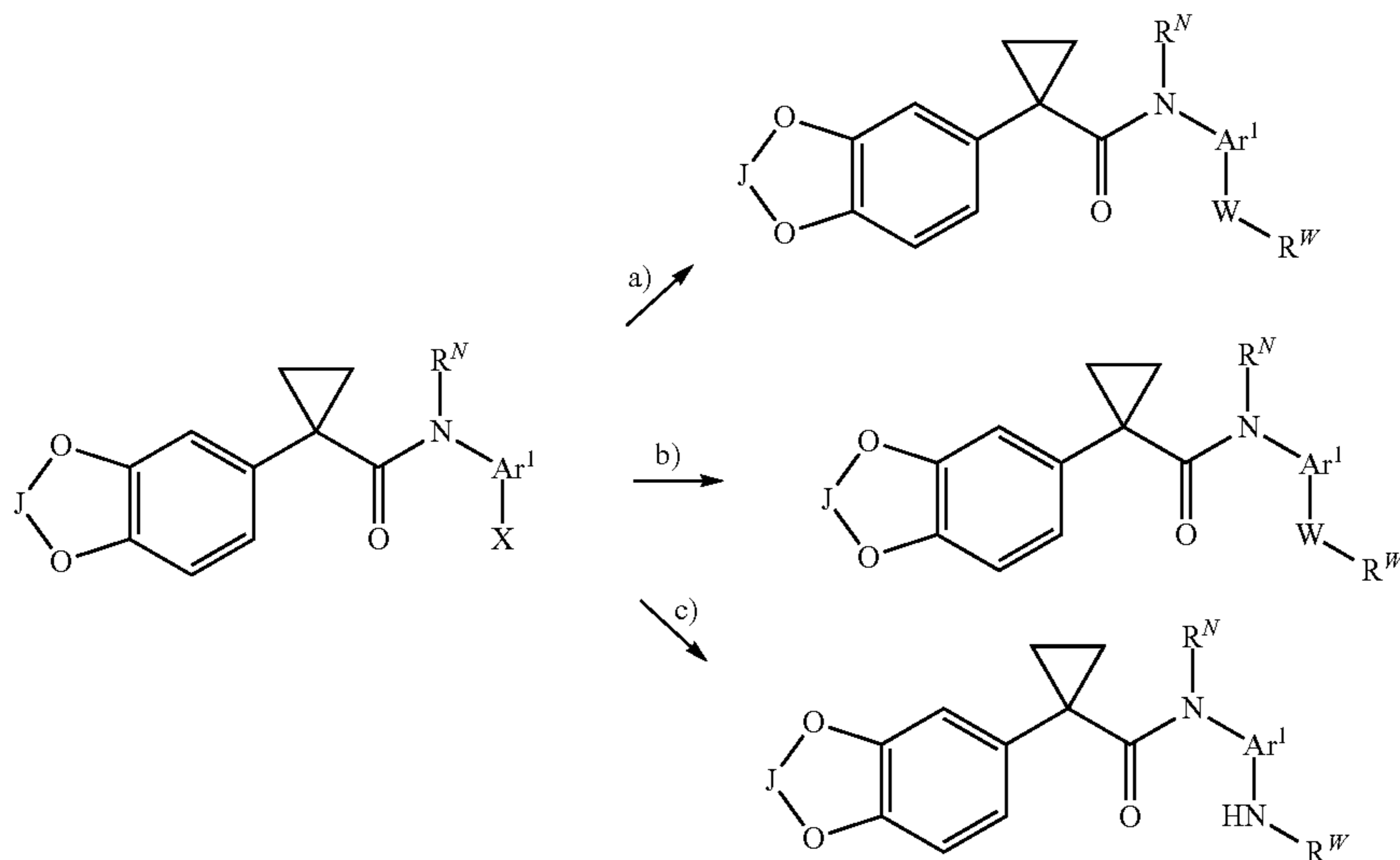
Scheme III - Derivatization of heteroarylhalides
