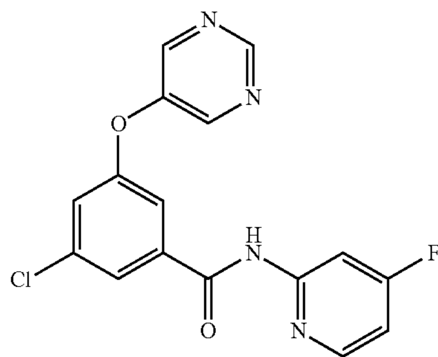
b. 3-chloro-N-(4-fluoropyridin-2-yl)-5-(pyrimidin-5-yloxy)benzamide (8)
