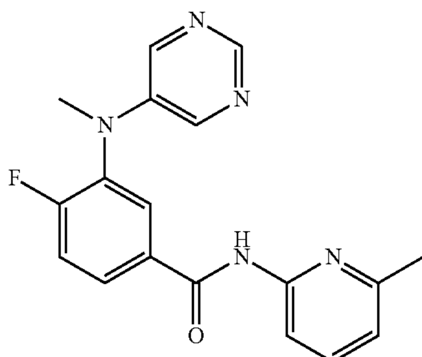
c. 4-fluoro-3-(methyl(pyrimidin-5-yl)amino)-N-(6-methylpyridin-2-yl)benzamide (21)
