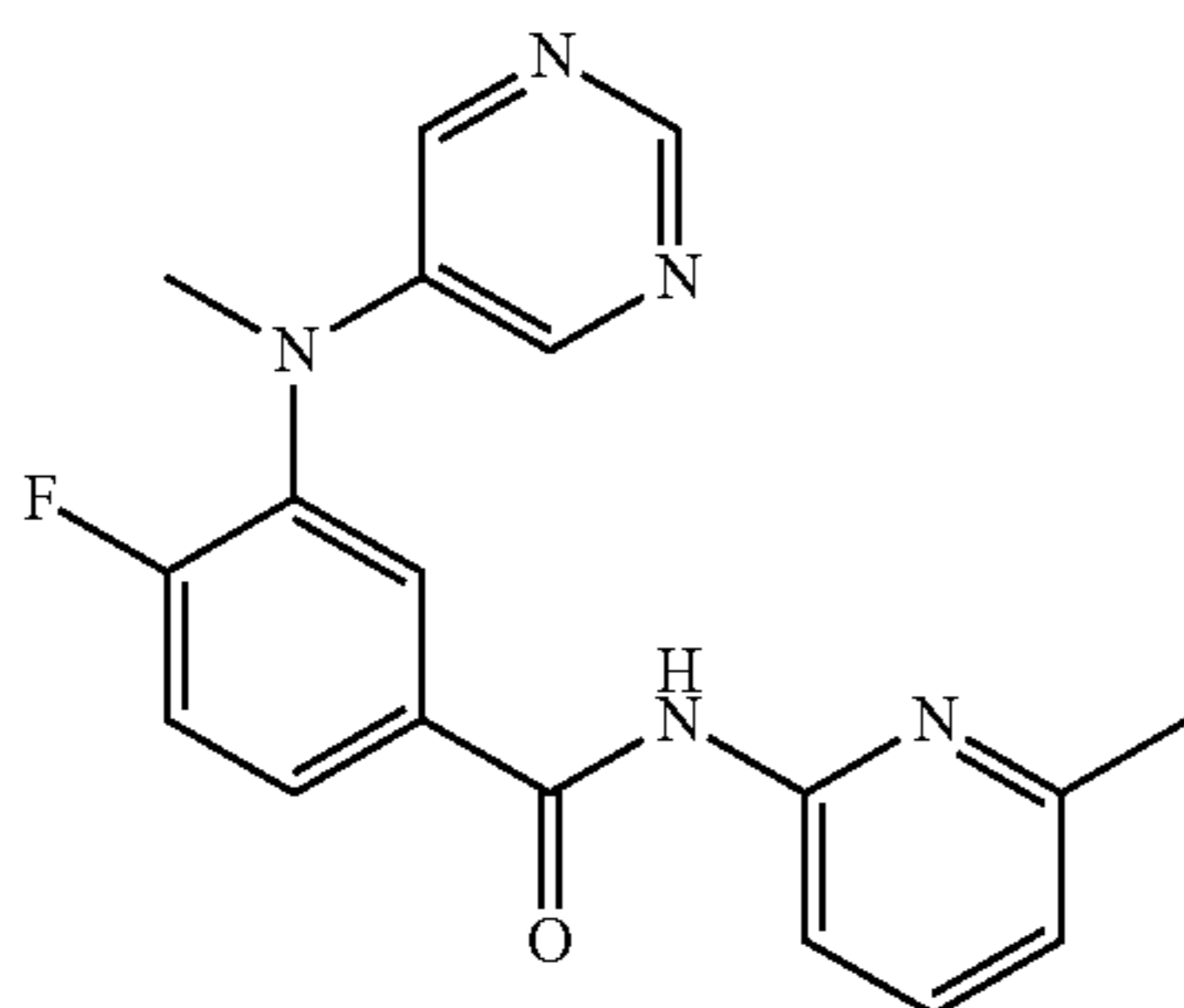
c. 4-fluoro-3-(methyl(pyrimidin-5-yl)amino)-N-(6-methylpyridin-2-yl)benzamide (21)
