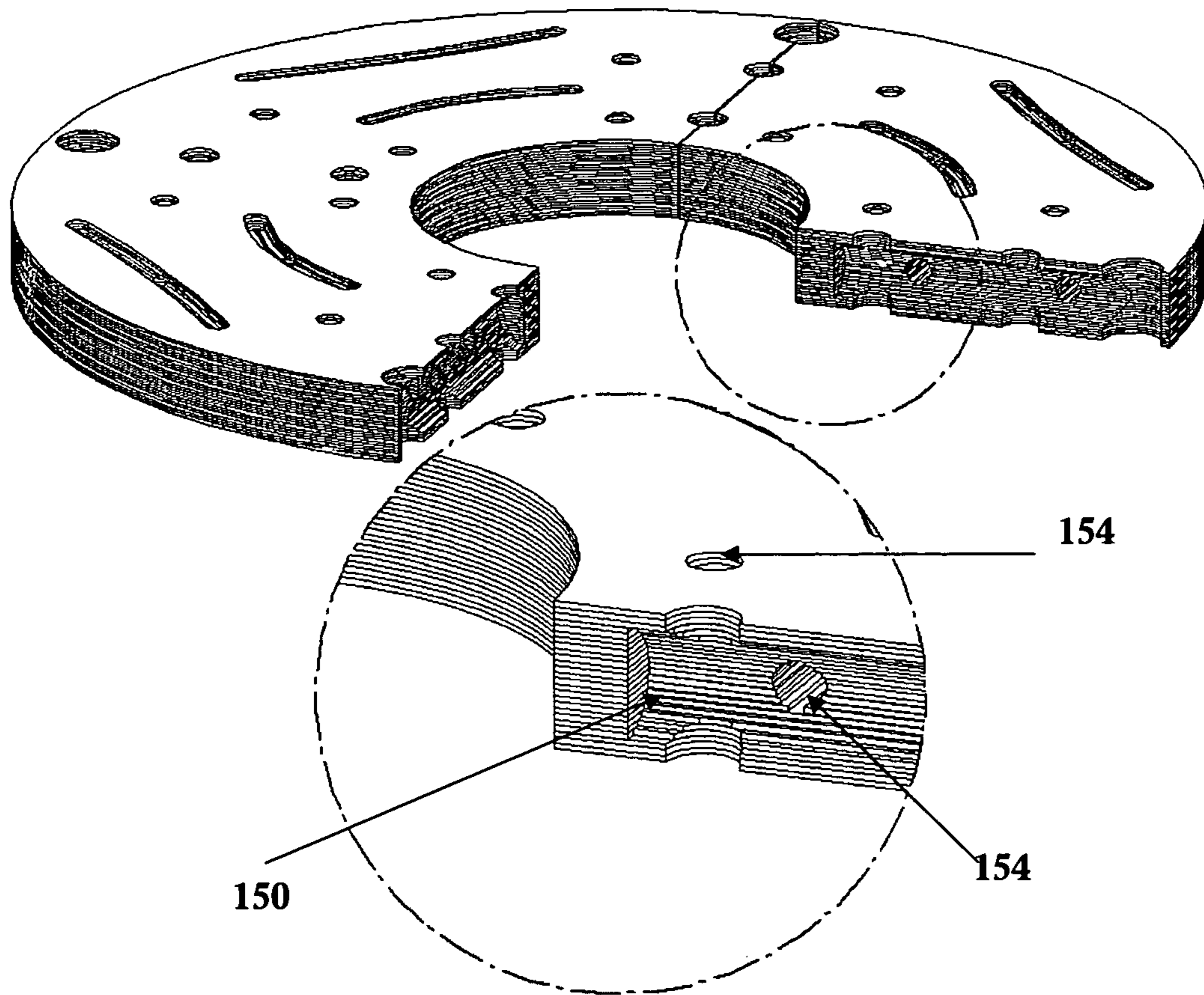
Channel Structure
