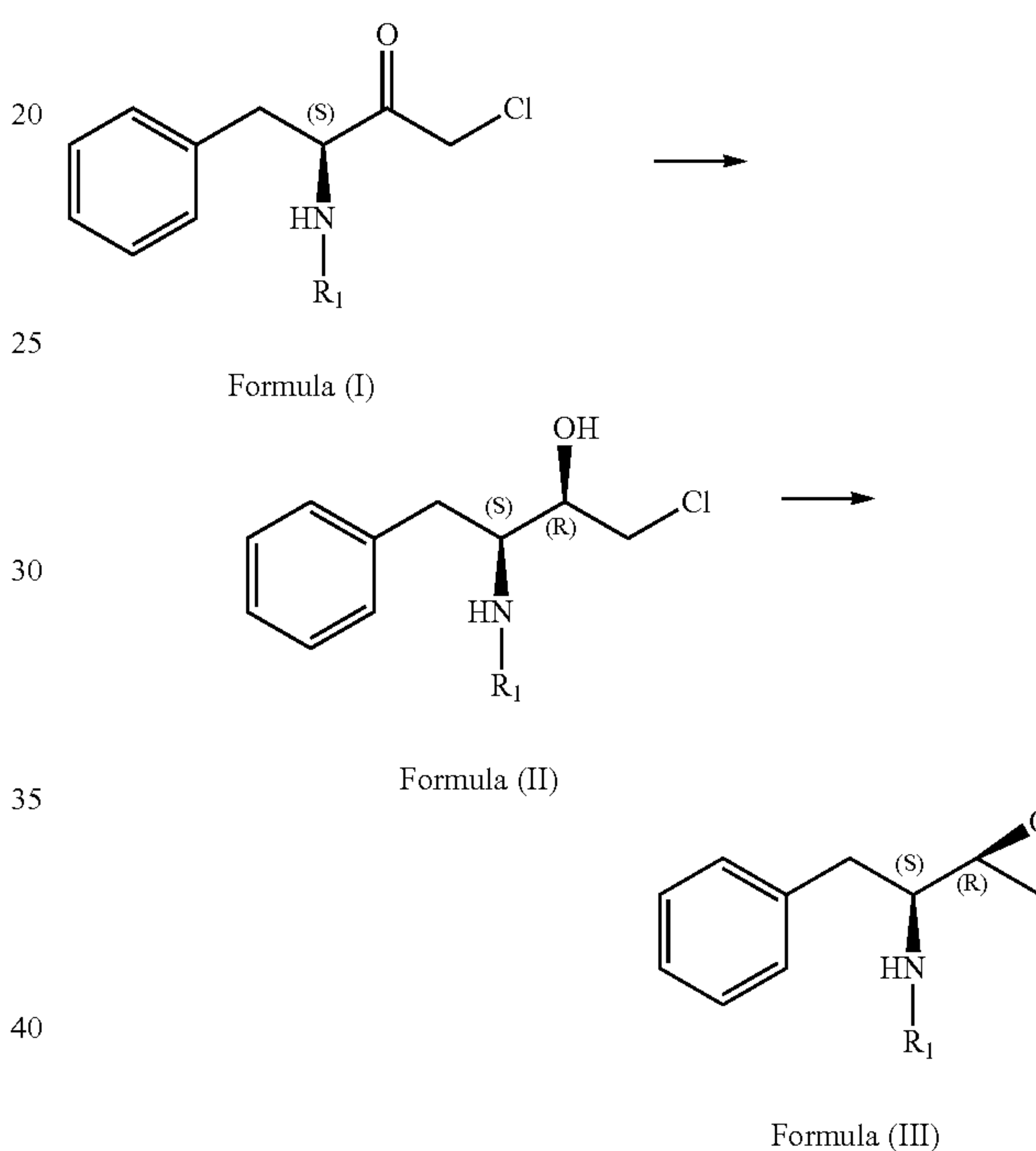
Scheme 3
