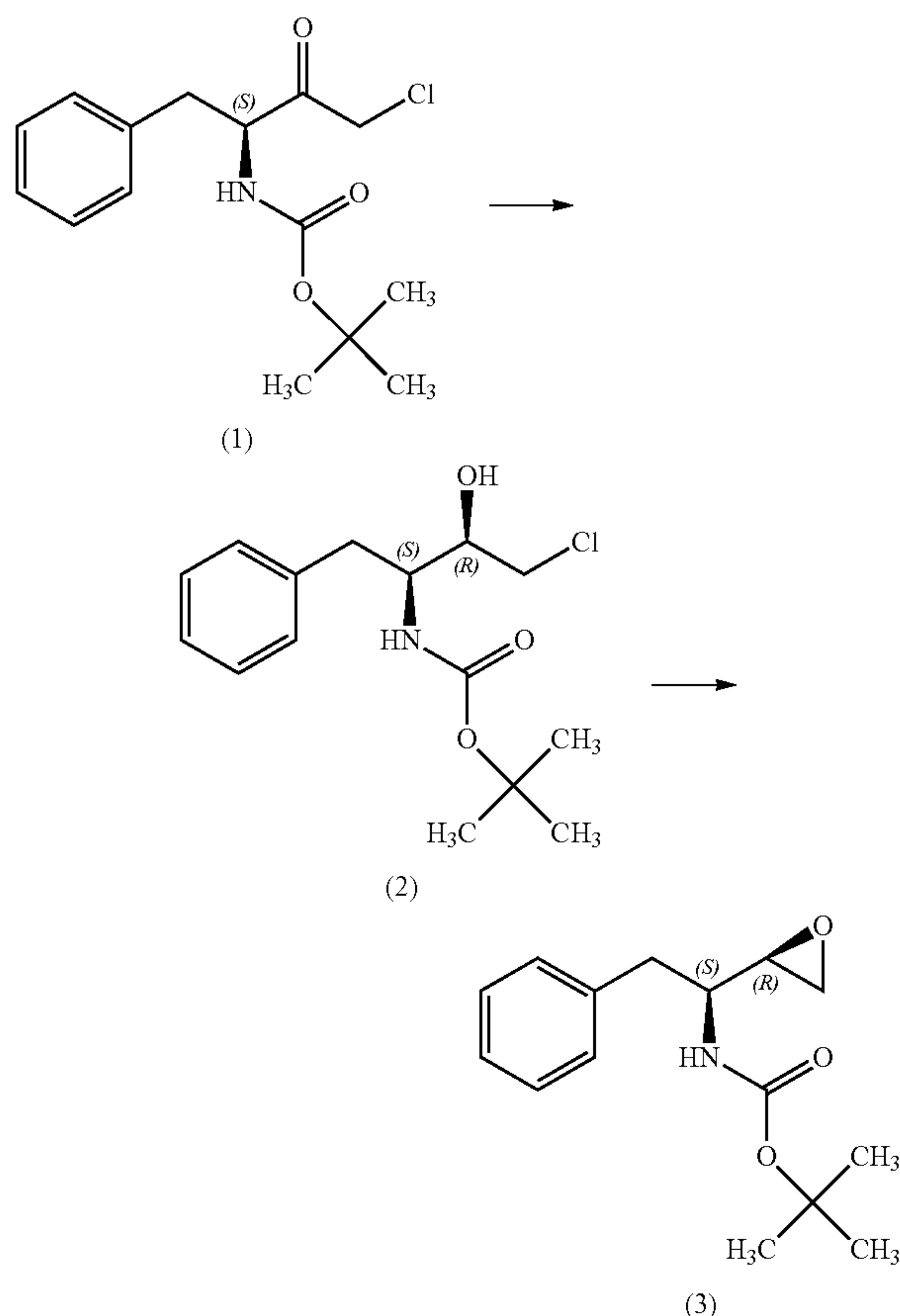
Scheme 4
