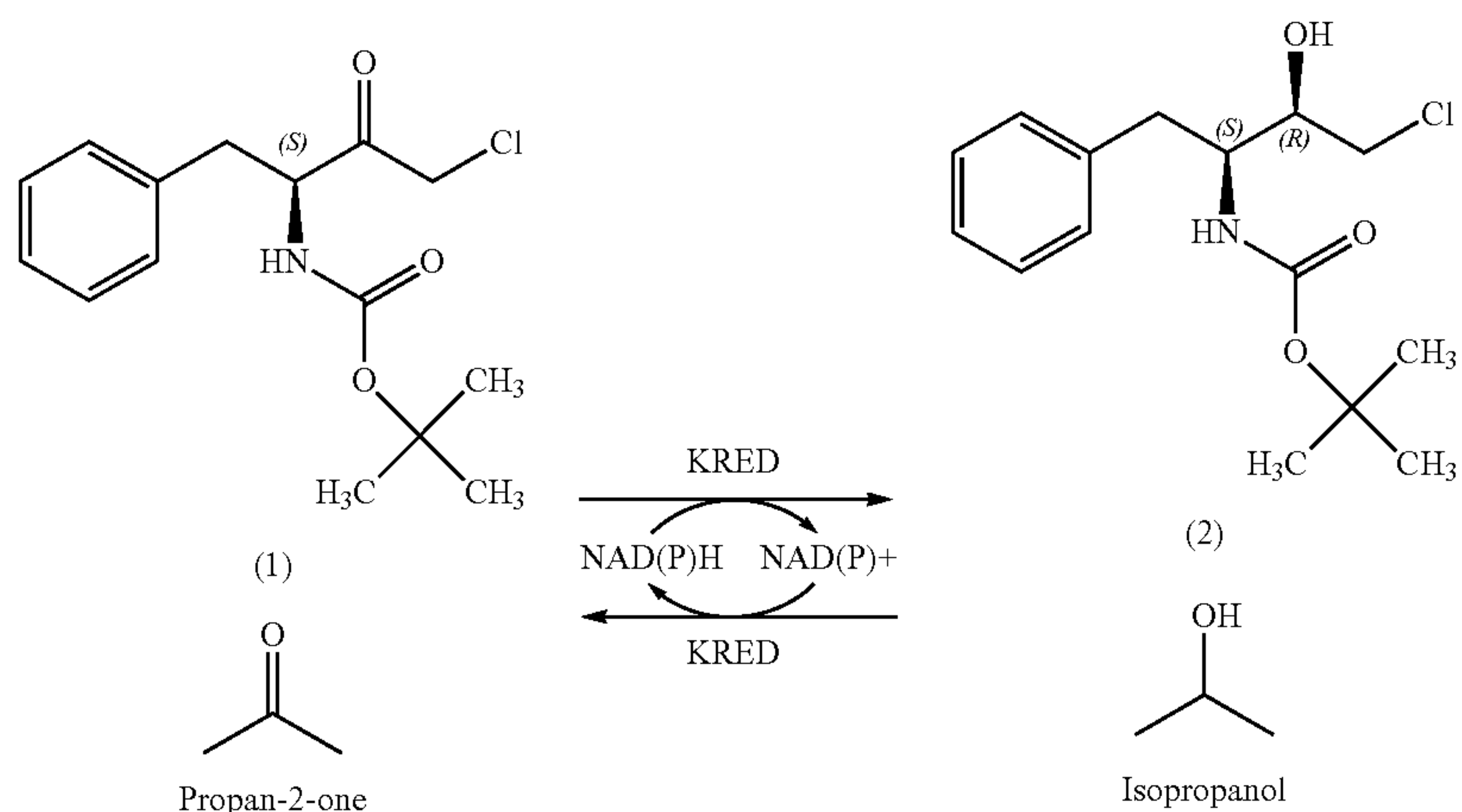
Scheme 7
