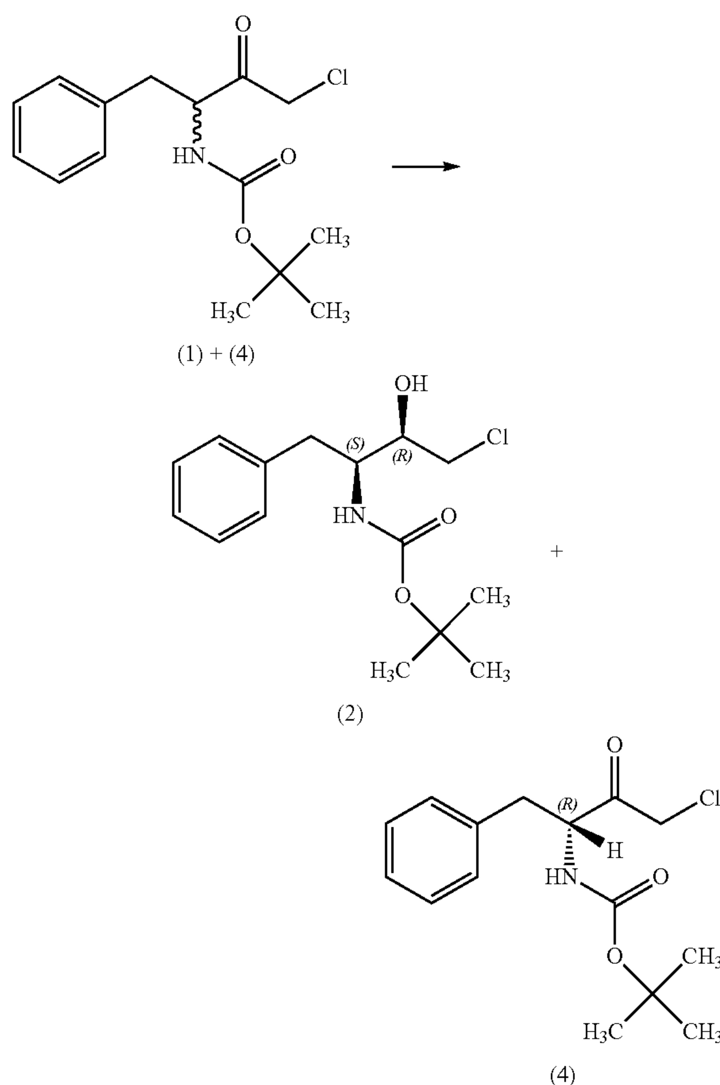
Scheme 5
