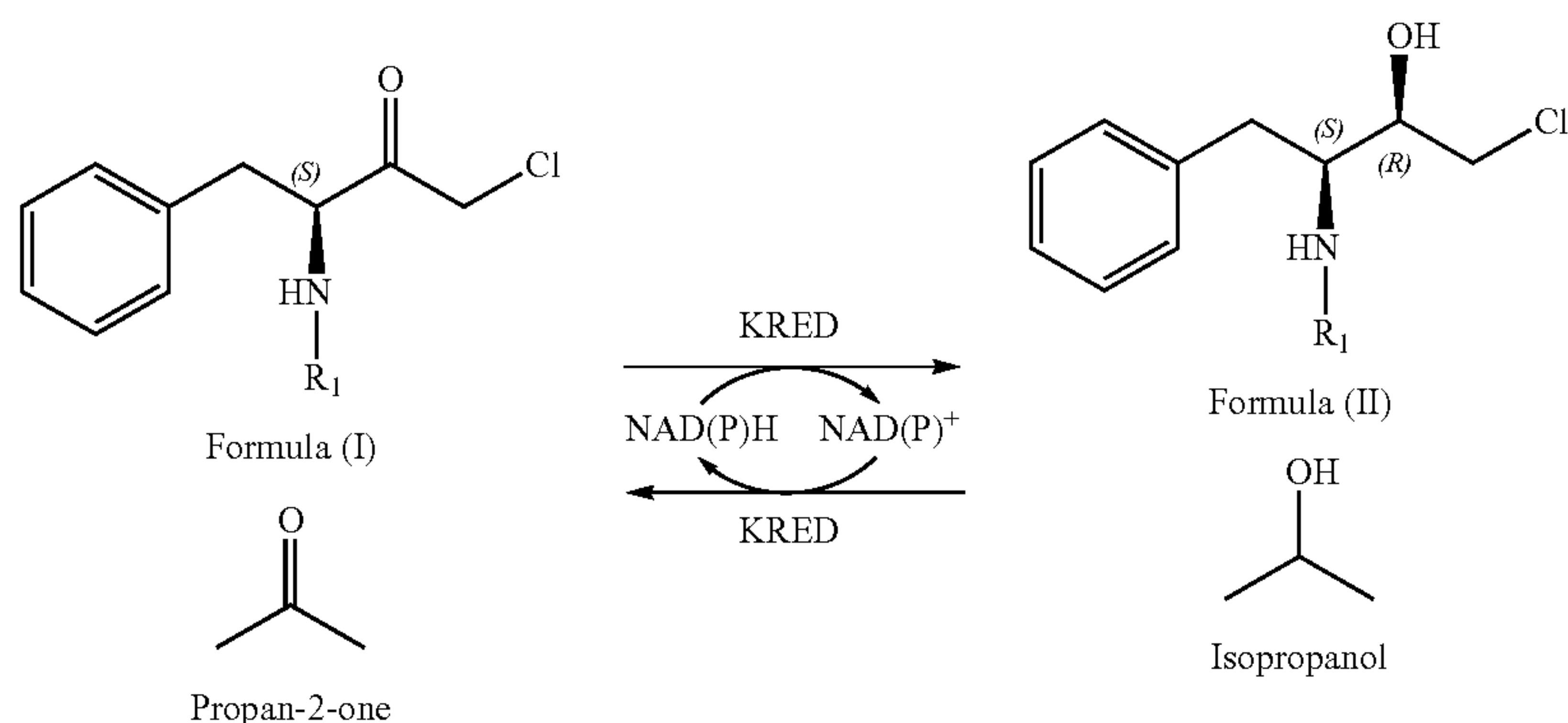
Scheme 6
