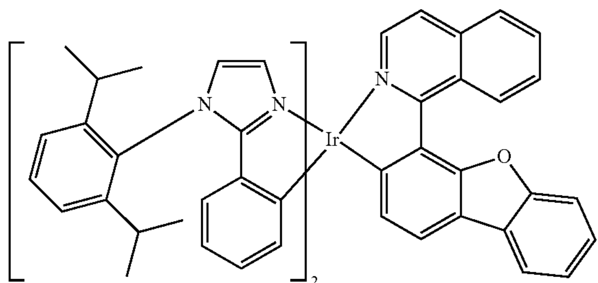
Compound 73
