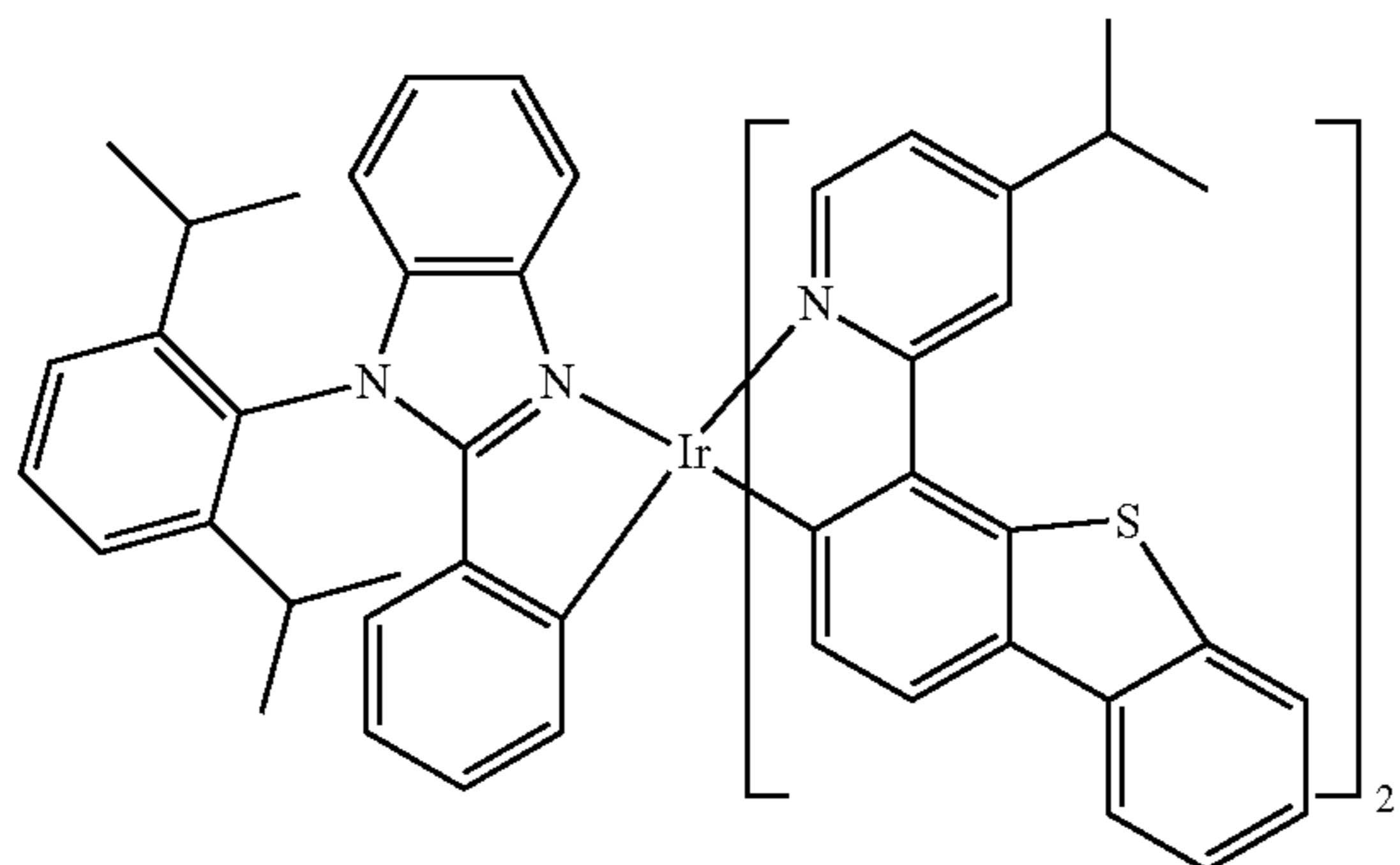
Compound 104
