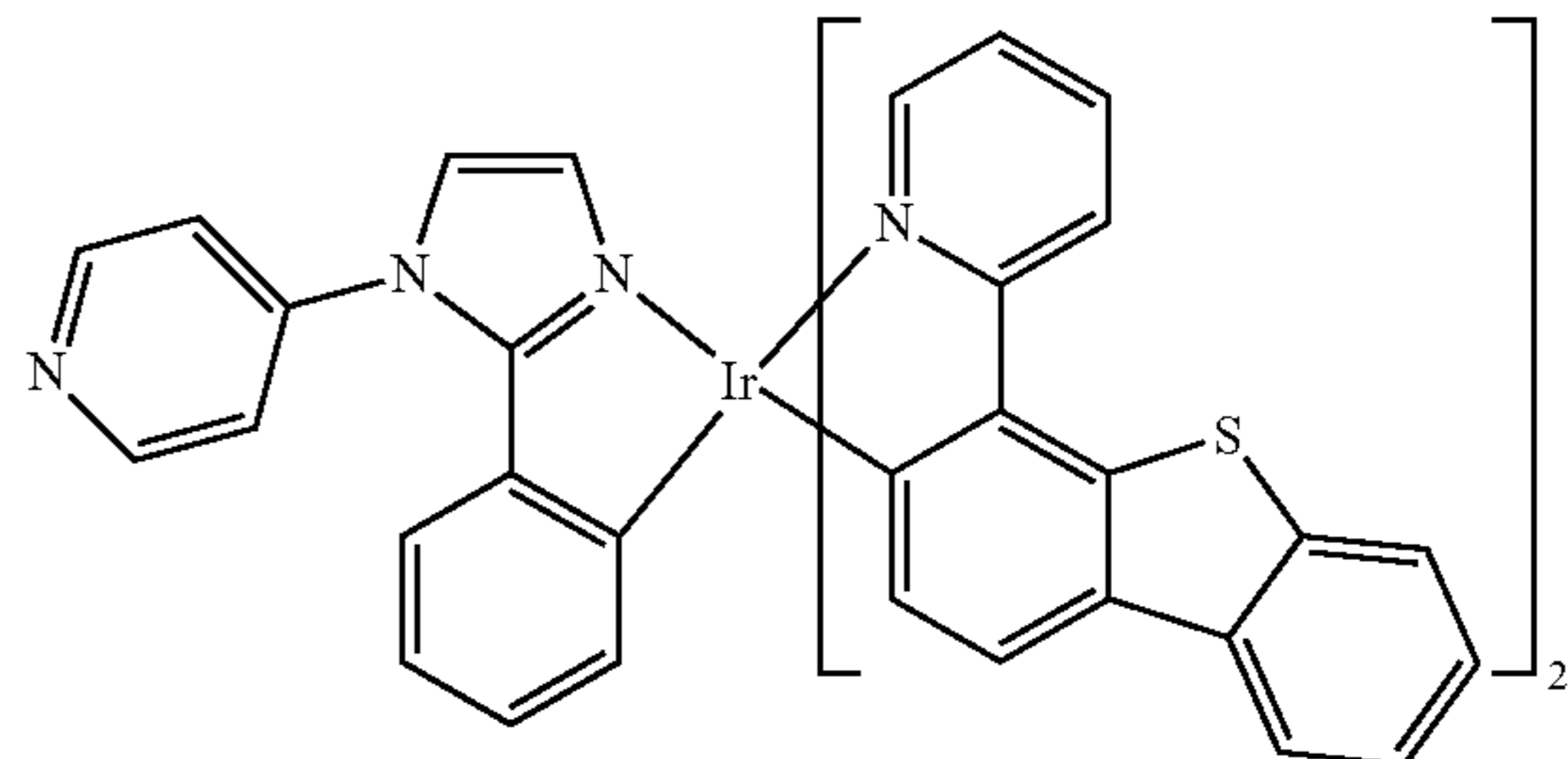
Compound 56
