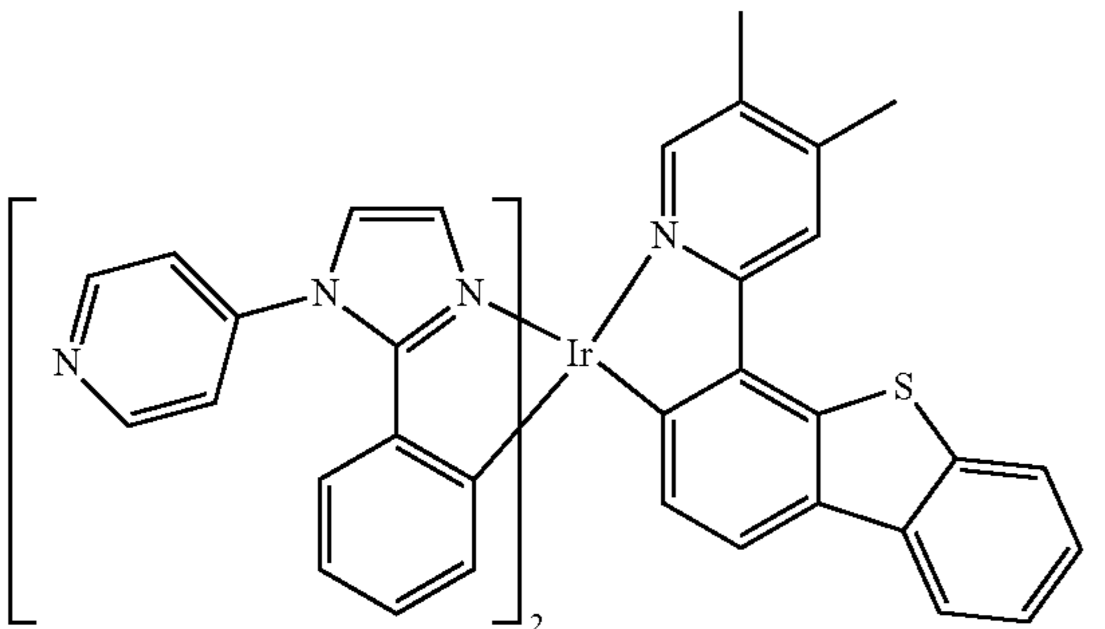
Compound 54
