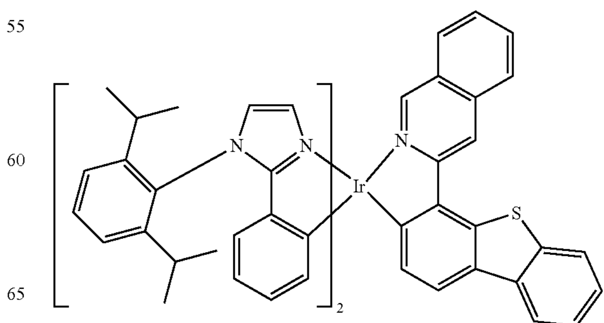
Compound 77
