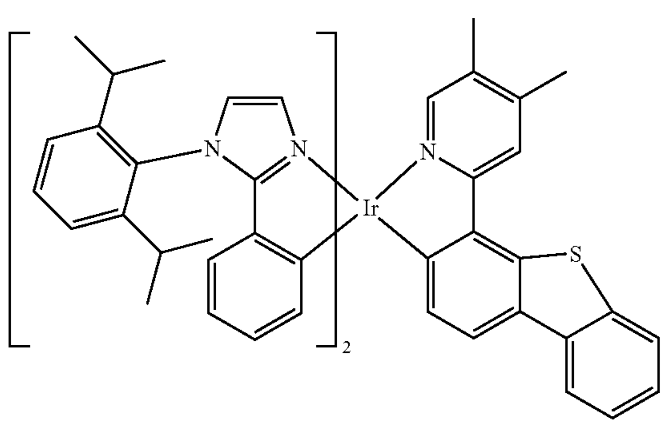
Compound 18
