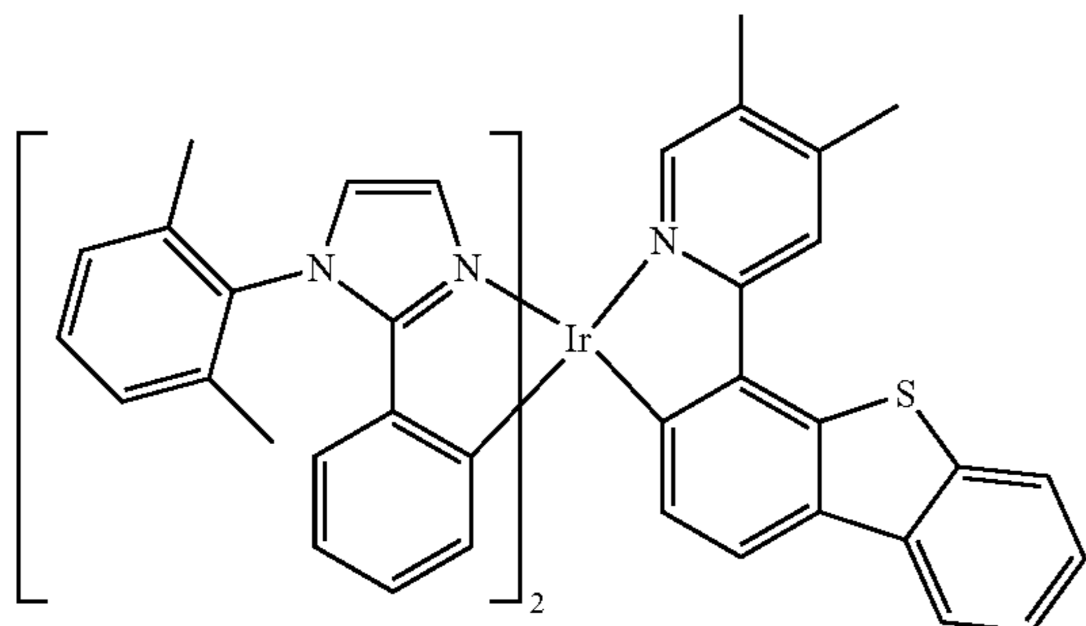
Compound 51
