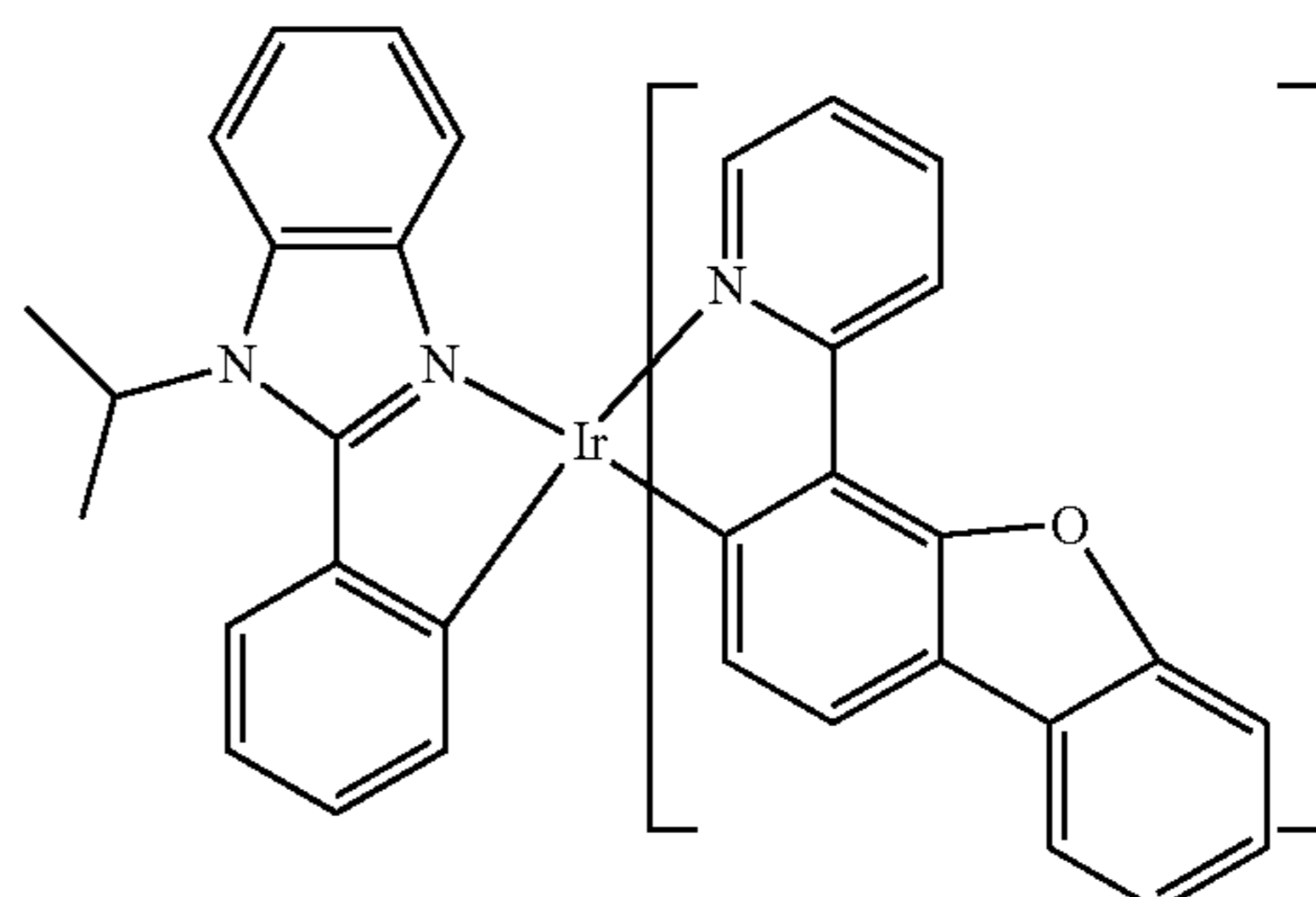
Compound 123
