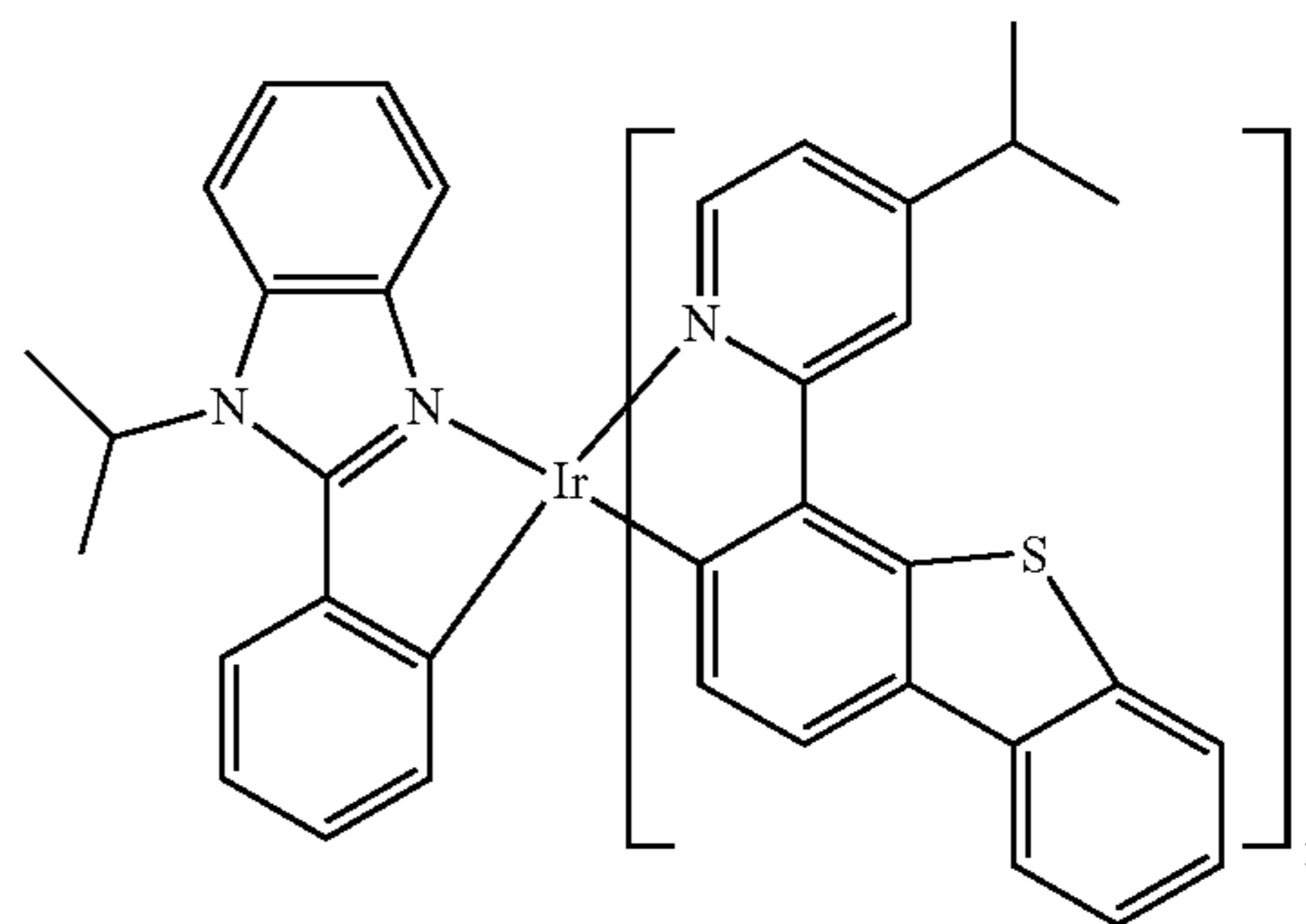
Compound 144
