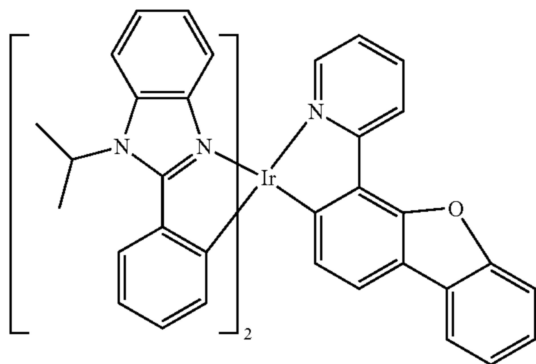
Compound 121
