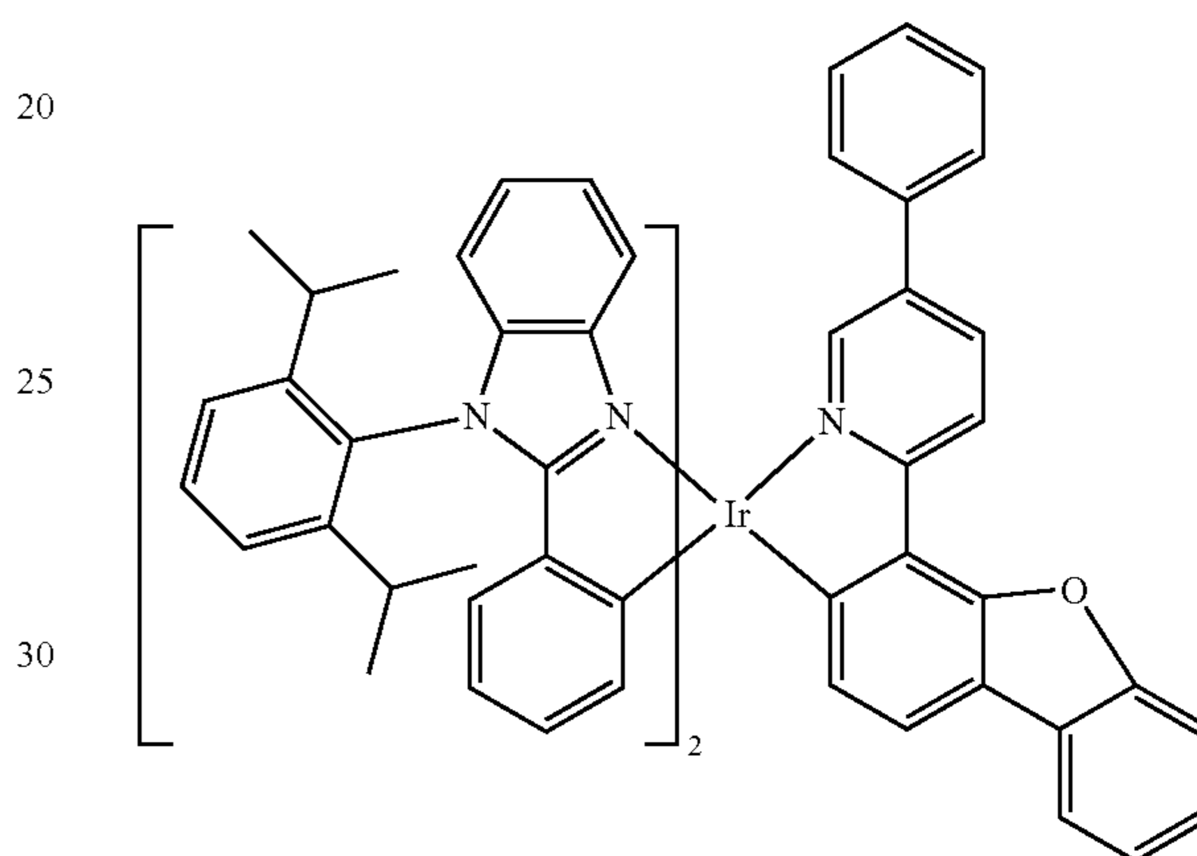
Compound 148
