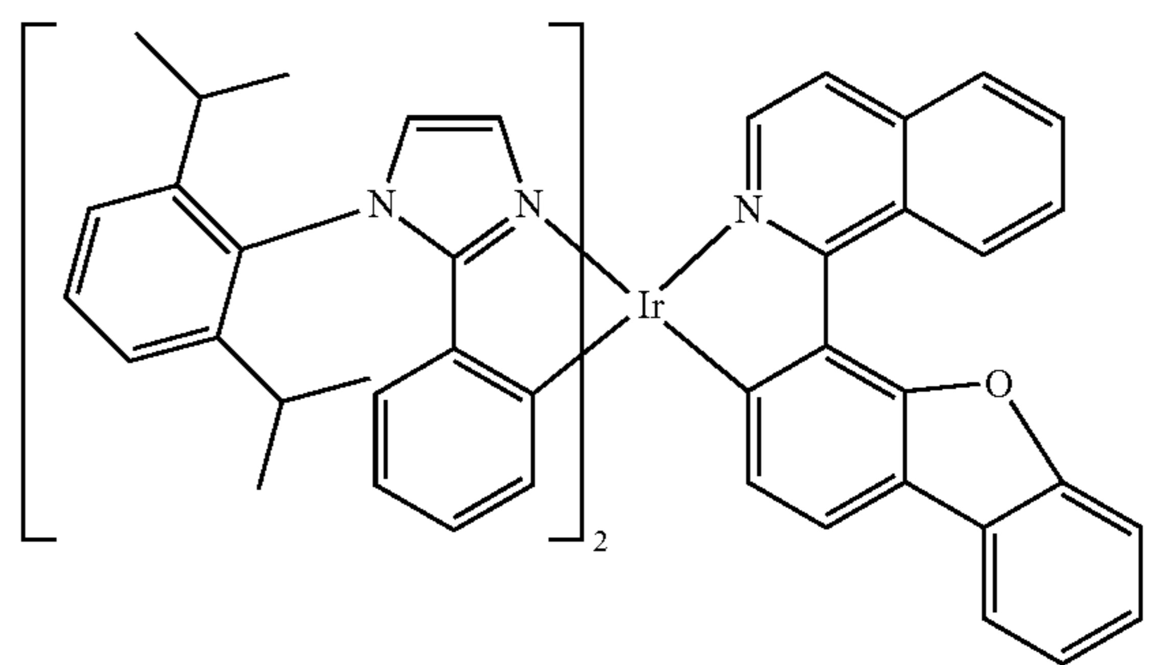
Compound 71
