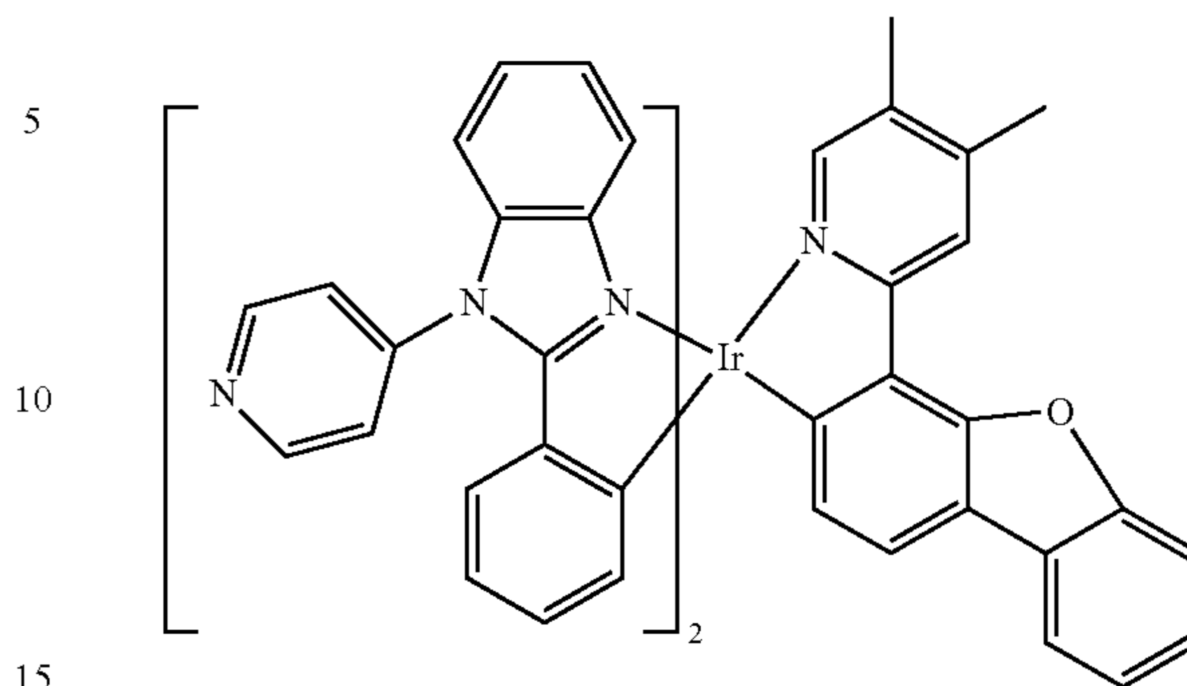
Compound 118
