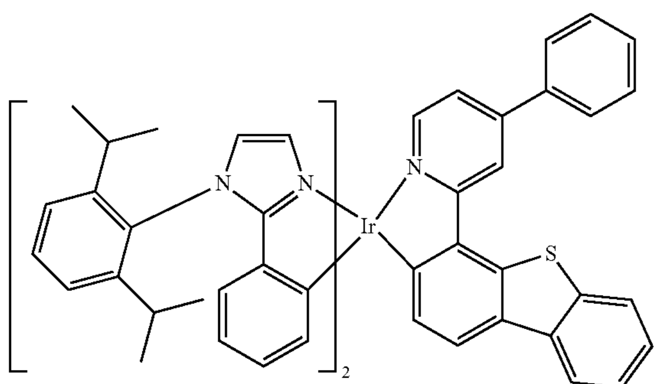
Compound 74
