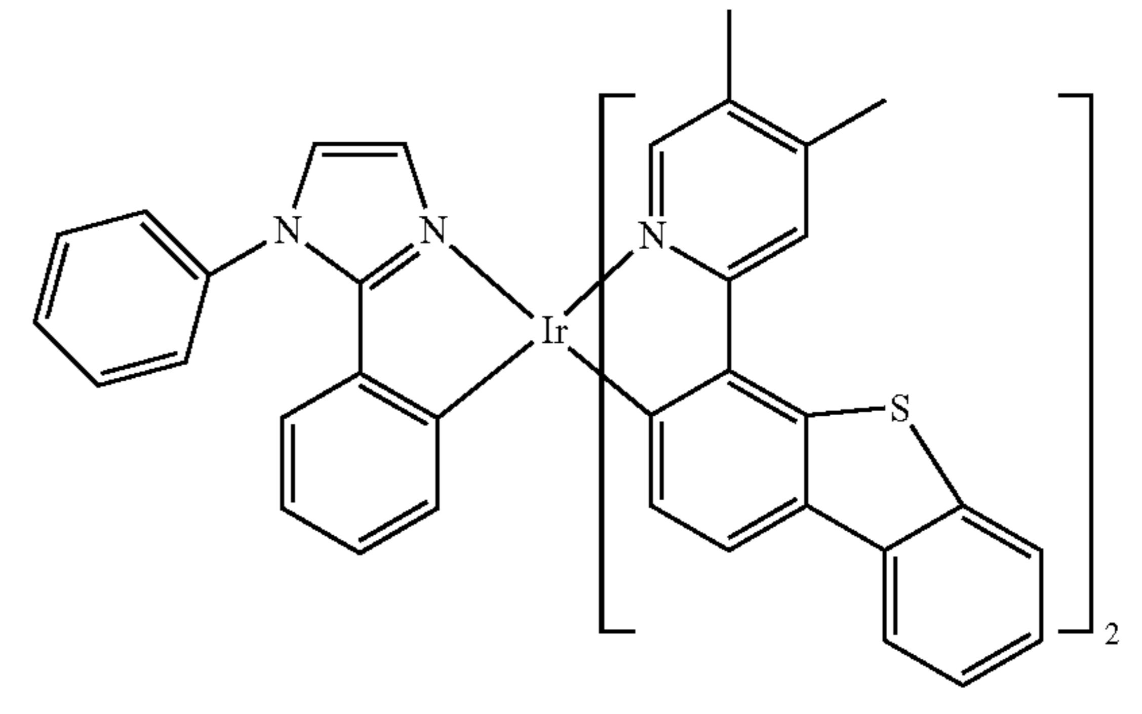
Compound 29
