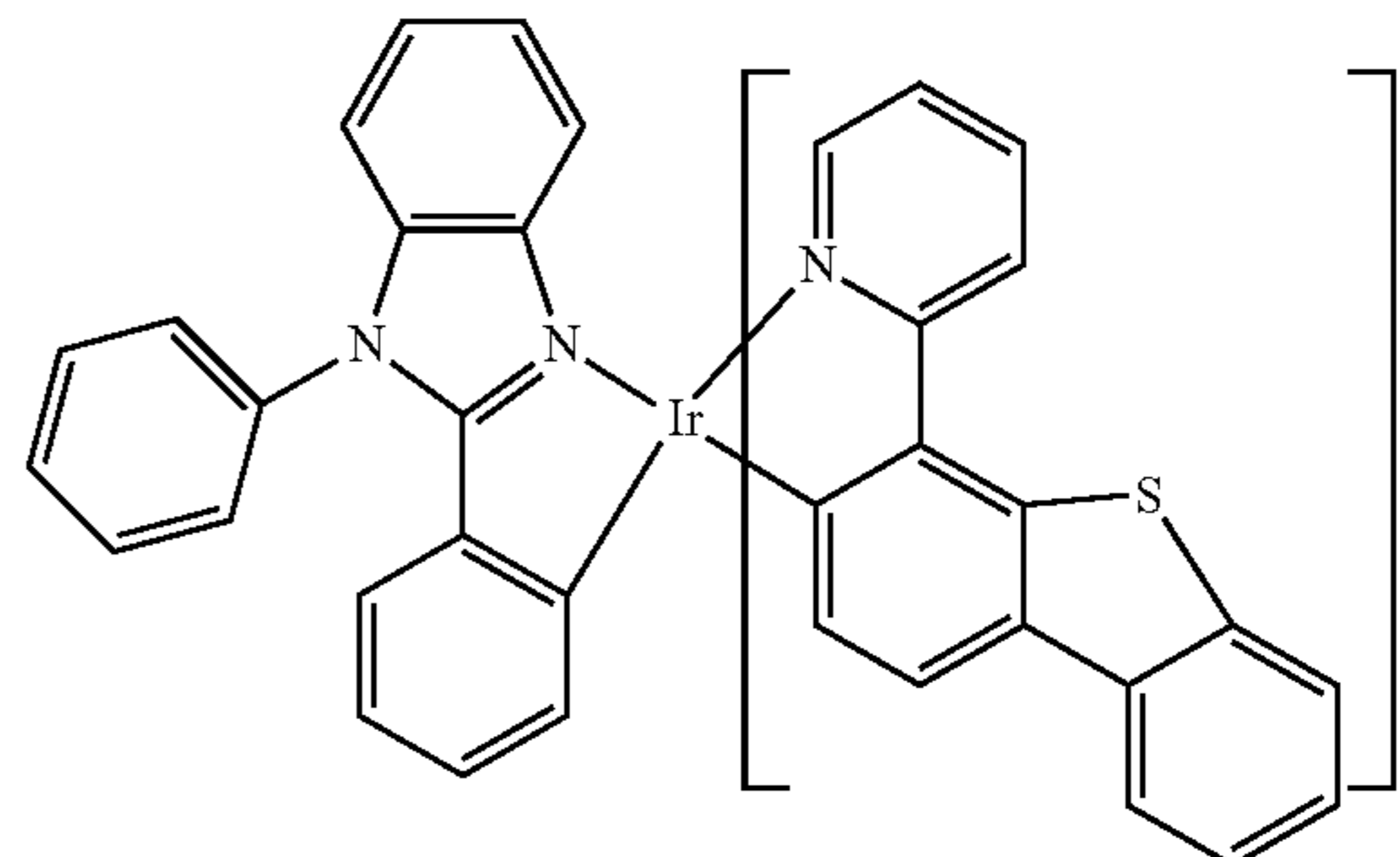
Compound 107
