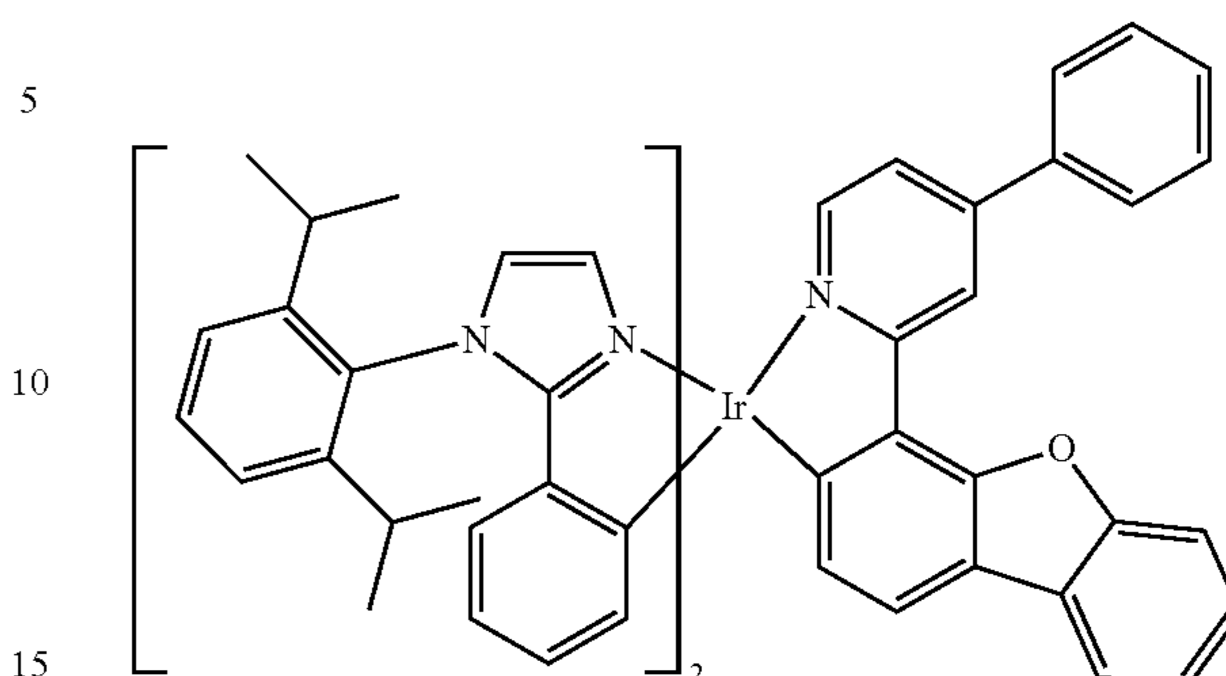
Compound 66
