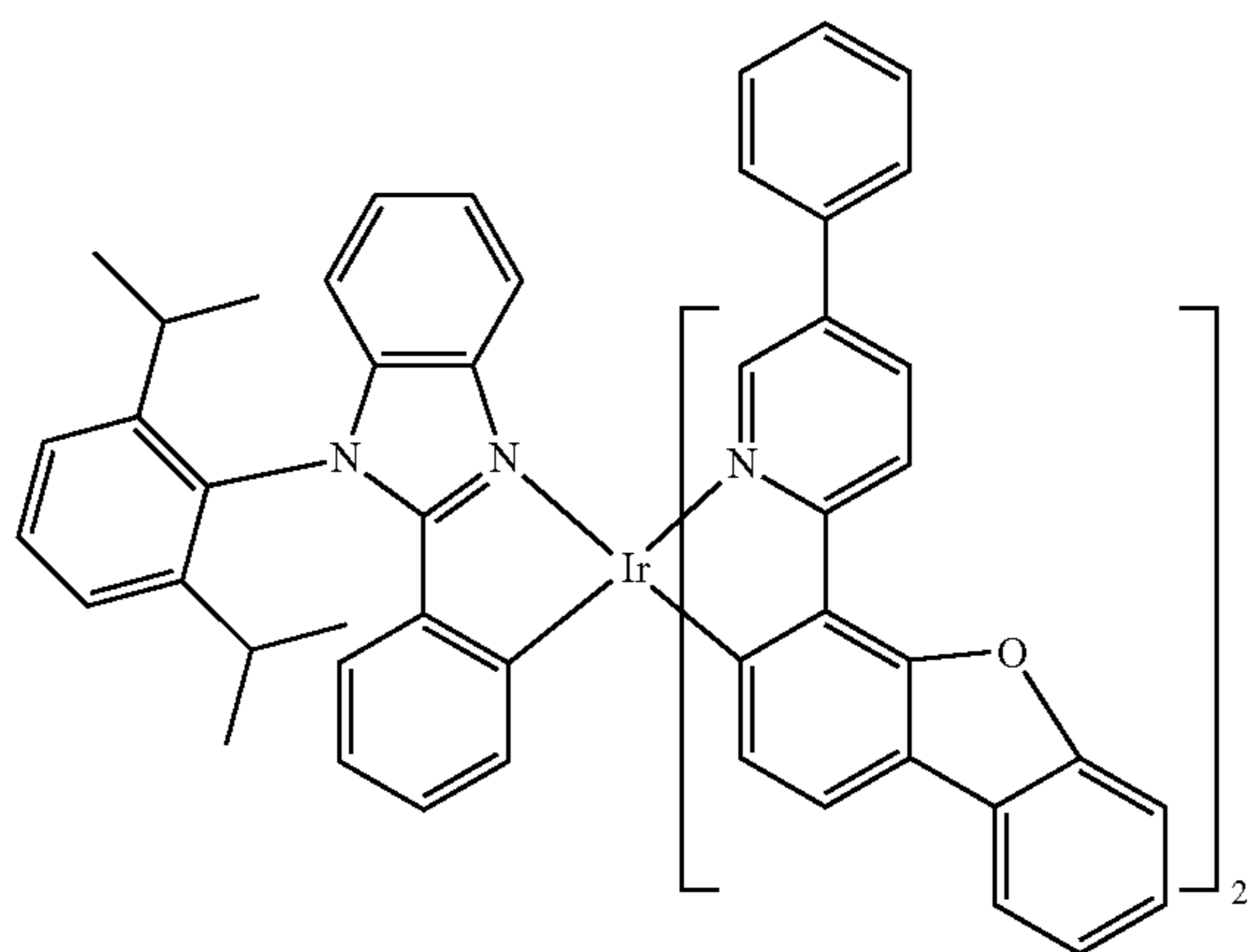
Compound 149
