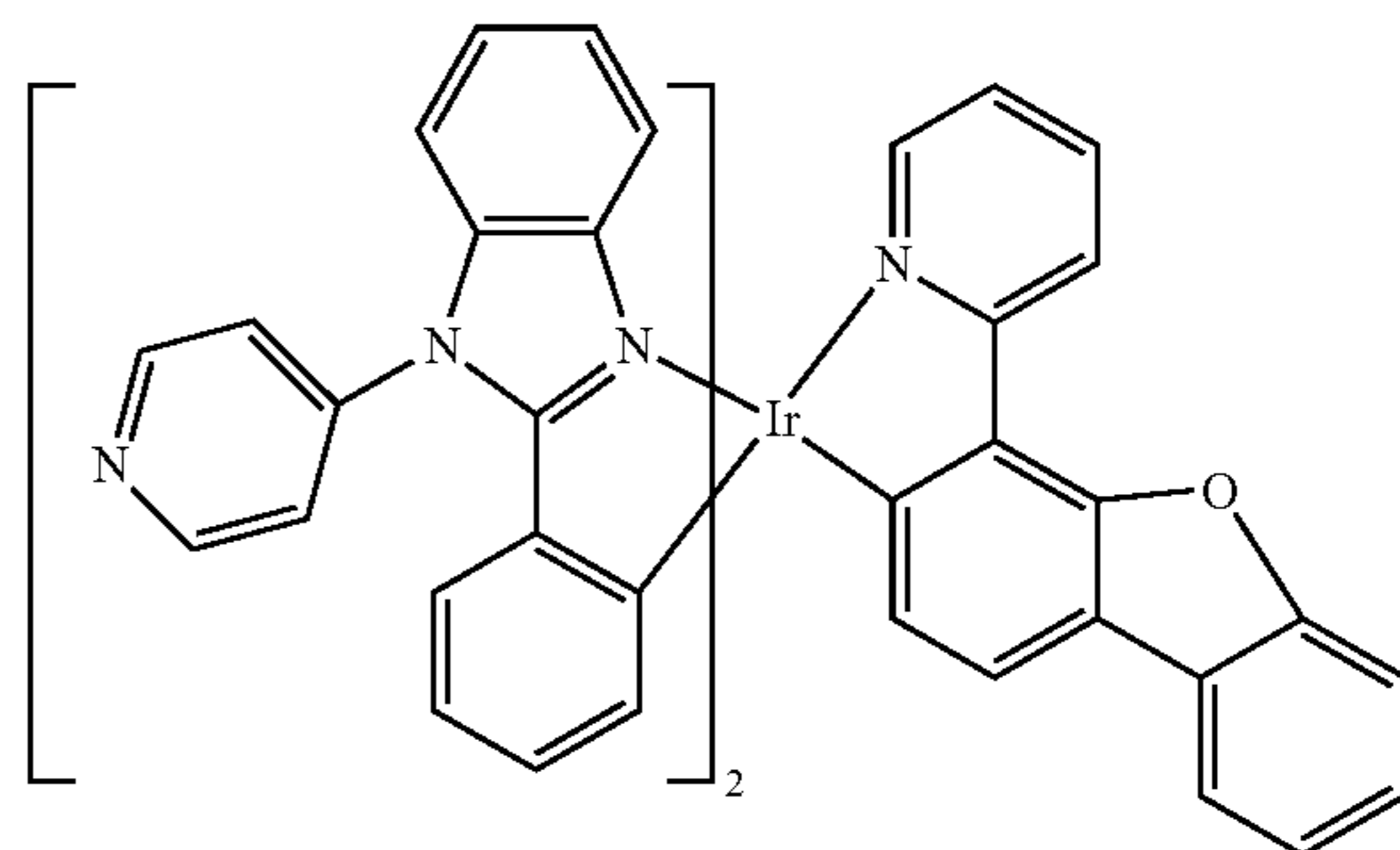
Compound 1117
