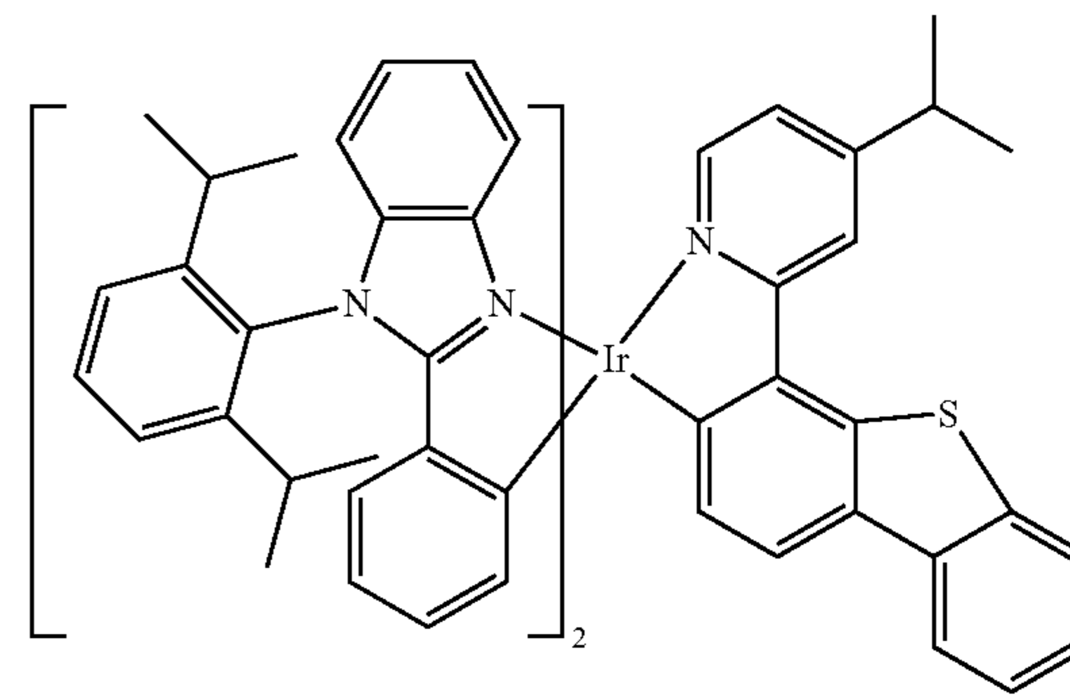
Compound 102
