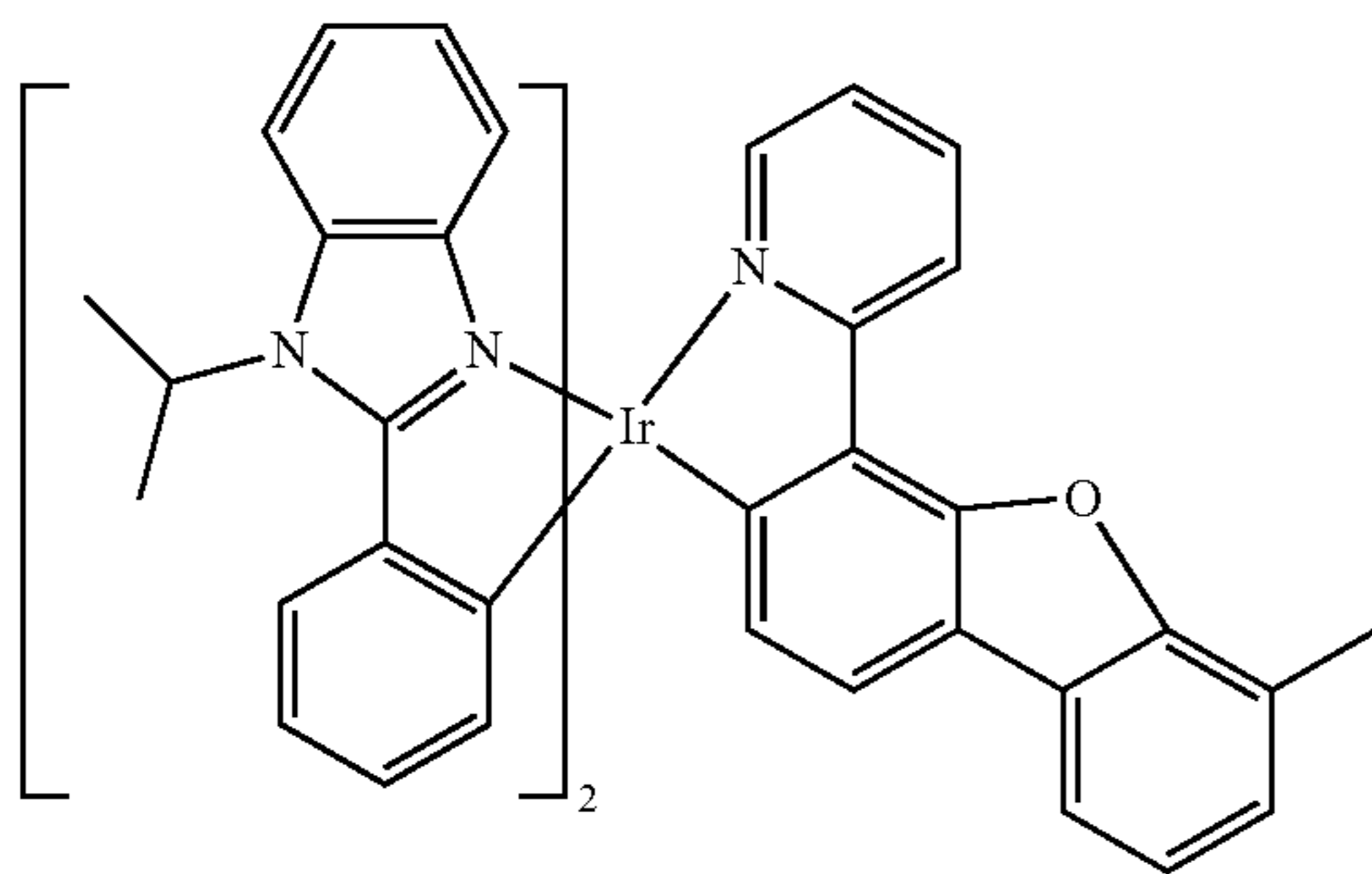
Compound 125
