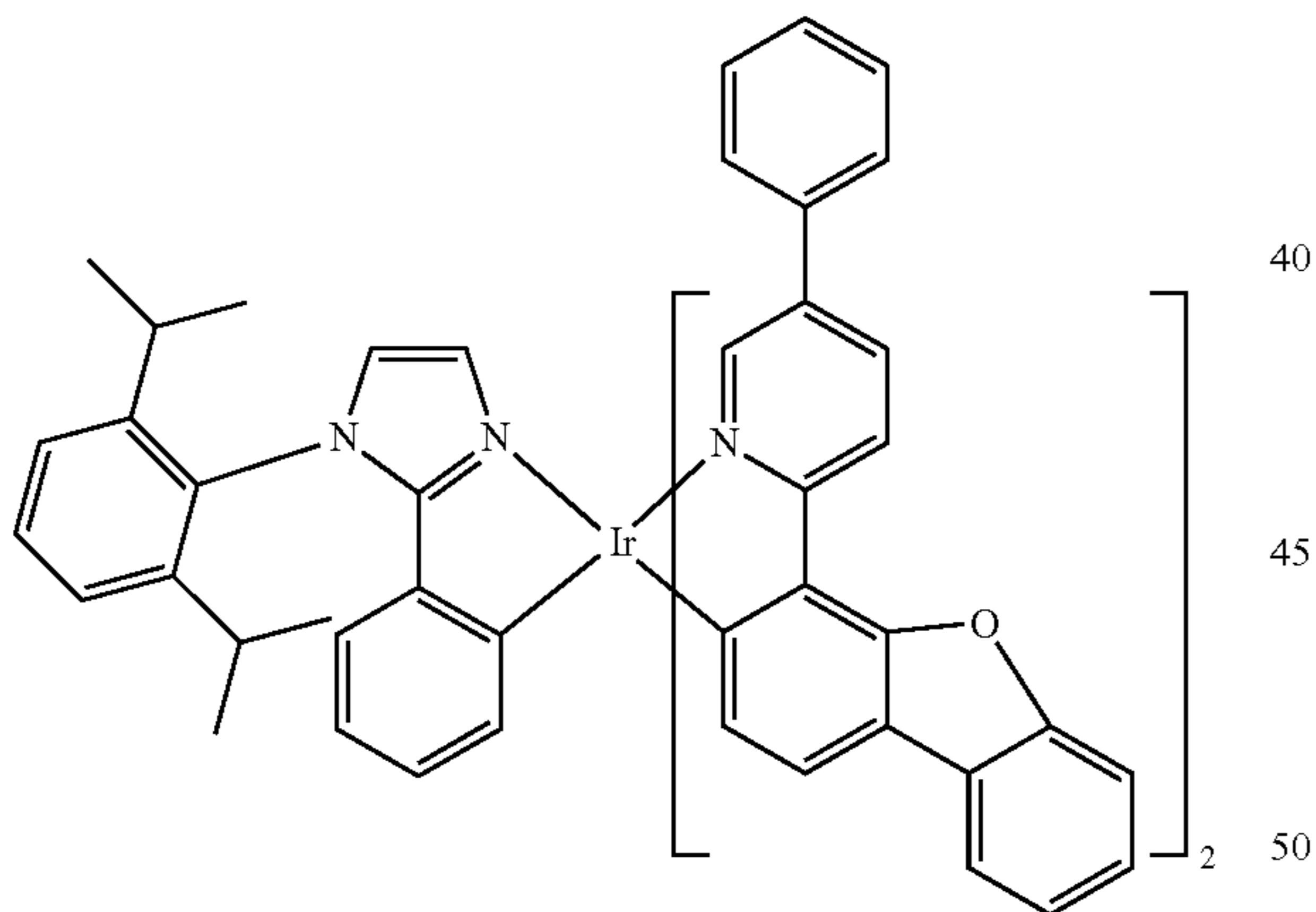
Compound 69
