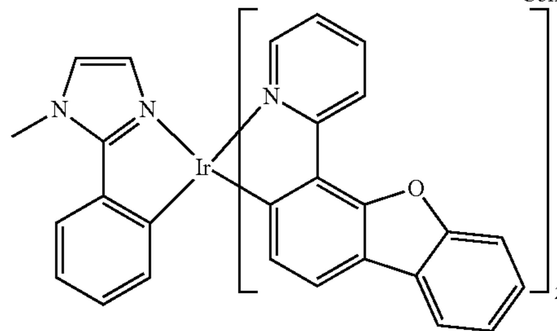
Compound 16
