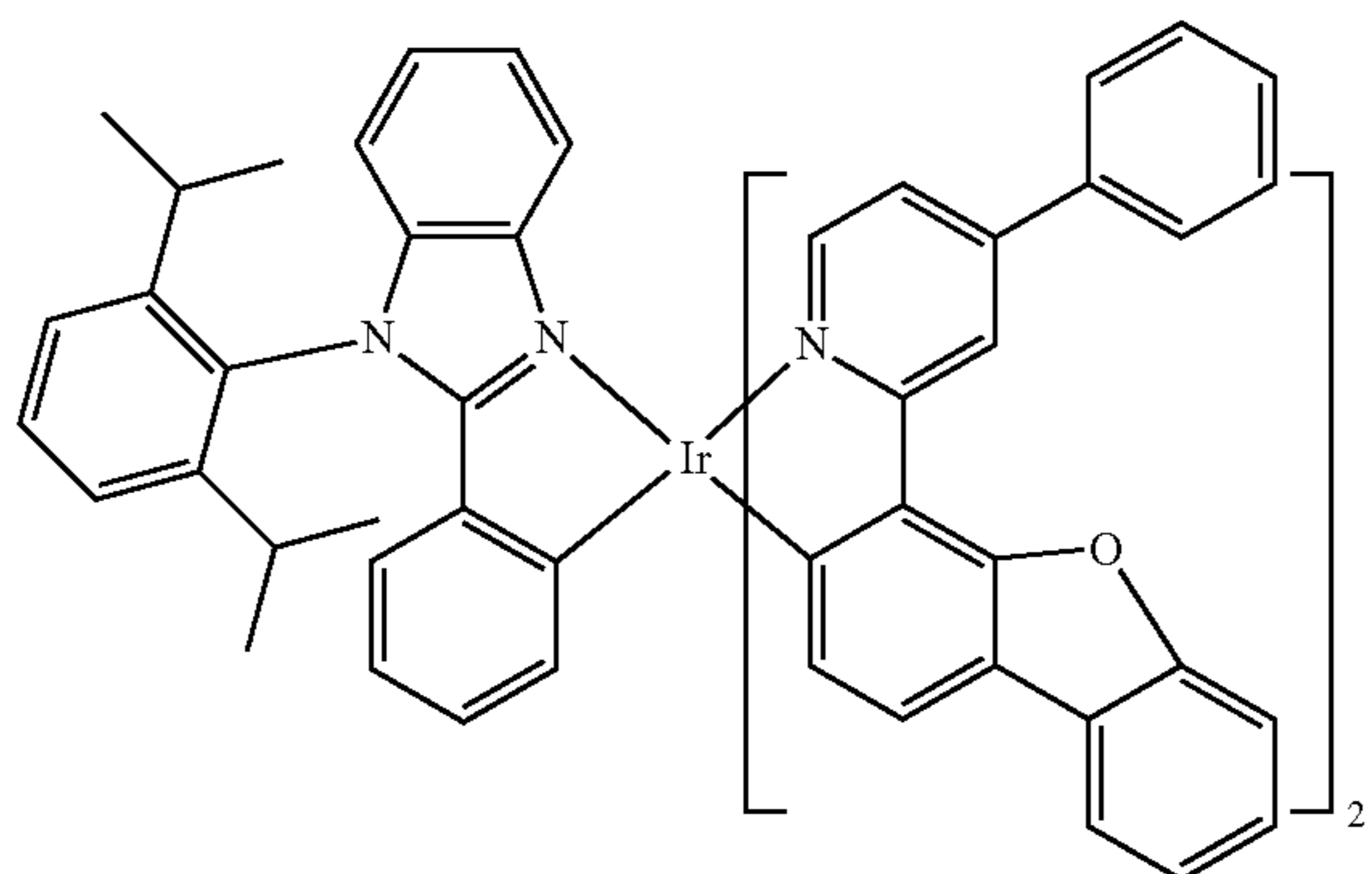
Compound 147
