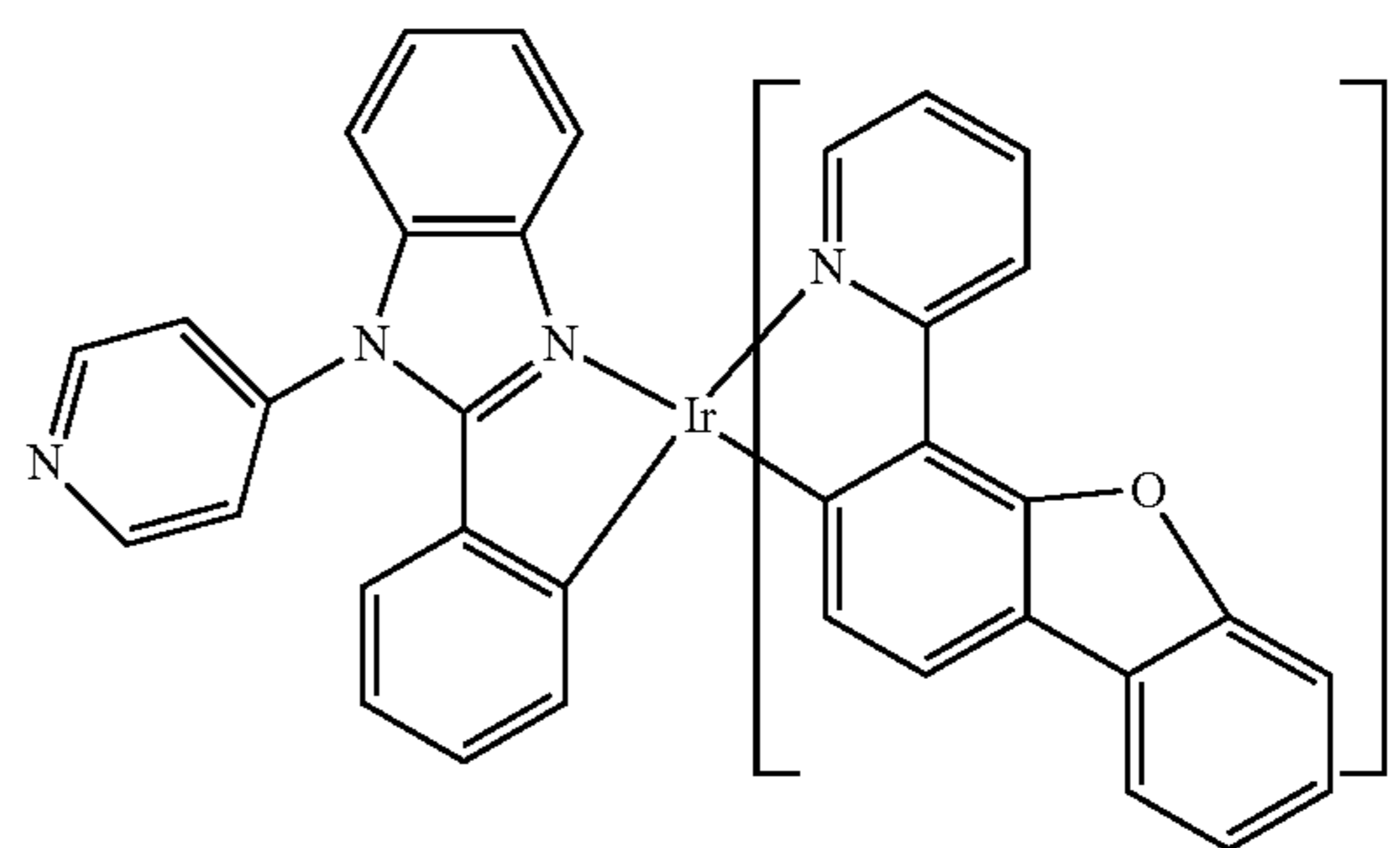
Compound 119
