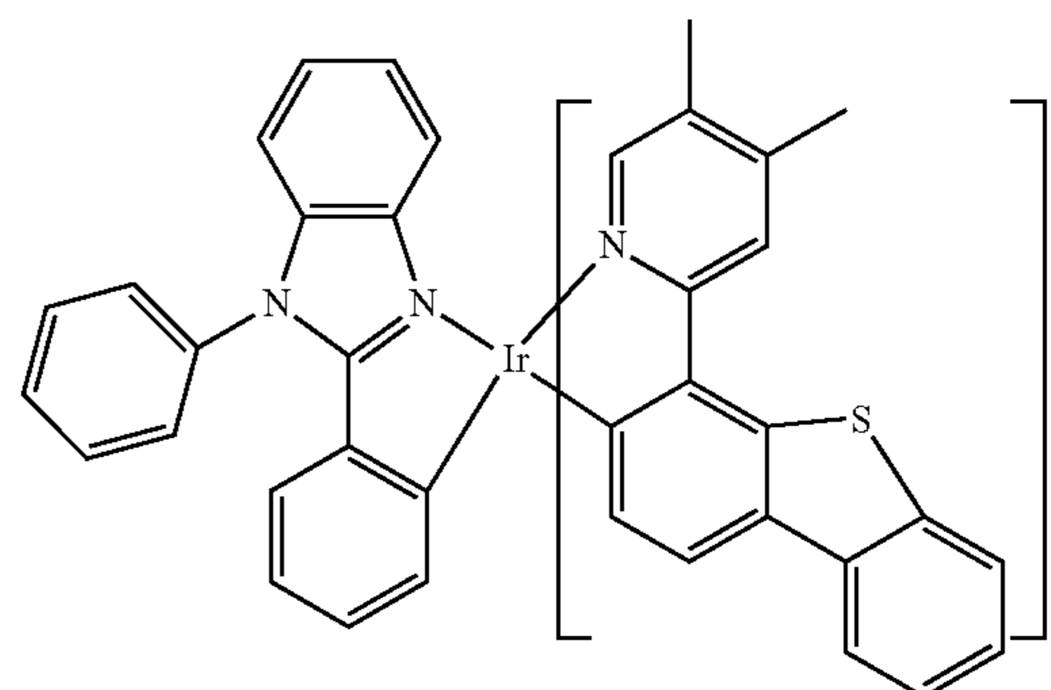
Compound 108
