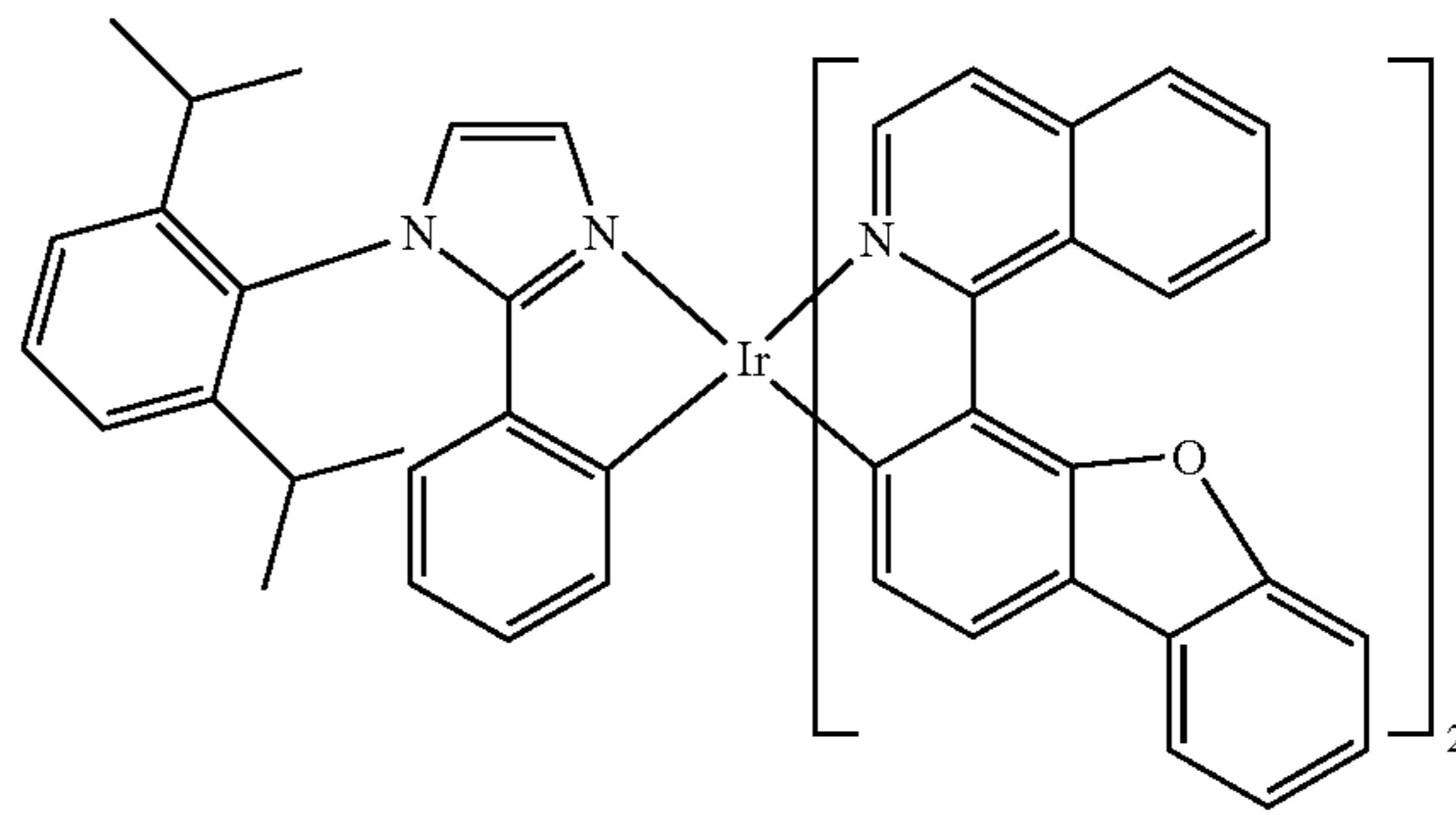
Compound 72
