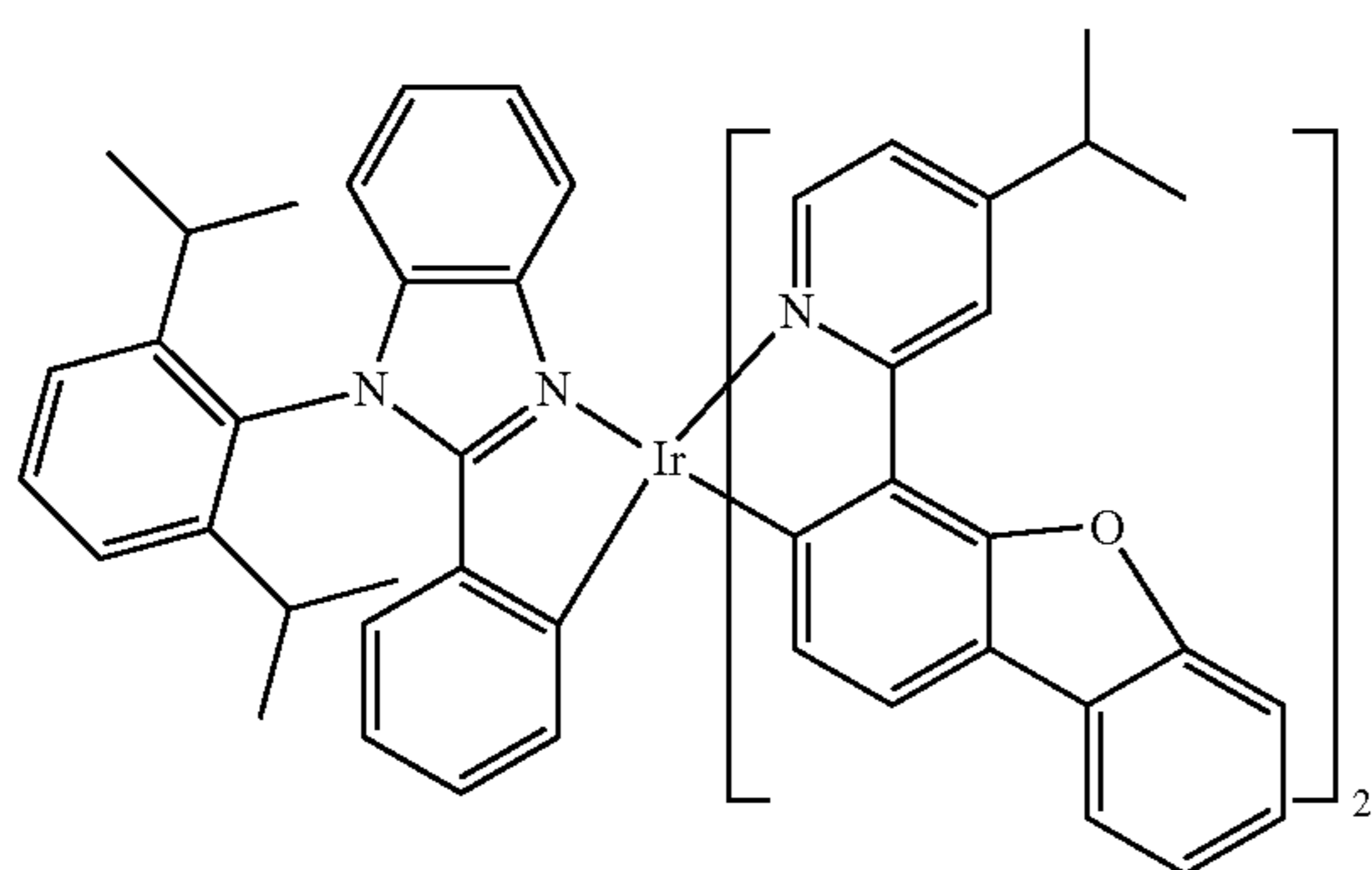
Compound 88
