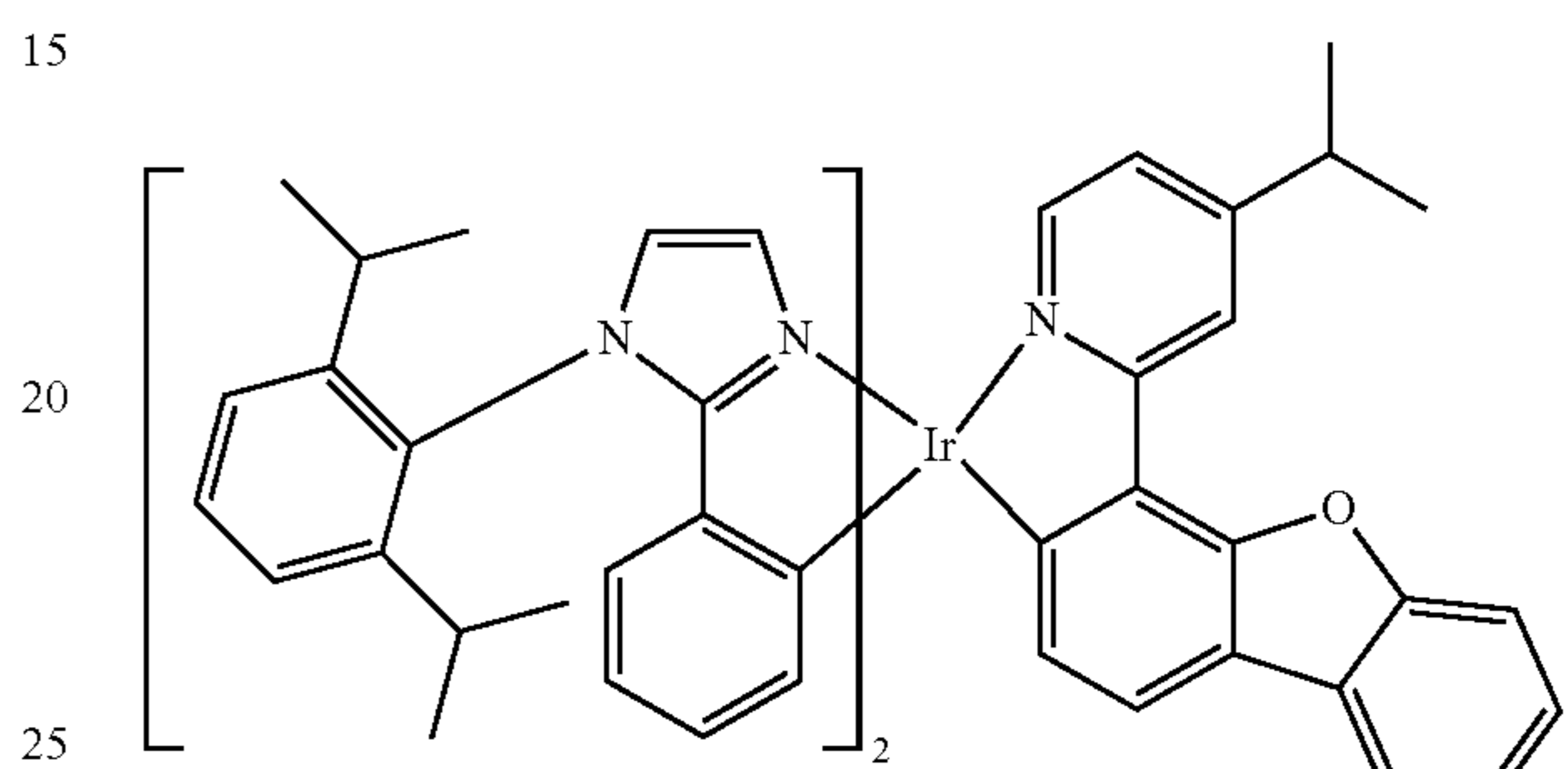
Compound 7
