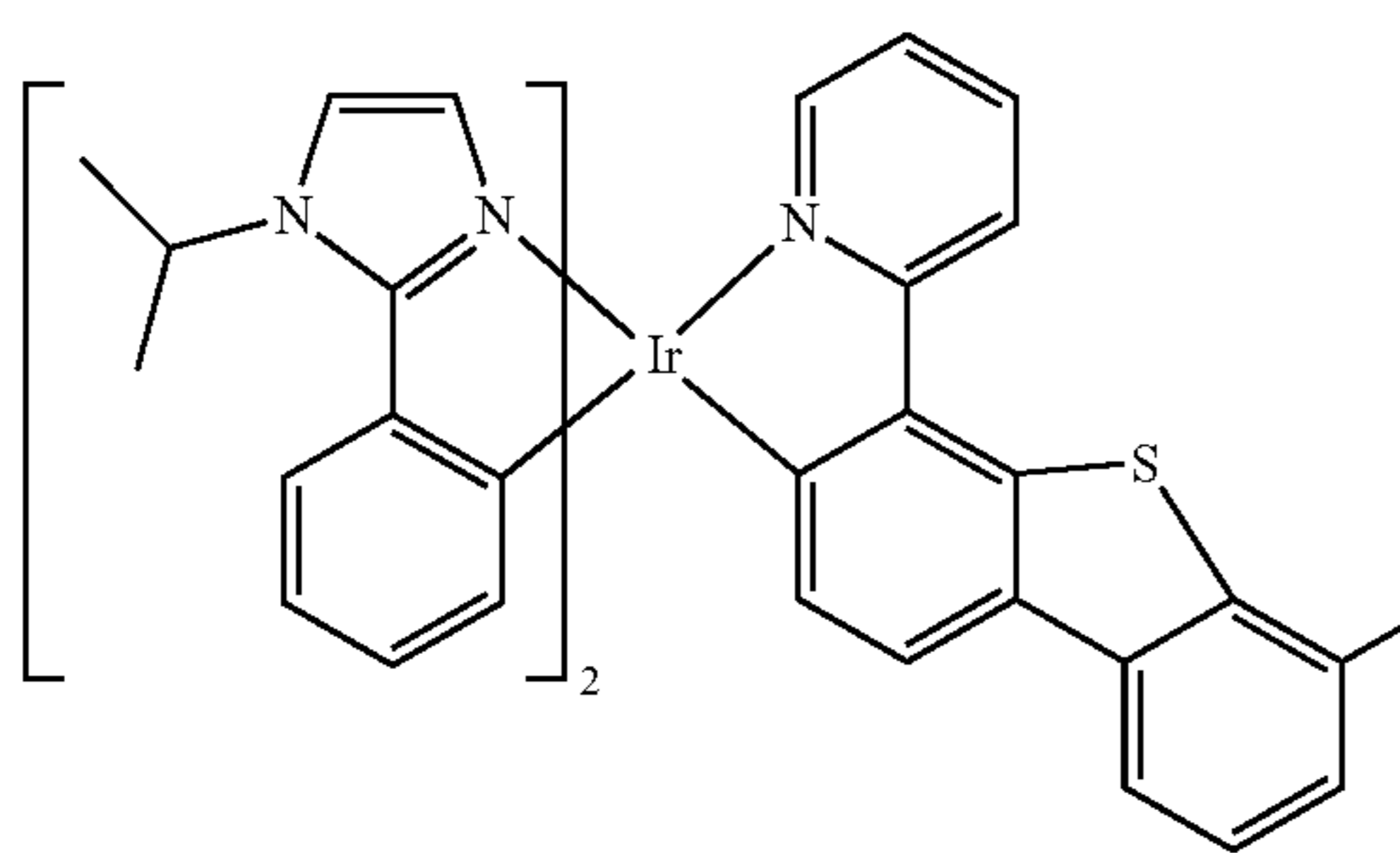
Compound 61
