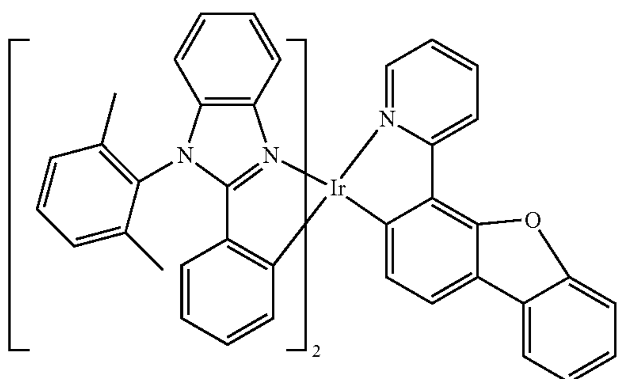
Compound 113
