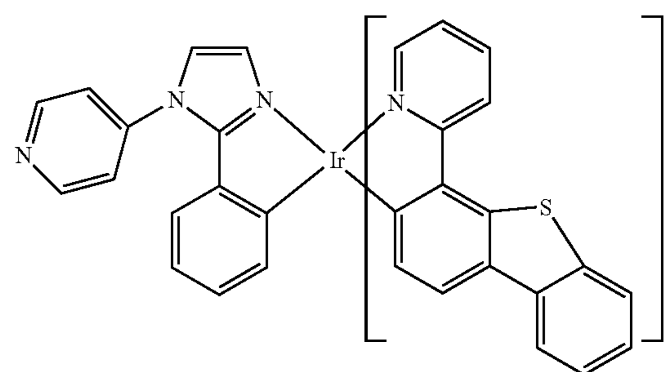
Compound 55
