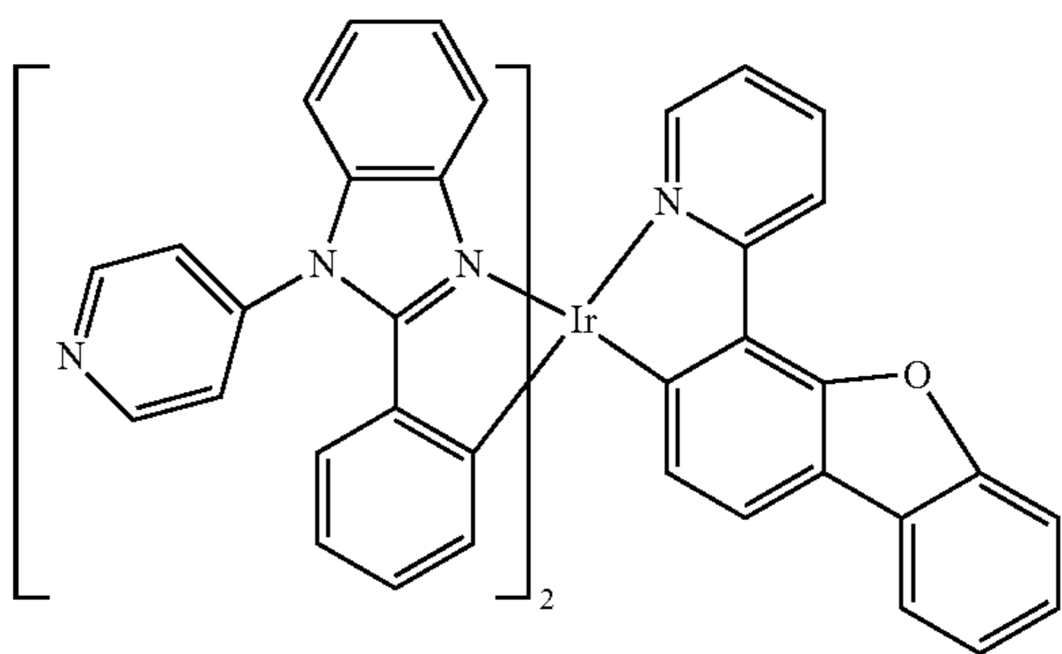
Compound 1117
