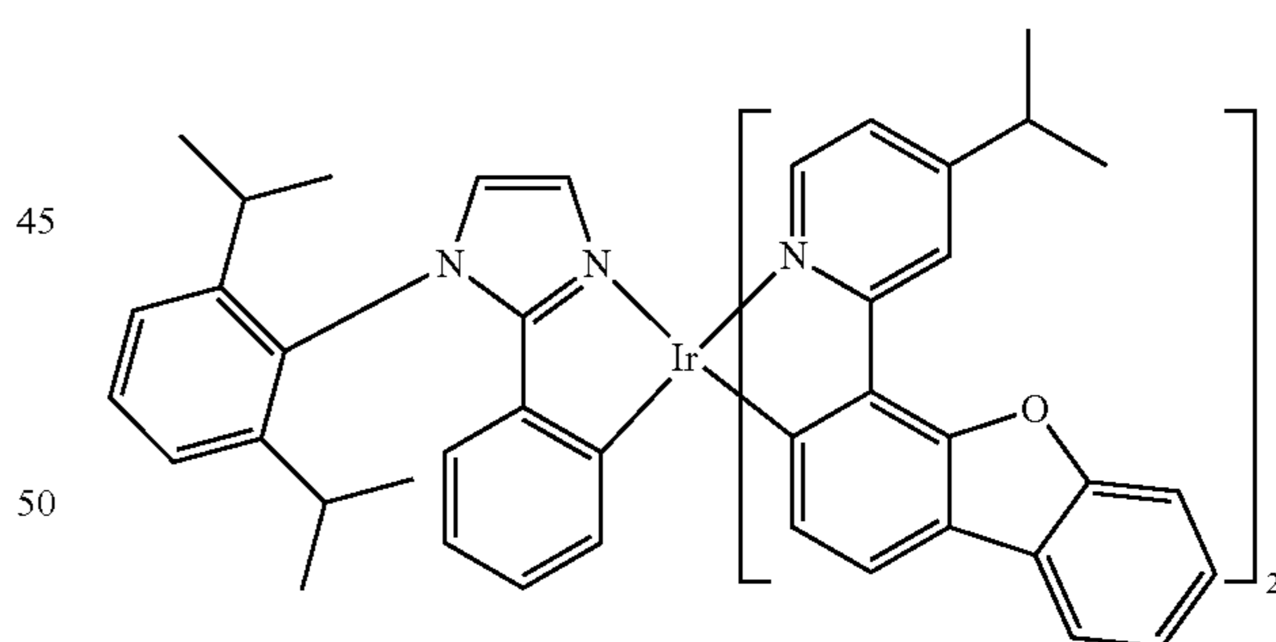
Compound 8
