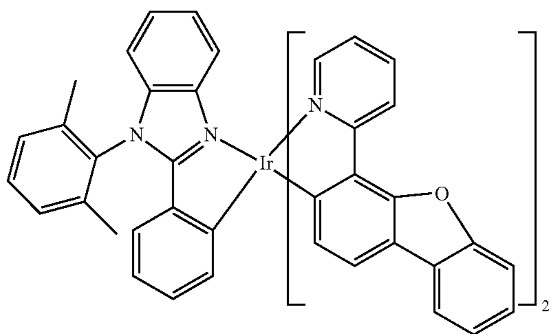
Compound 115
