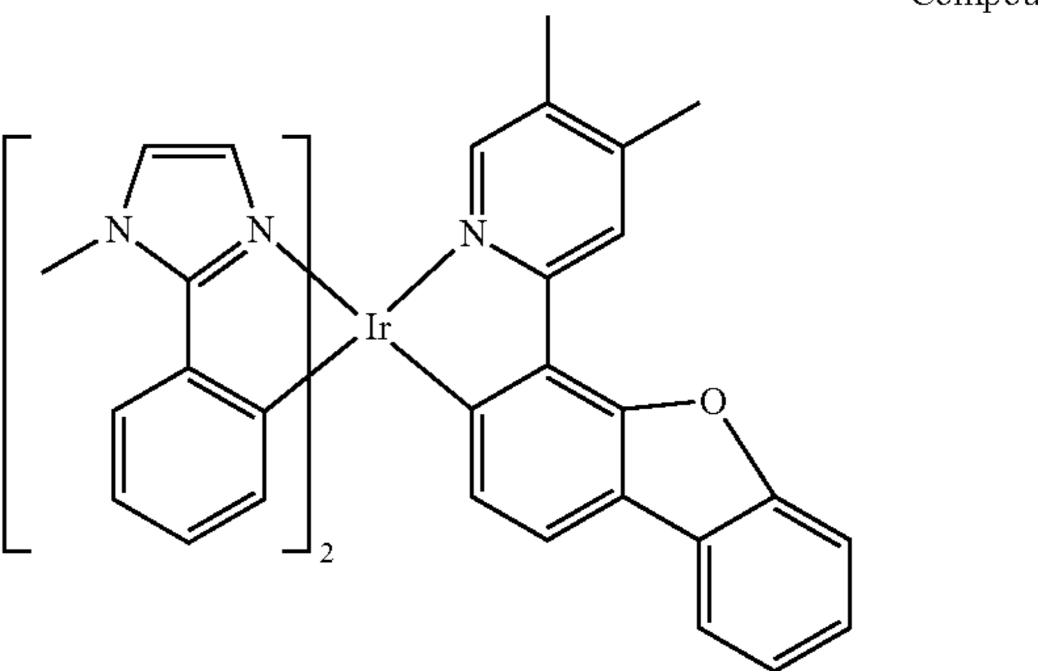
Compound 15
