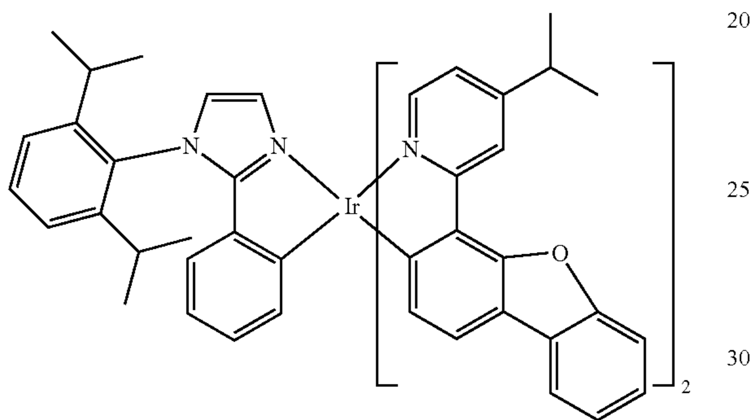
Compound 8
