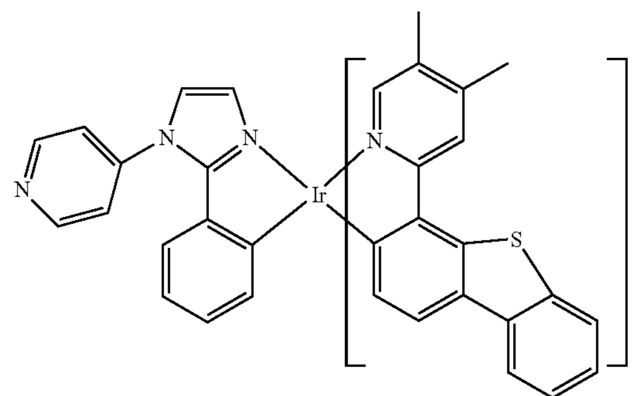
Compound 56
