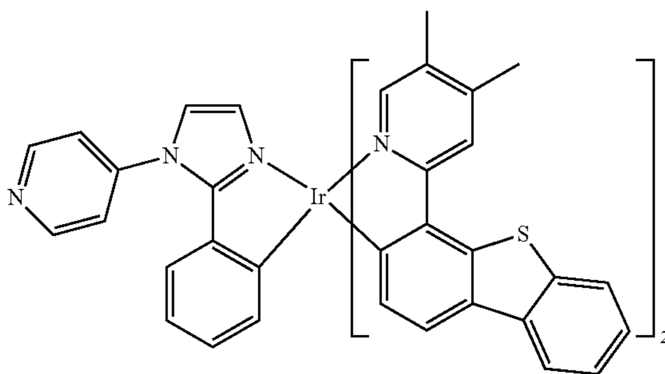
Compound 57
