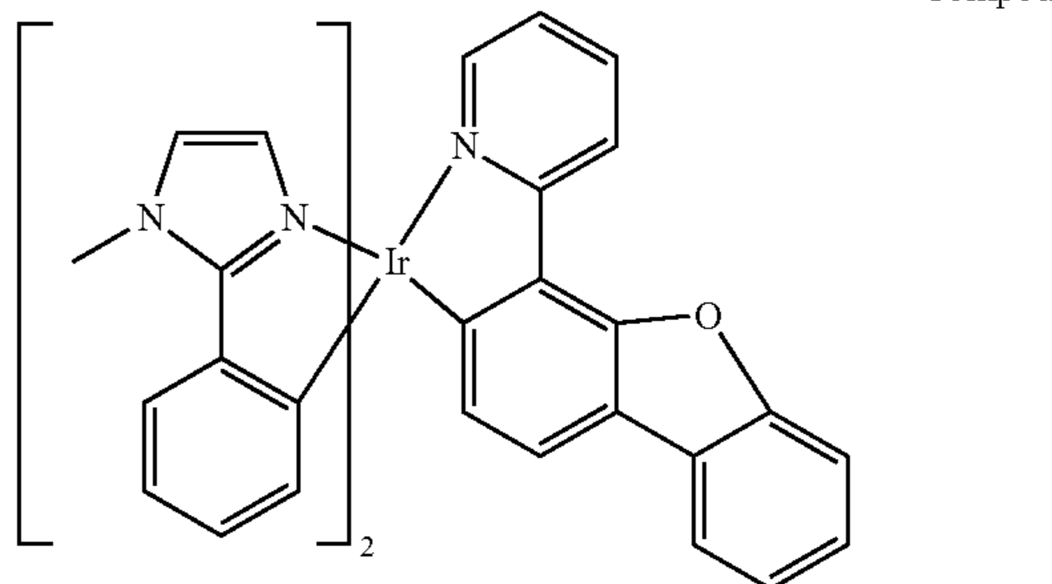
Compound 14
