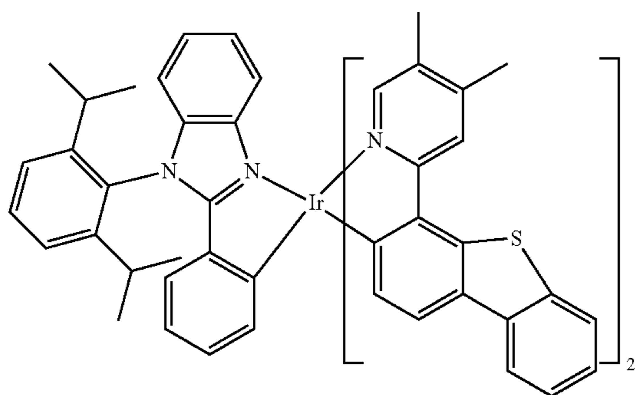
Compound 100
