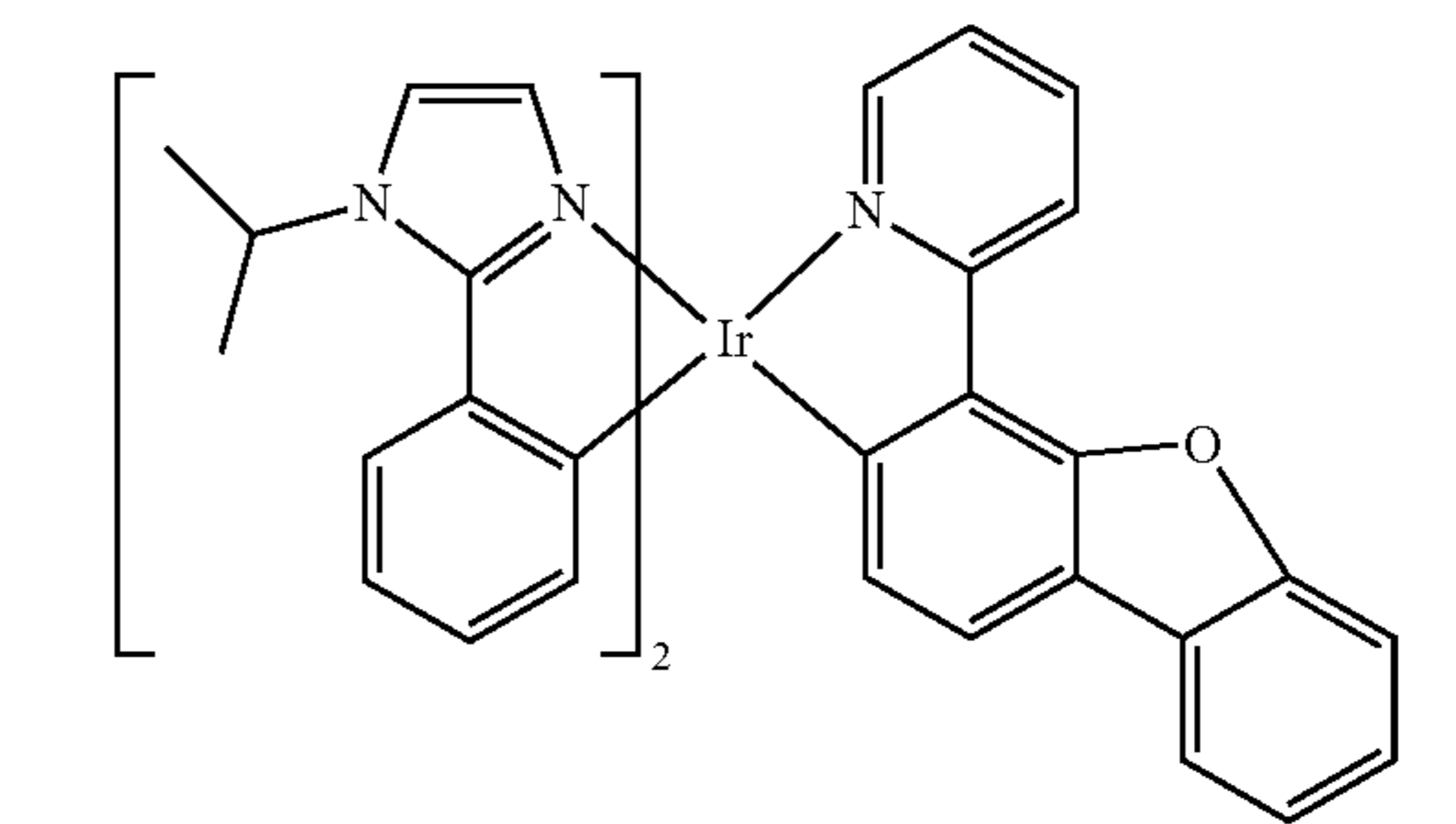
Compound 41
