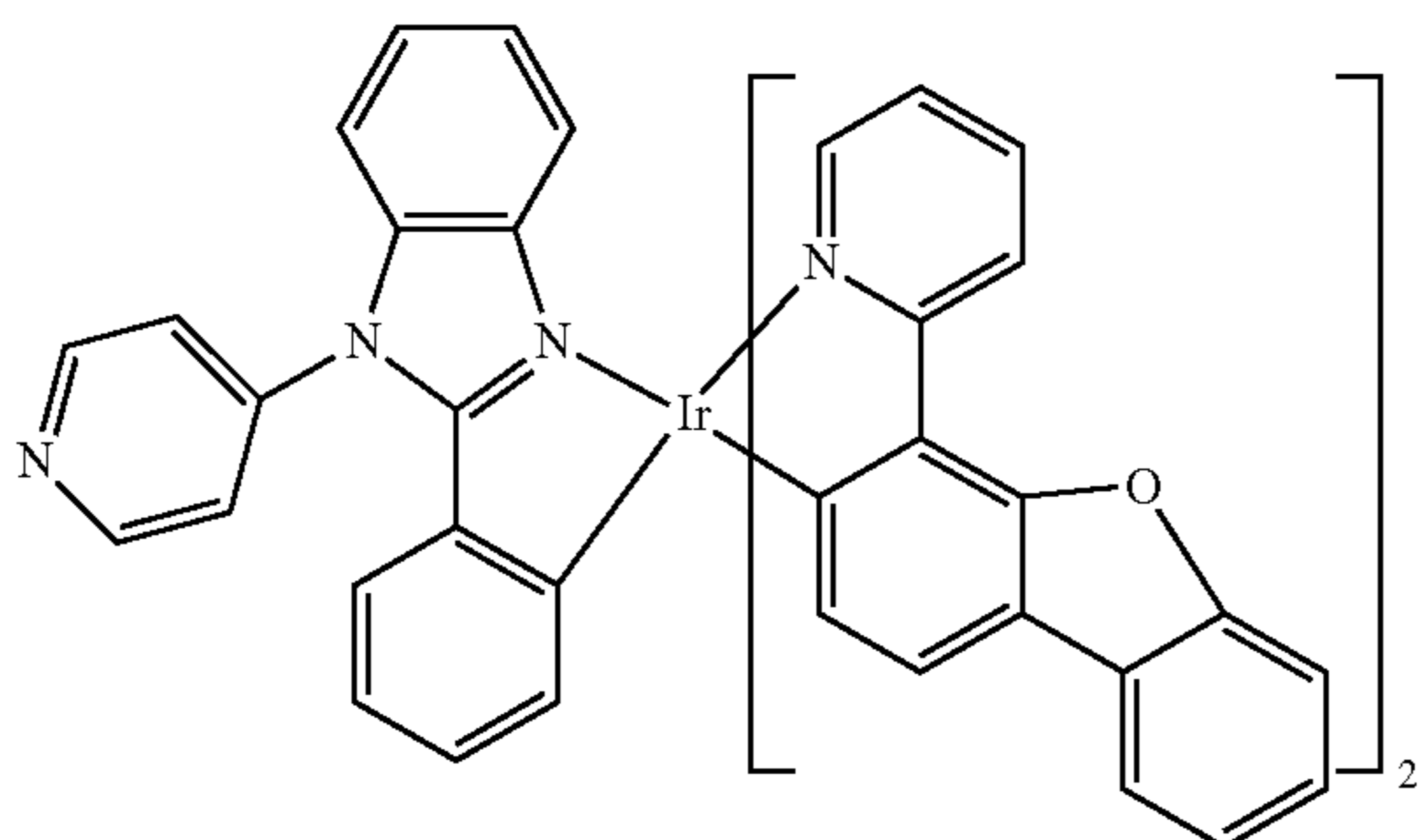
Compound 119
