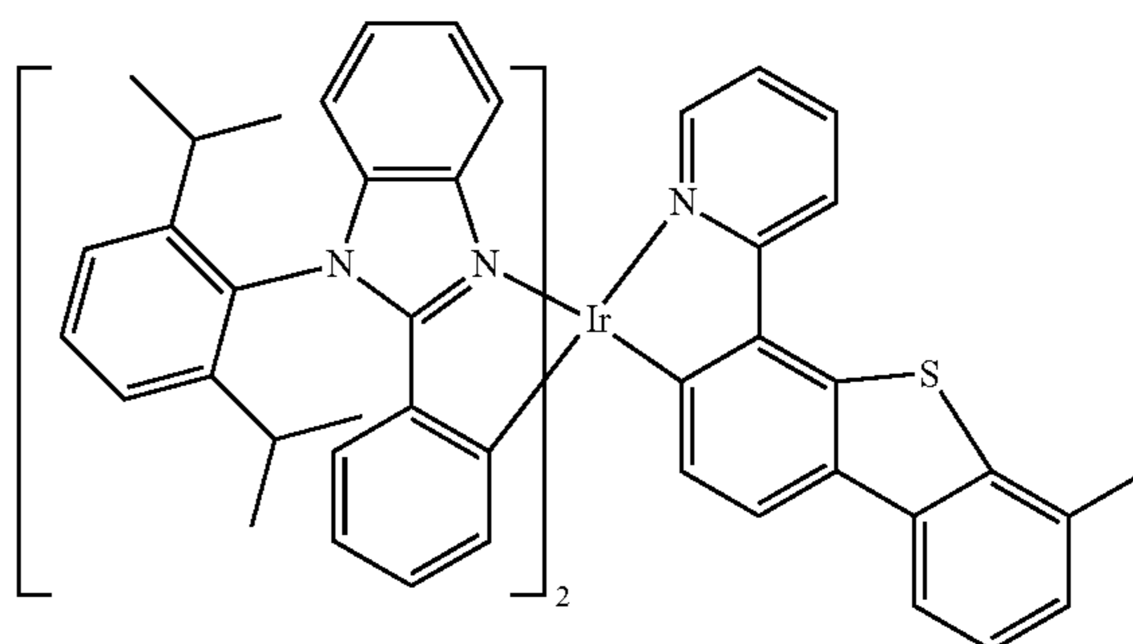
Compound 101
