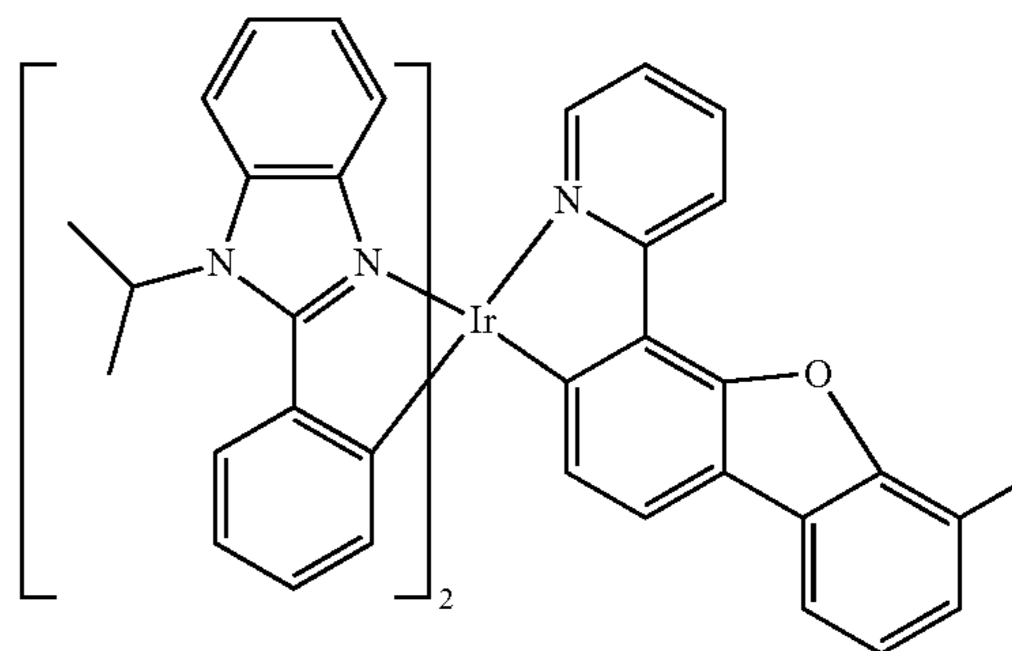
Compound 125
