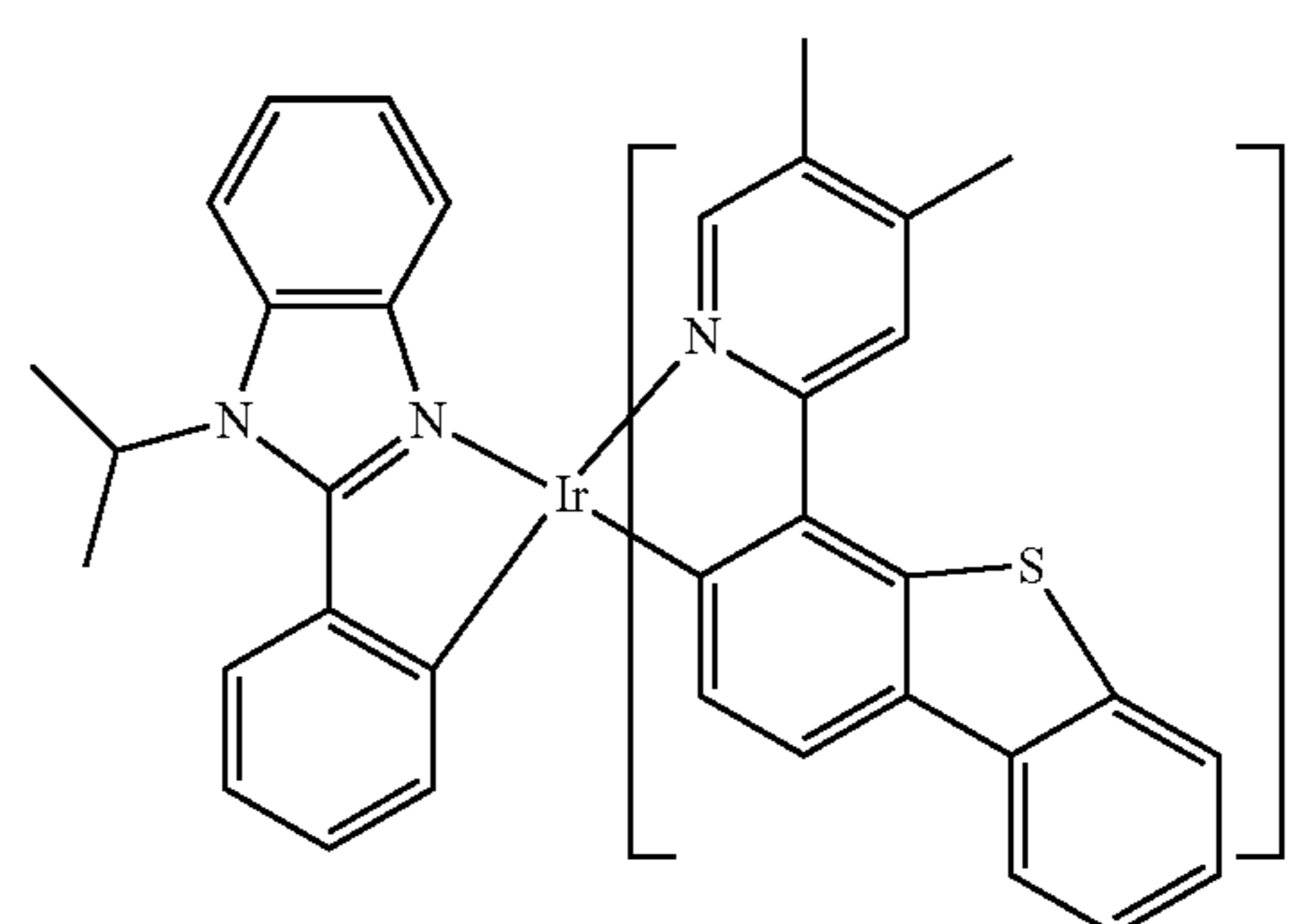
Compound 140
