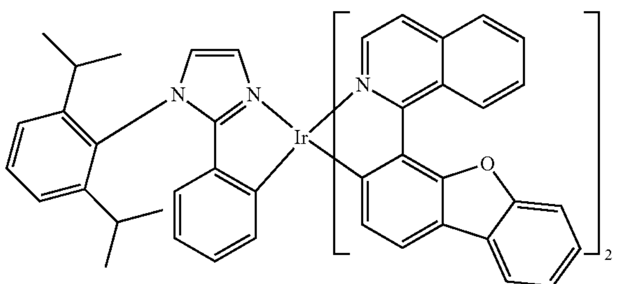
Compound 74
