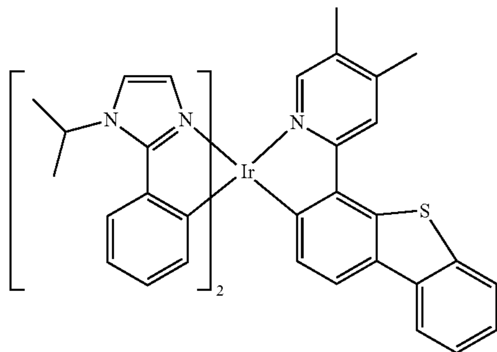
Compound 58
