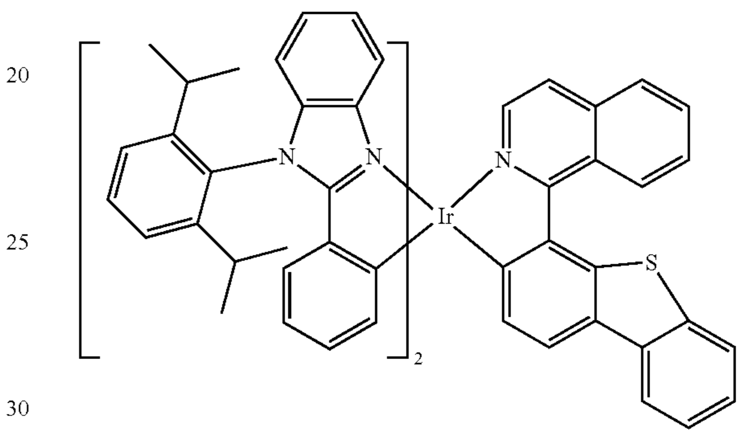
Compound 156
