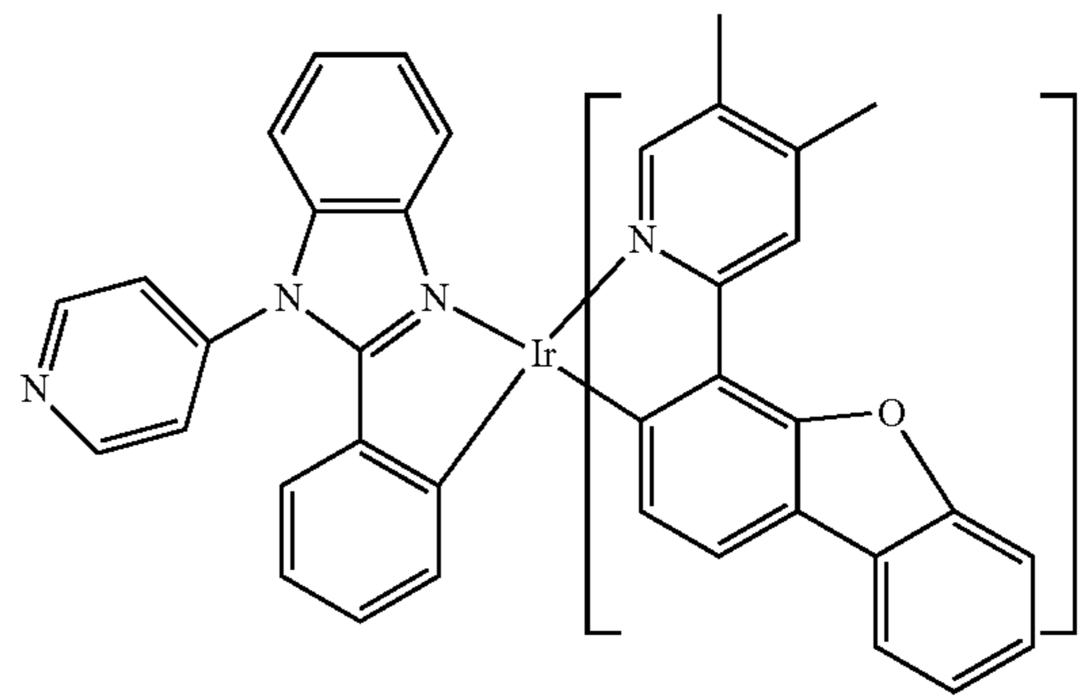
Compound 120
