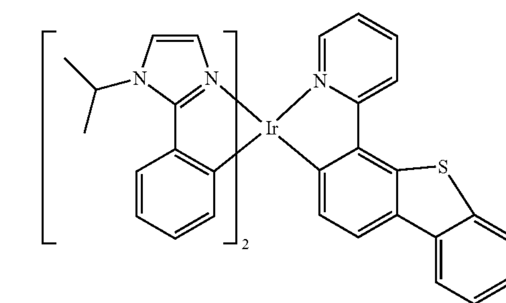
Compound 57
