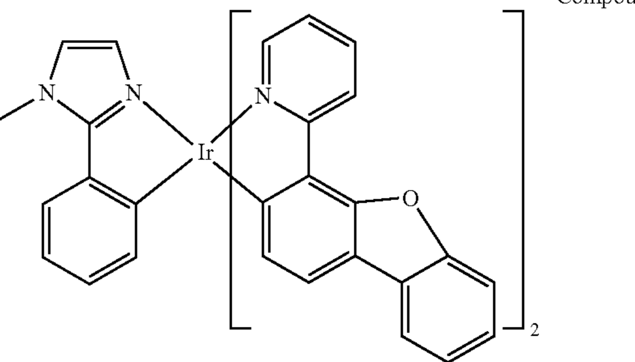
Compound 15
