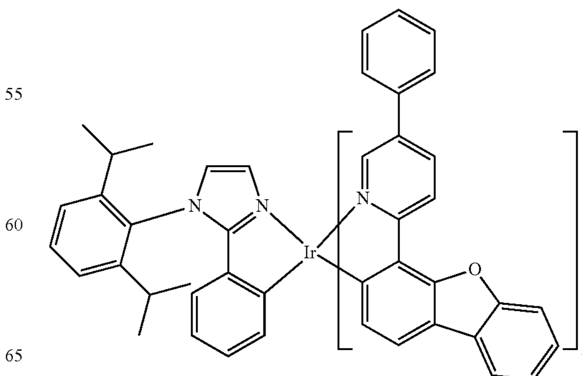
Compound 68
