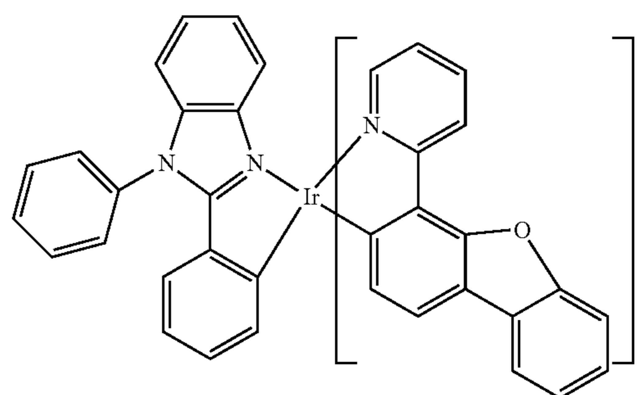
Compound 91
