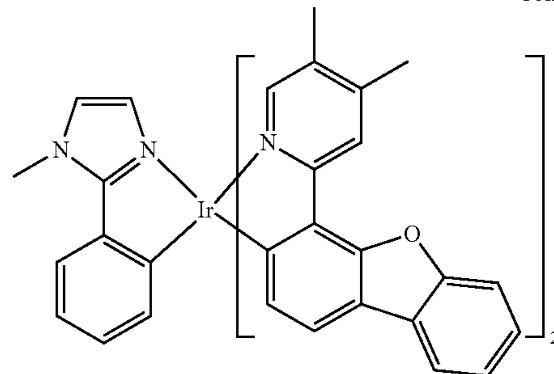
Compound 16
