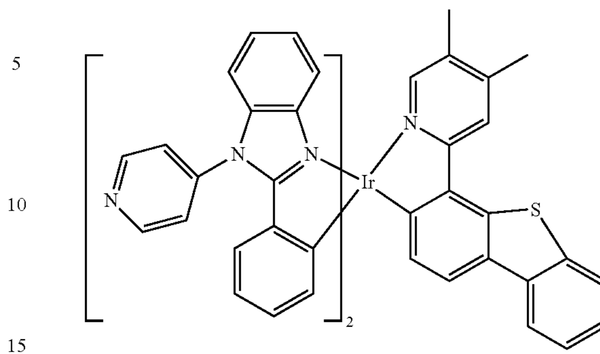
Compound 134
