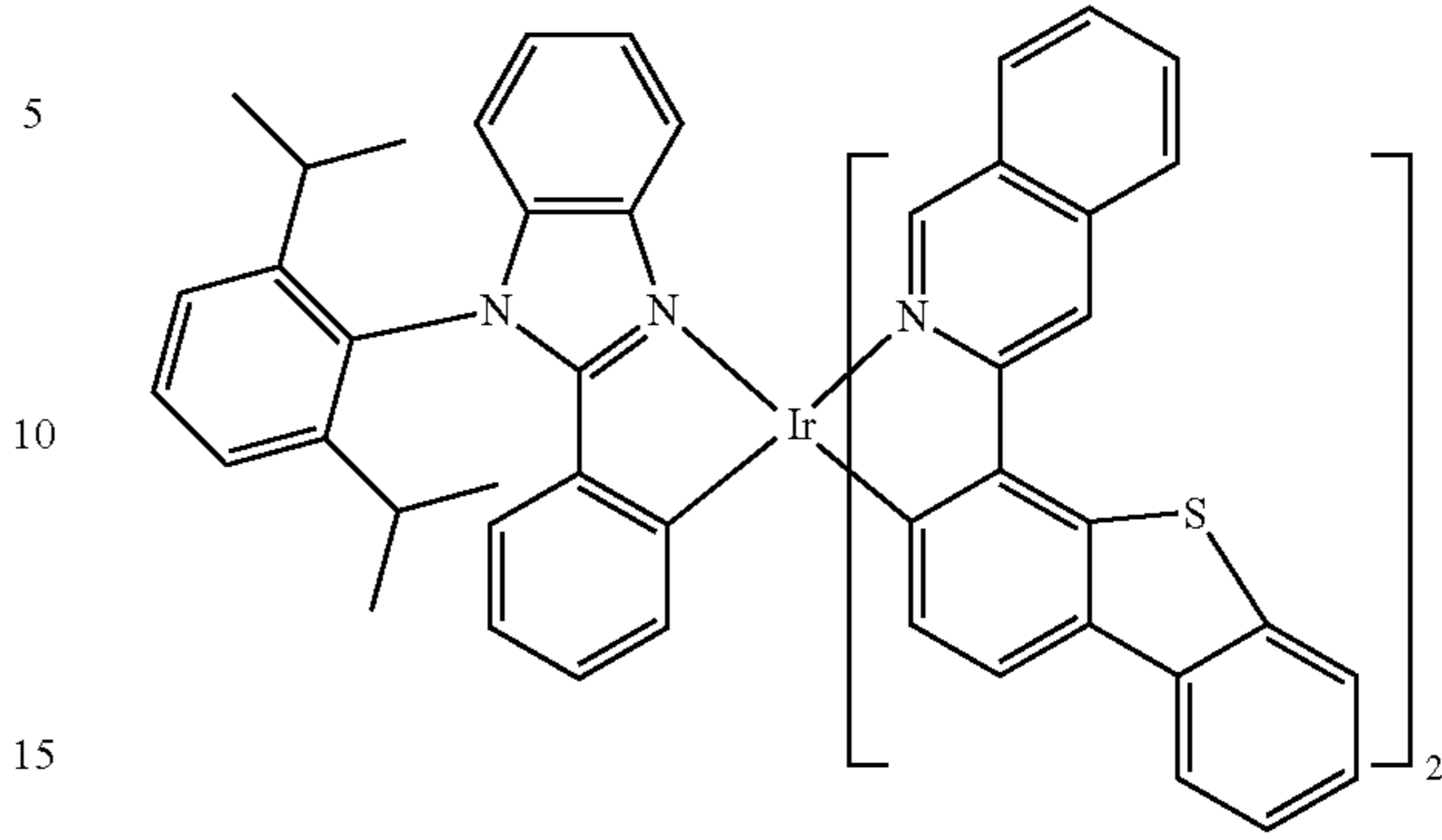
Compound 155
