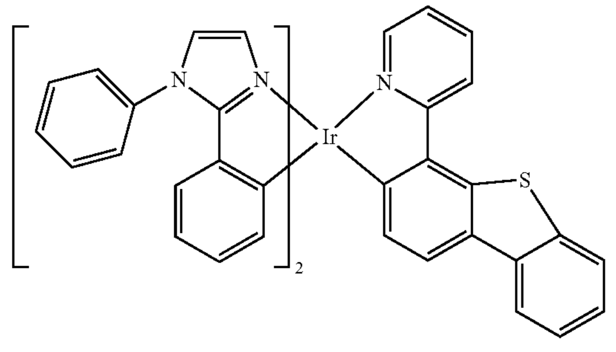
Compound 25
