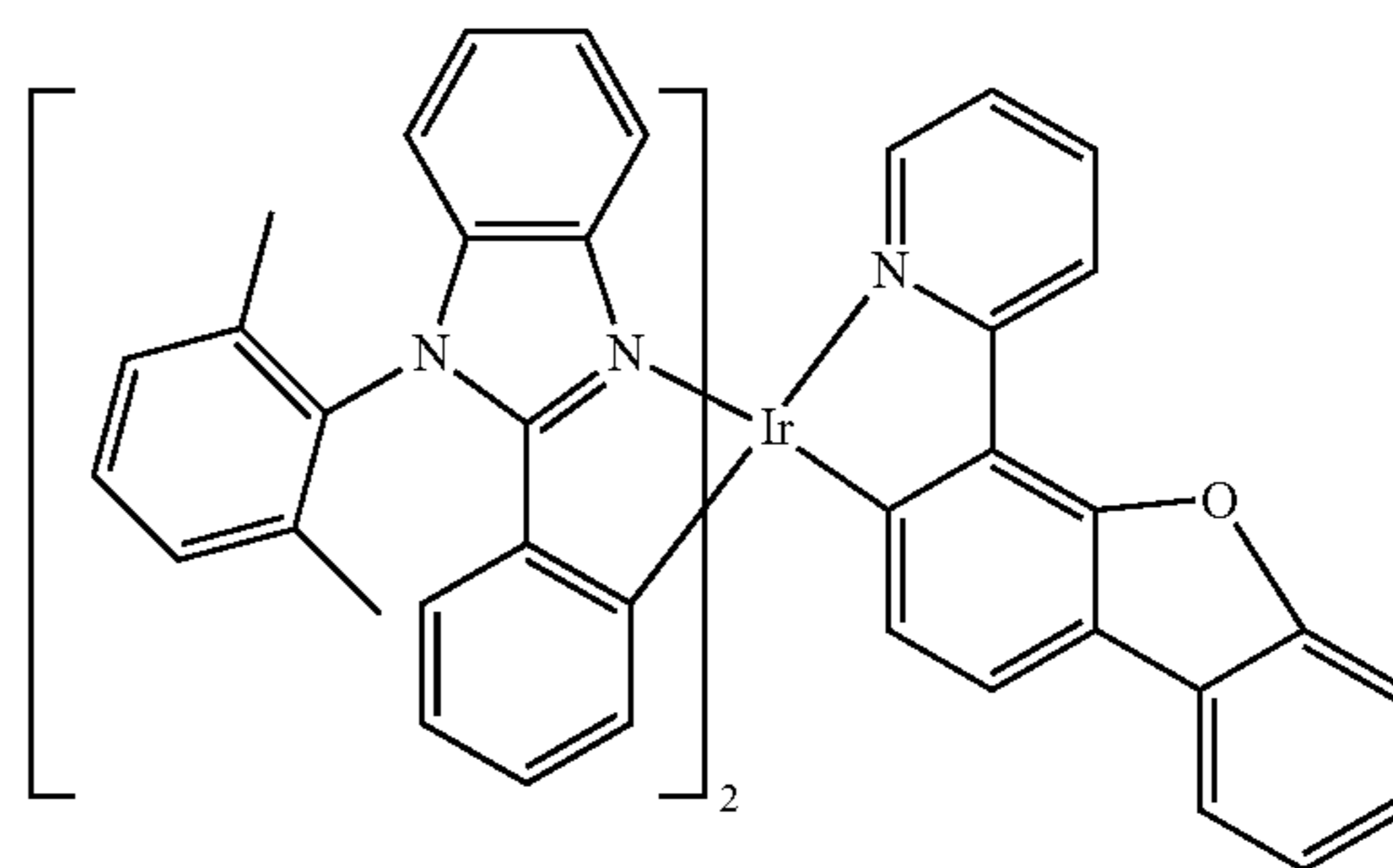
Compound 113
