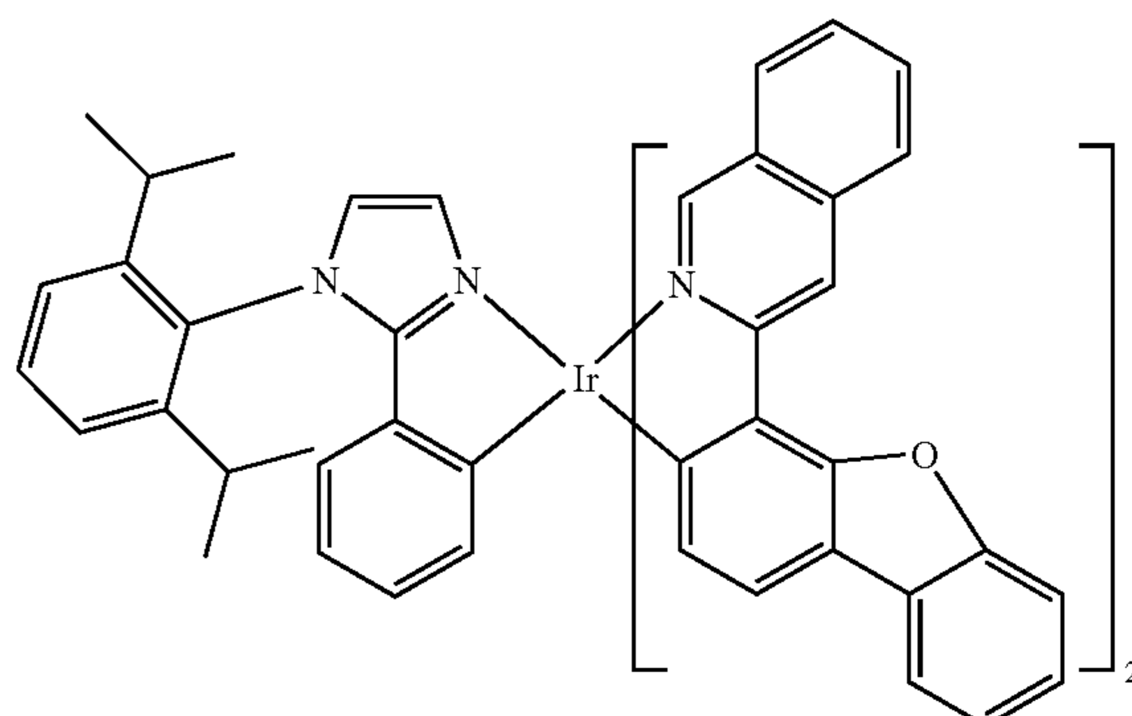
Compound 71
