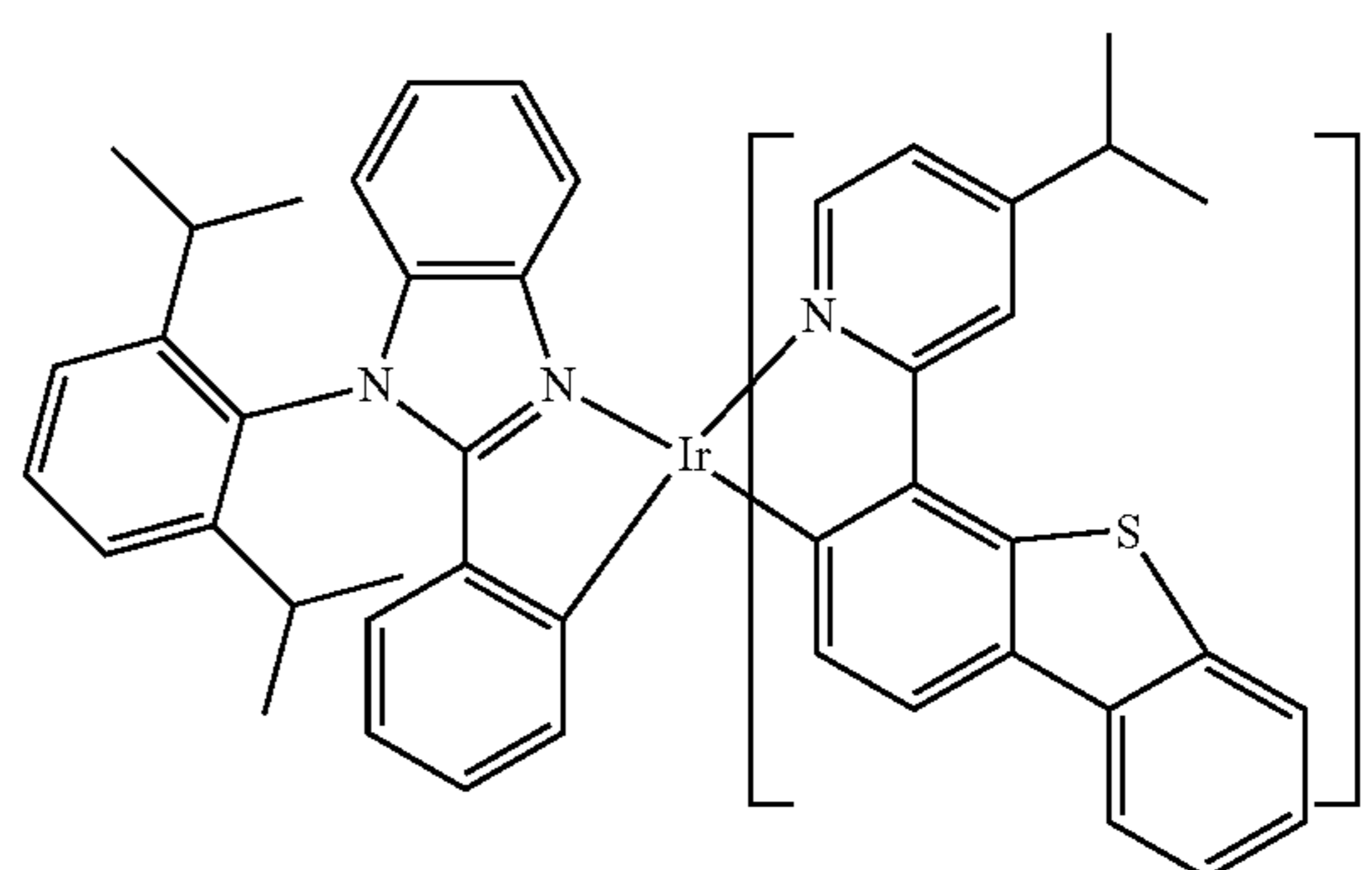
Compound 104
