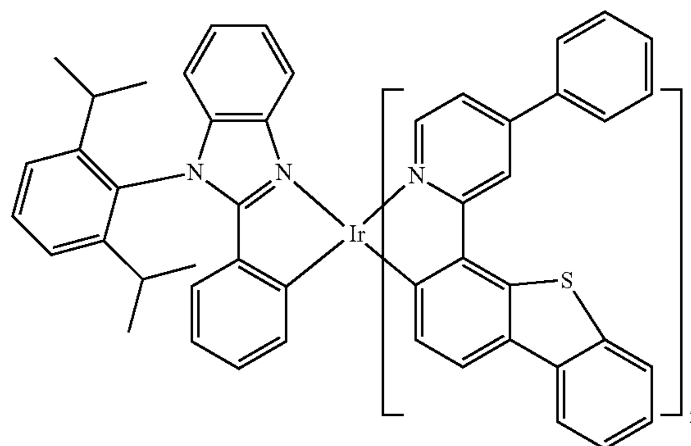
Compound 151
