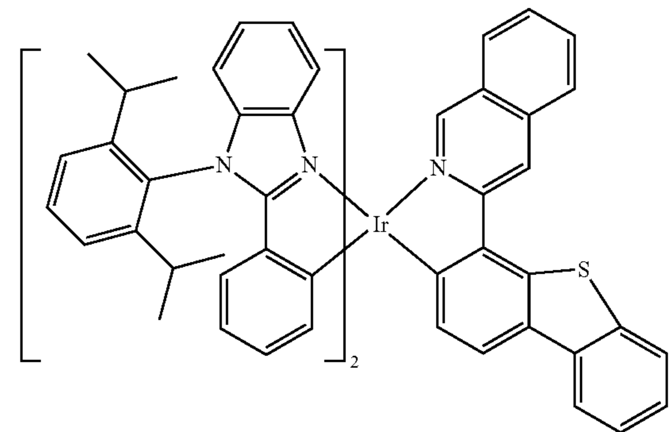
Compound 153
