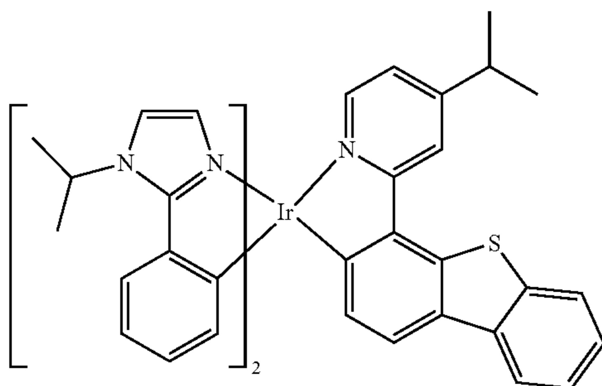
Compound 63
