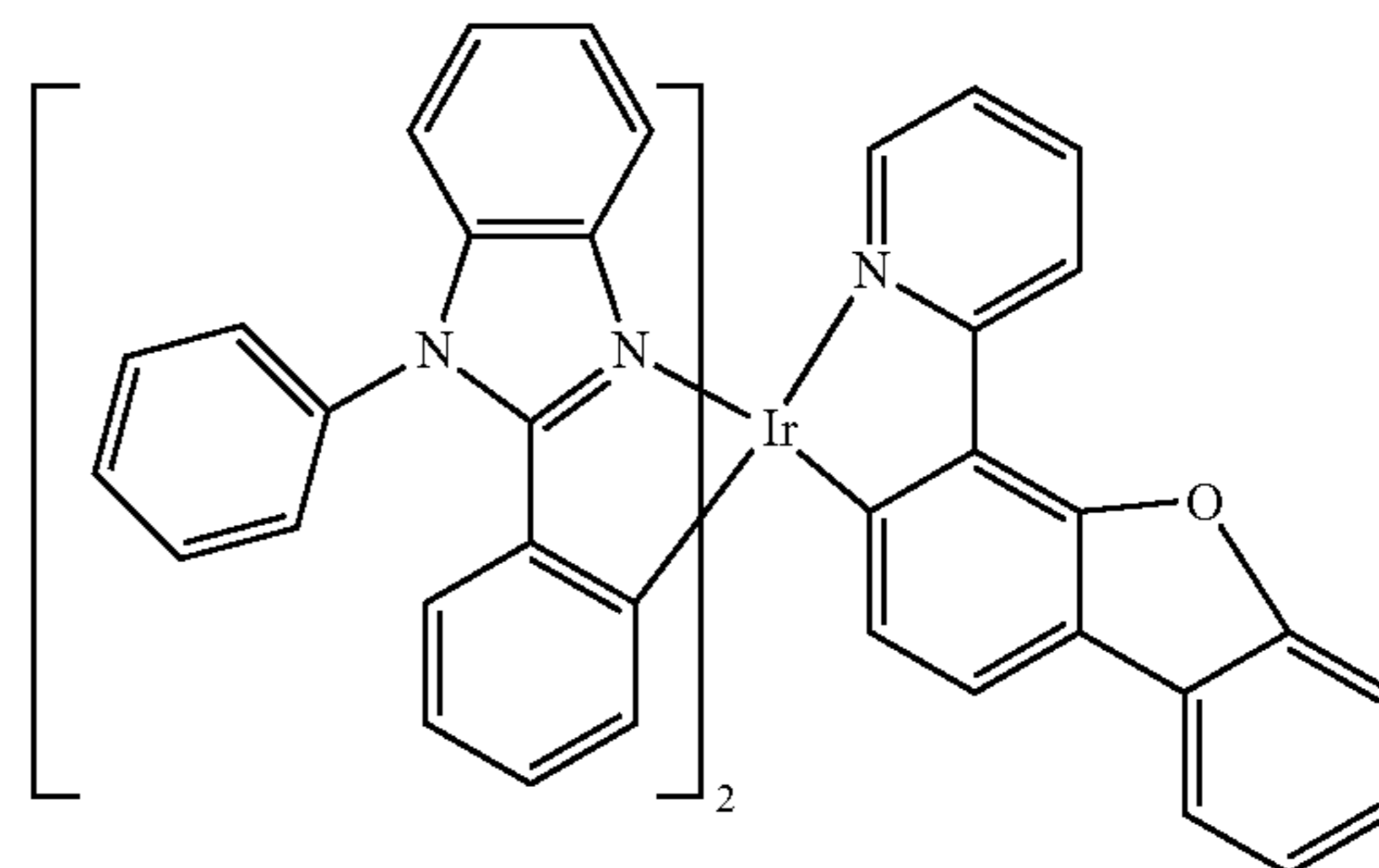
Compound 89
