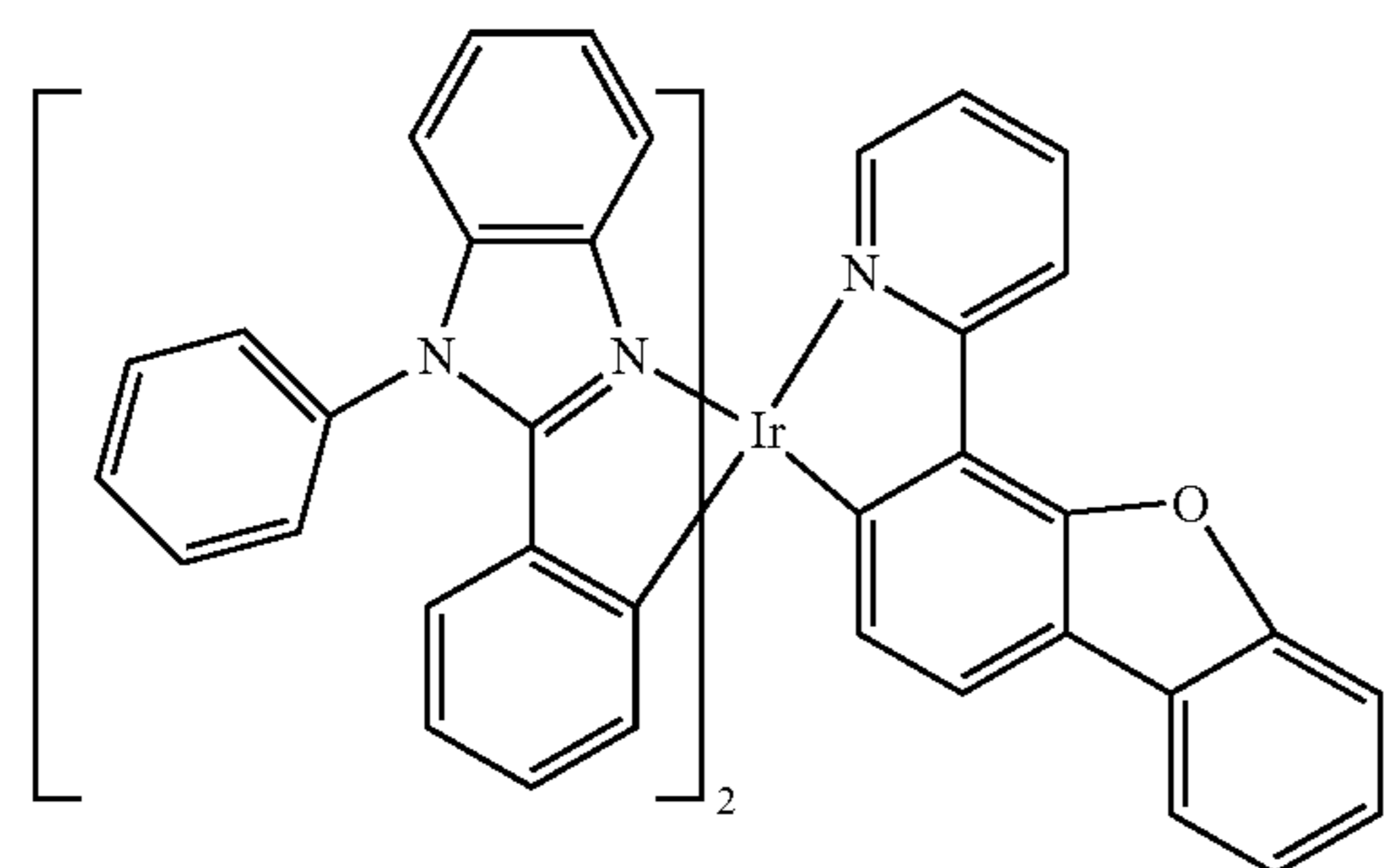
Compound 89
