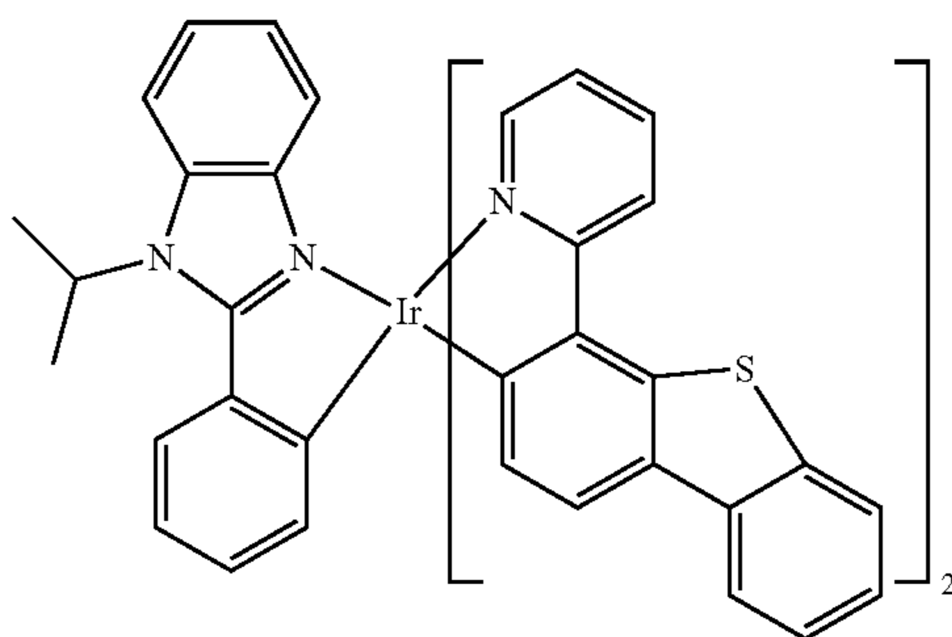
Compound 139
