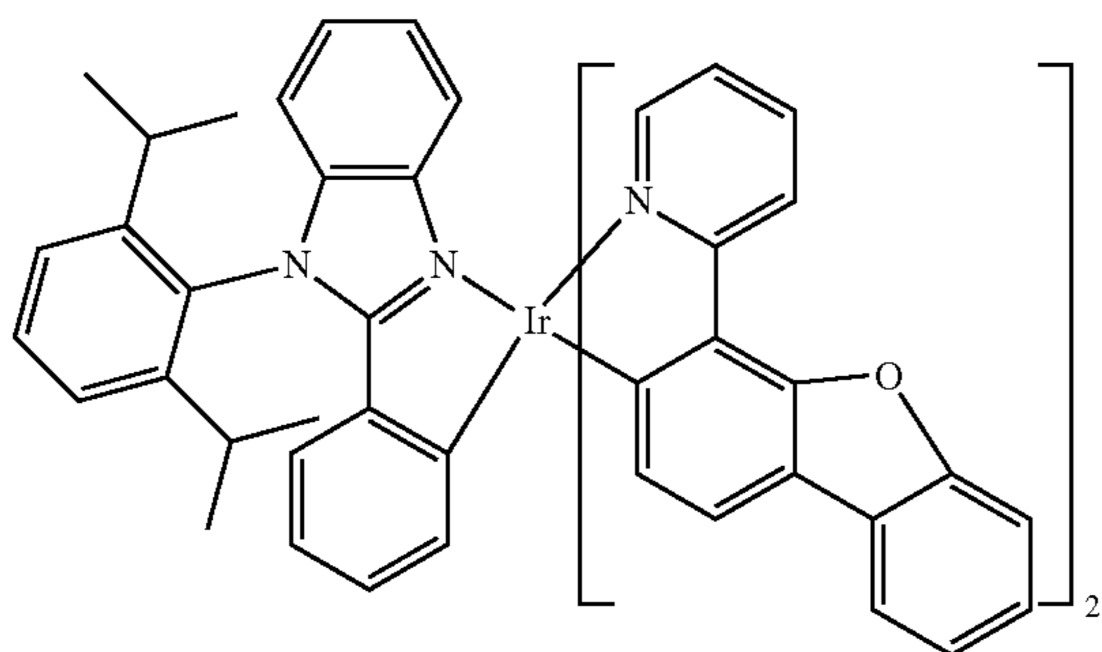
Compound 83
