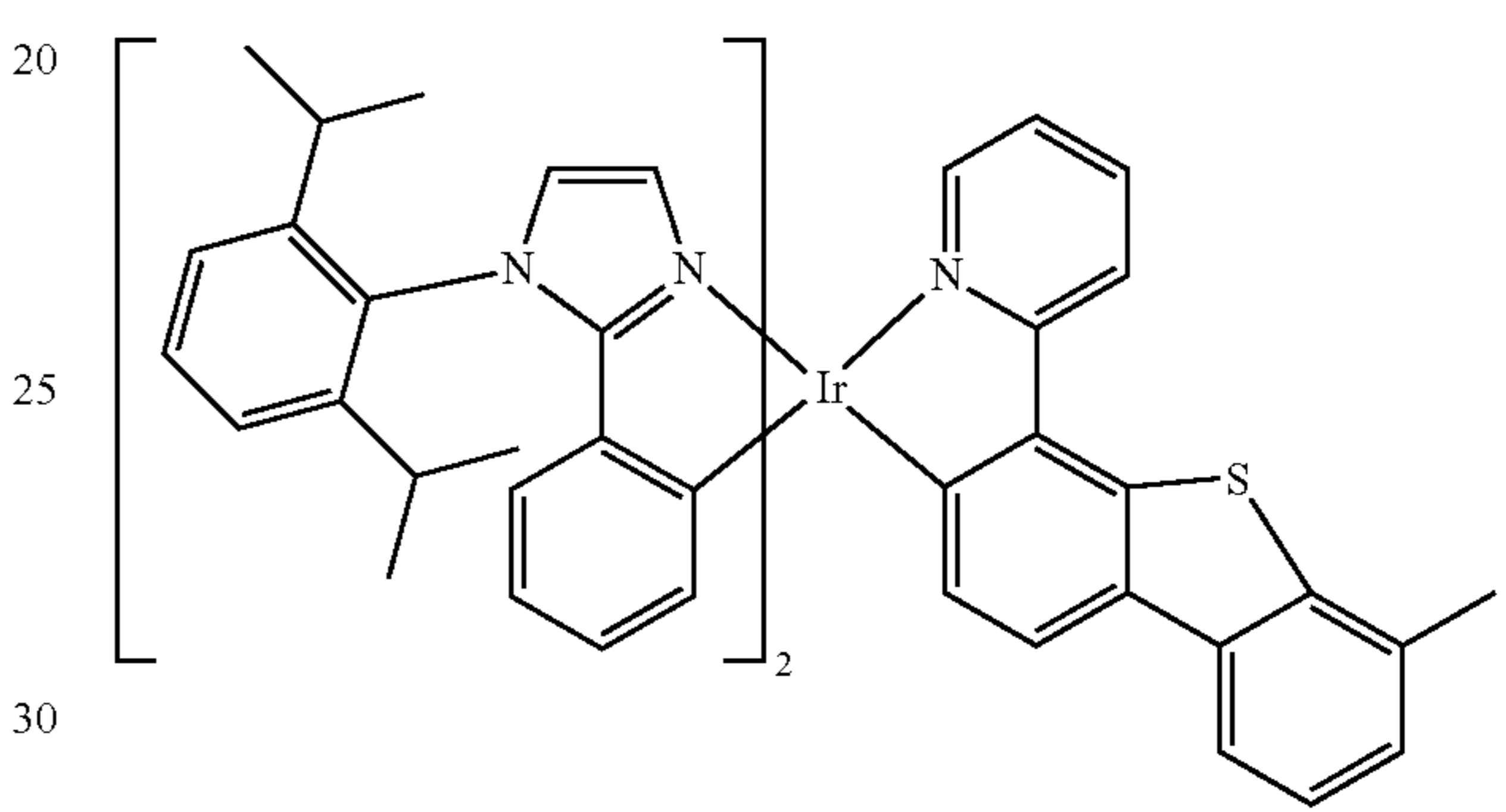
Compound 21
