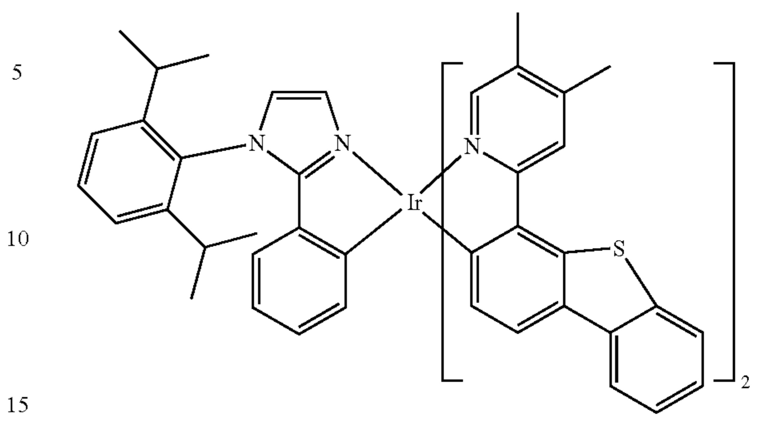
Compound 20
