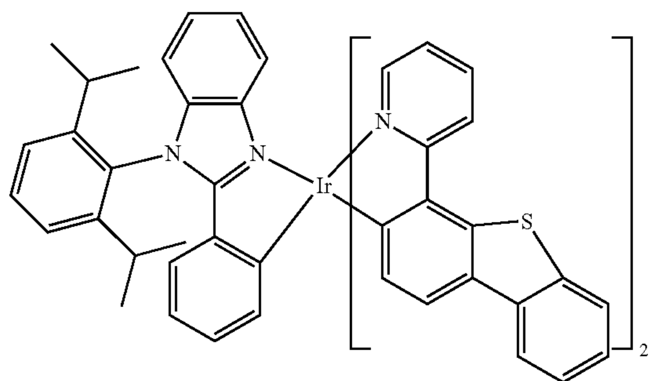
Compound 99
