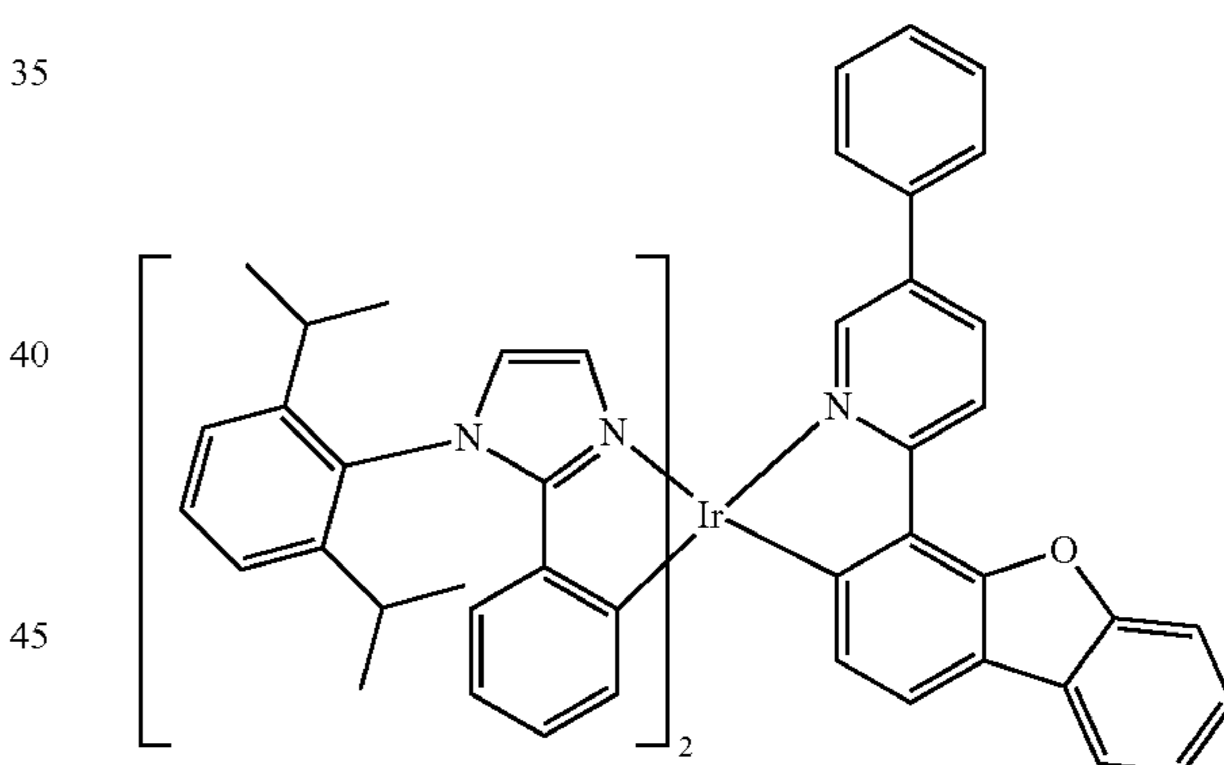
Compound 67
