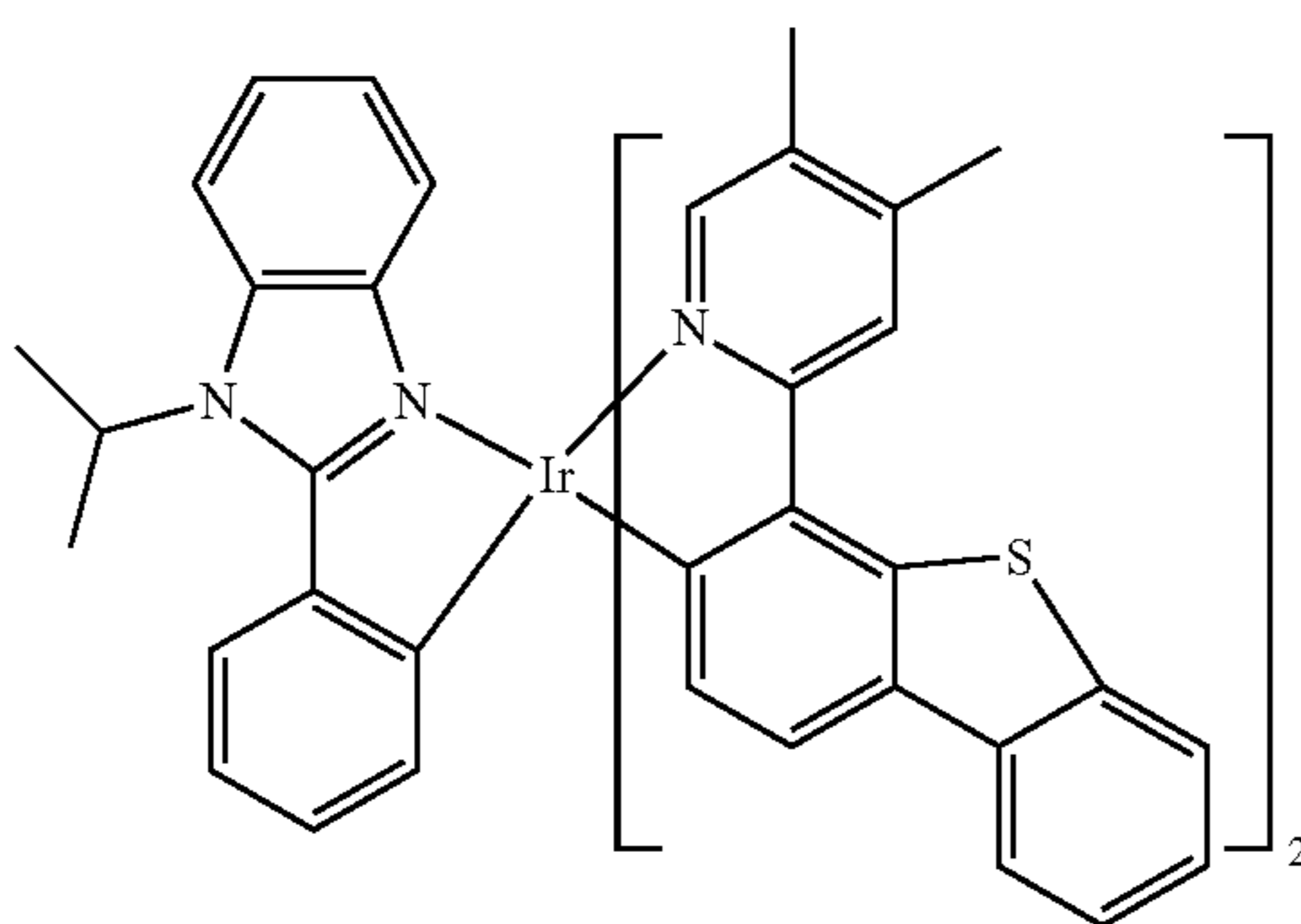
Compound 140
