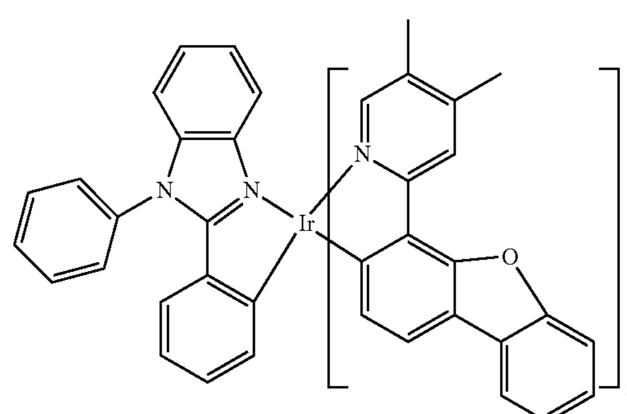
Compound 92
