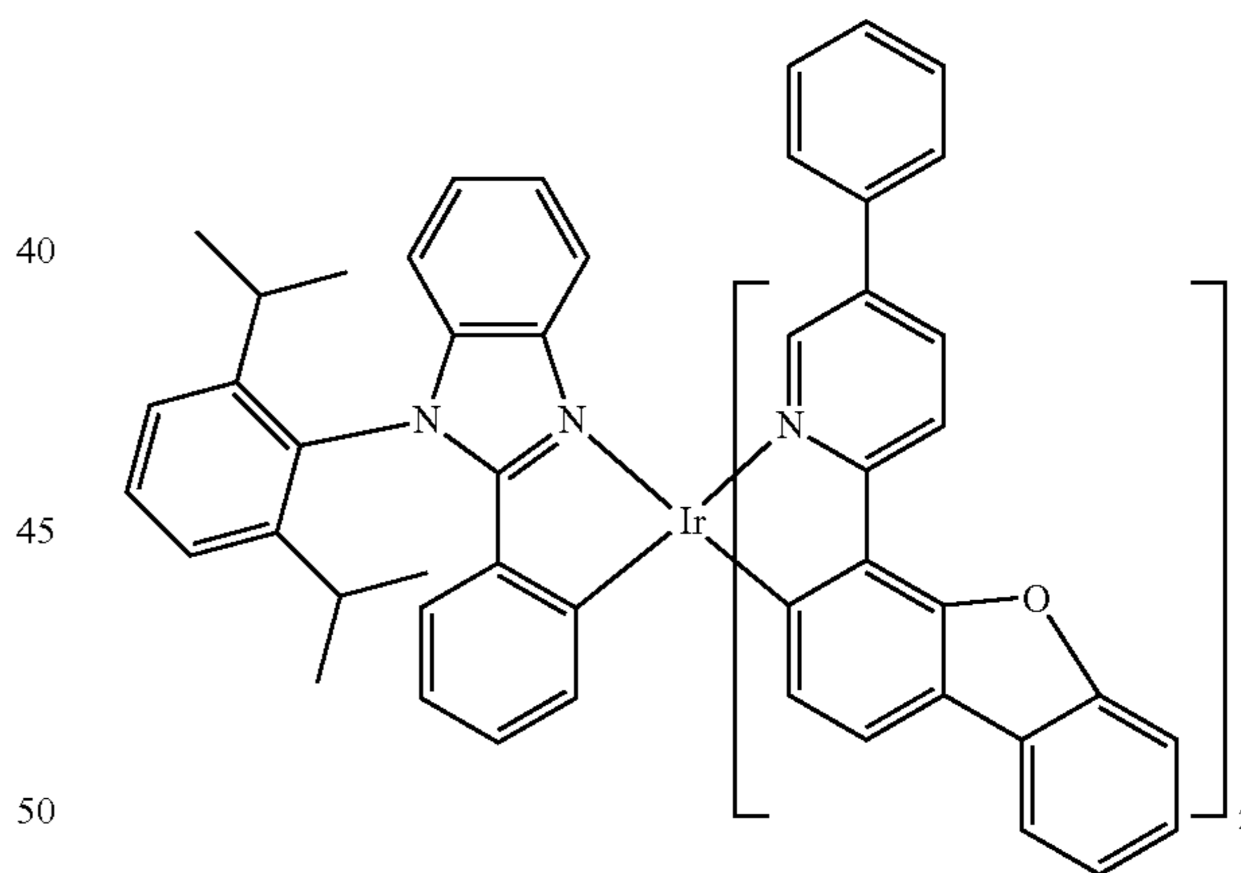
Compound 149
