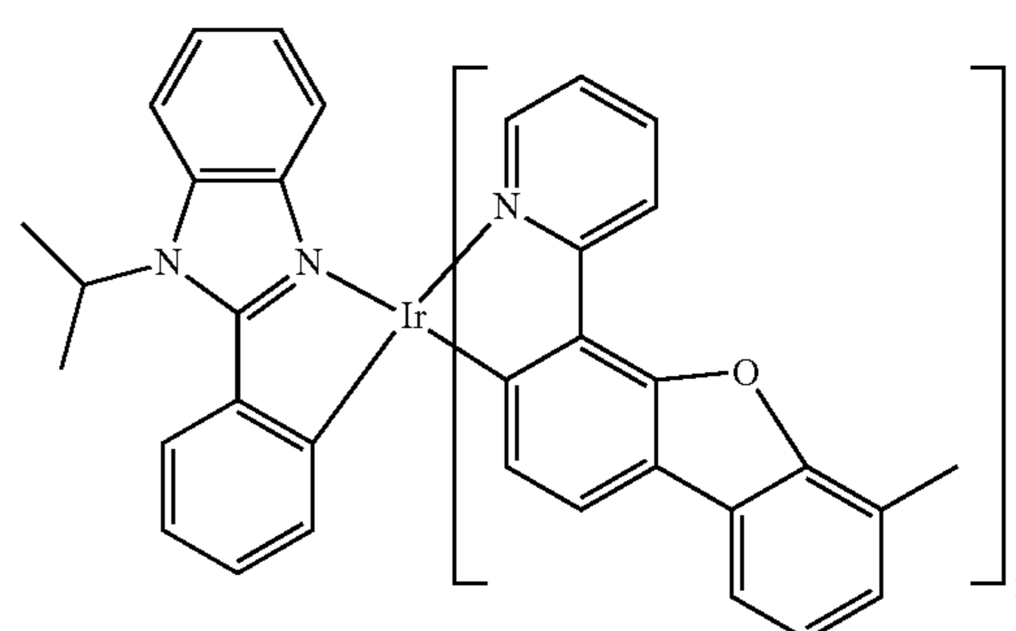
Compound 127
