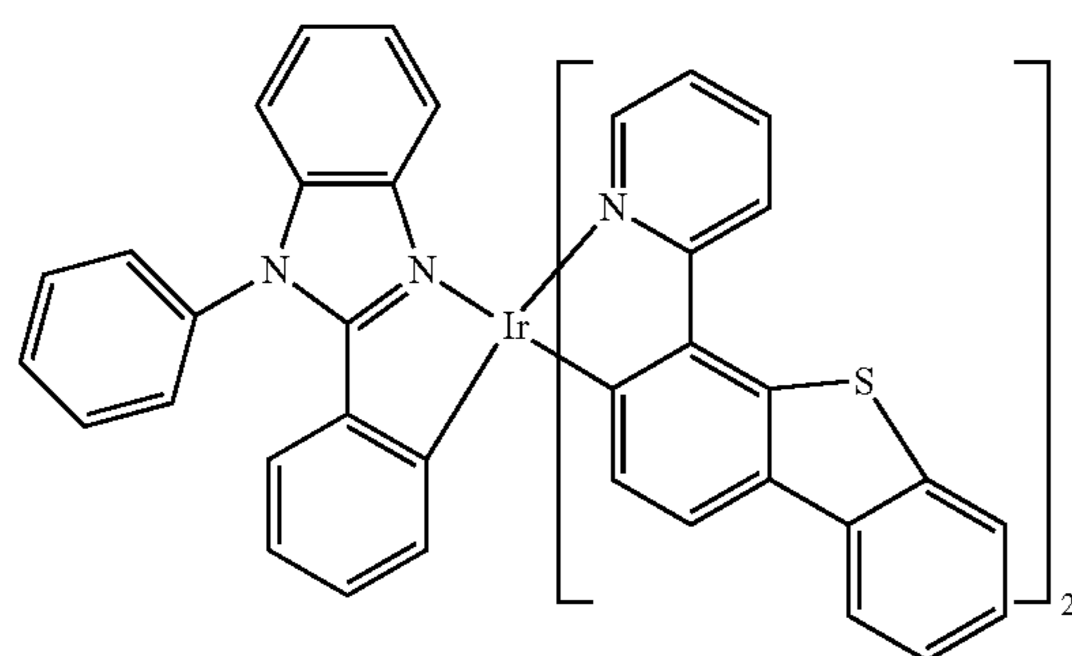
Compound 107
