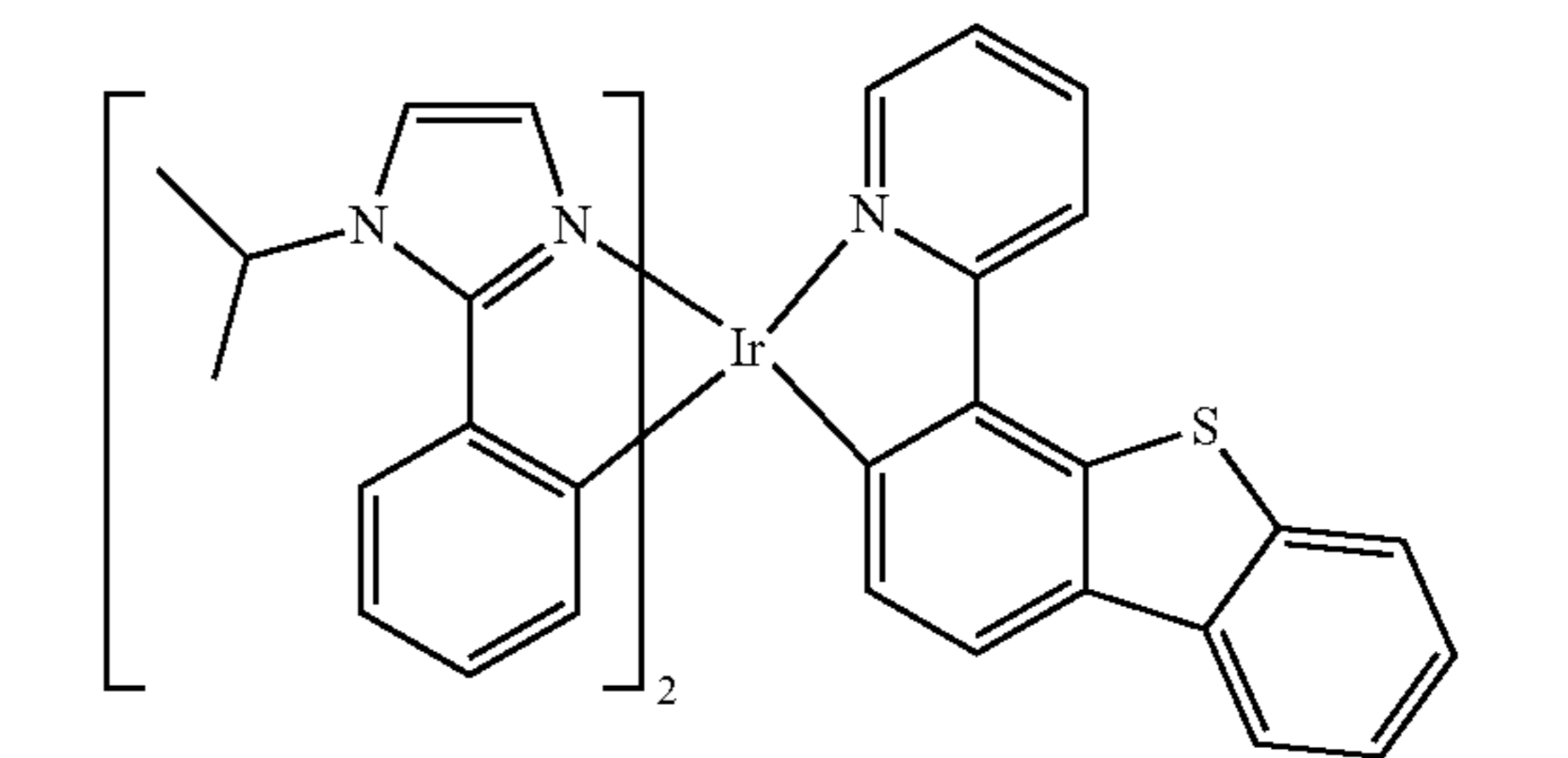
Compound 57
