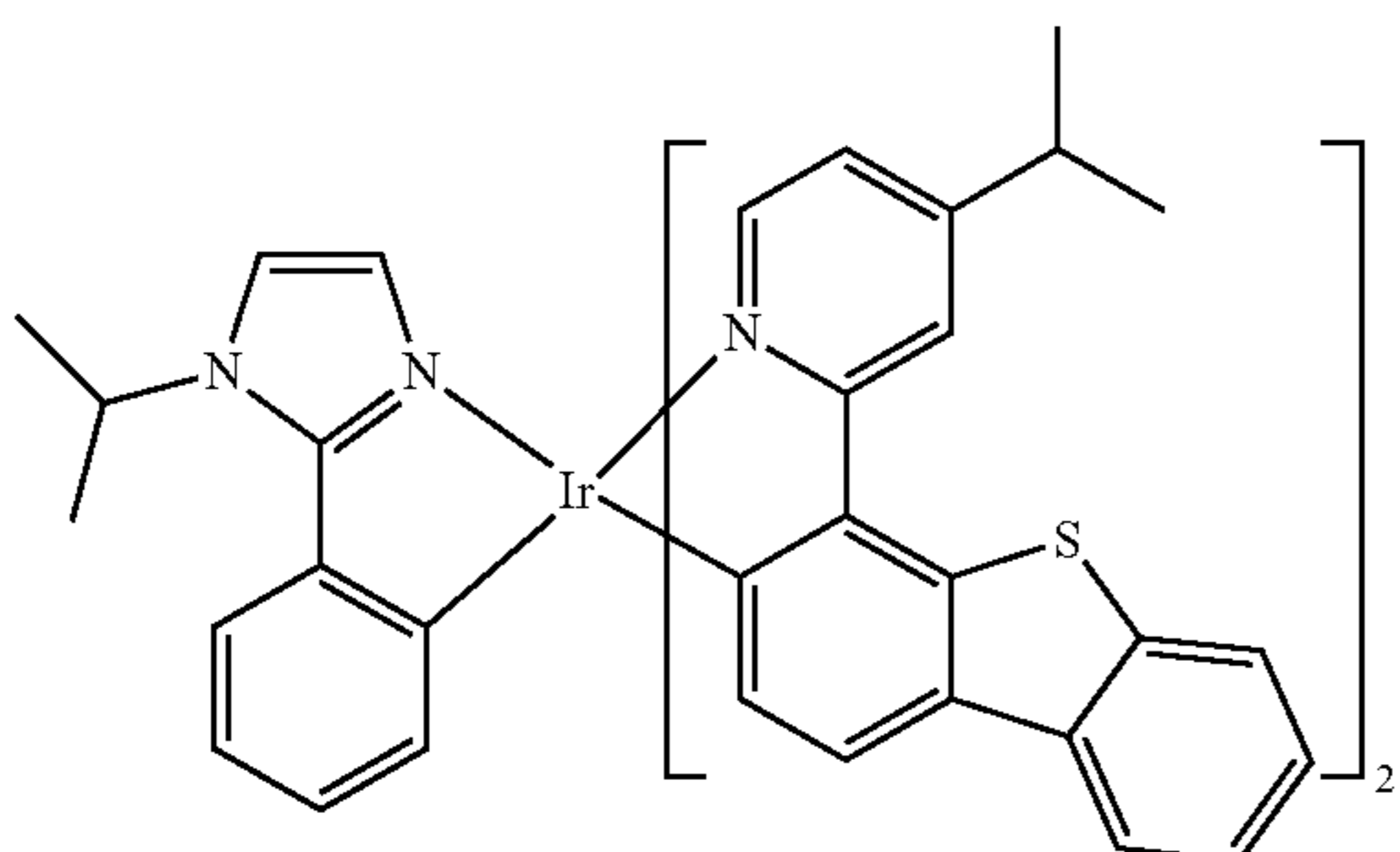
Compound 64
