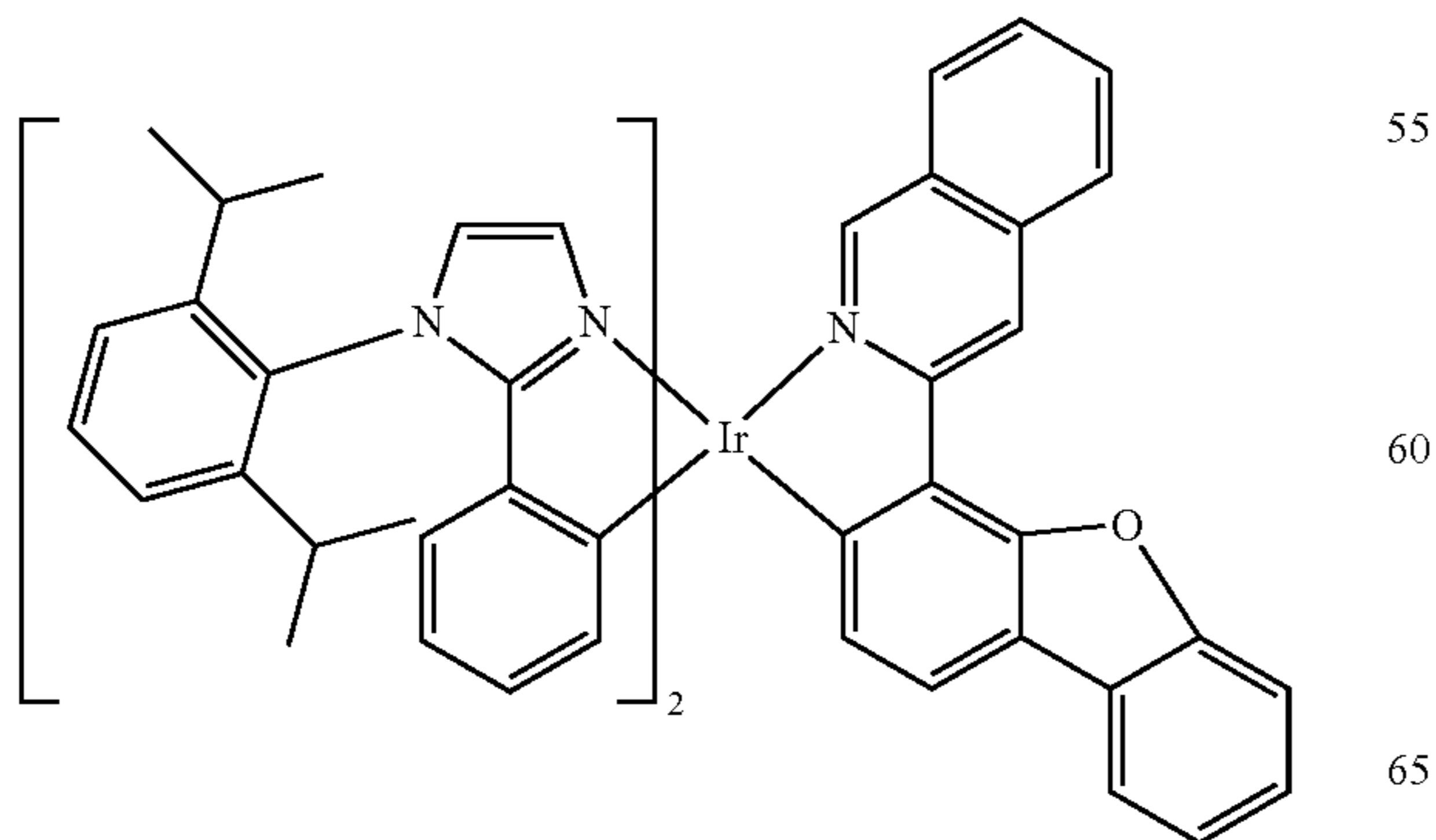
Compound 69
