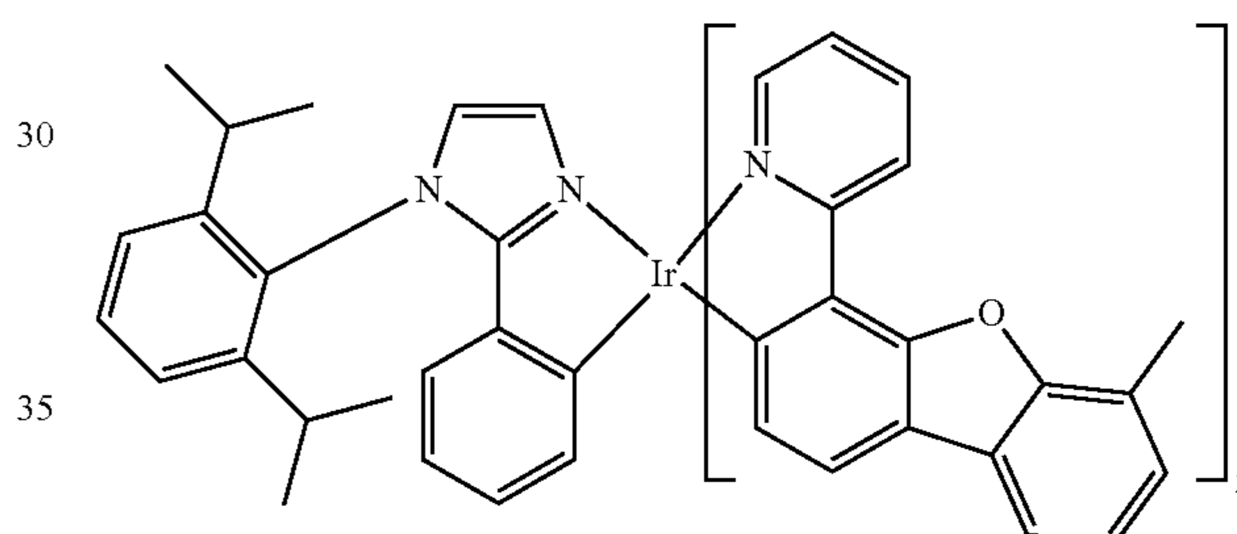
Compound 7
