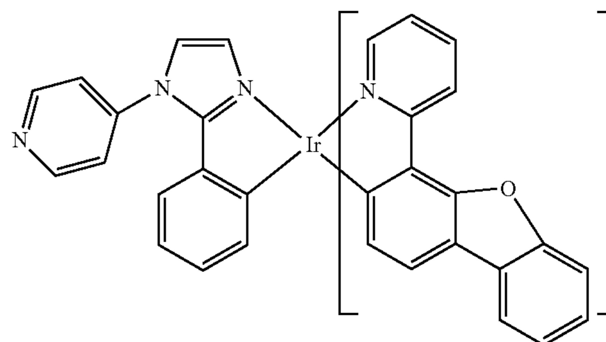
Compound 40
