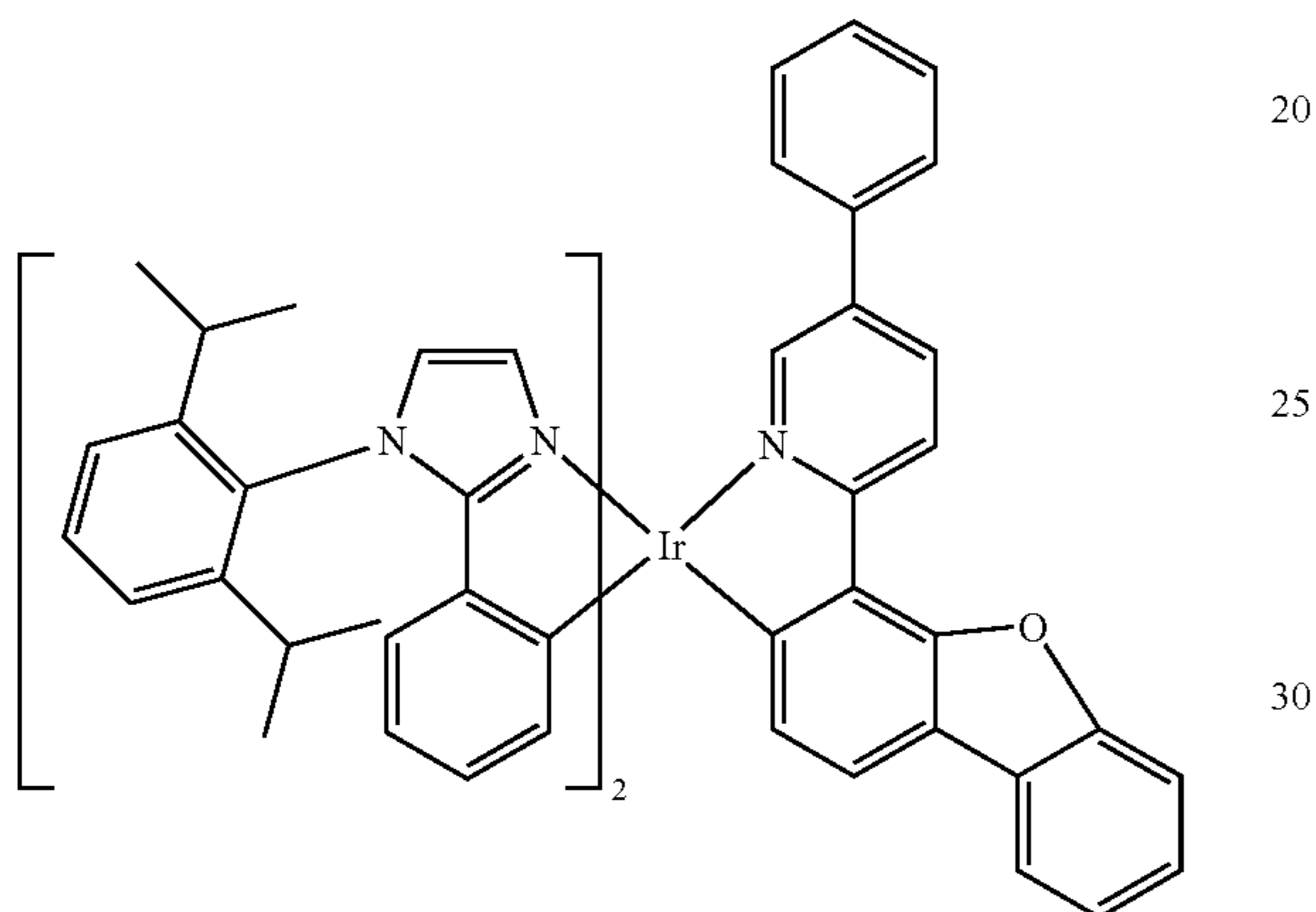
Compound 68
