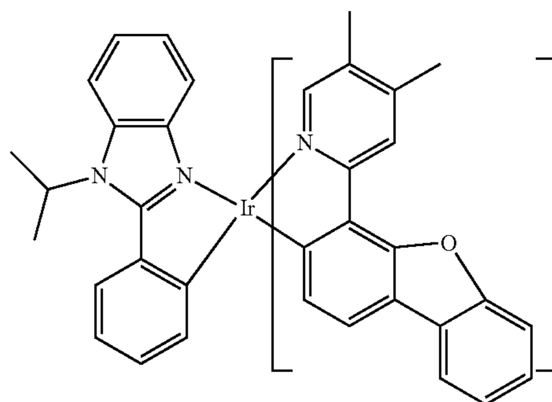
Compound 124
