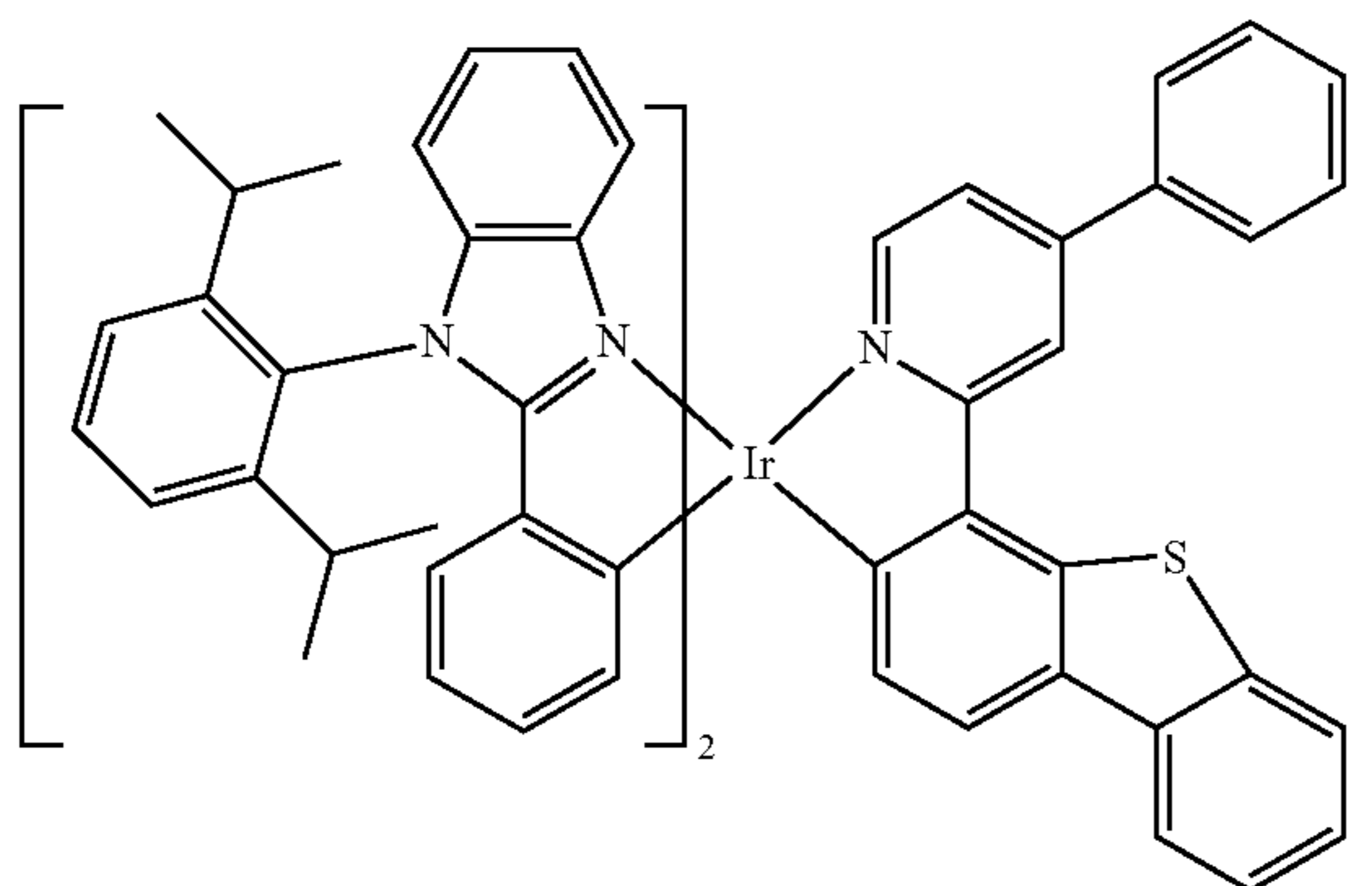
Compound 149
