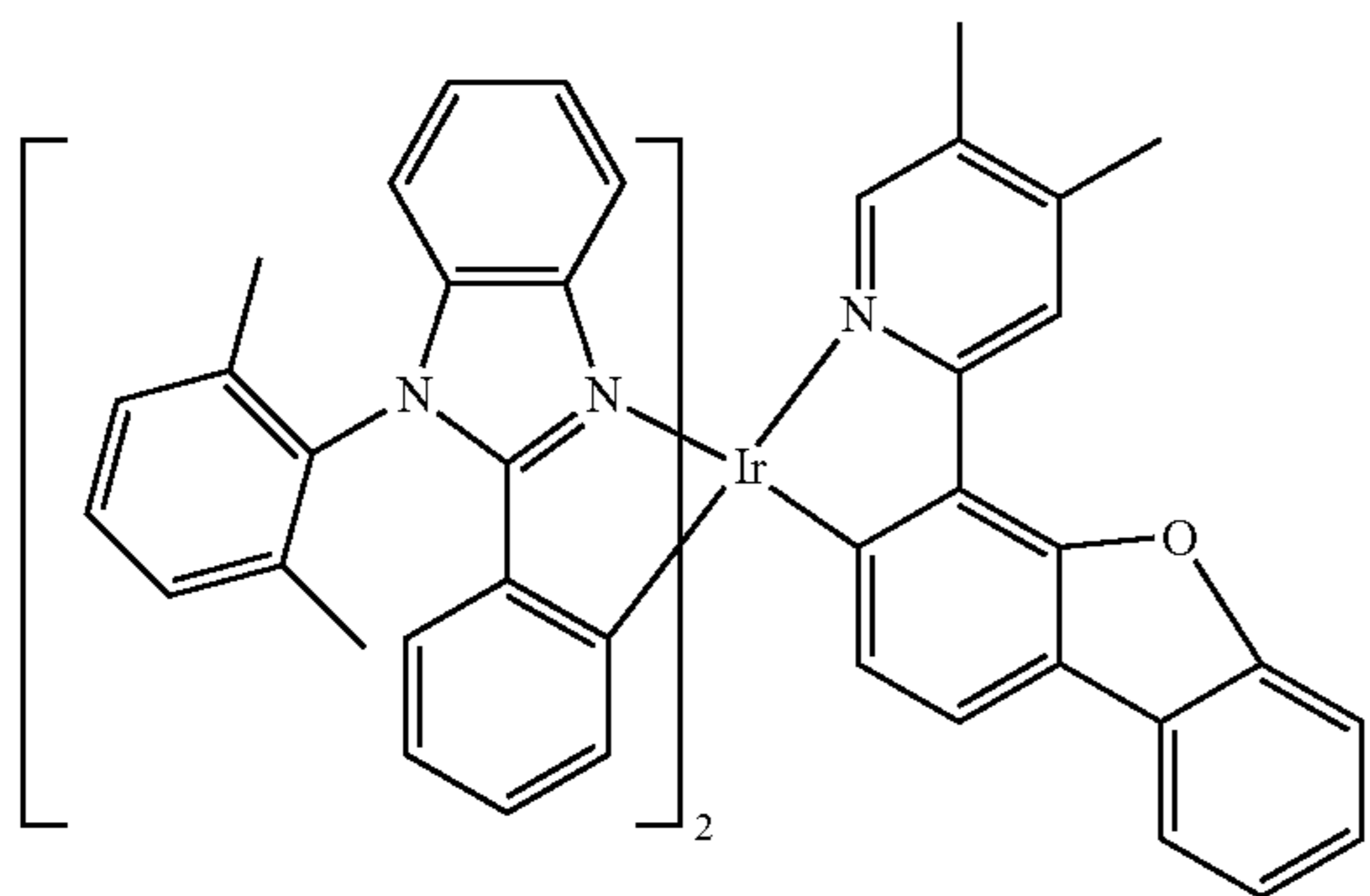
Compound 114
