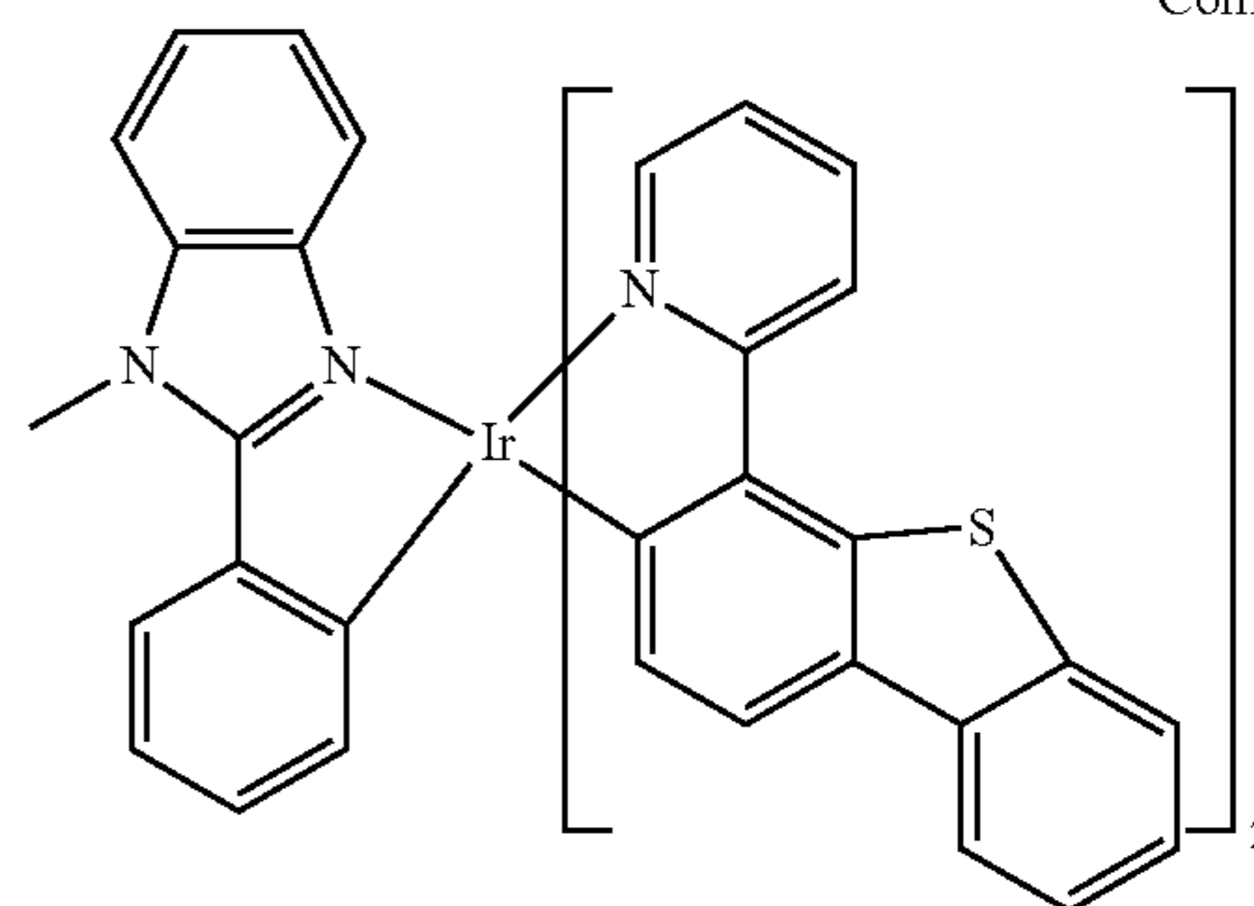
Compound 111
