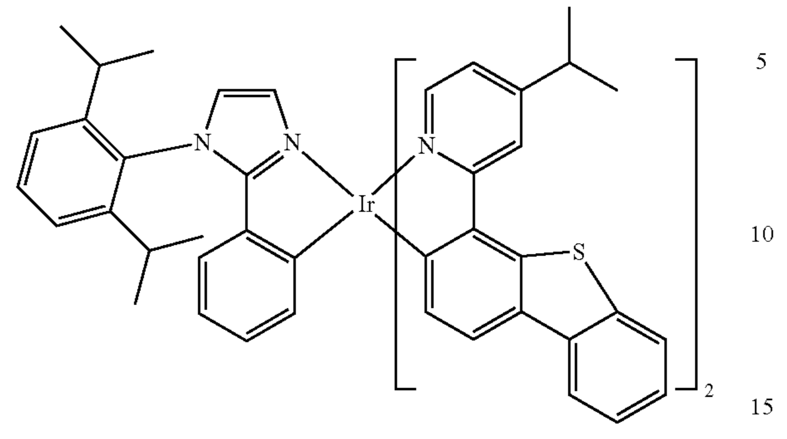
Compound 24
