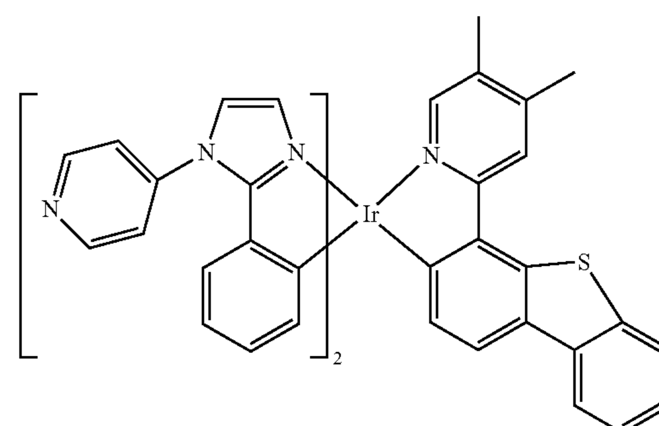
Compound 54
