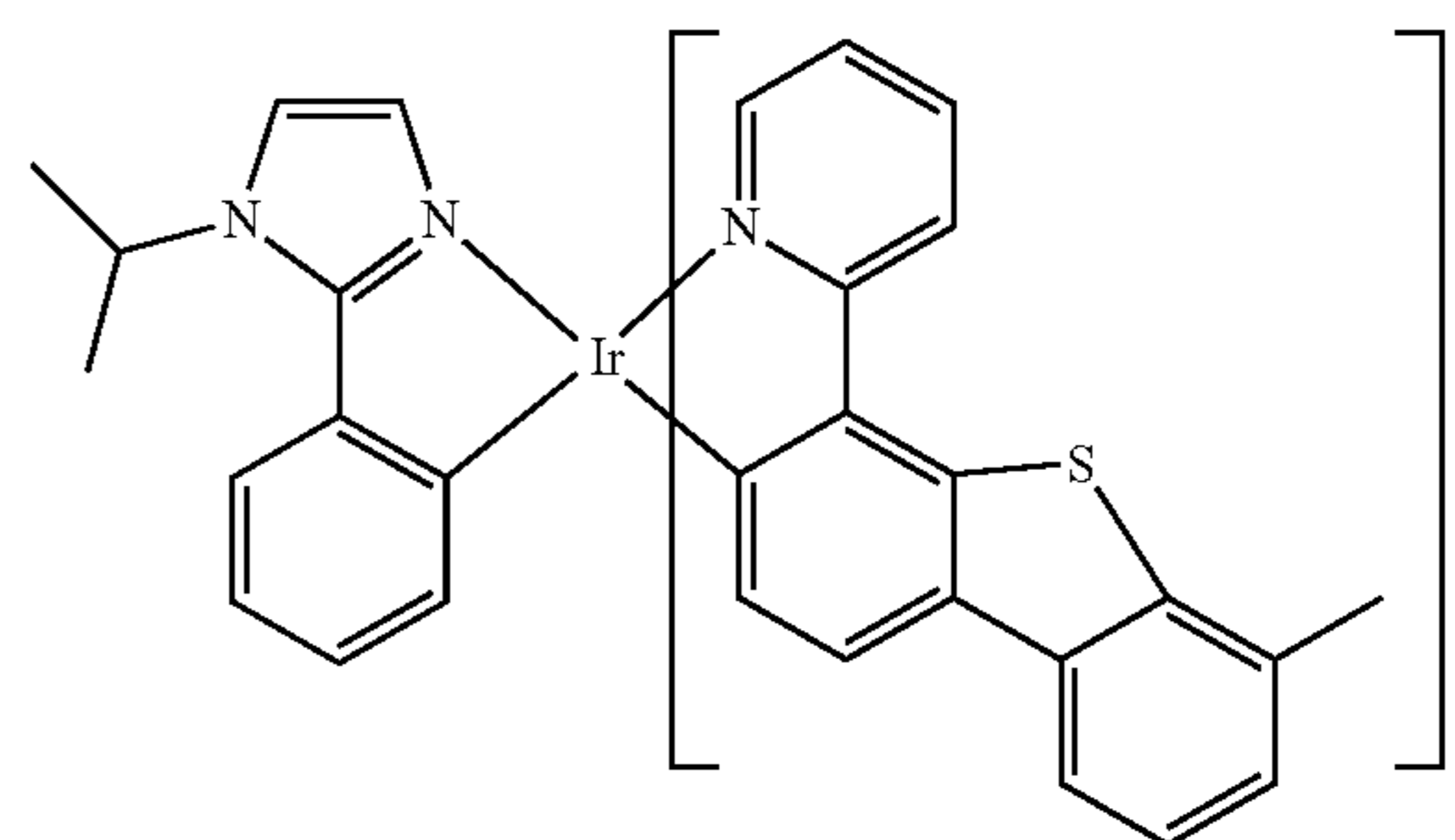
Compound 63
