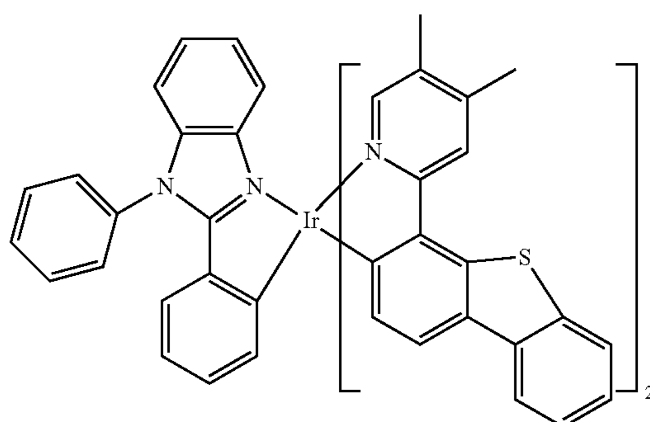
Compound 108
