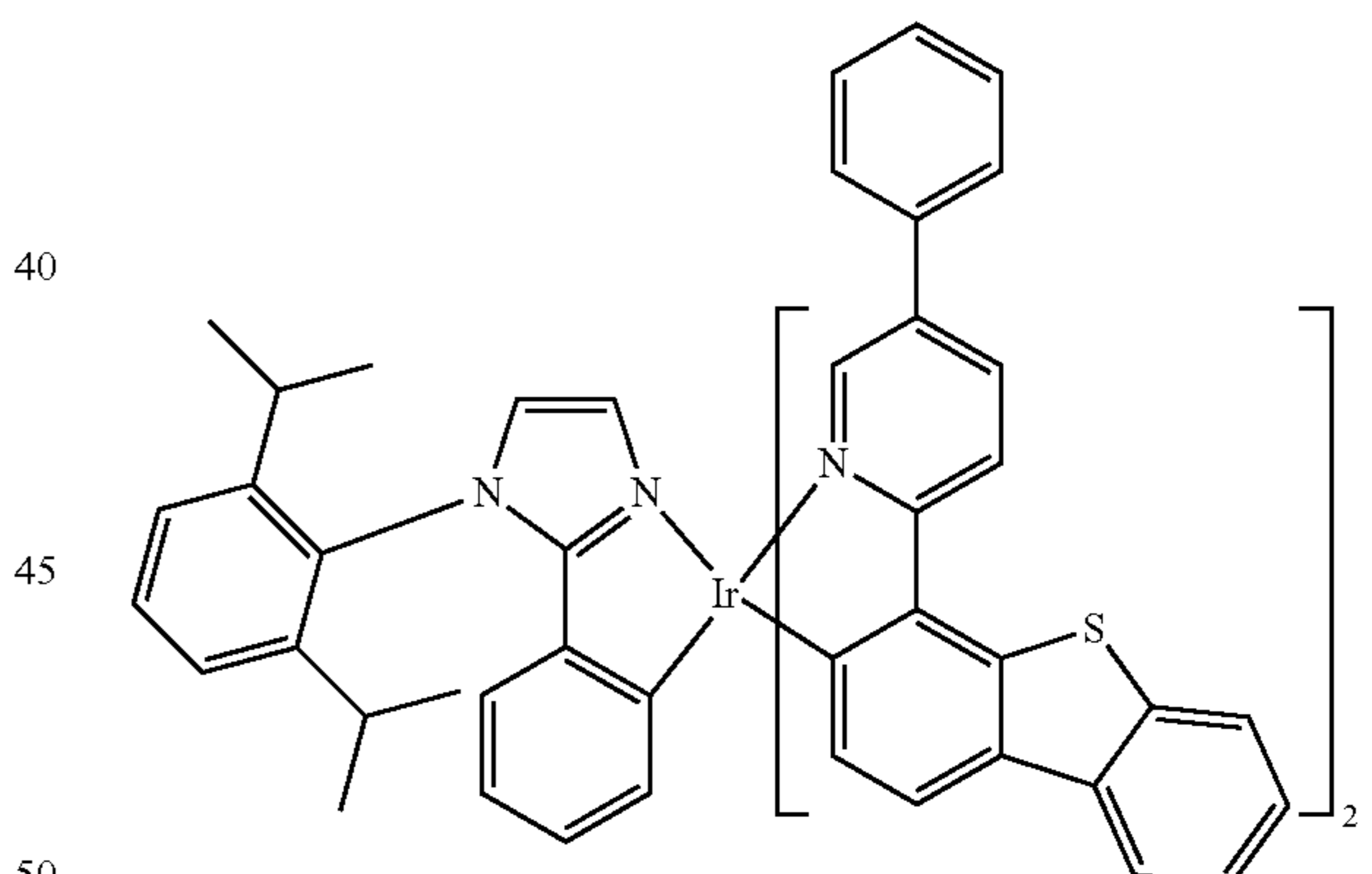
Compound 76
