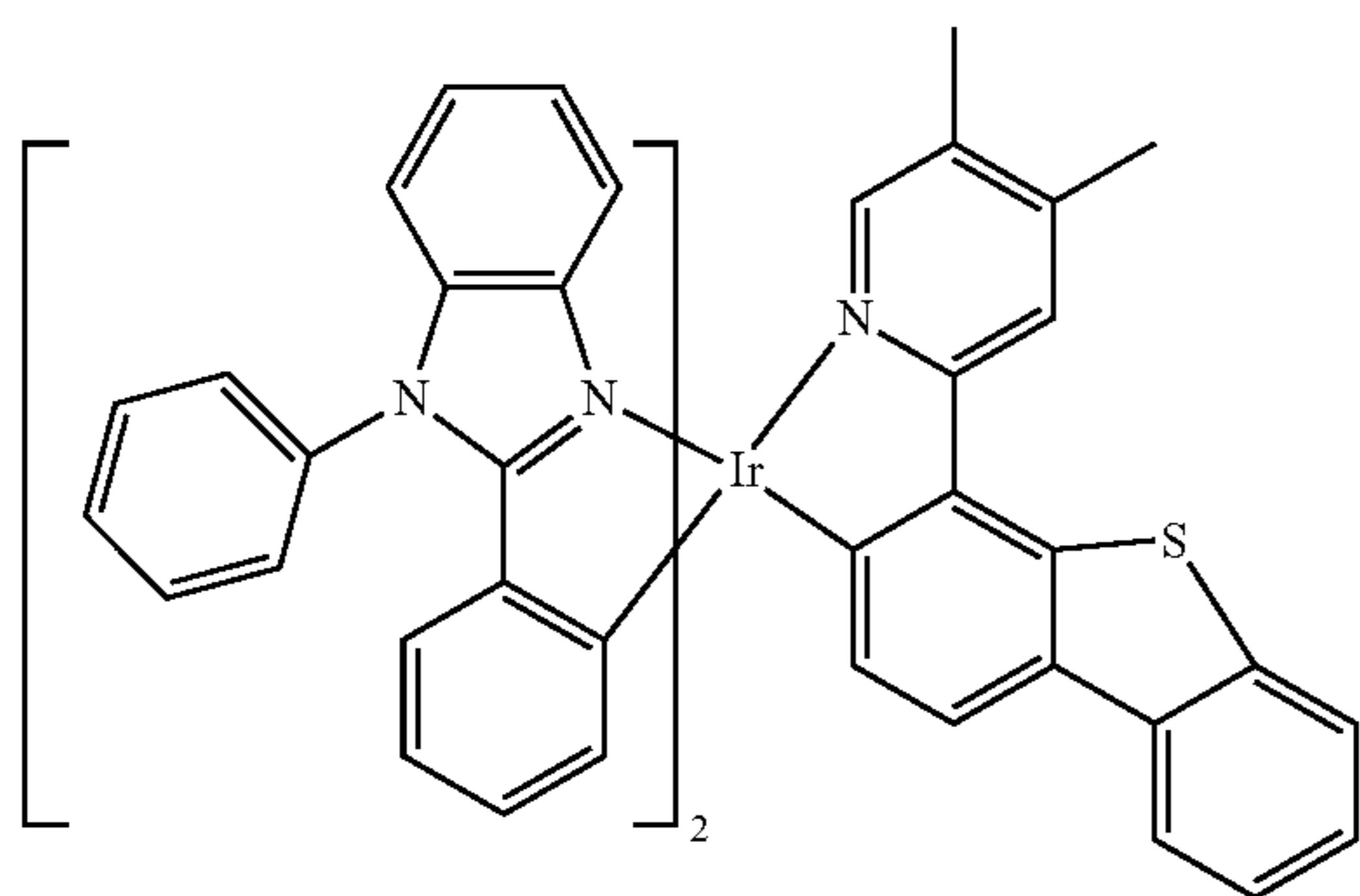
Compound 106
