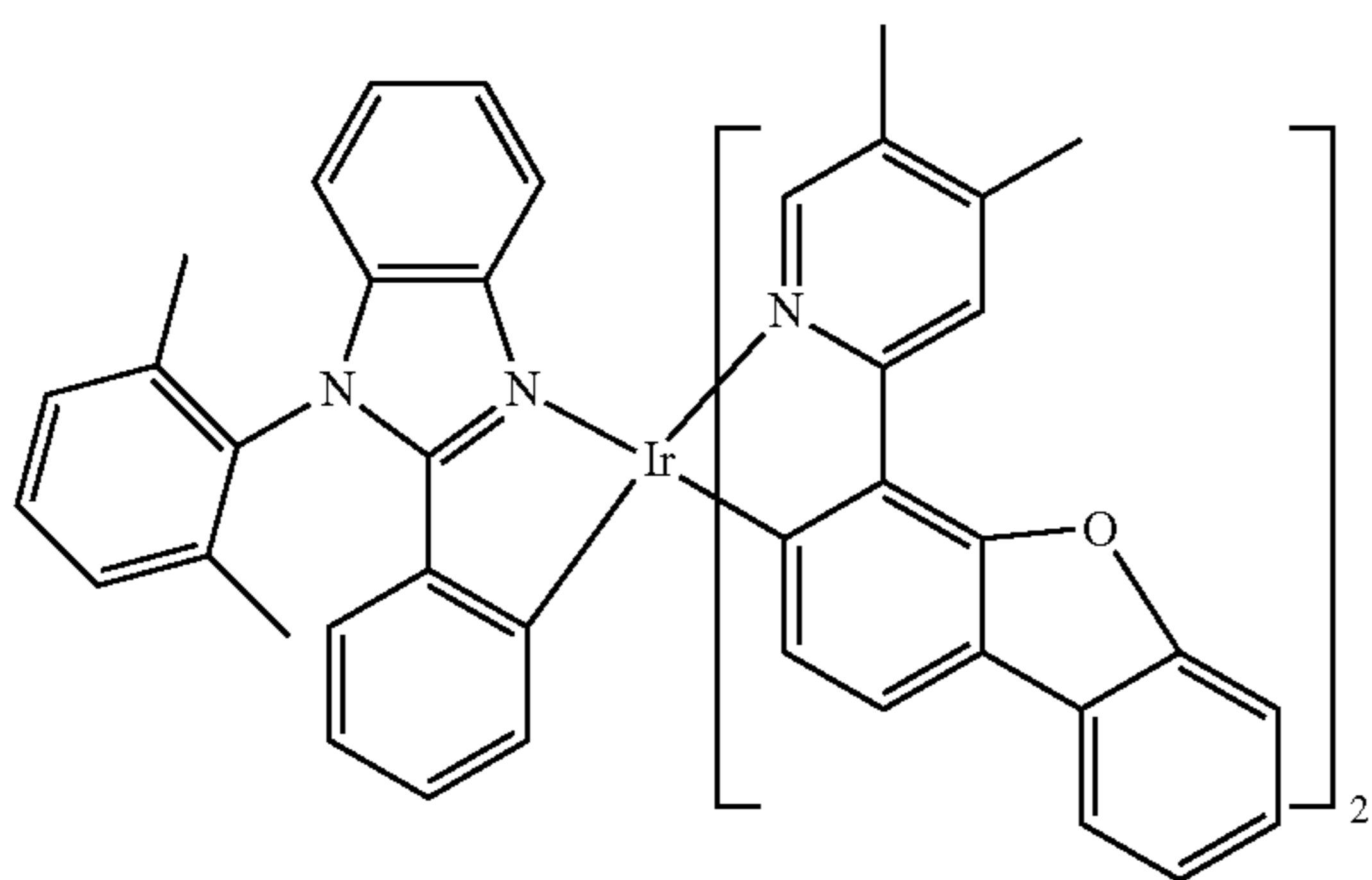
Compound 116
