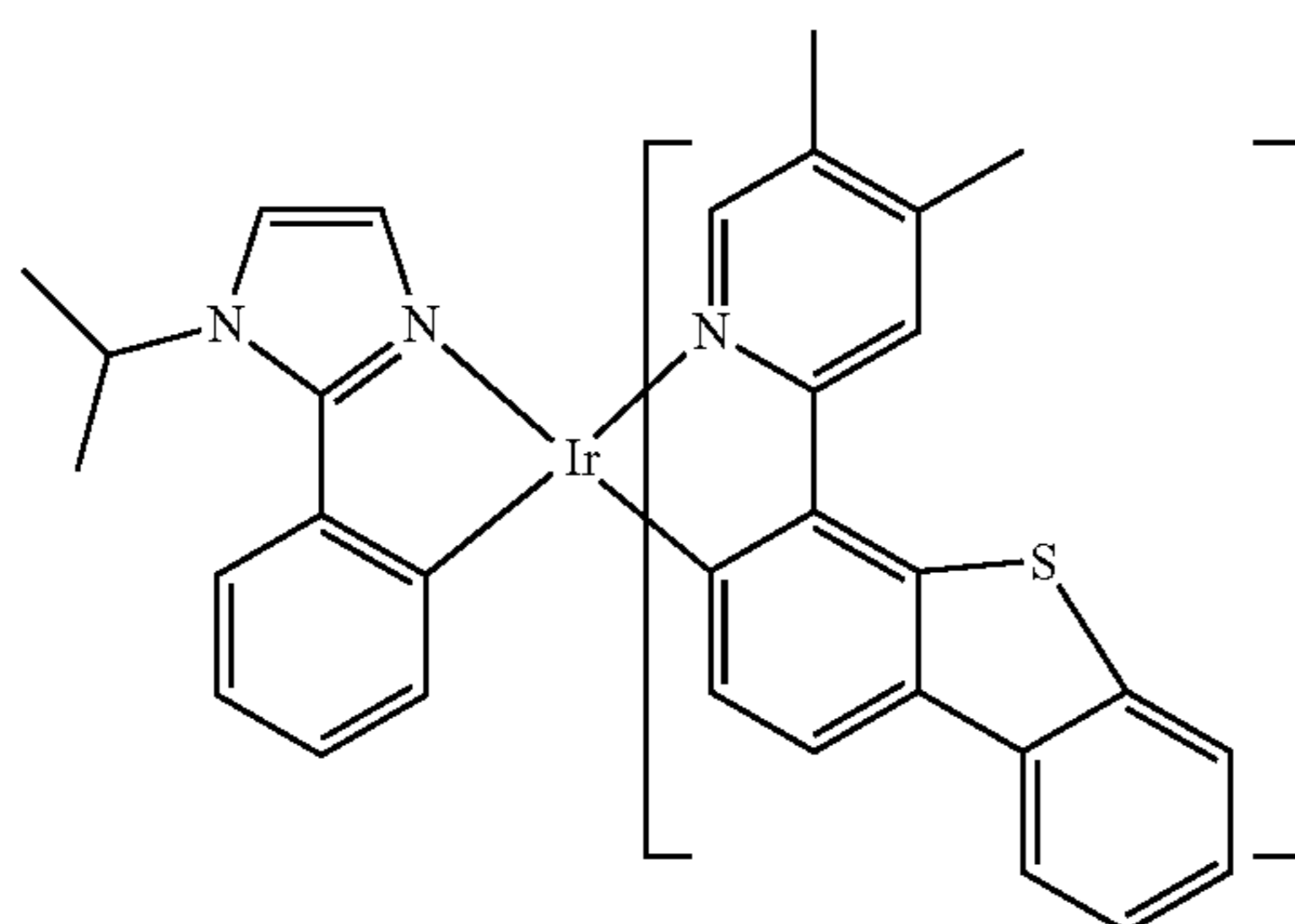
Compound 60
