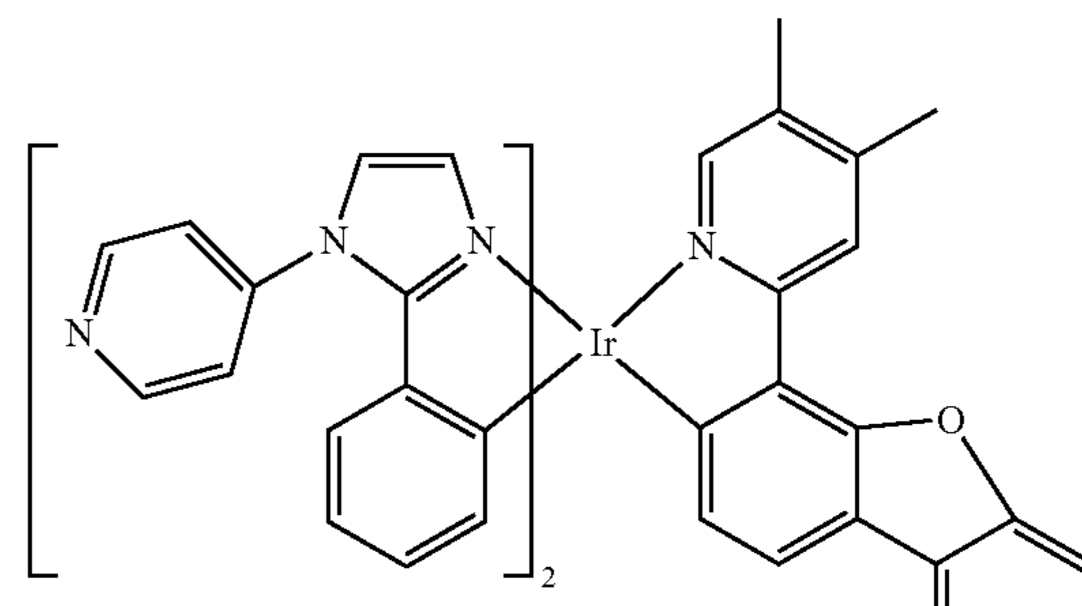
Compound 38
