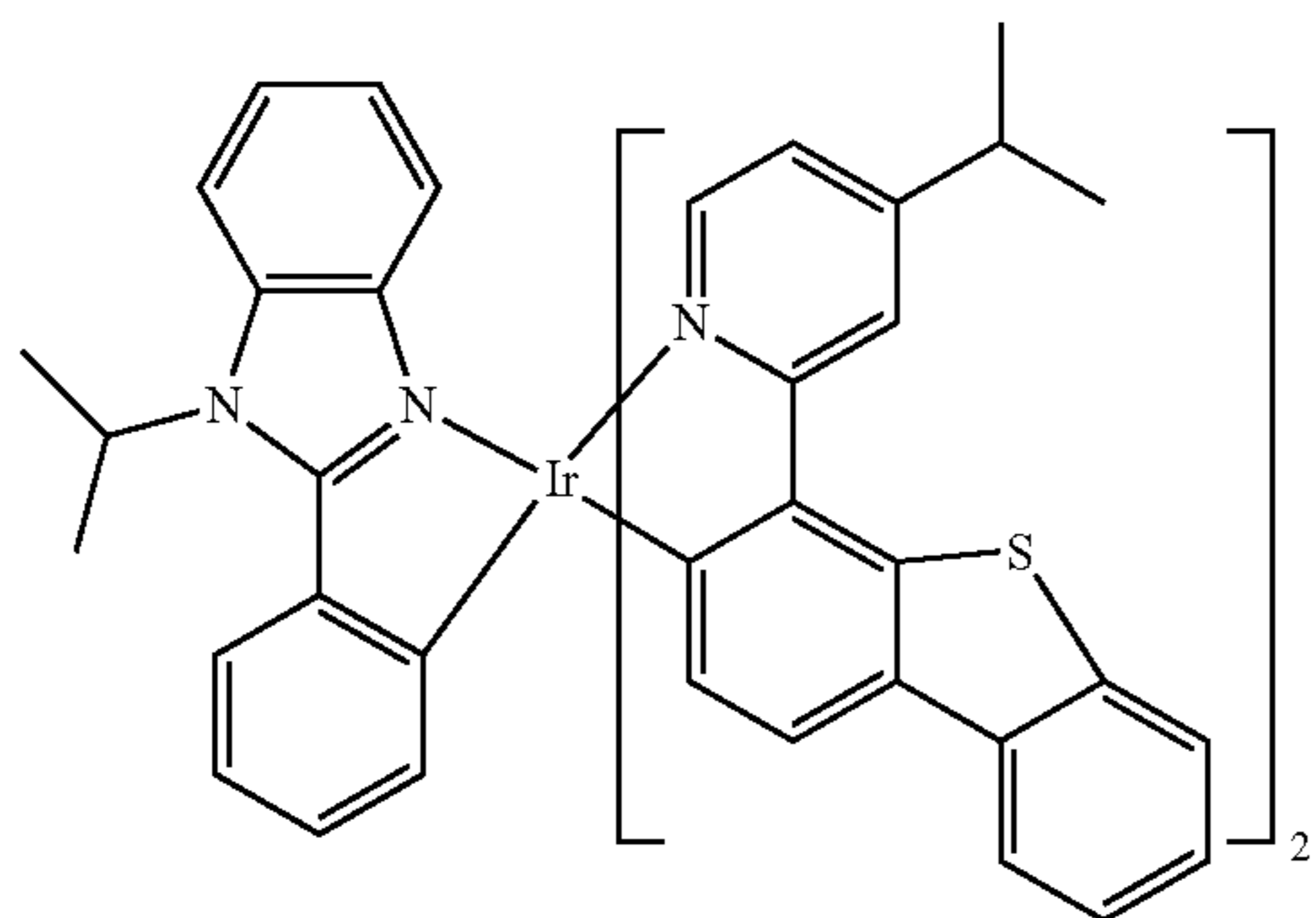
Compound 144
