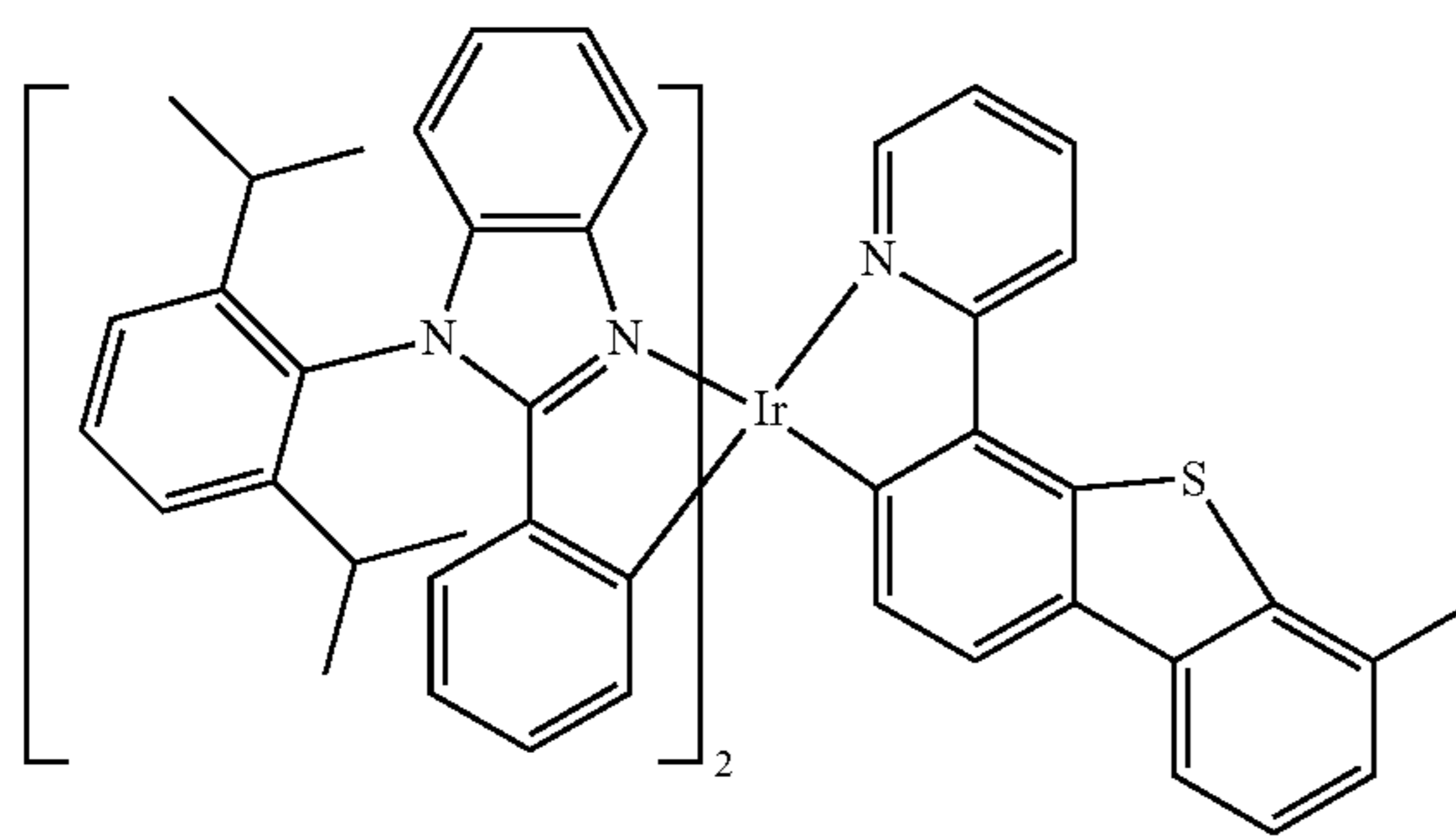
Compound 101
