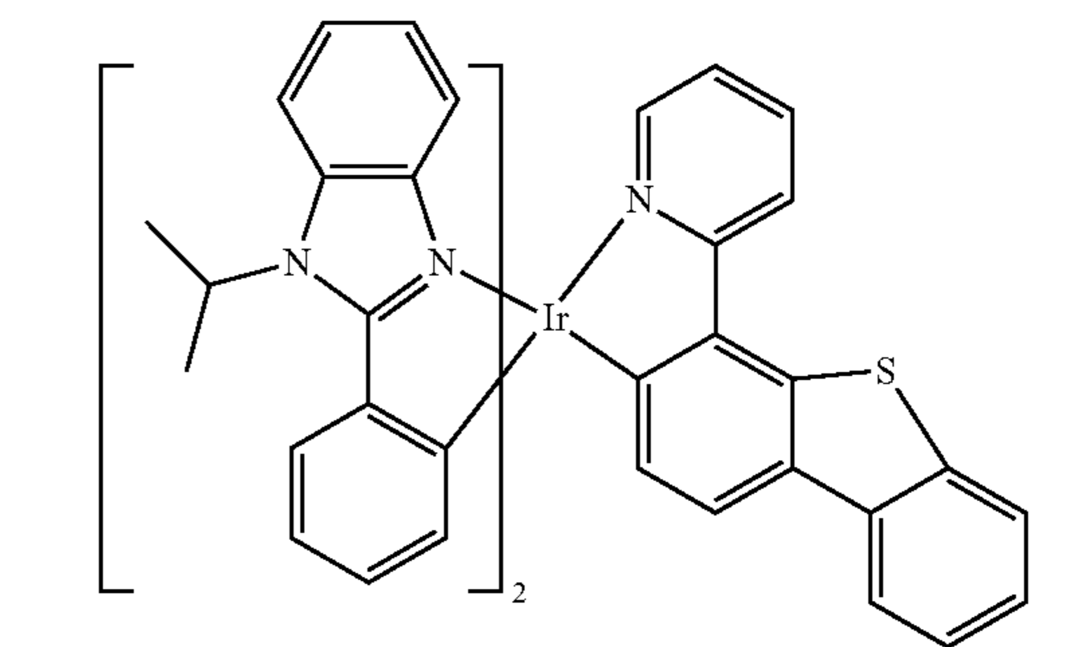
Compound 137
