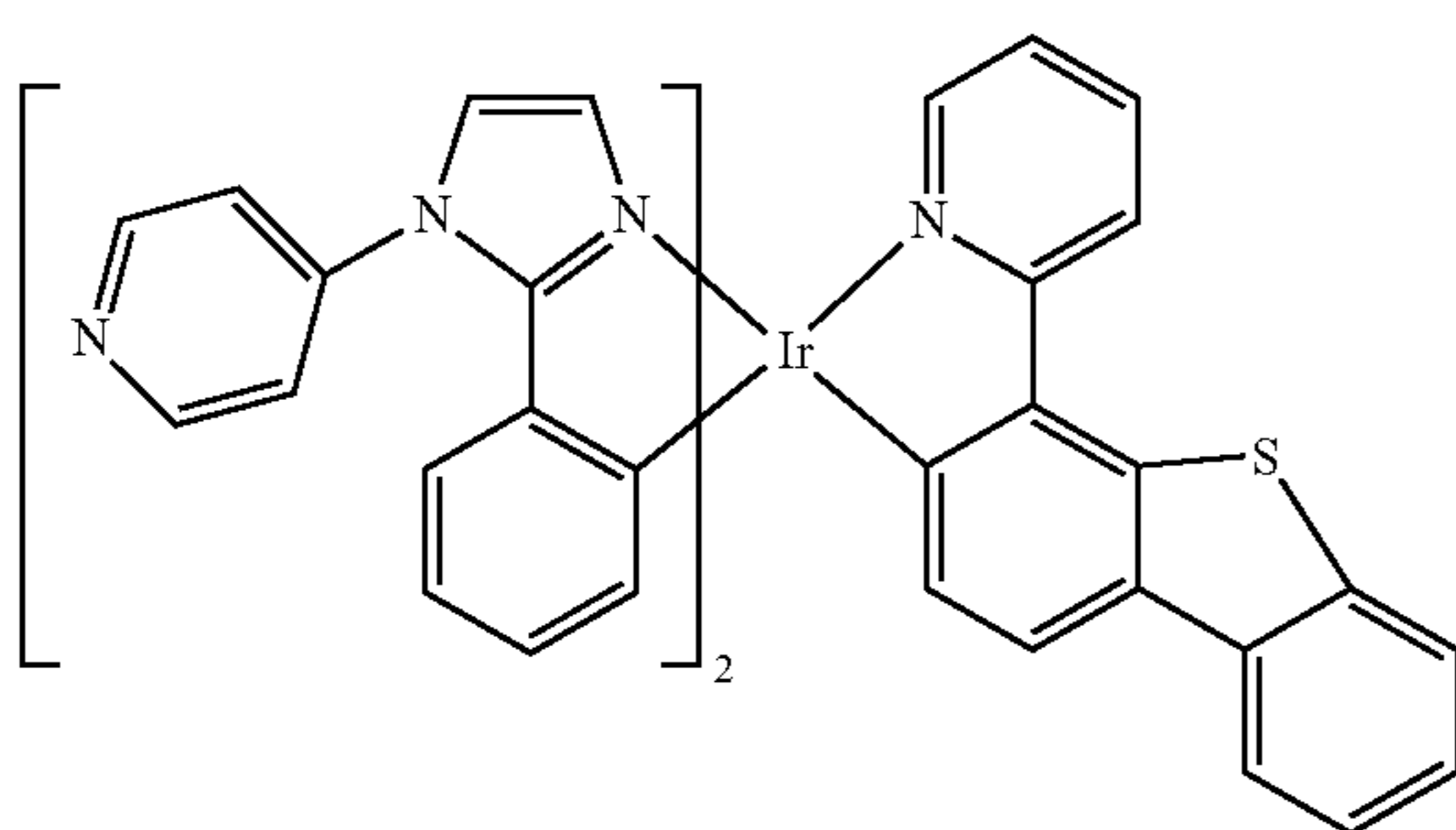
Compound 53
