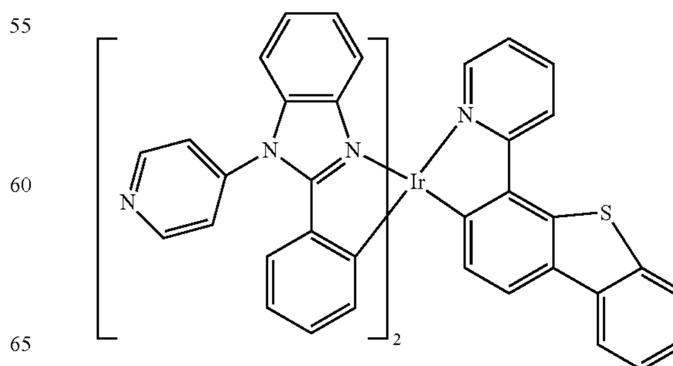
Compound 133
