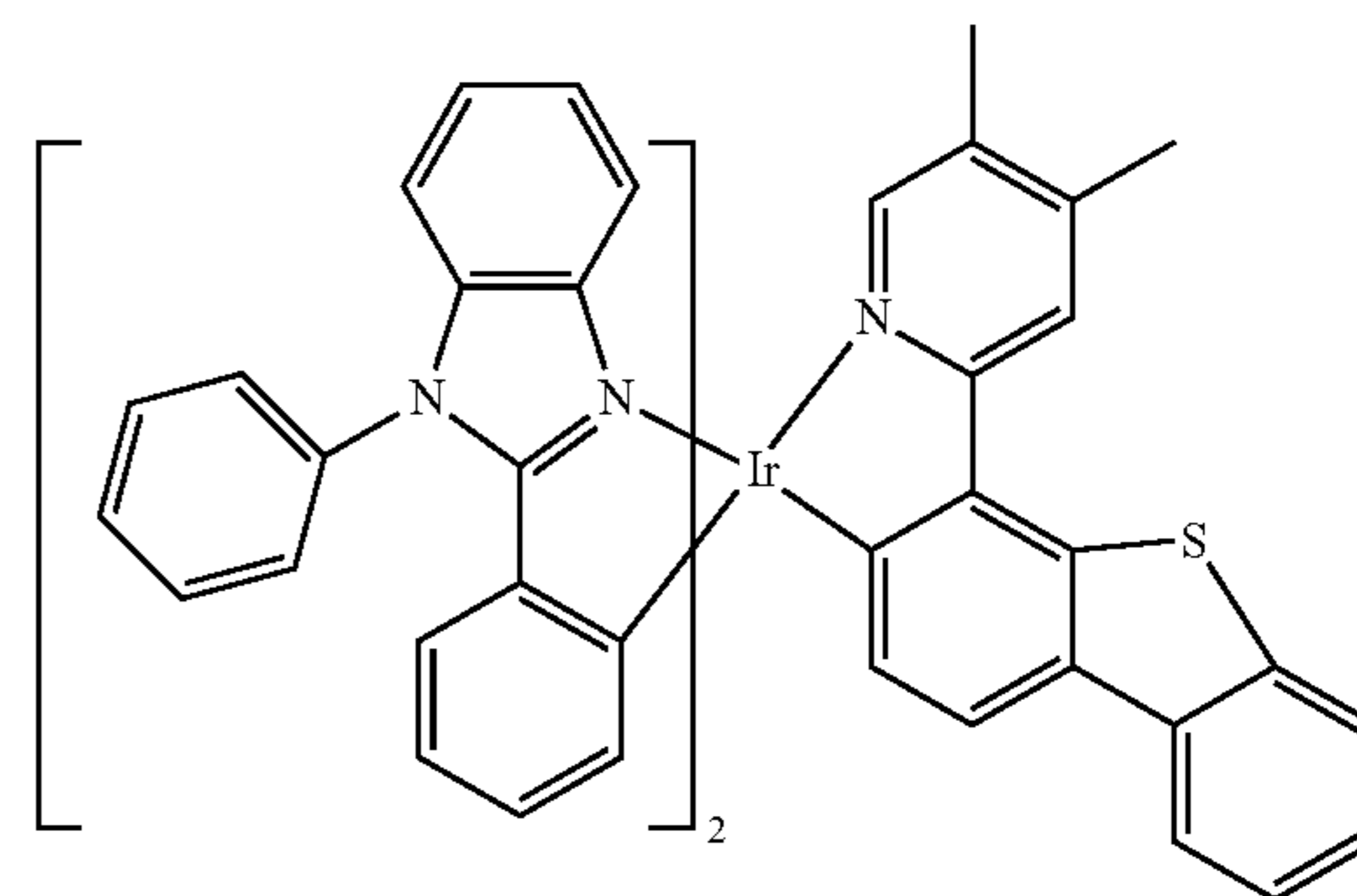
Compound 106
