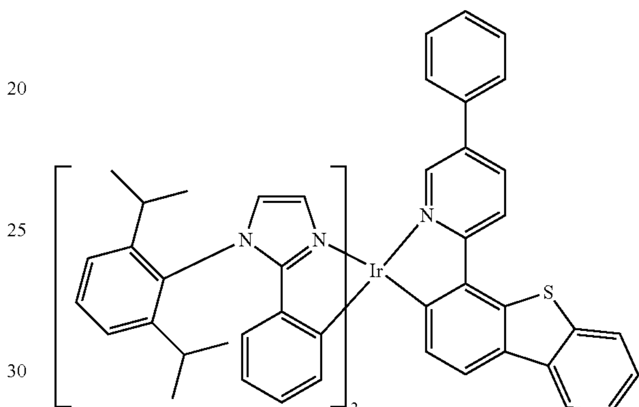
Compound 75
