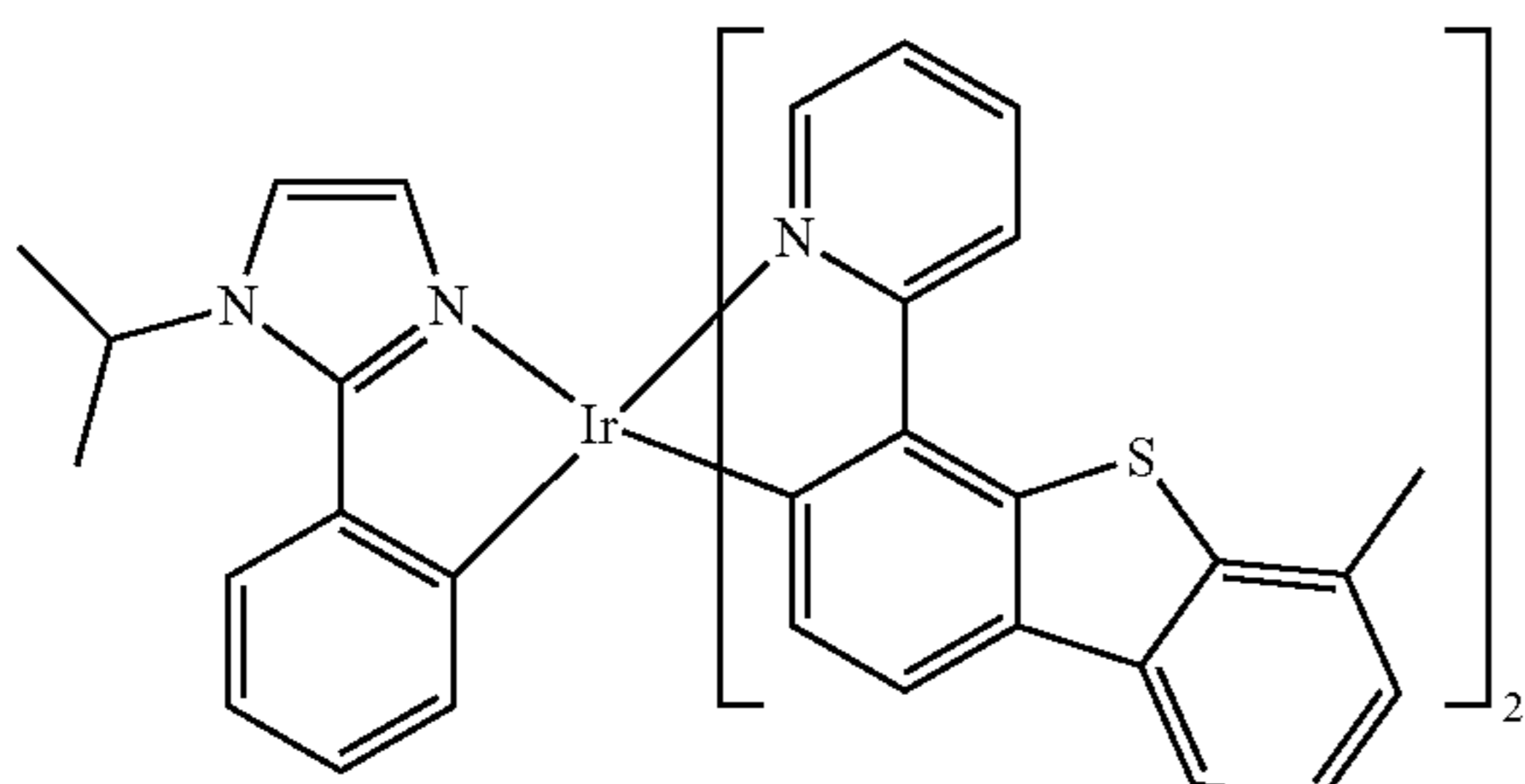
Compound 63
