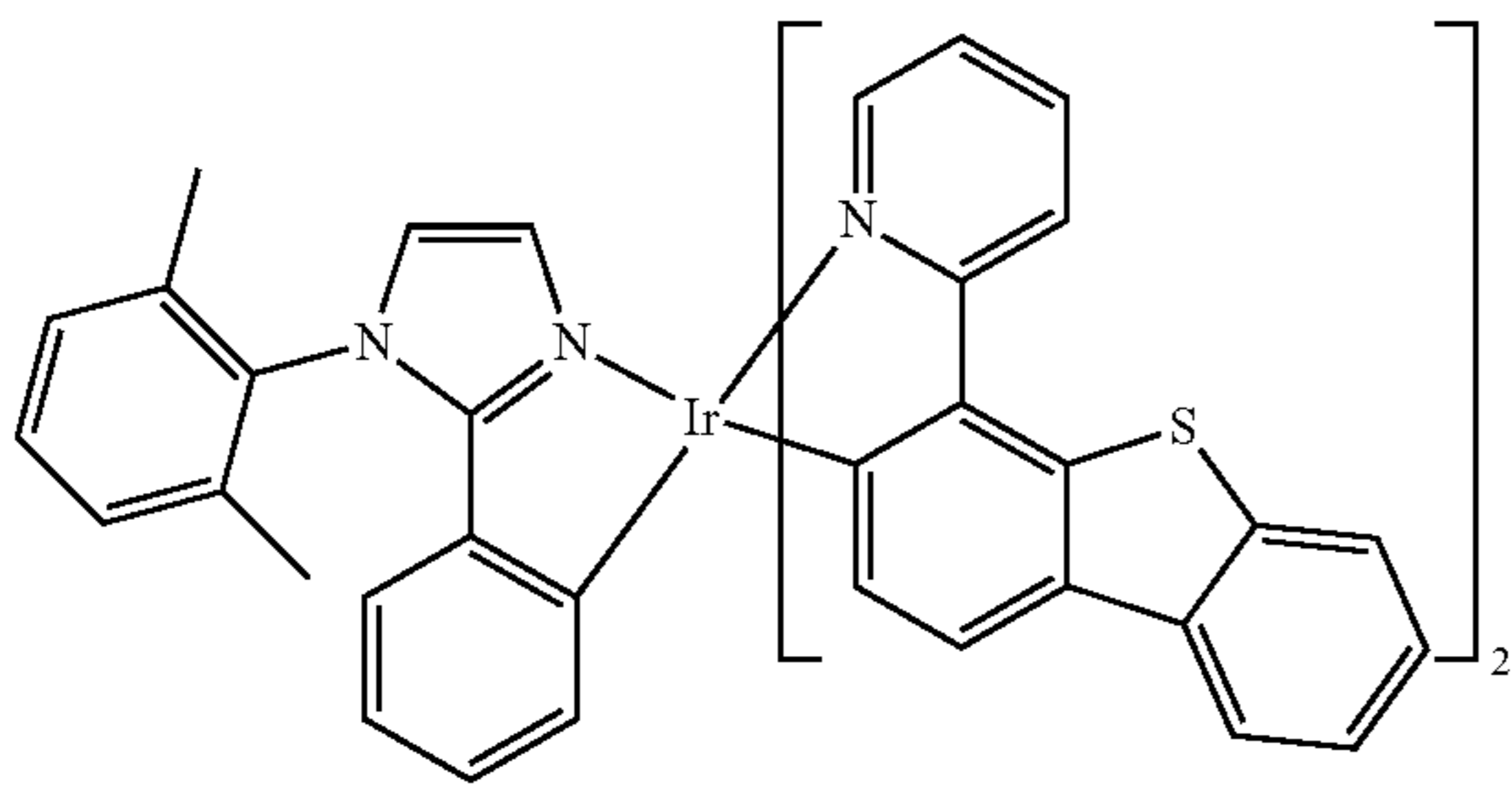
Compound 52
