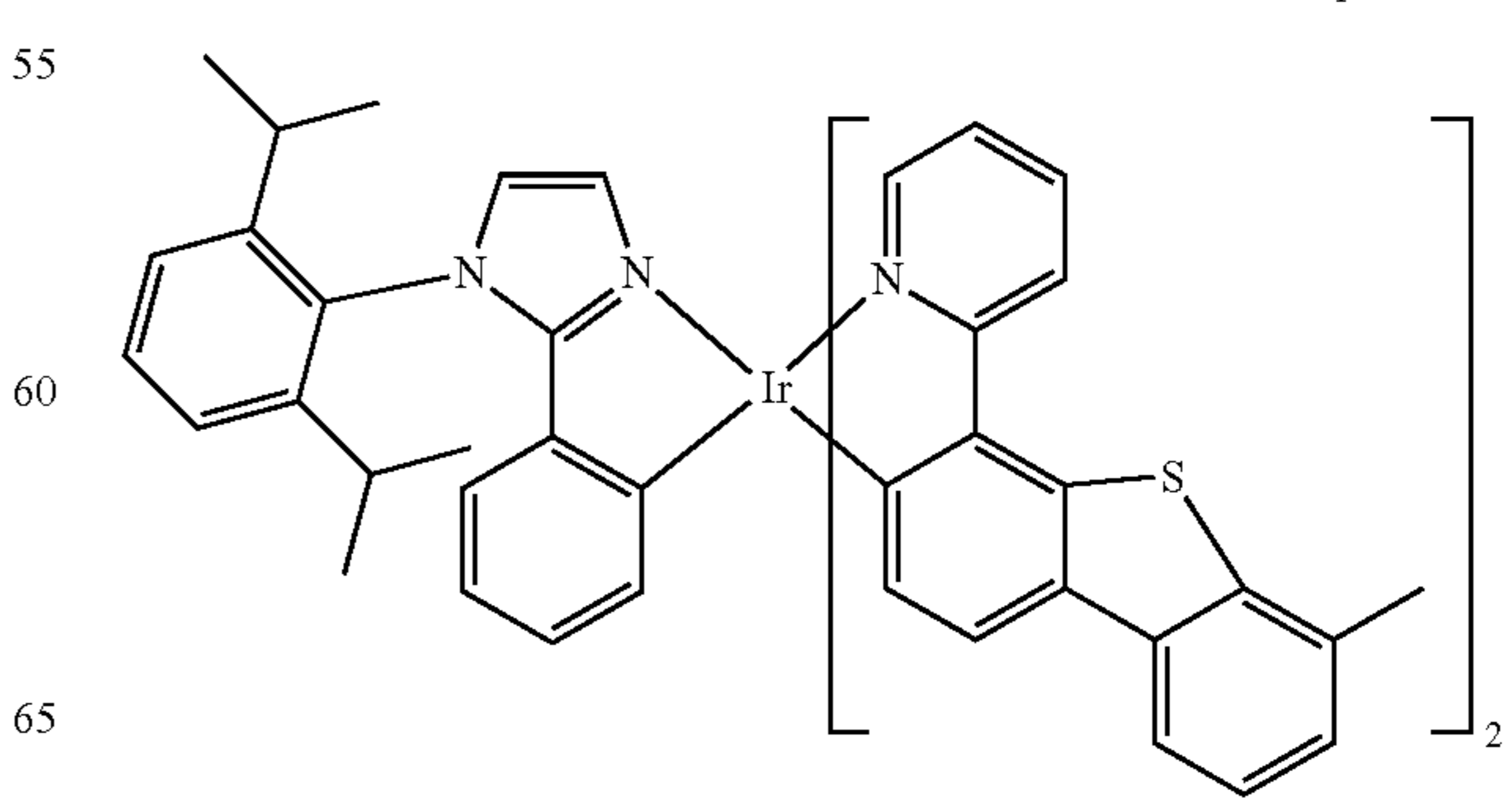
Compound 23
