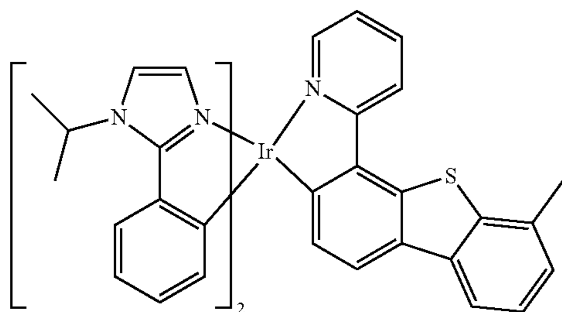
Compound 62
