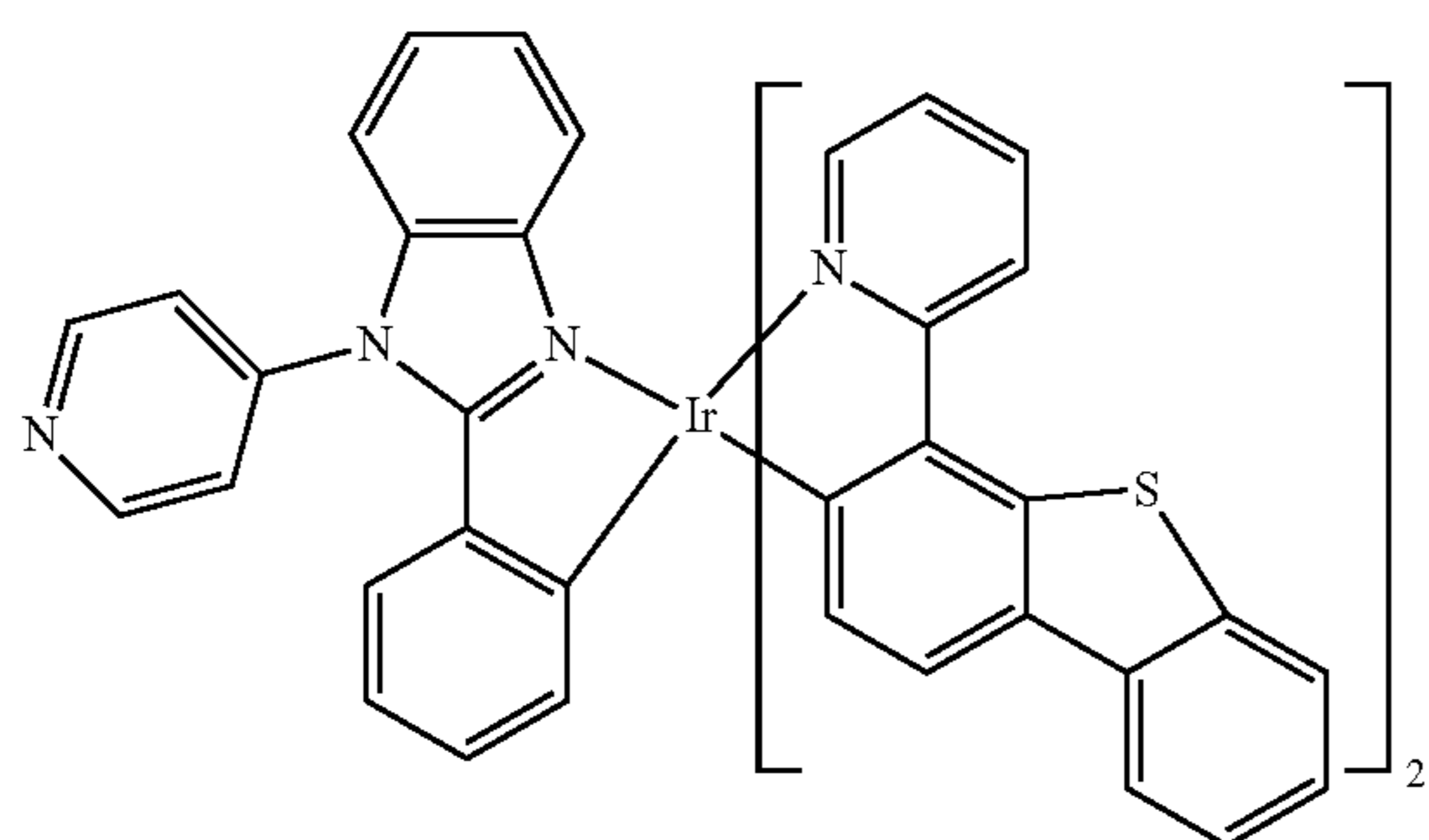
Compound 135
