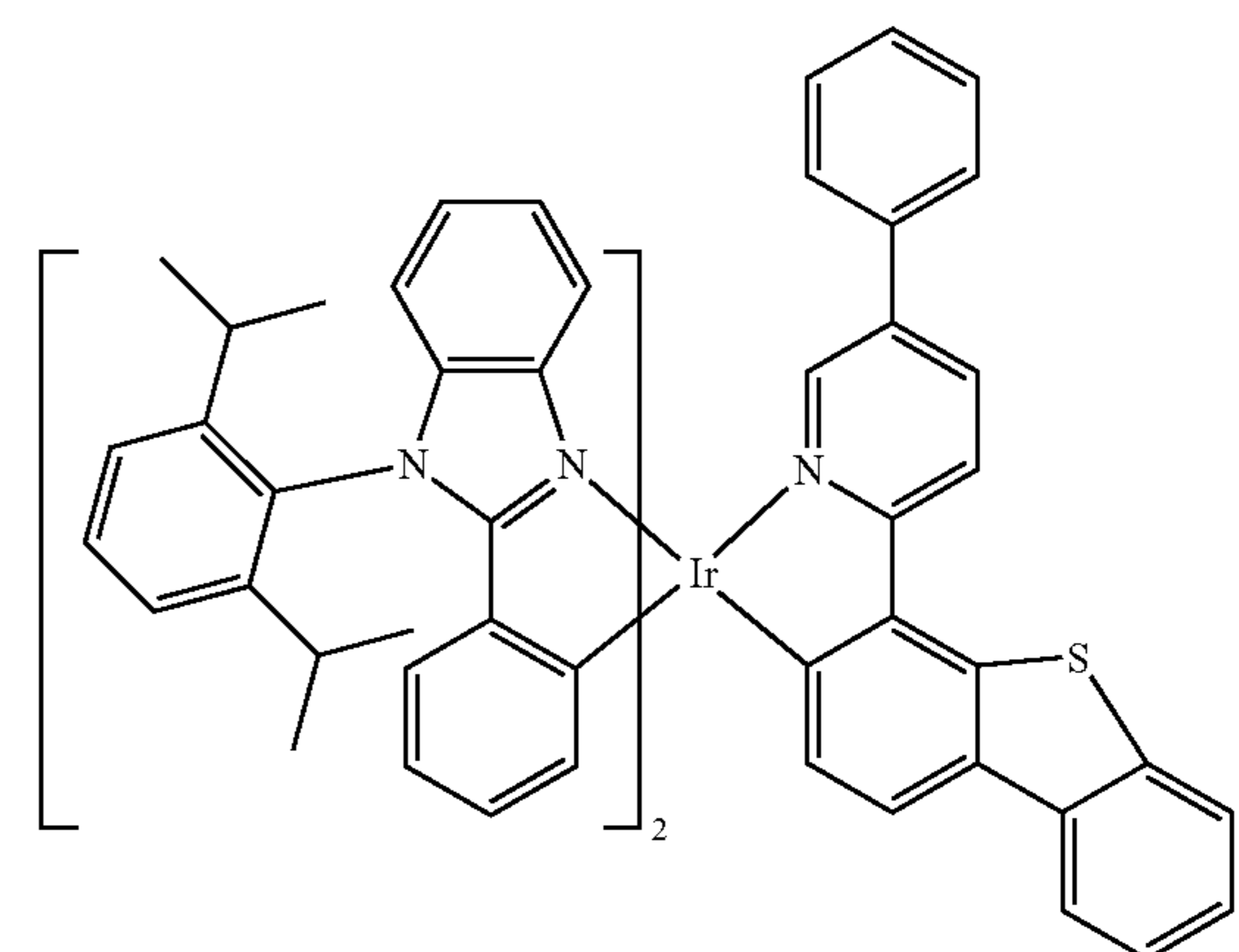
Compound 152
