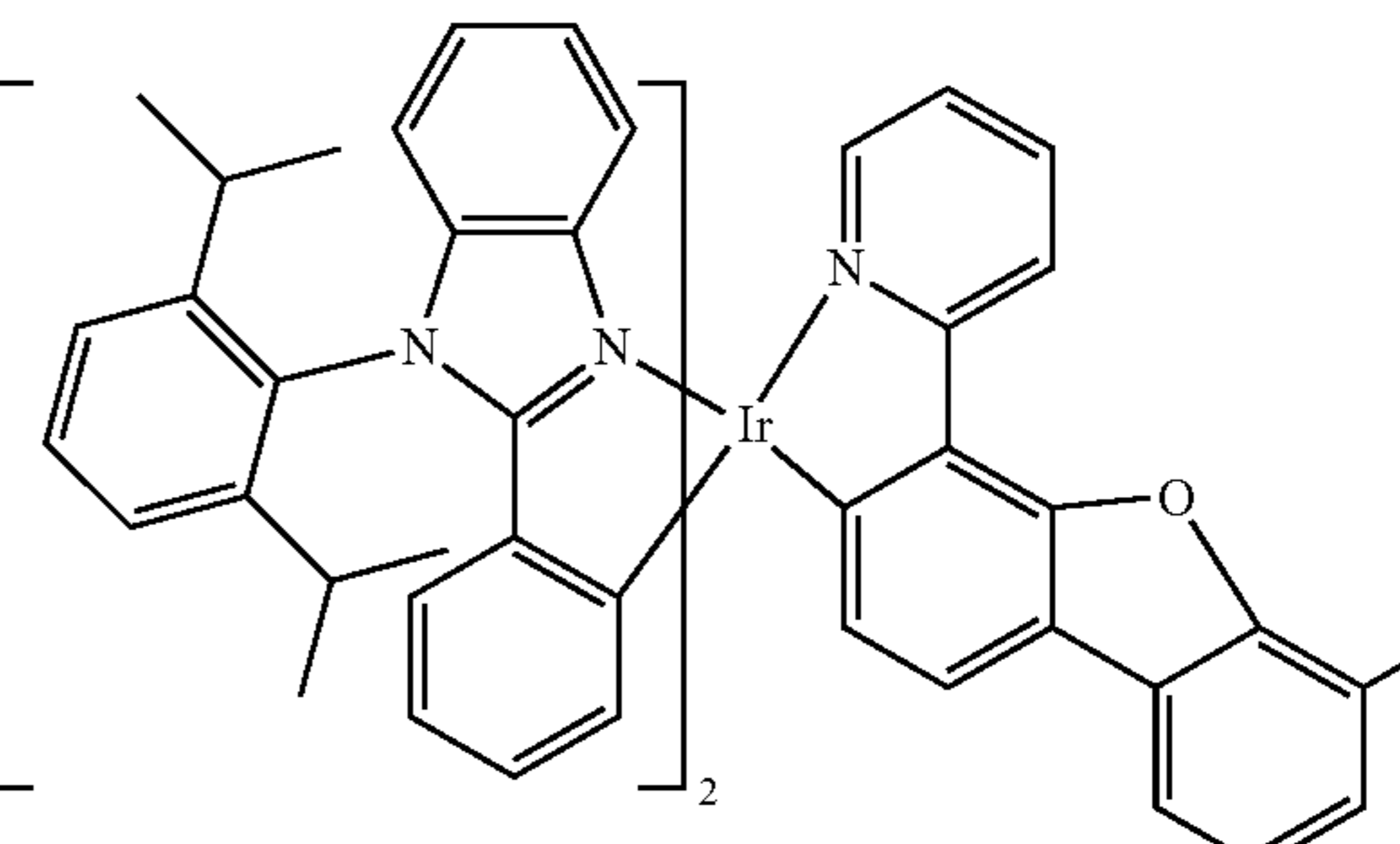
Compound 85
