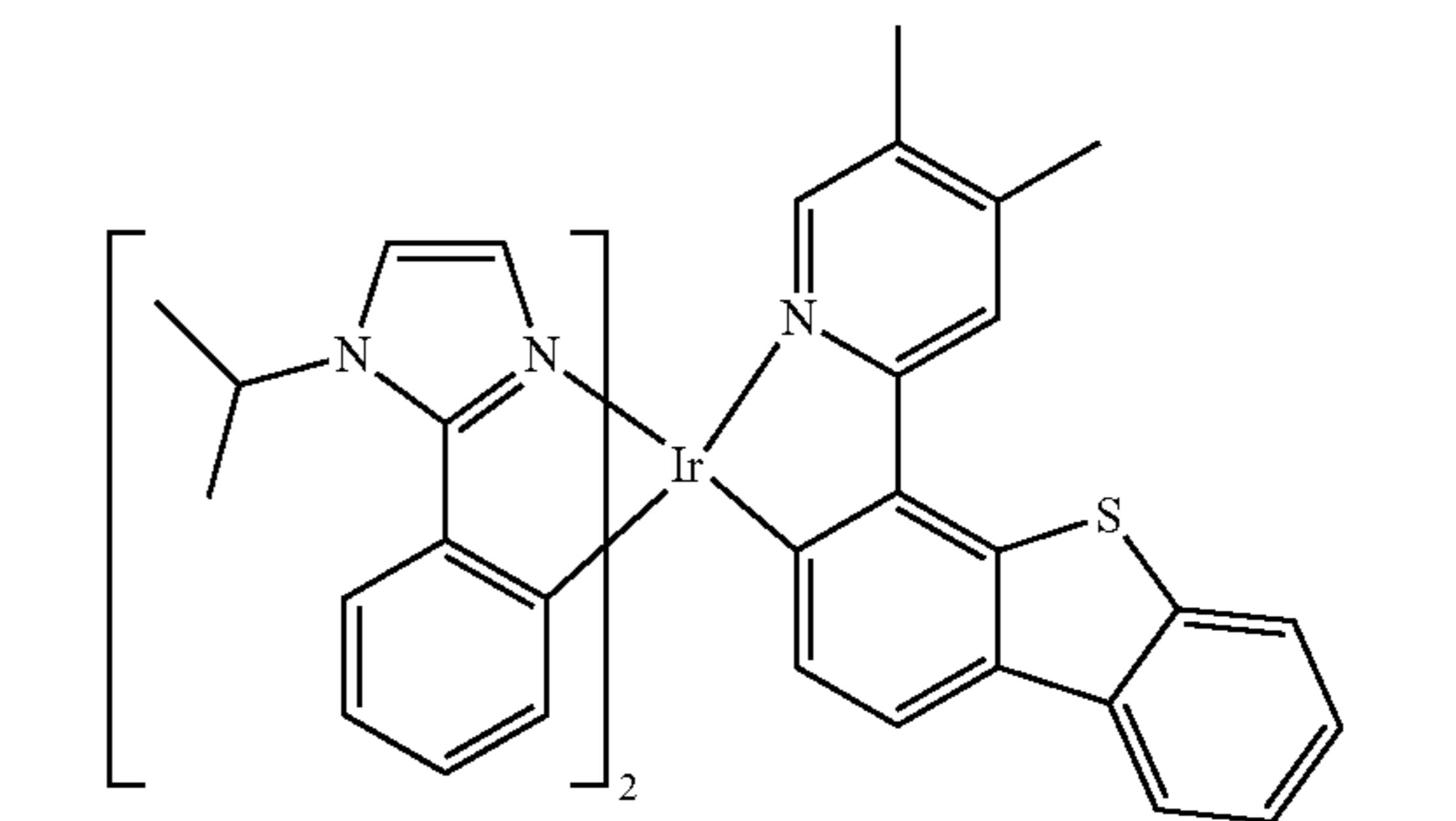
Compound 58
