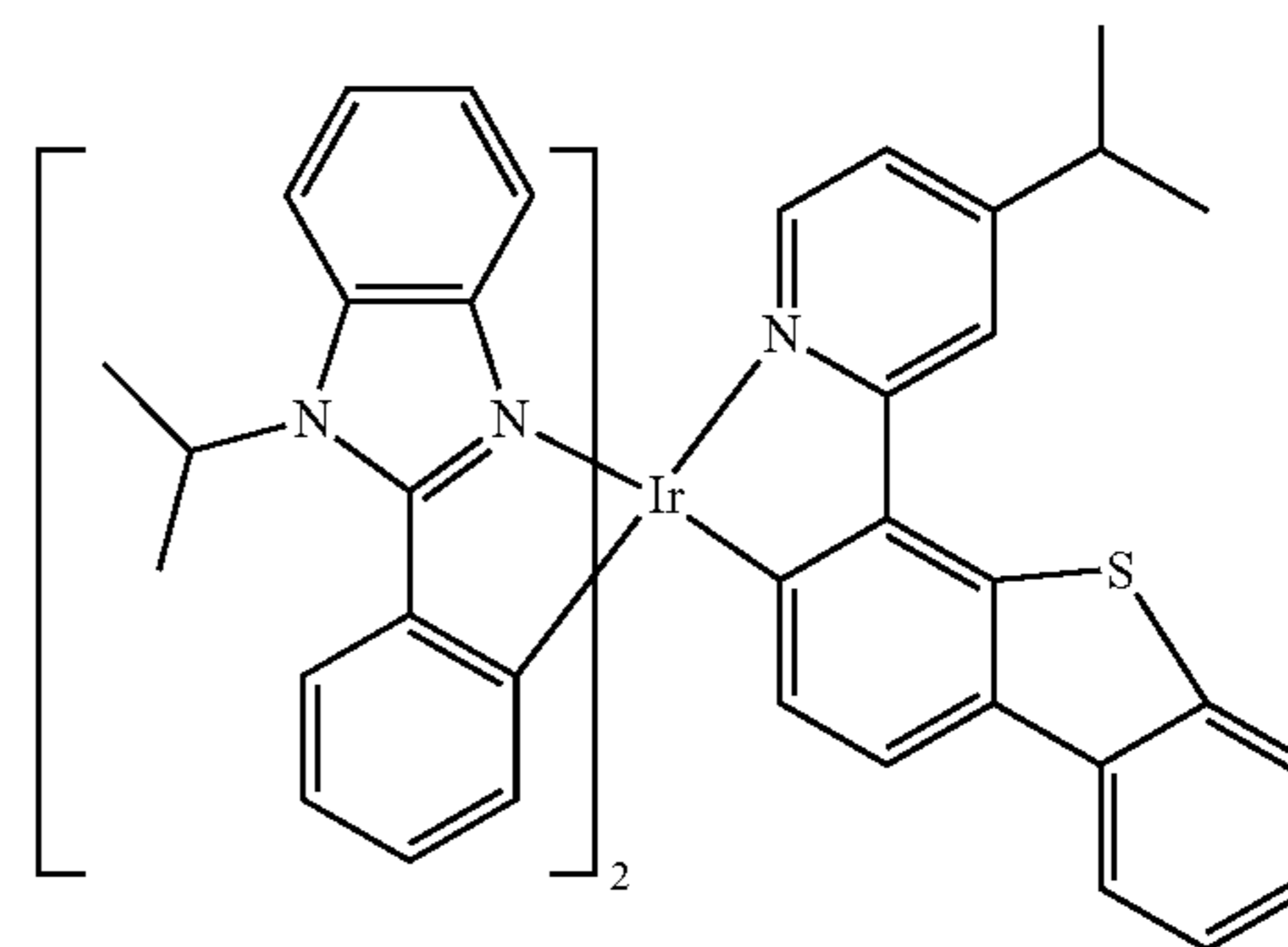
Compound 142
