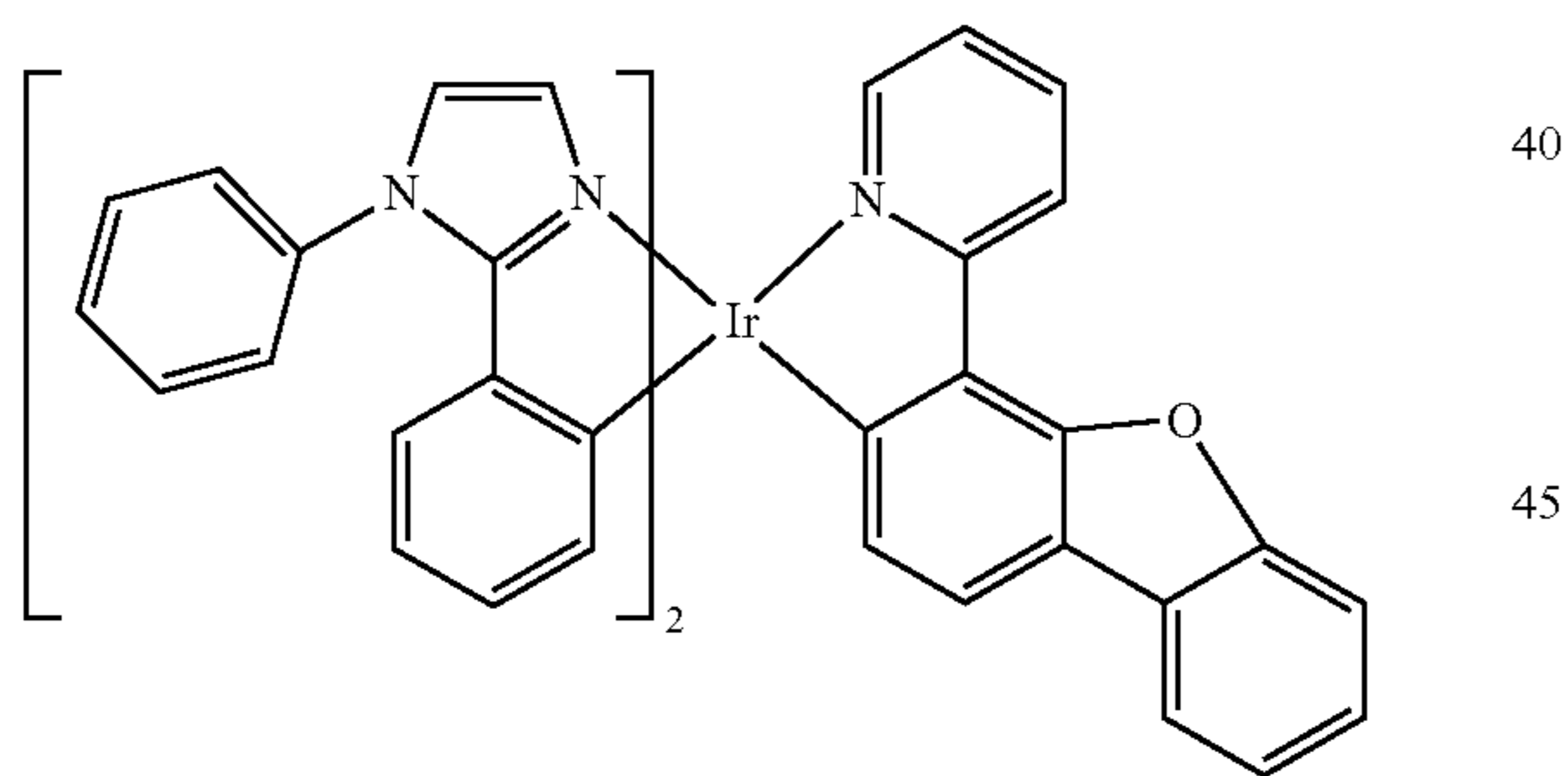
Compound 9
