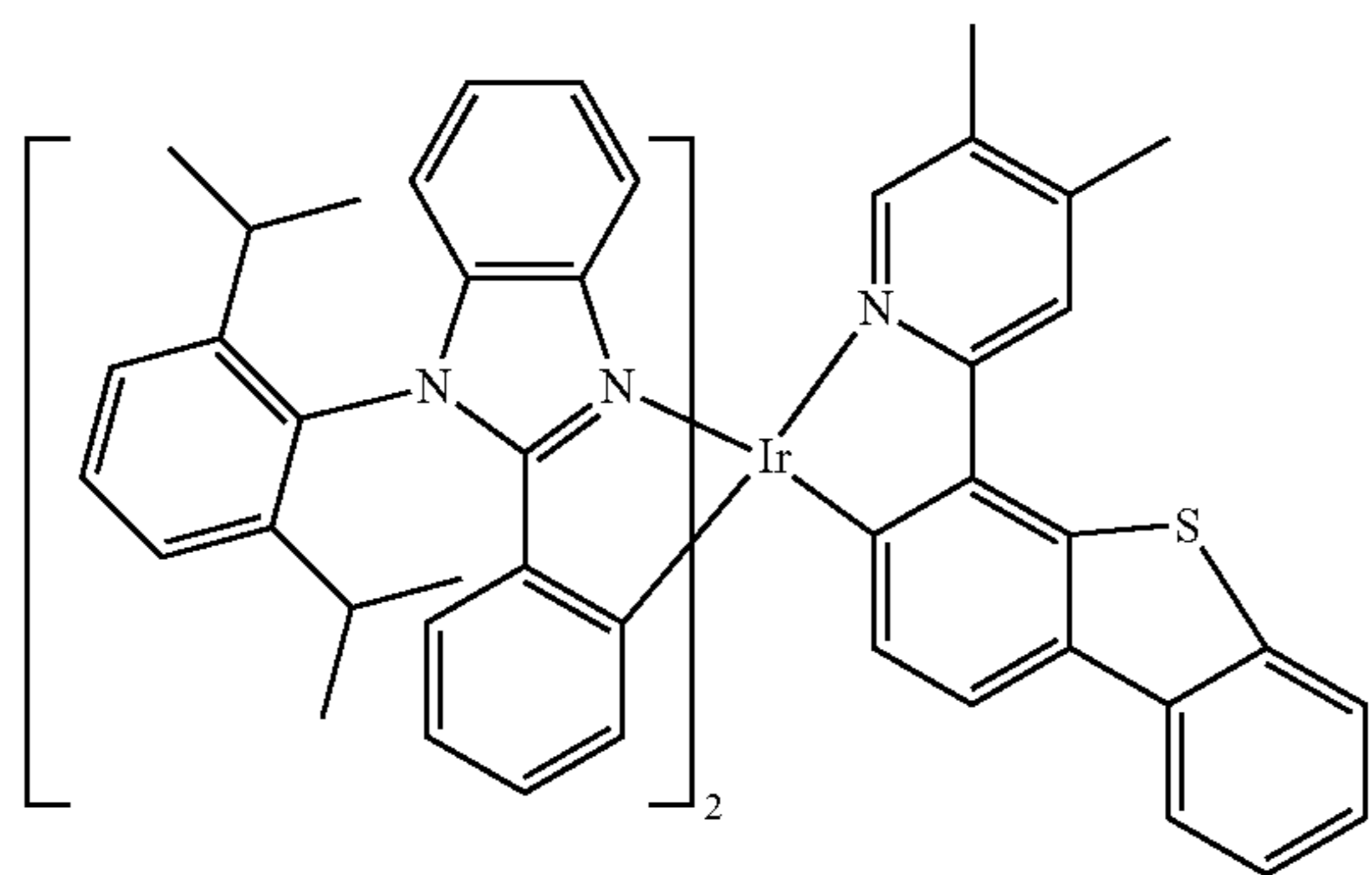
Compound 98
