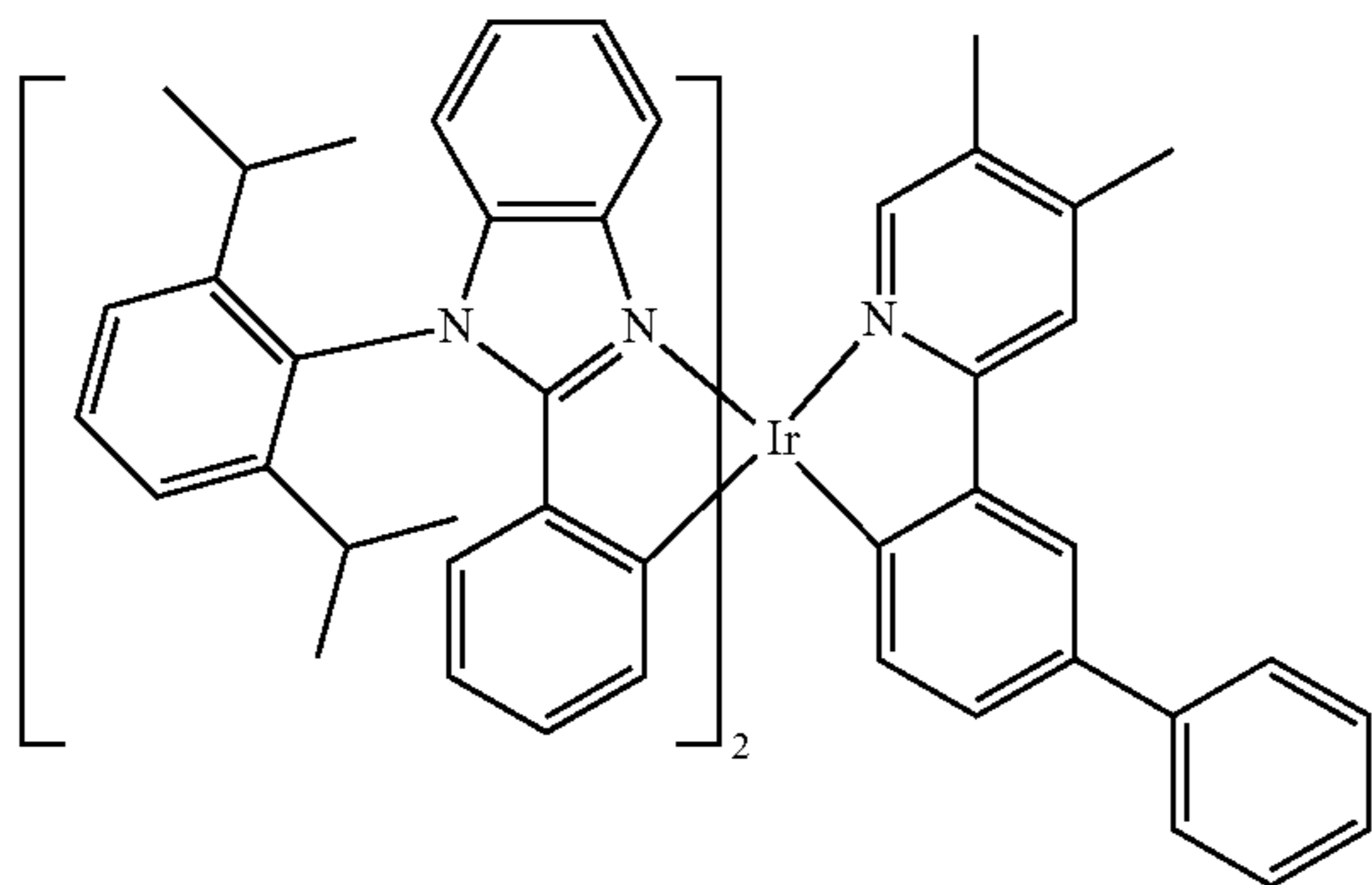
Compound C
