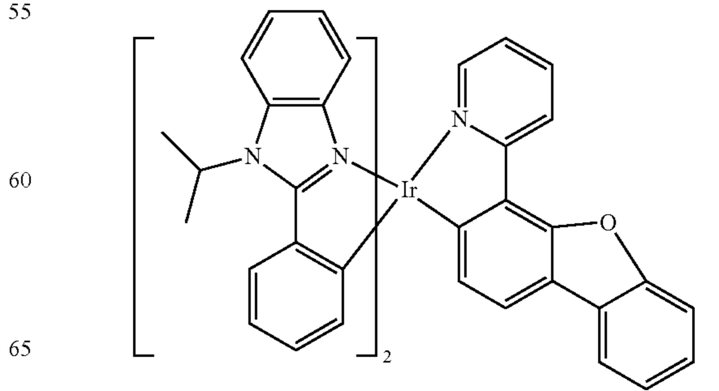
Compound 121
