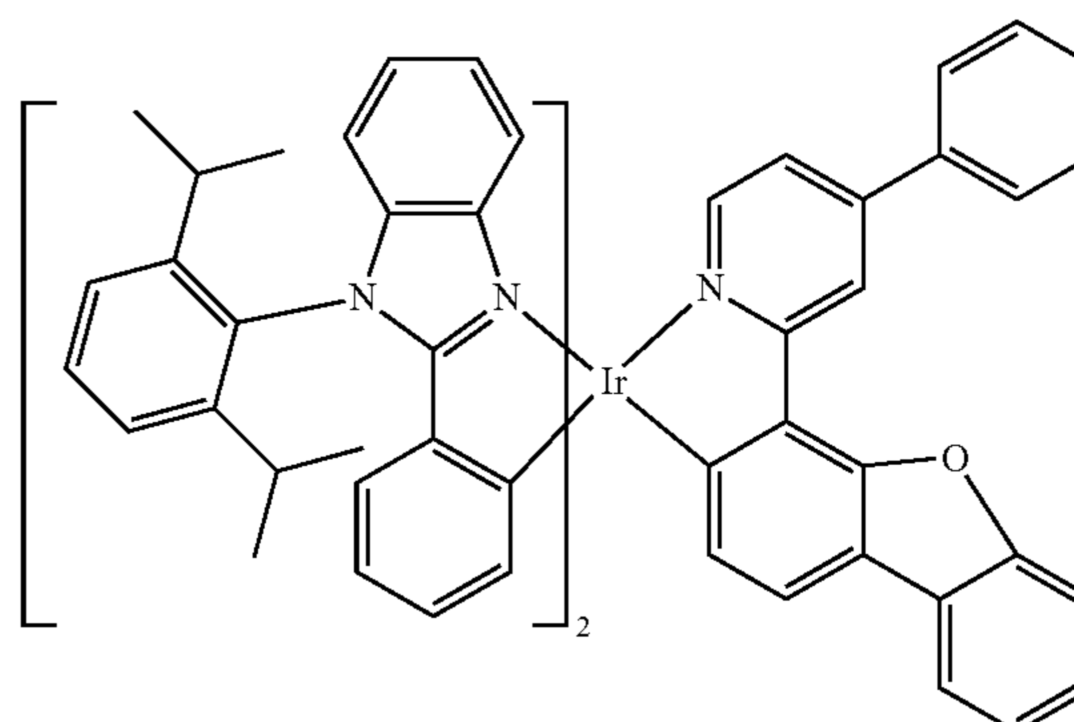
Compound 145
