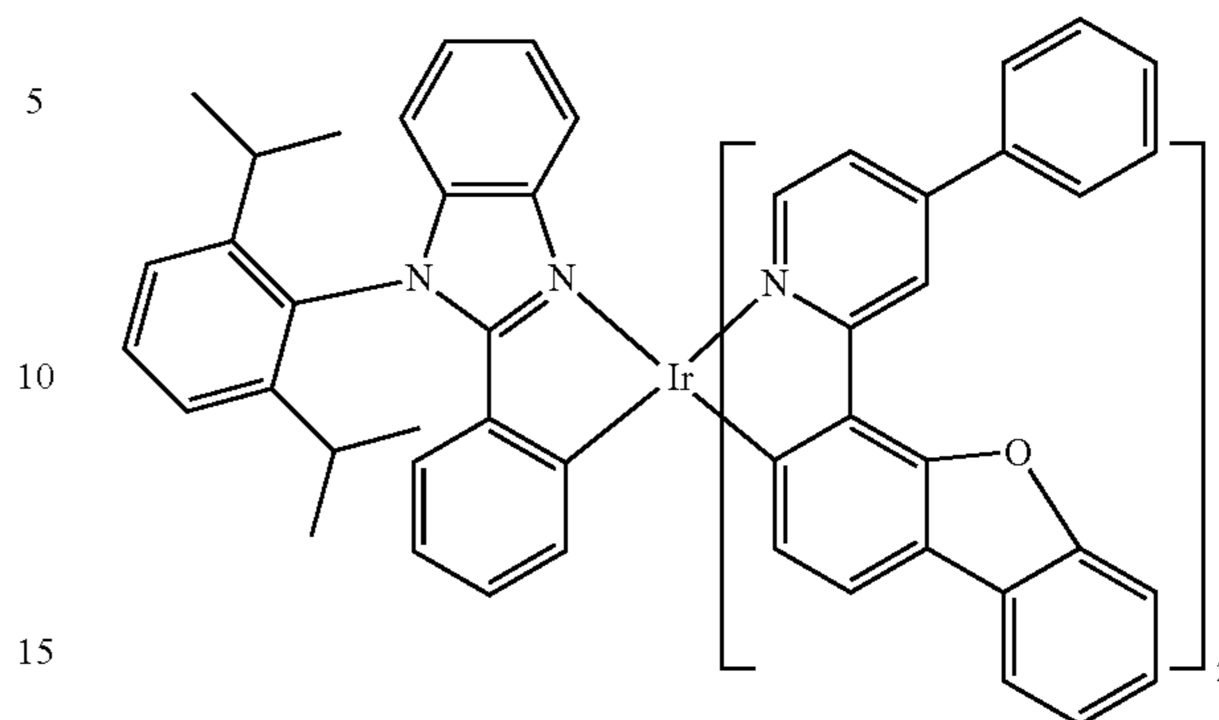
Compound 147
