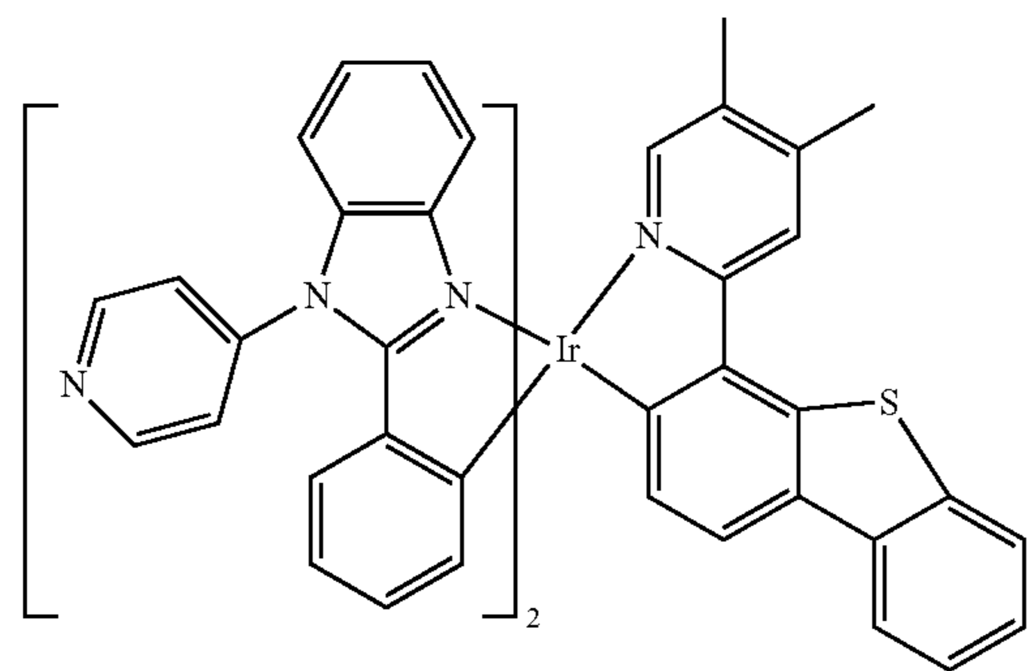
Compound 134
