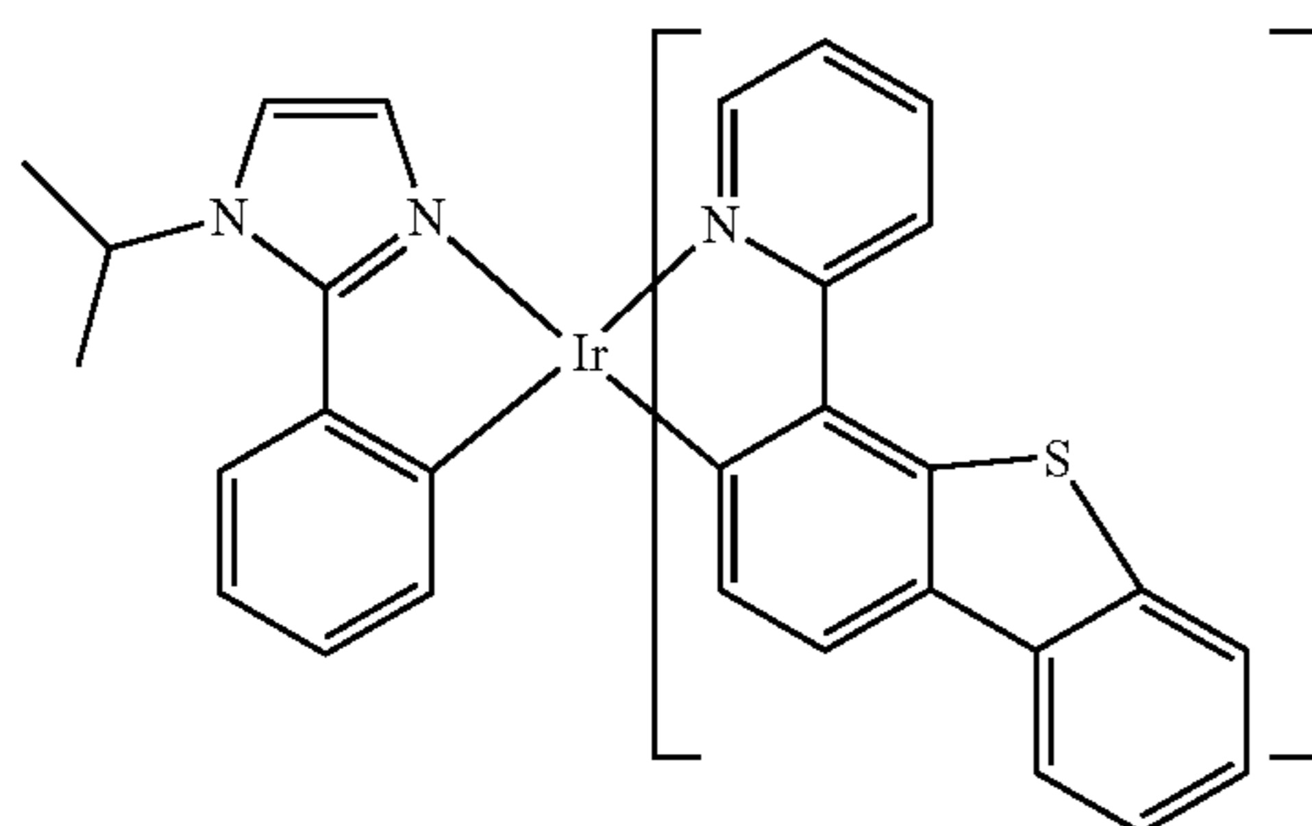
Compound 59
