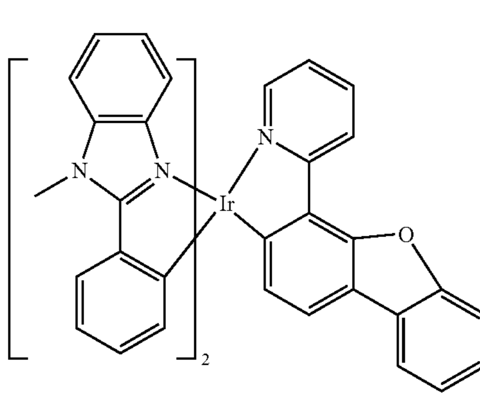
Compound 93
