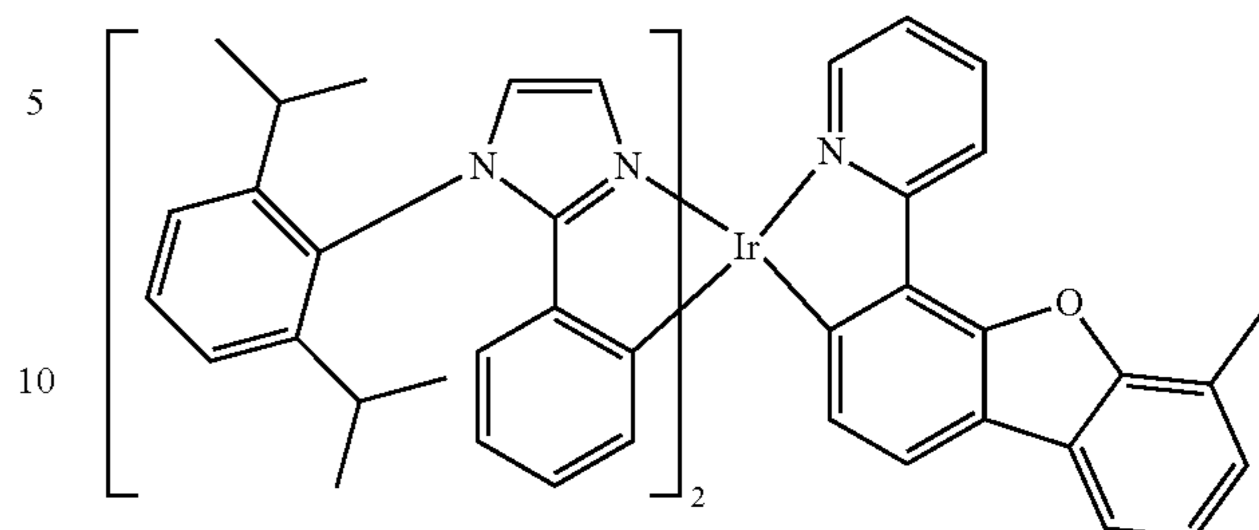
Compound 6
