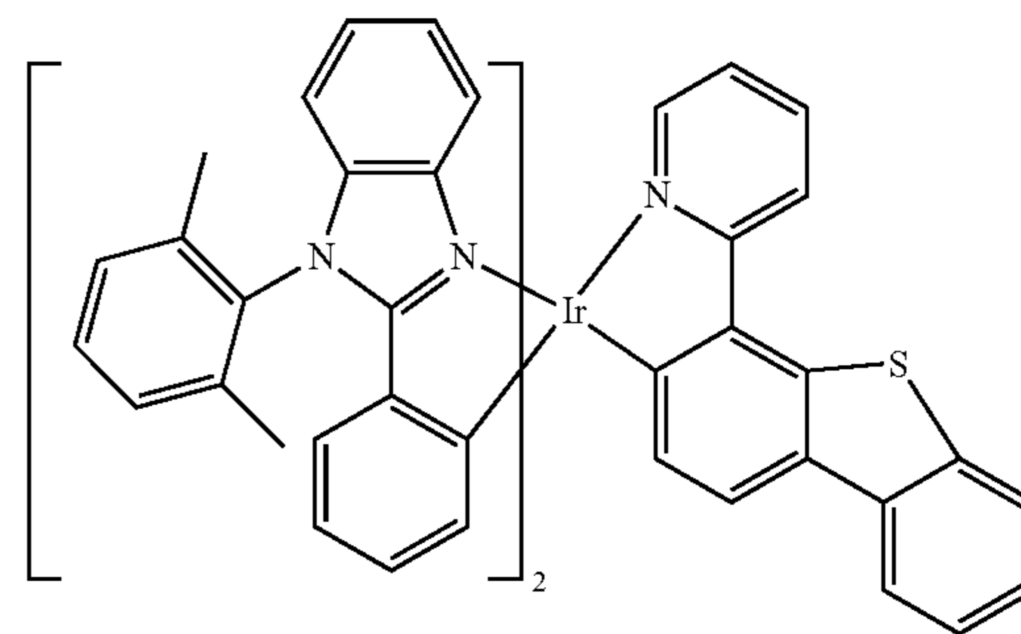
Compound 129
