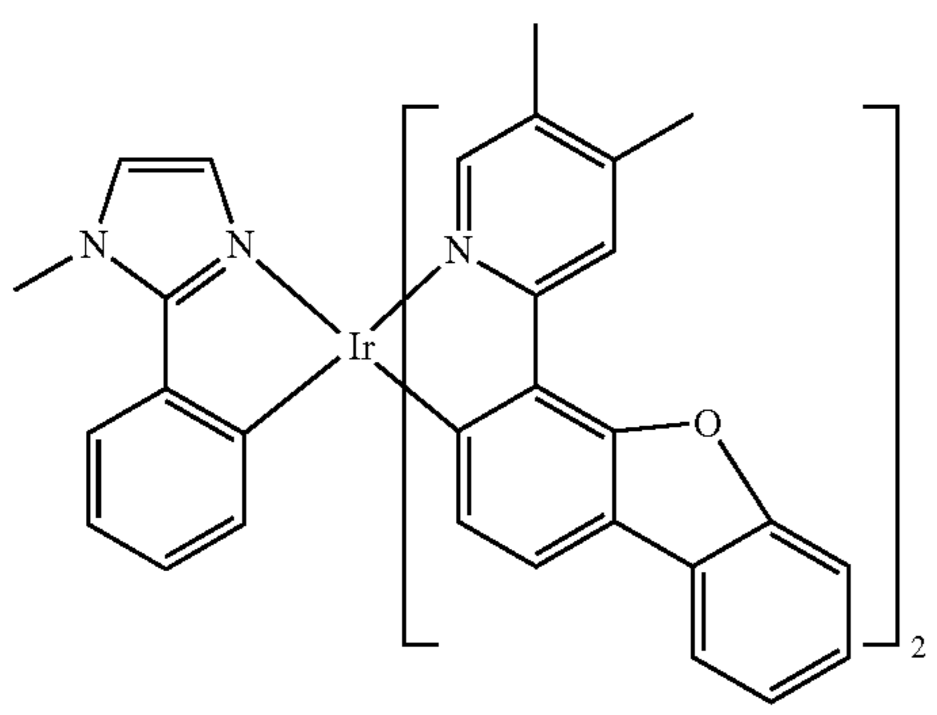
Compound 16
