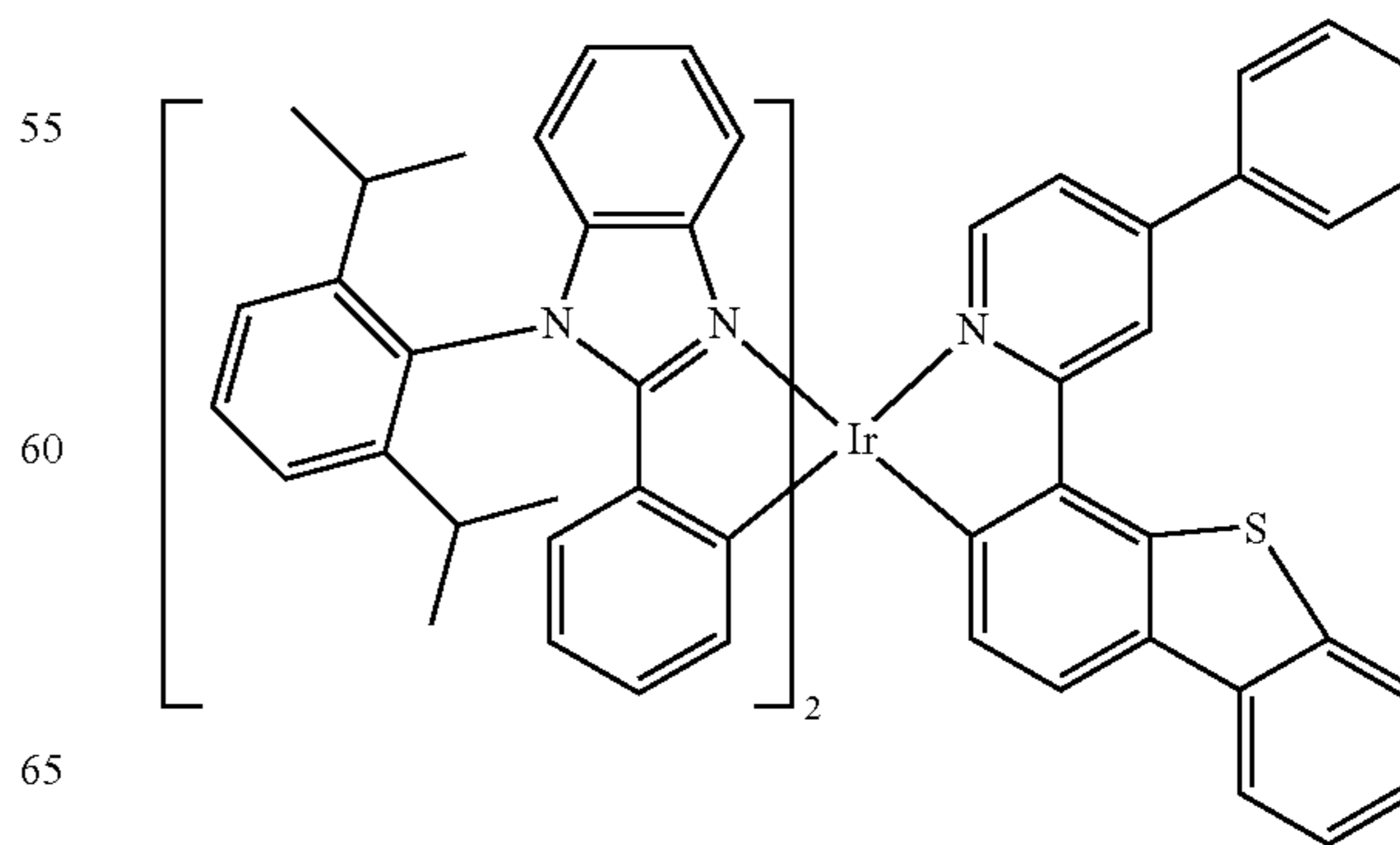
Compound 149
