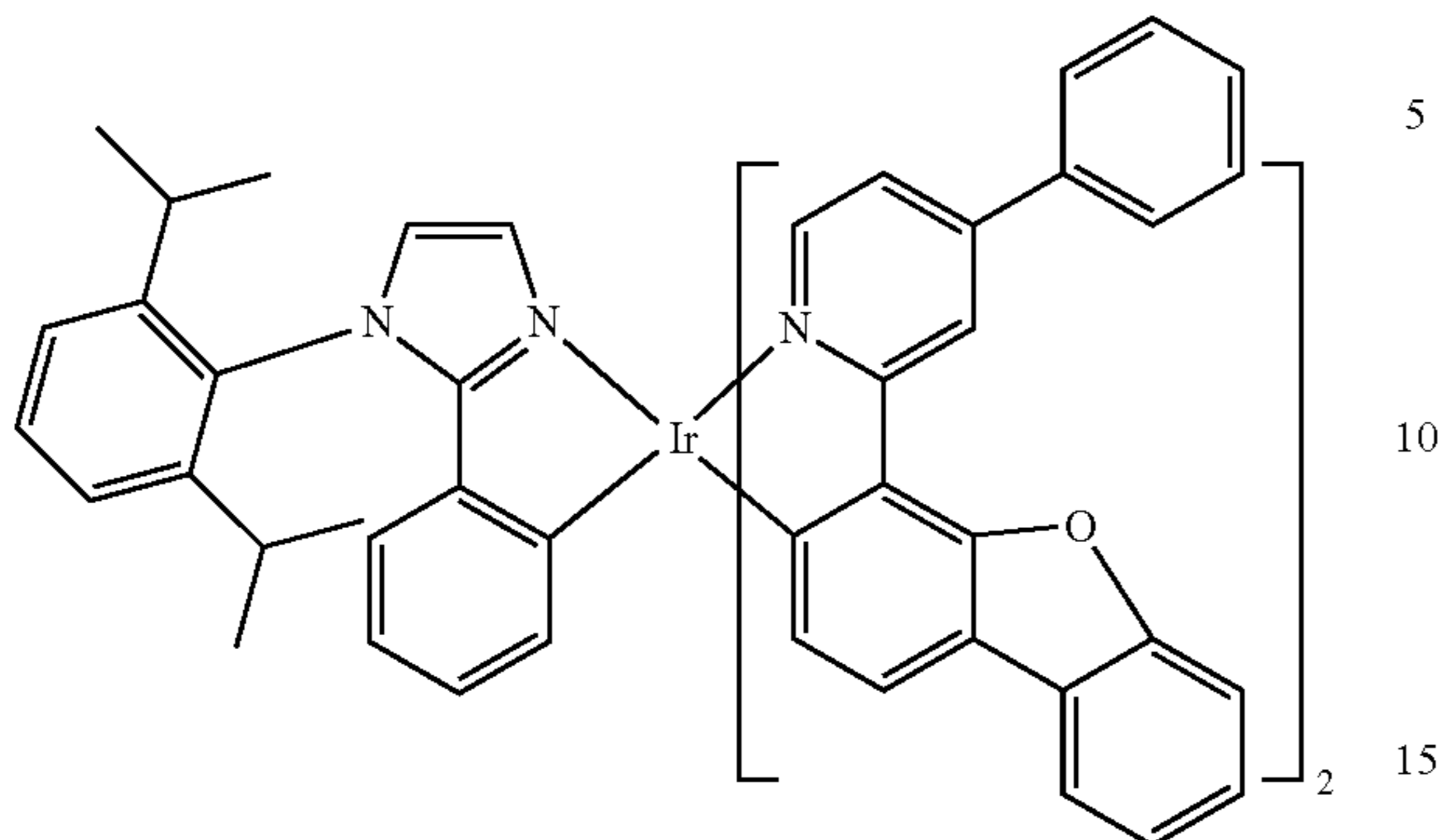
Compound 67
