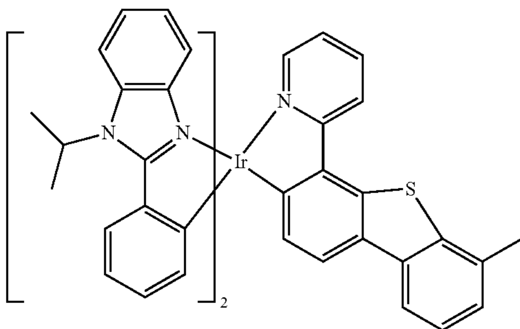
Compound 141
