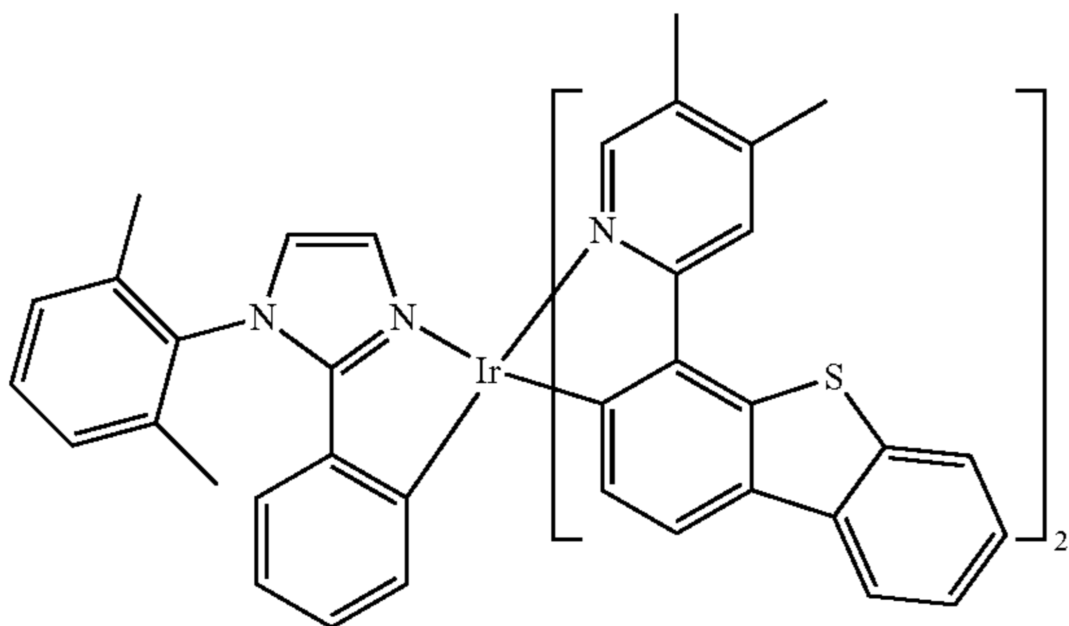
Compound 53
