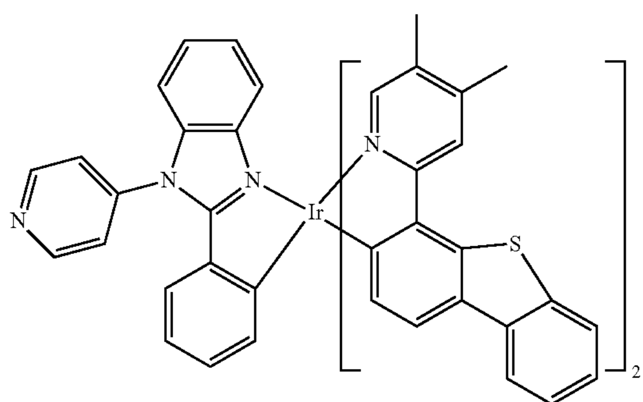
Compound 136
