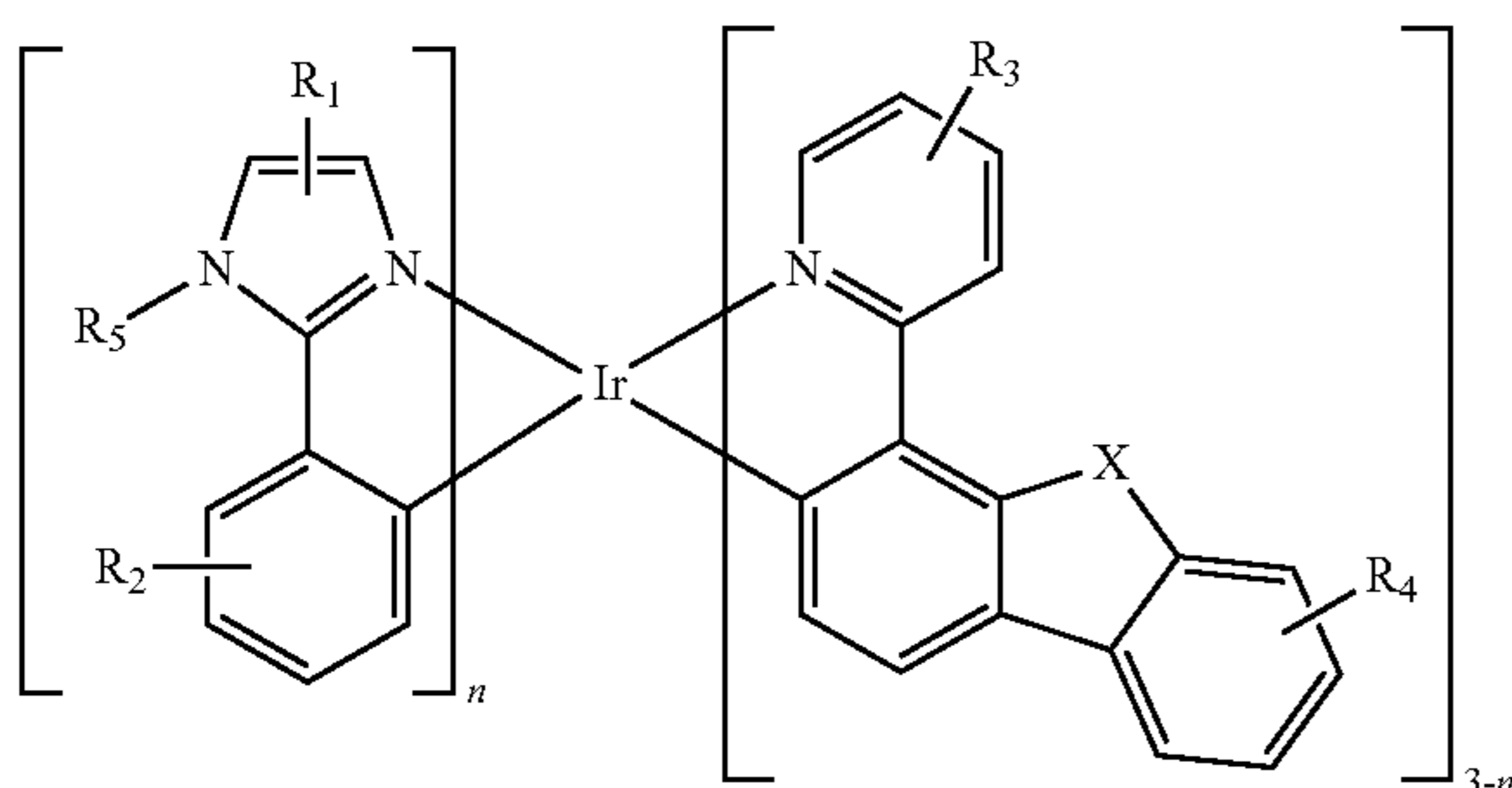
Formula I
