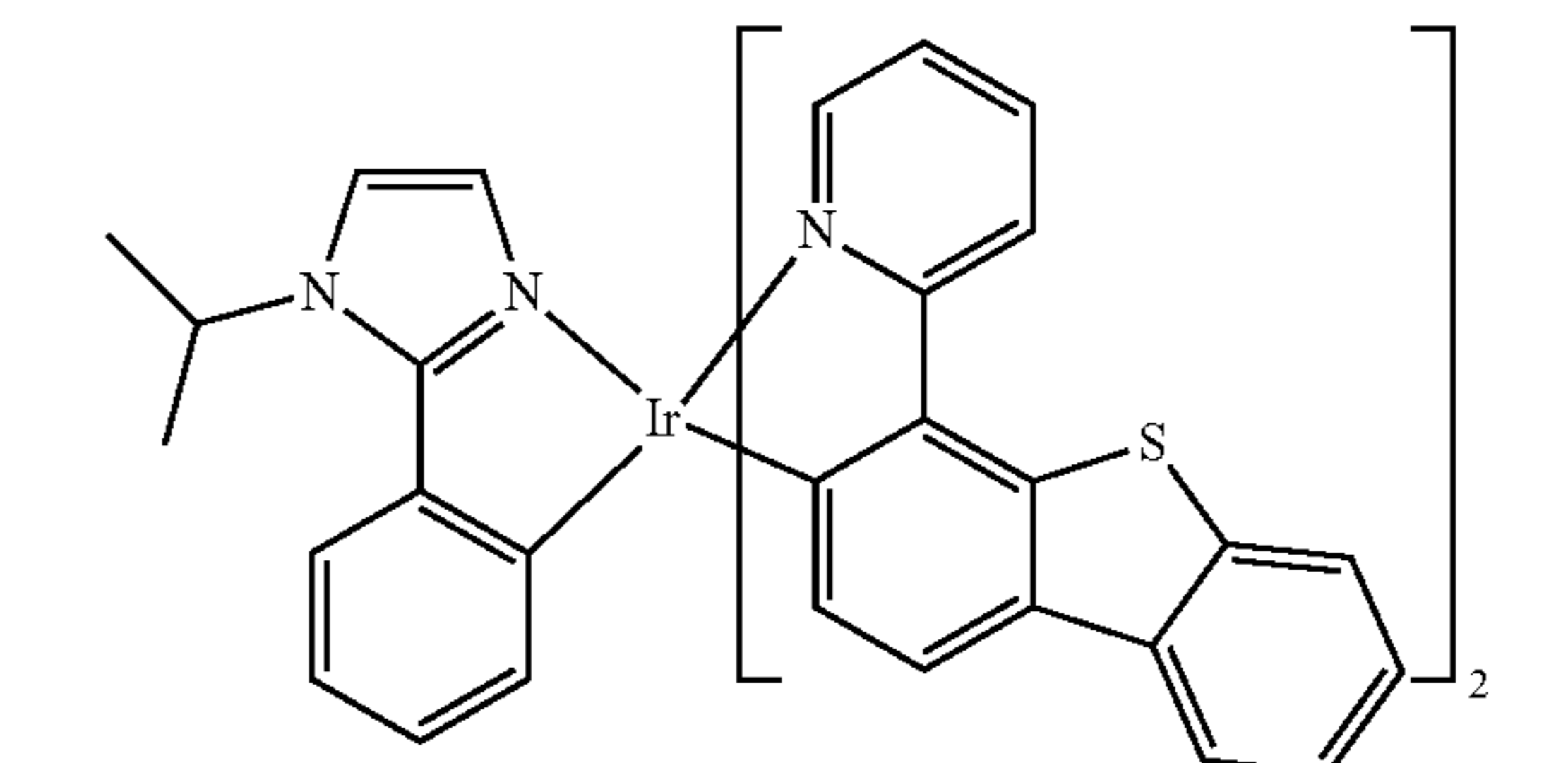
Compound 59
