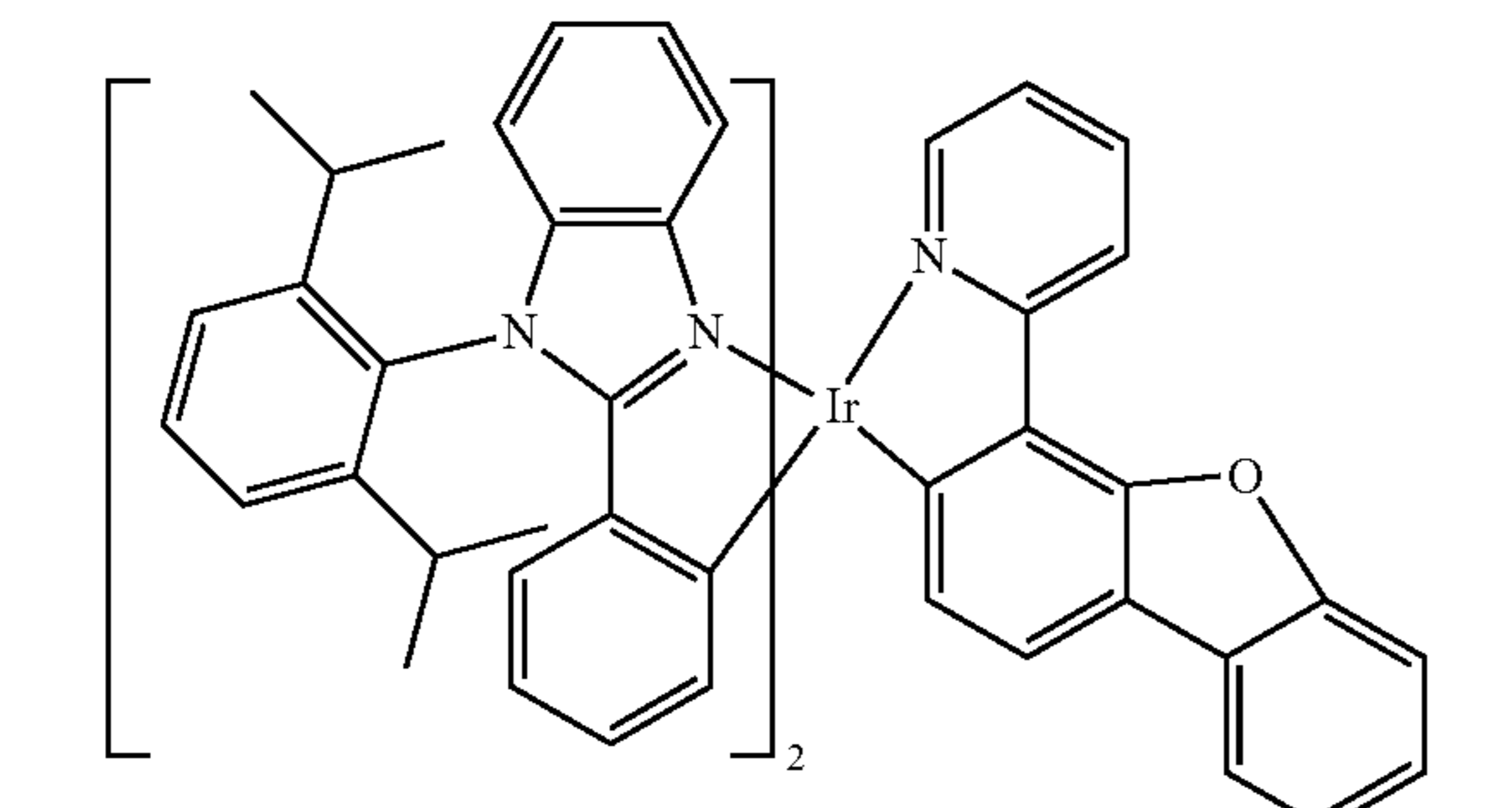
Compound 81
