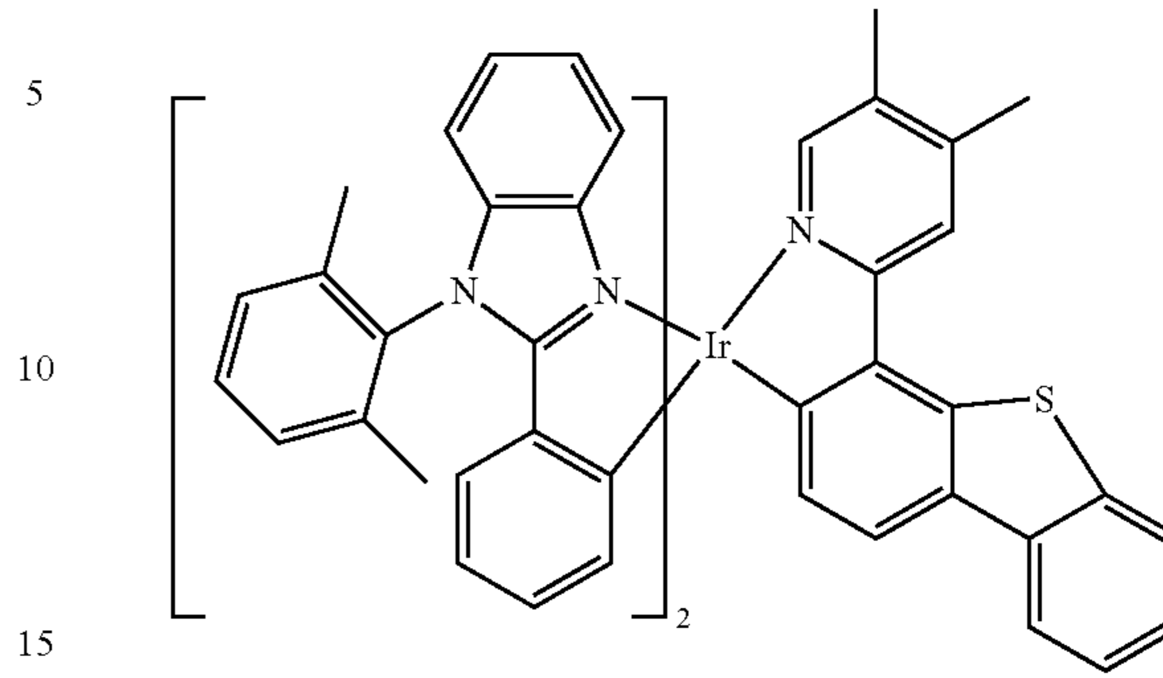
Compound 130
