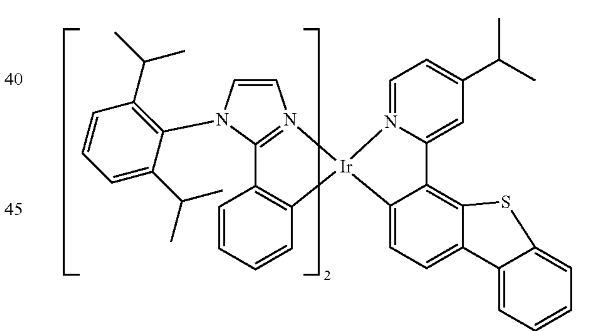
Compound 22
