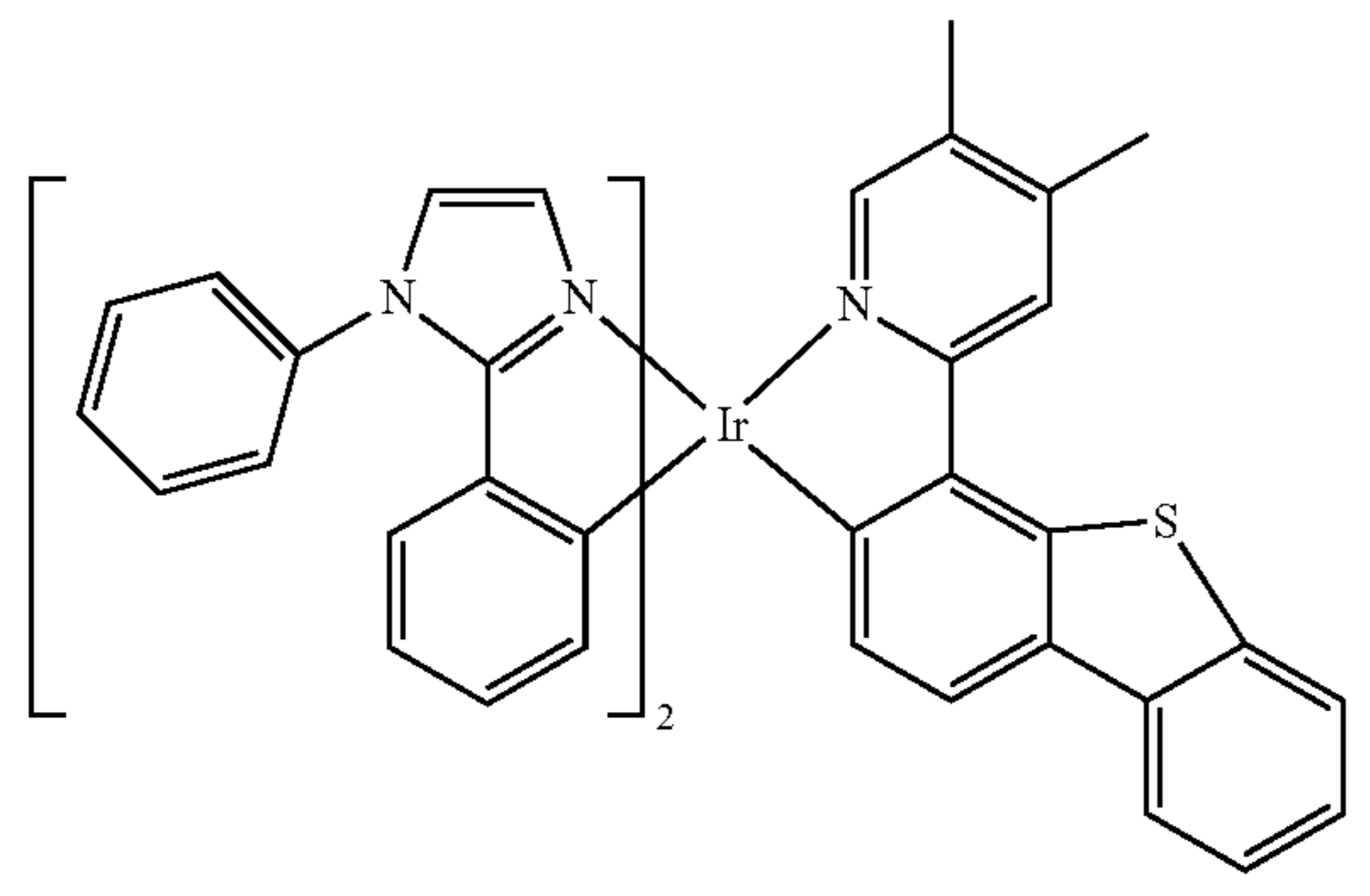
Compound 26
