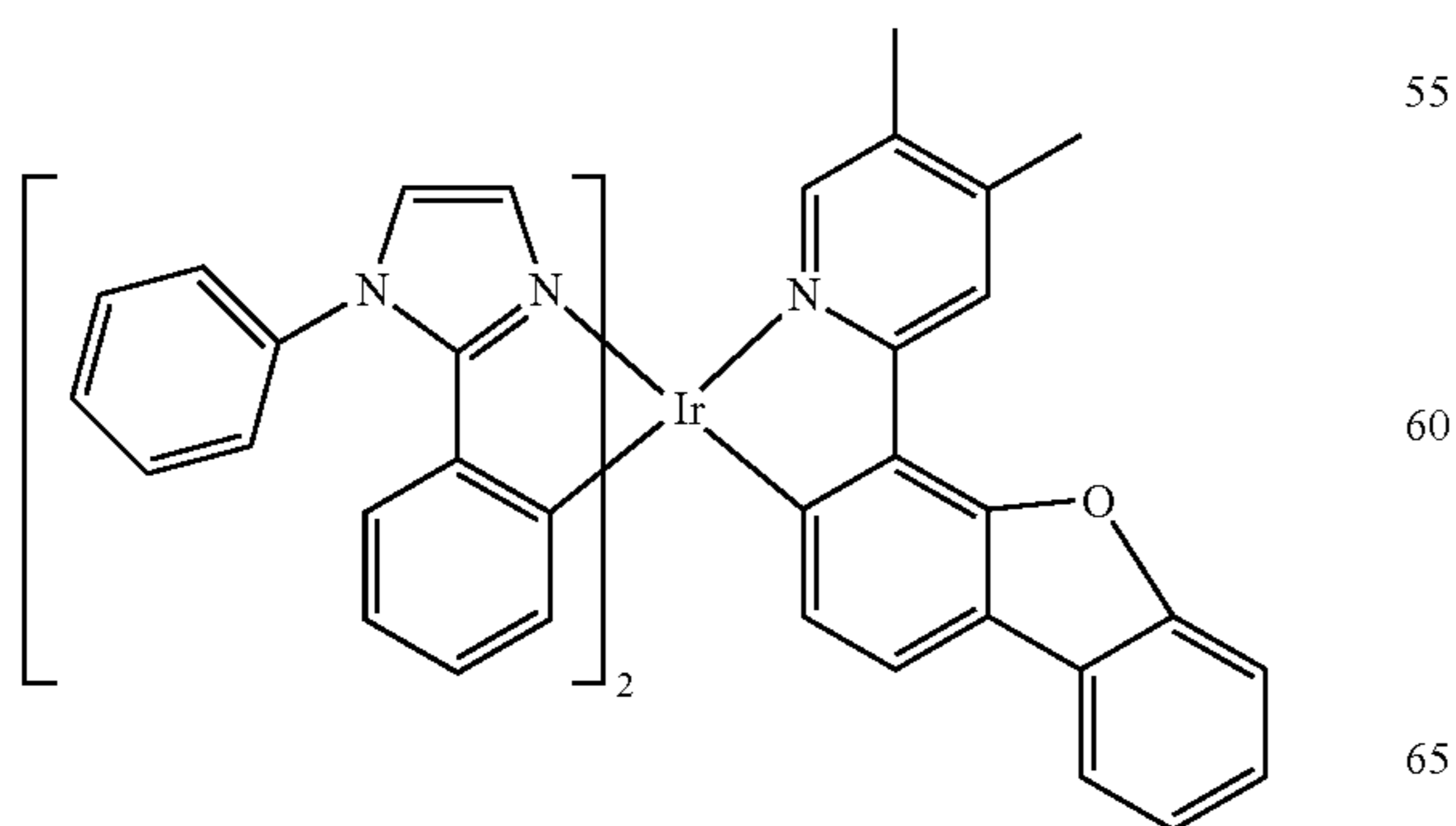
Compound 10
