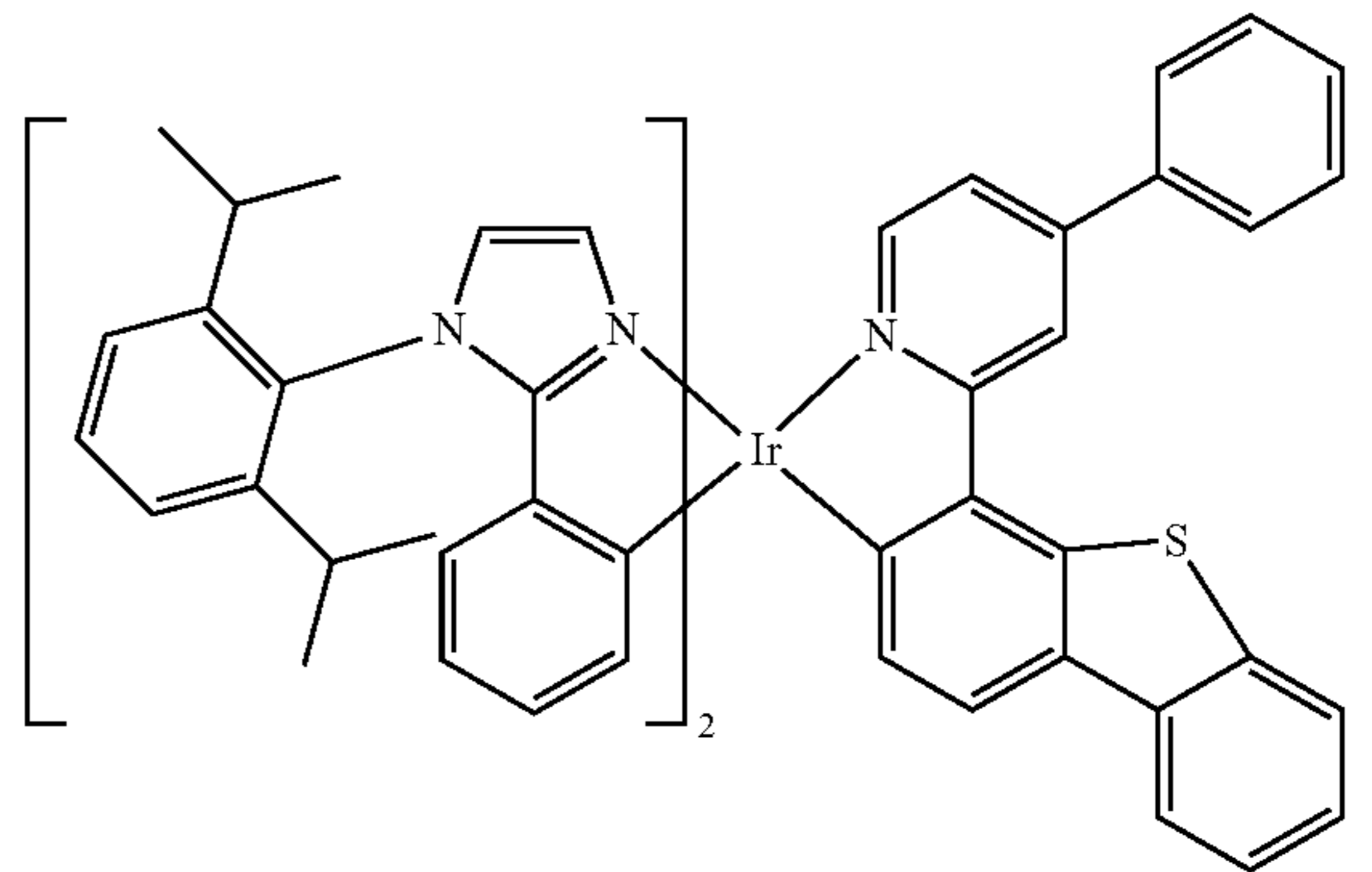
Compound 73
