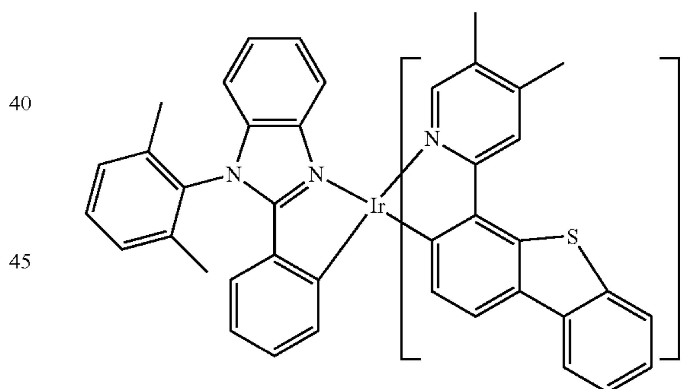
Compound 132
