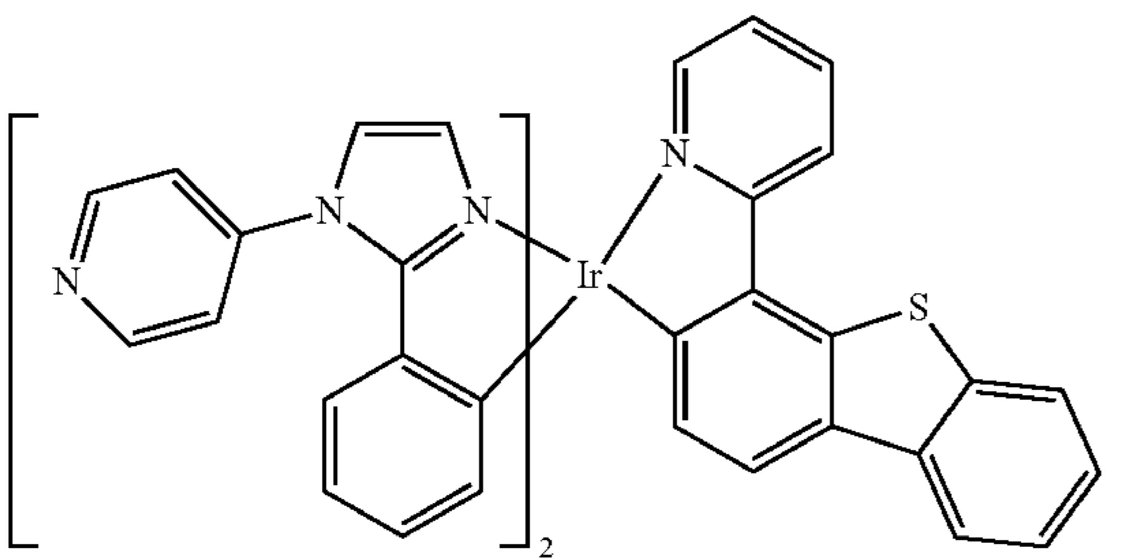
Compound 54
