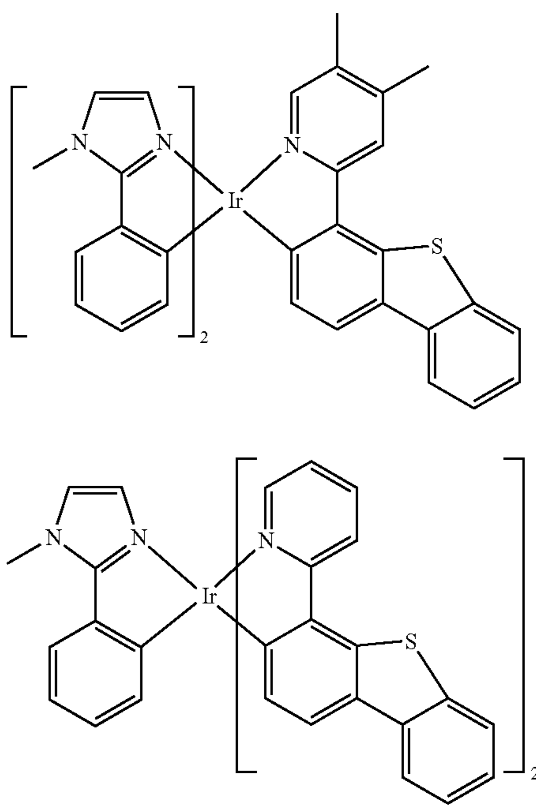
Compound 30
