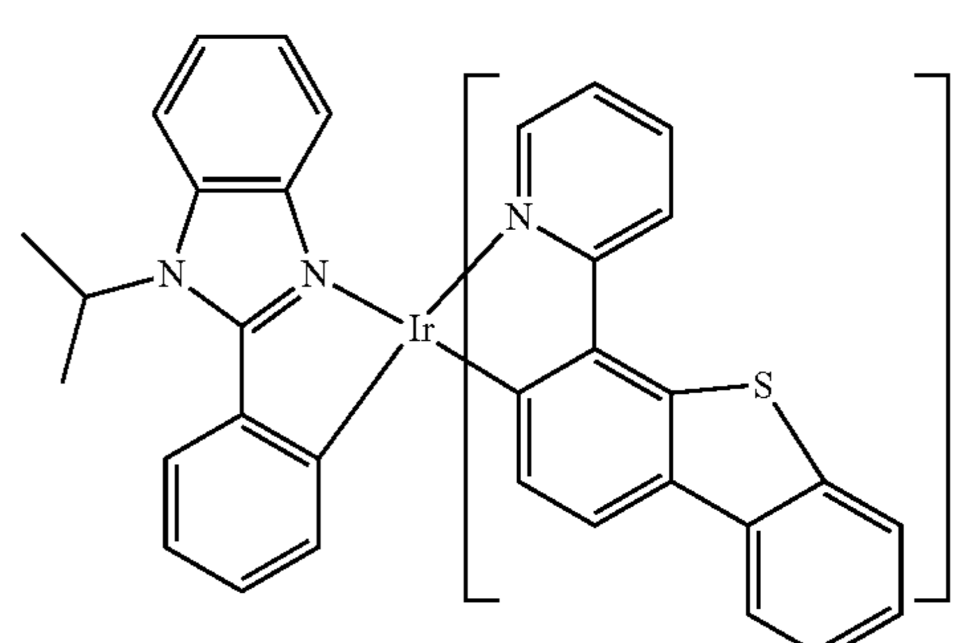
Compound 139
