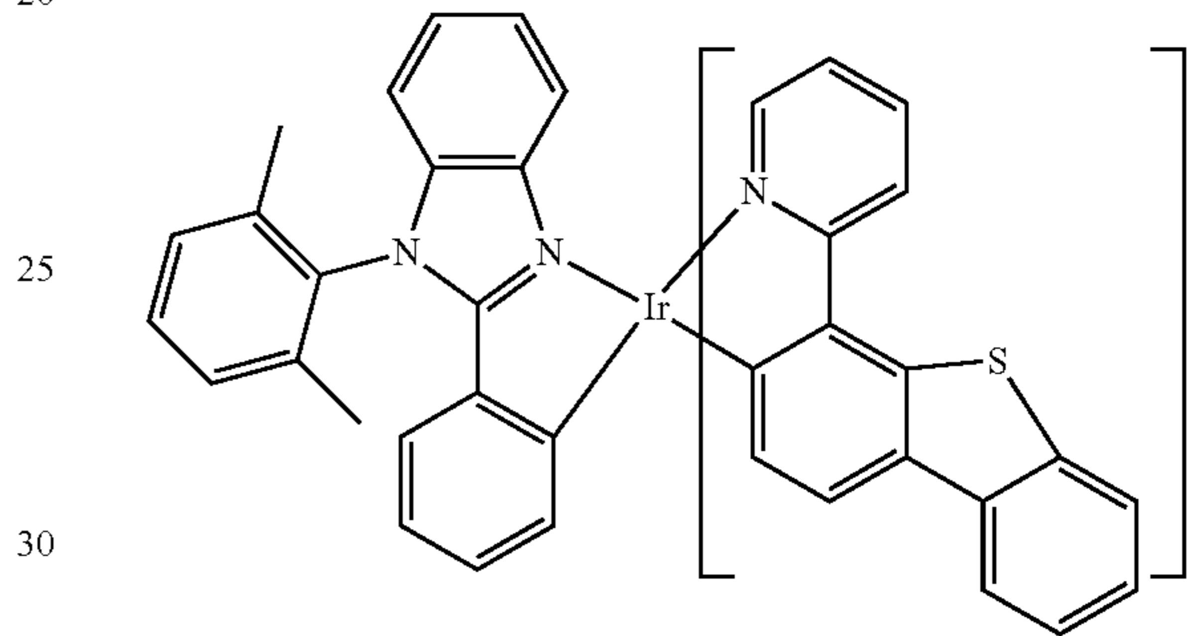
Compound 131
