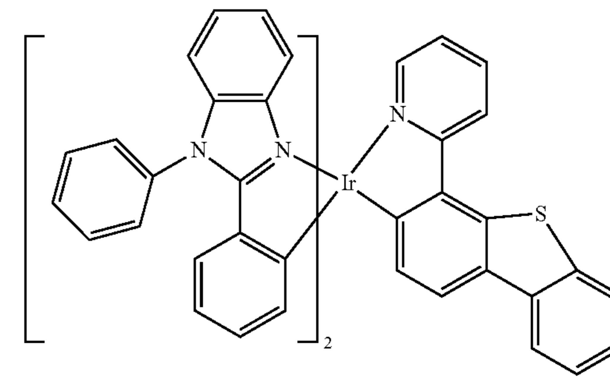
Compound 105
