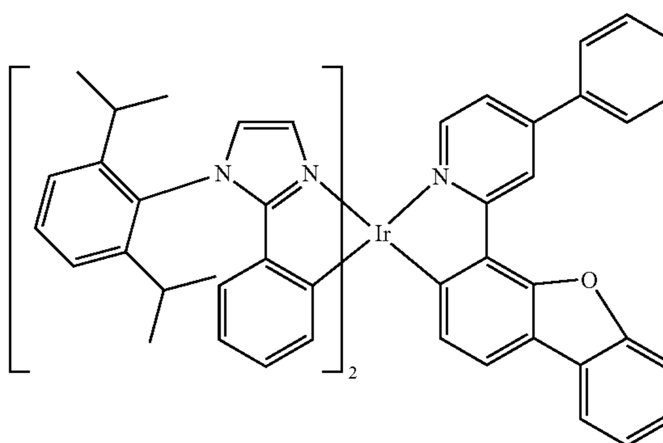
Compound 65
