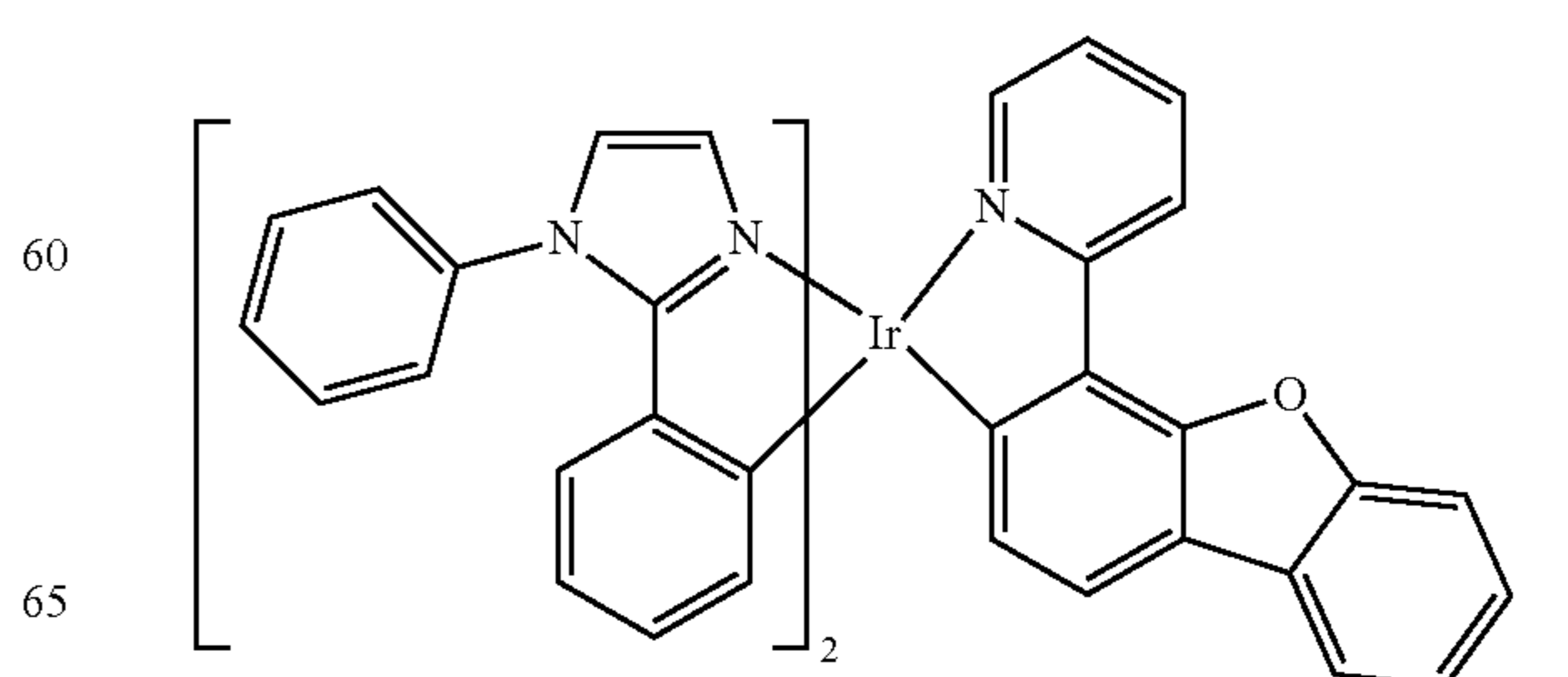
Compound 9
