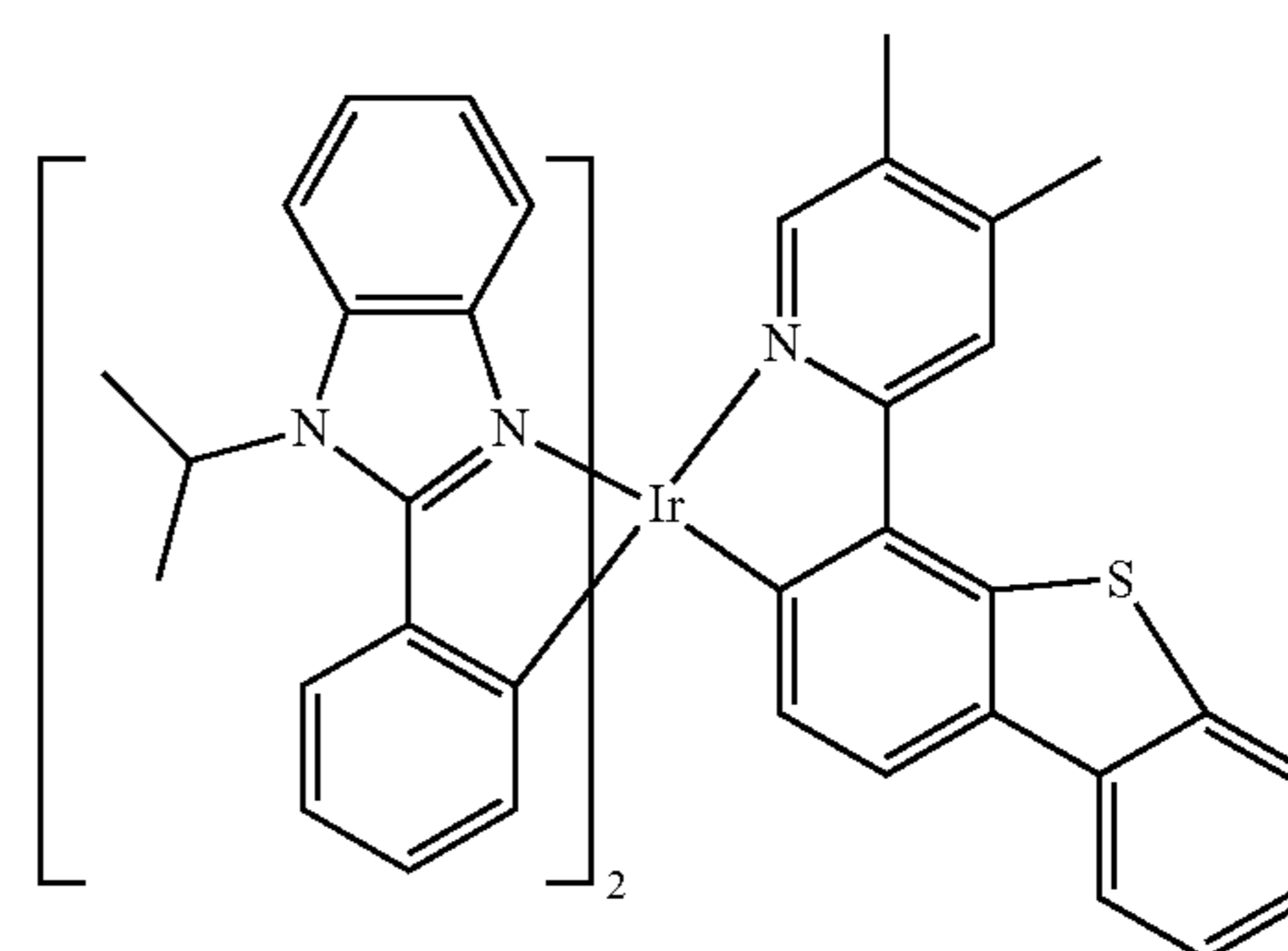
Compound 138
