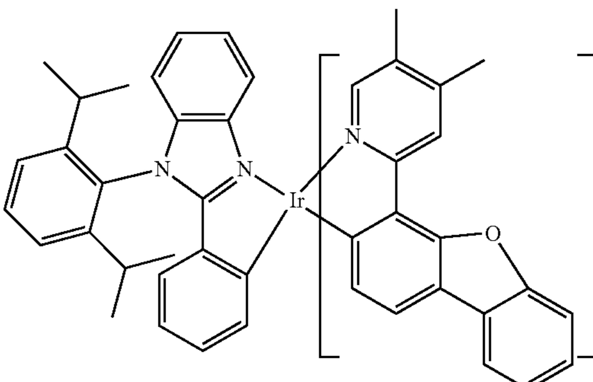
Compound 84
