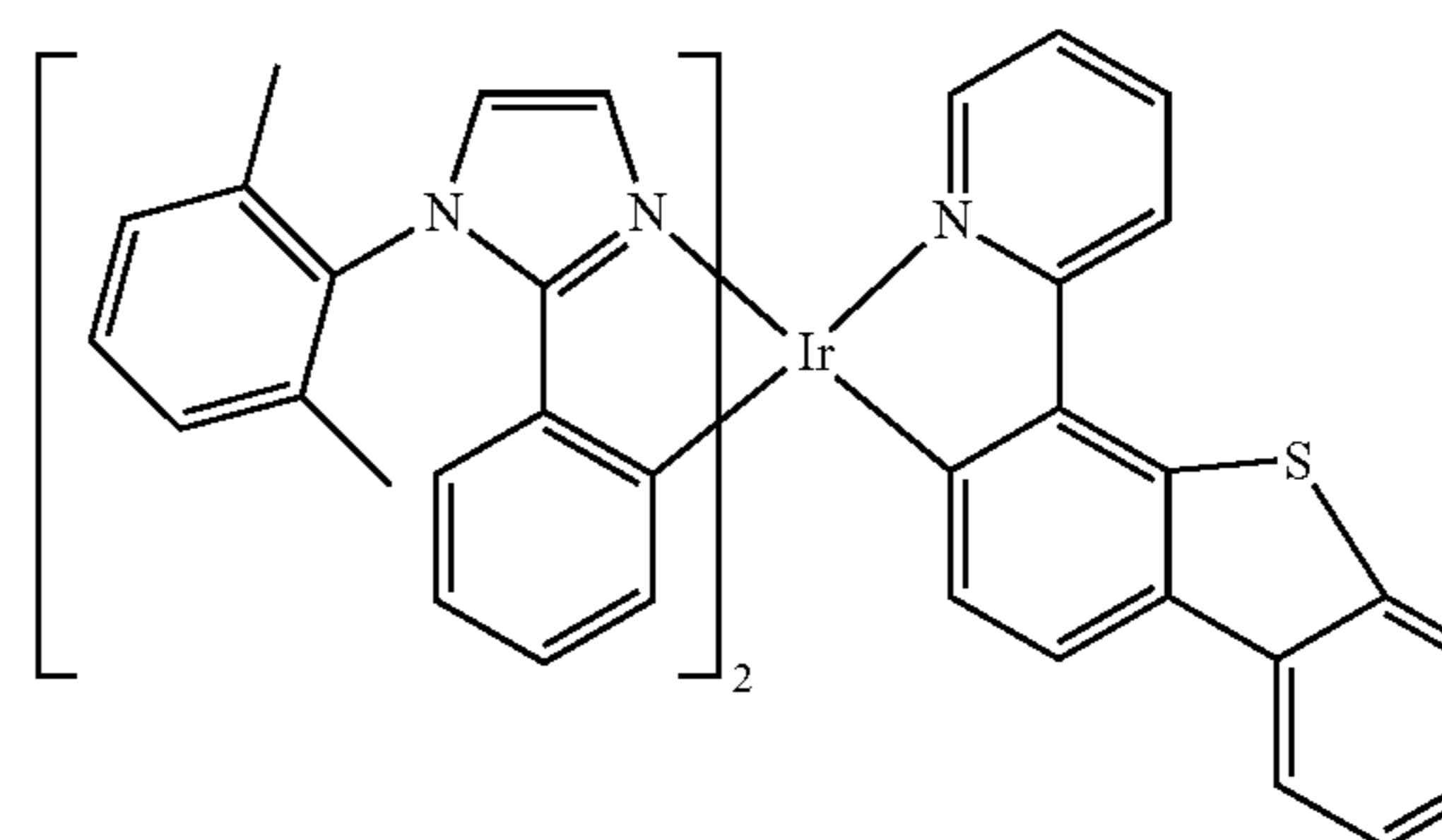
Compound 49
