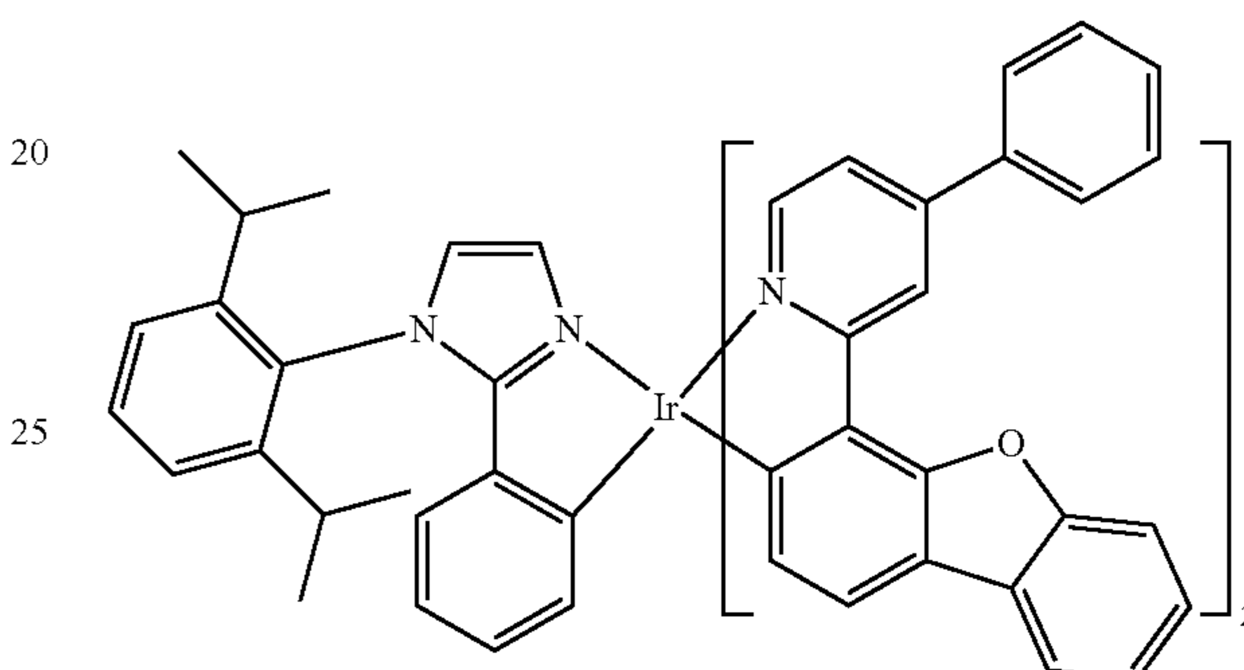
Compound 66
