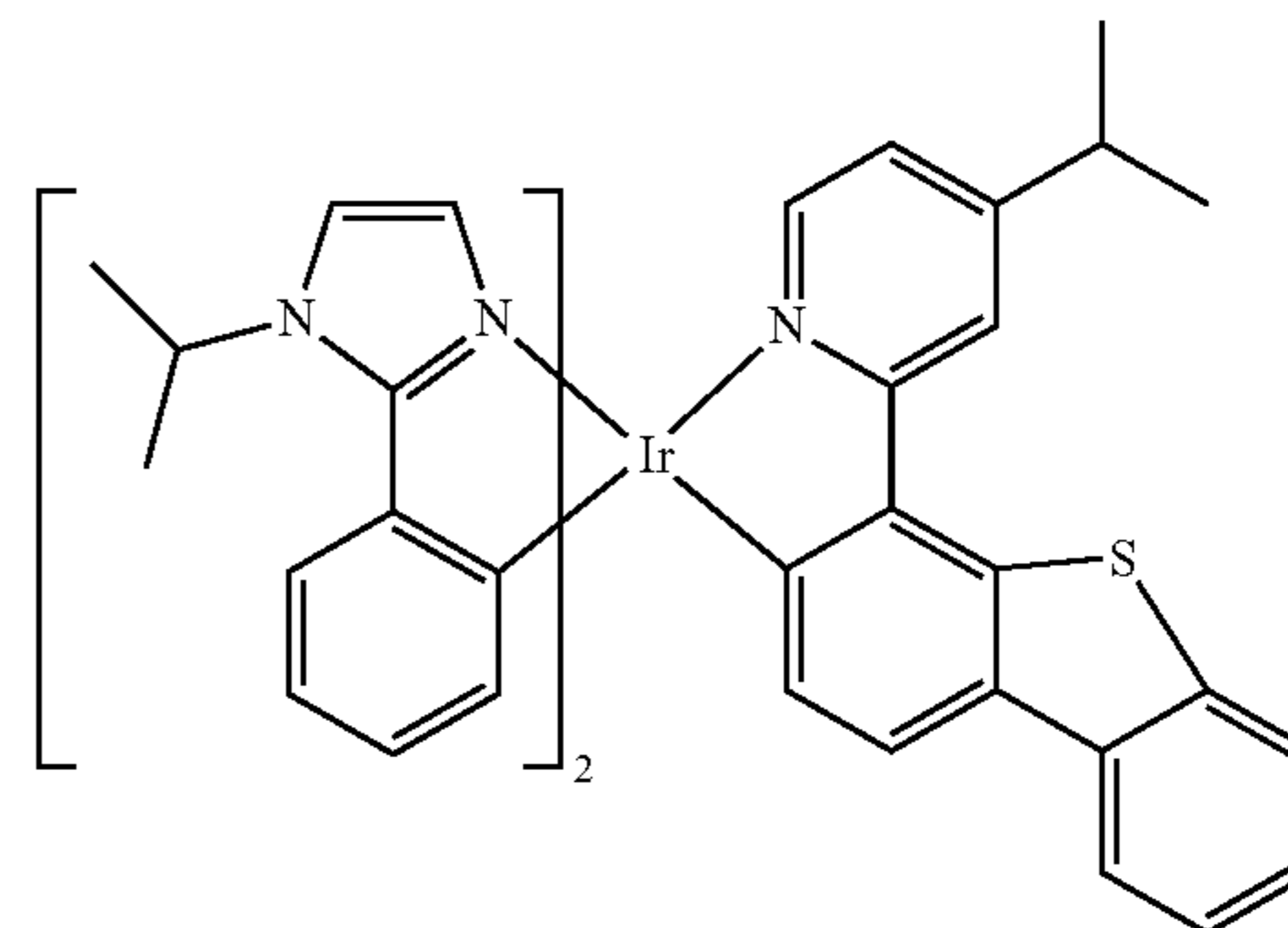
Compound 62
