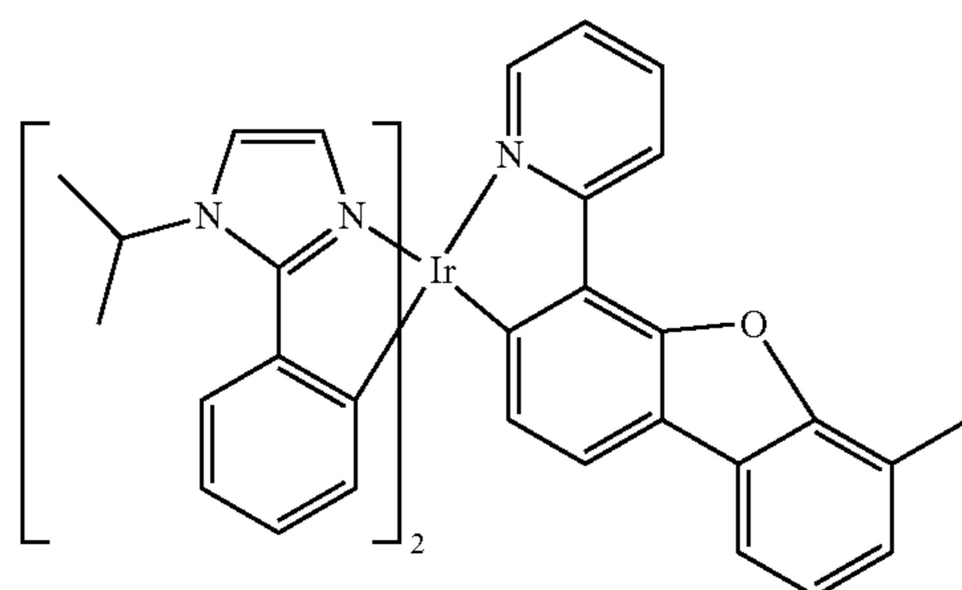
Compound 45
