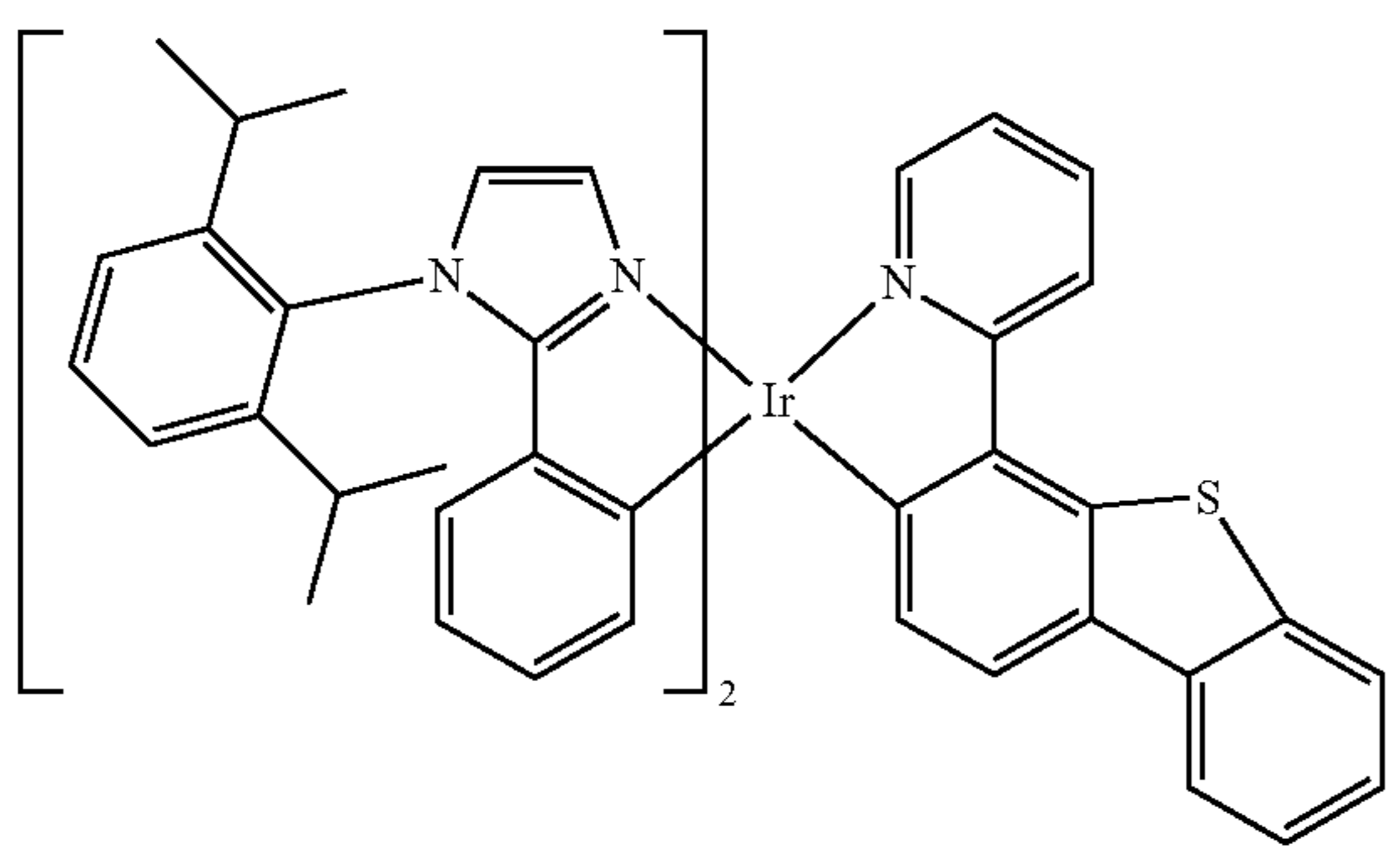
Compound 17
