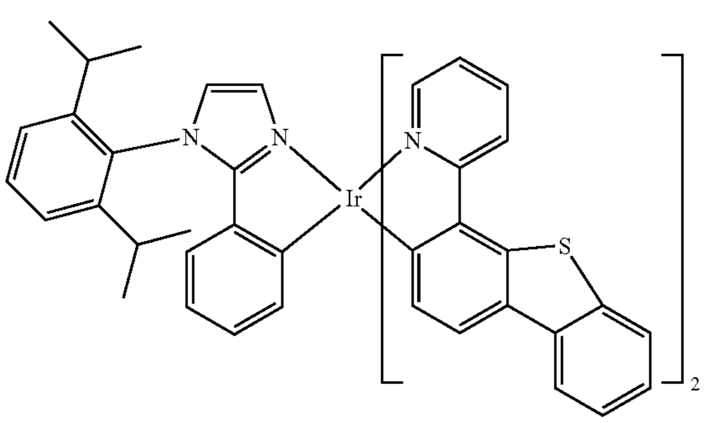
Compound 19
