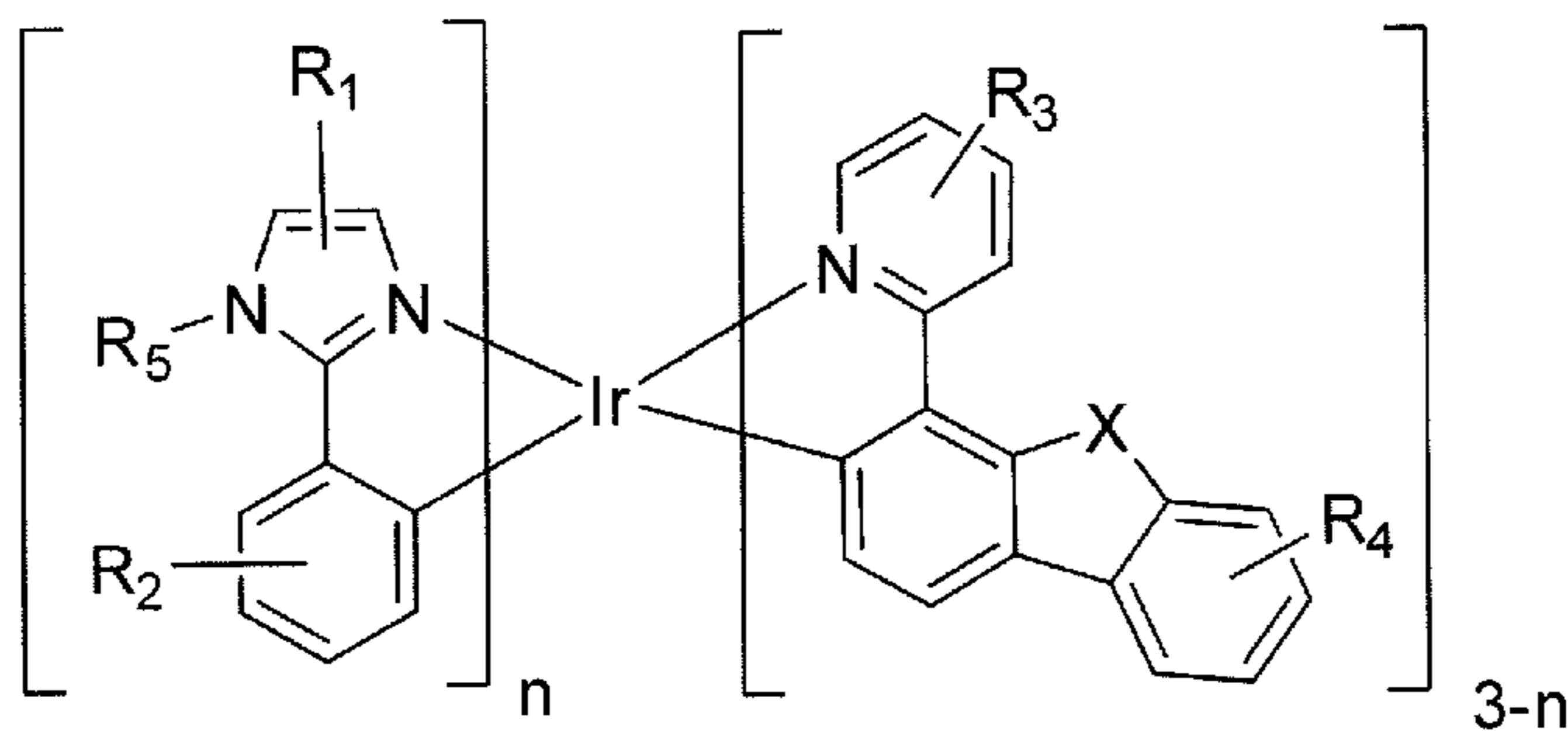
Formula I
