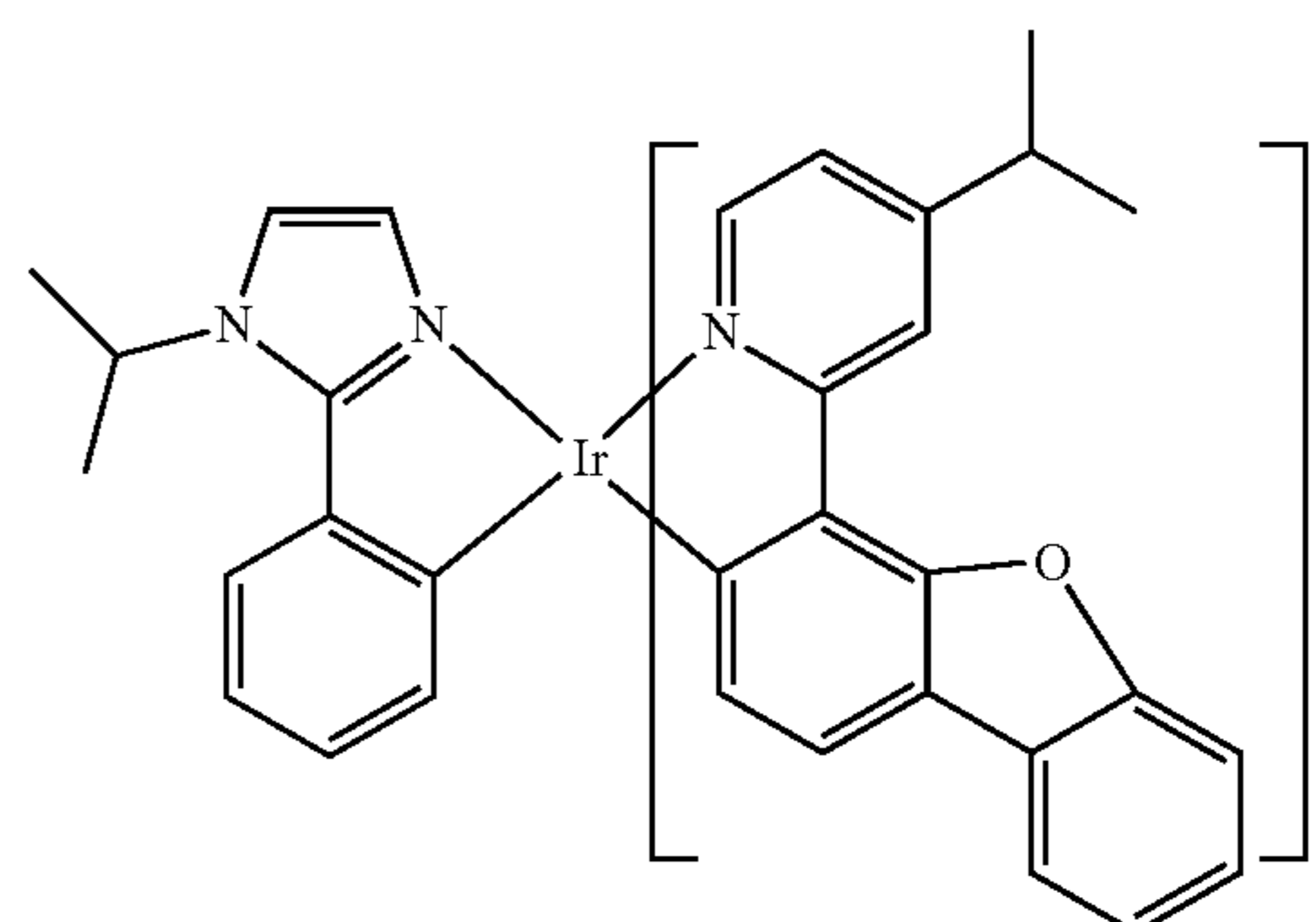
Compound 48
