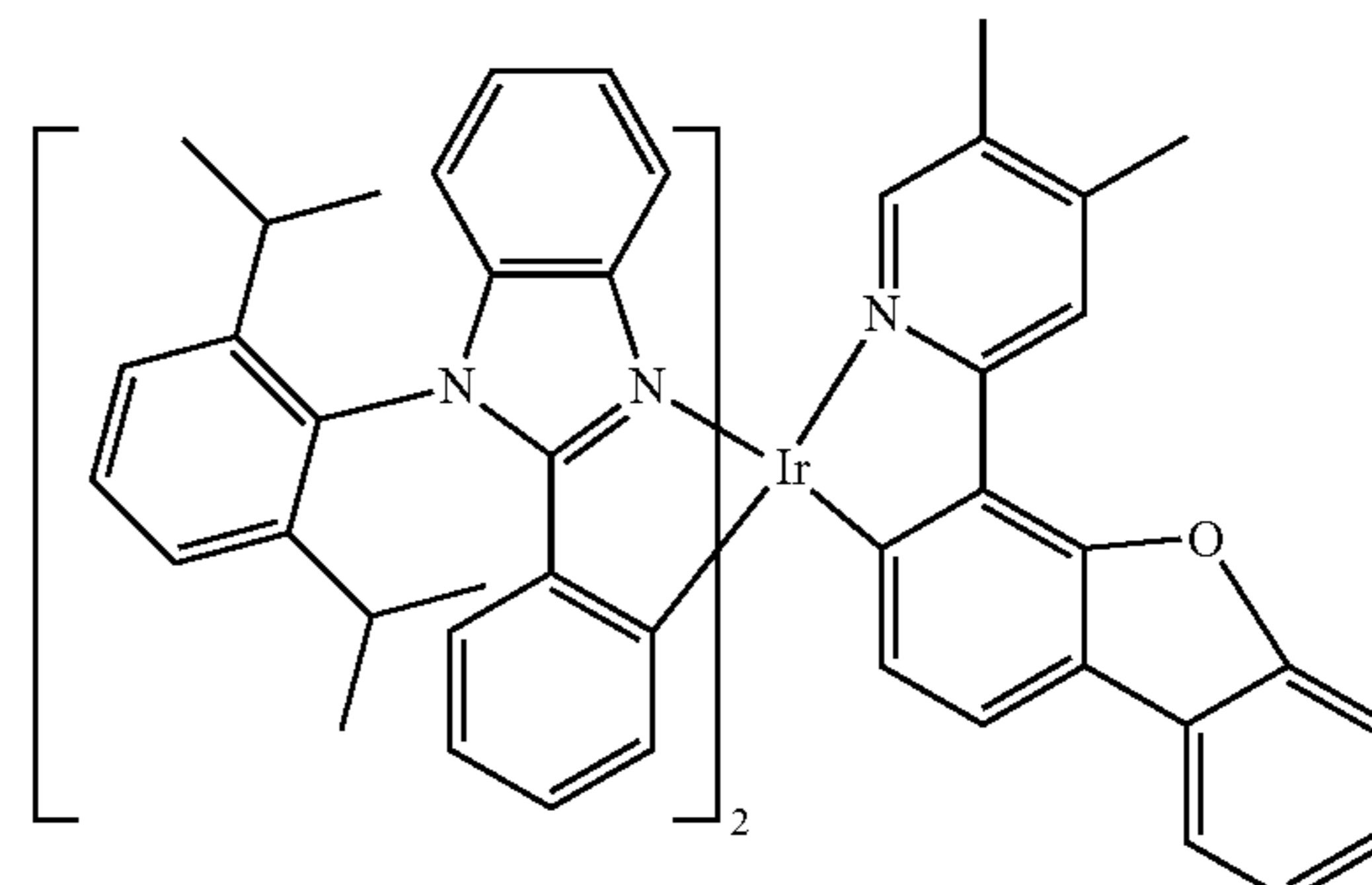
Compound 82
