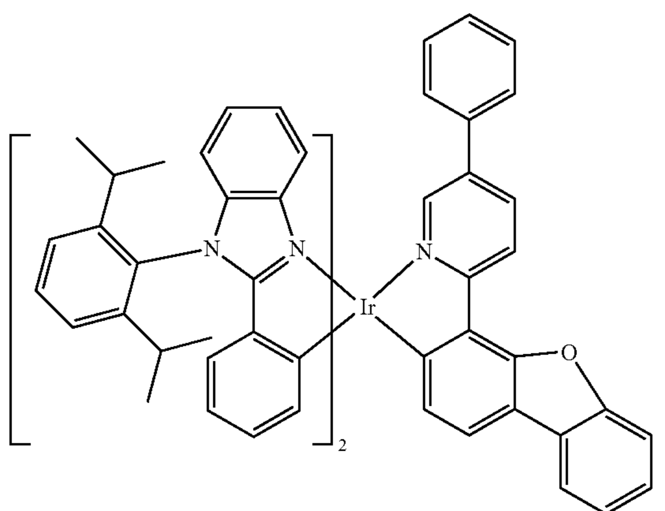
Compound 148
