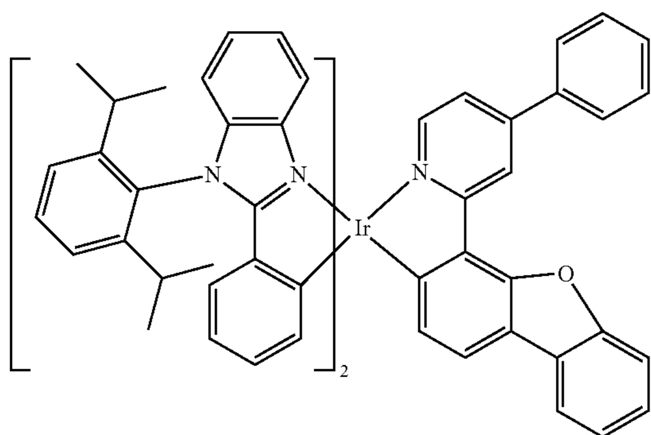
Compound 145
