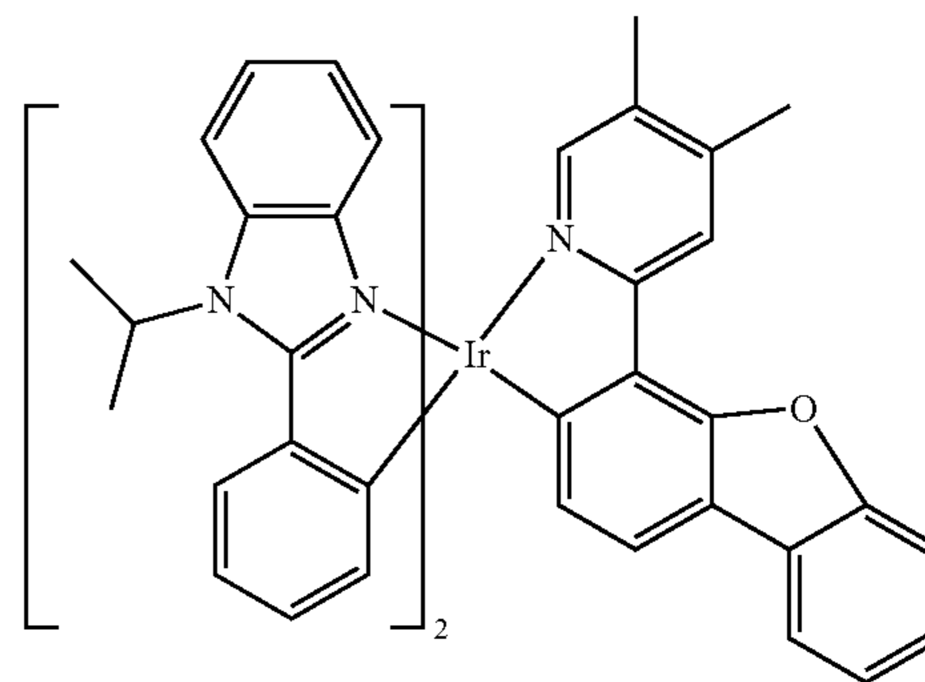
Compound 122
