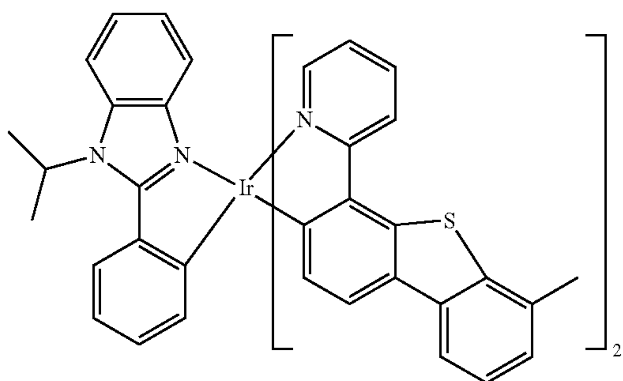
Compound 143
