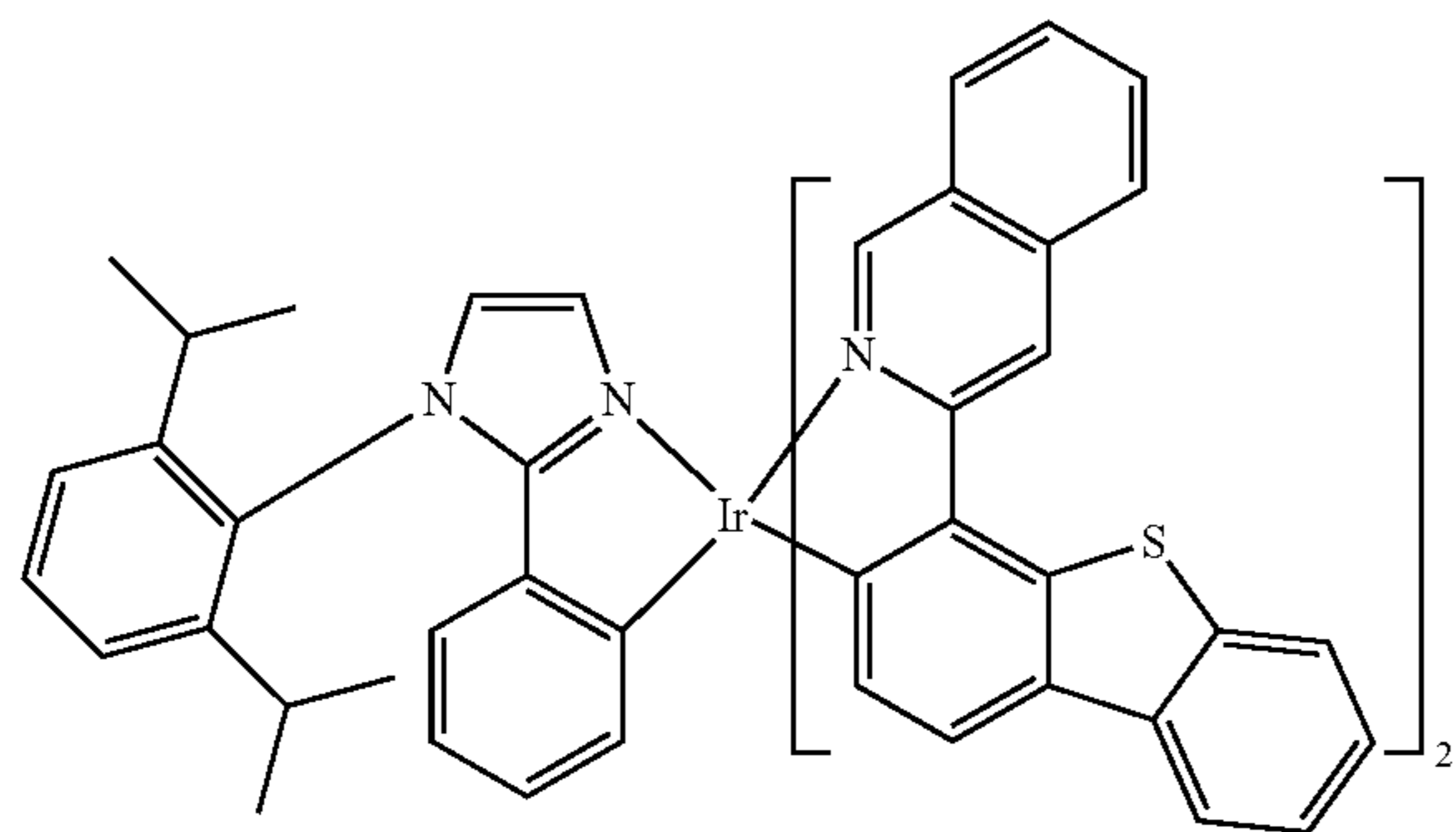
Compound 78
