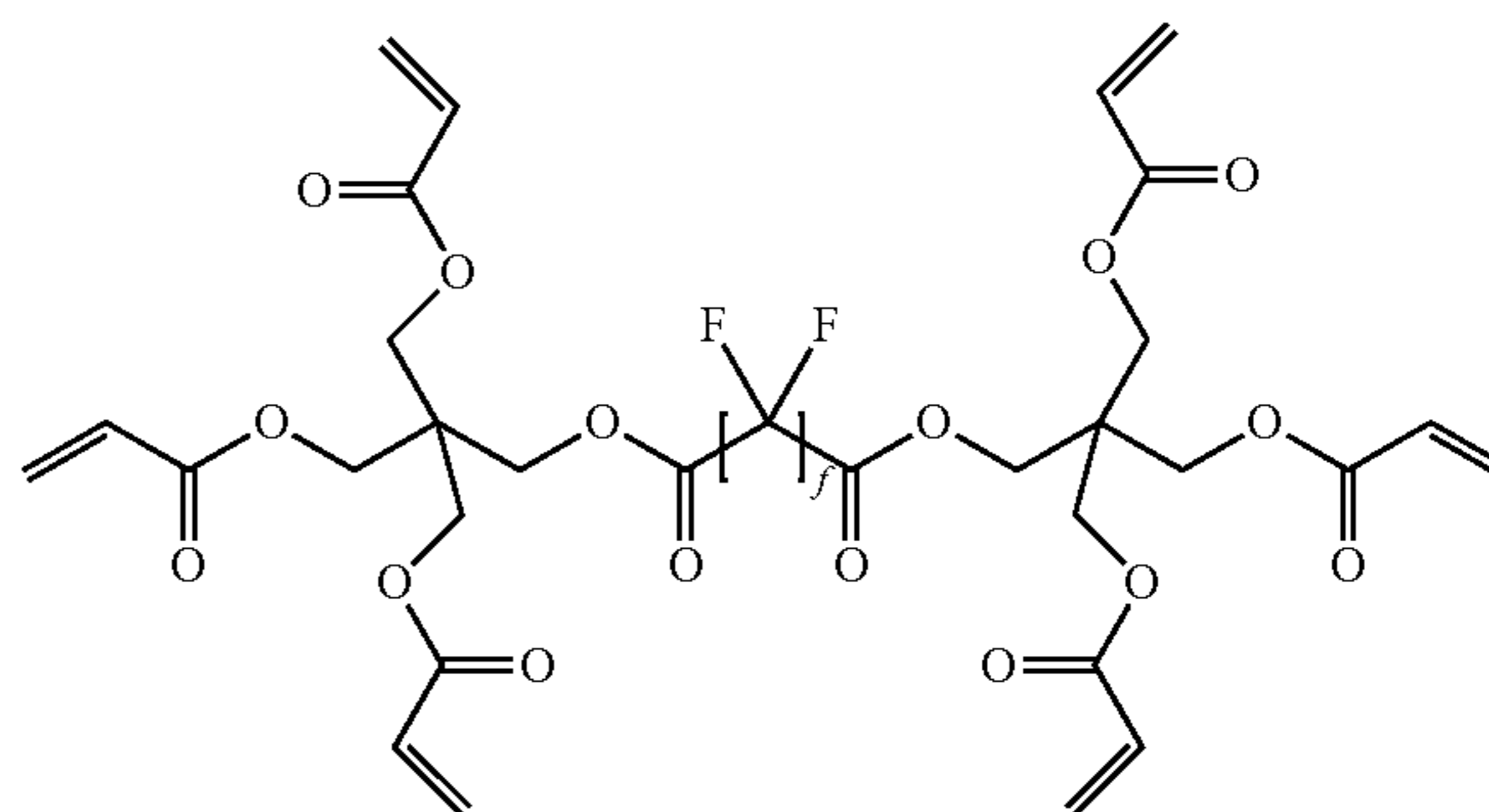
[Chemical Formula 5]
