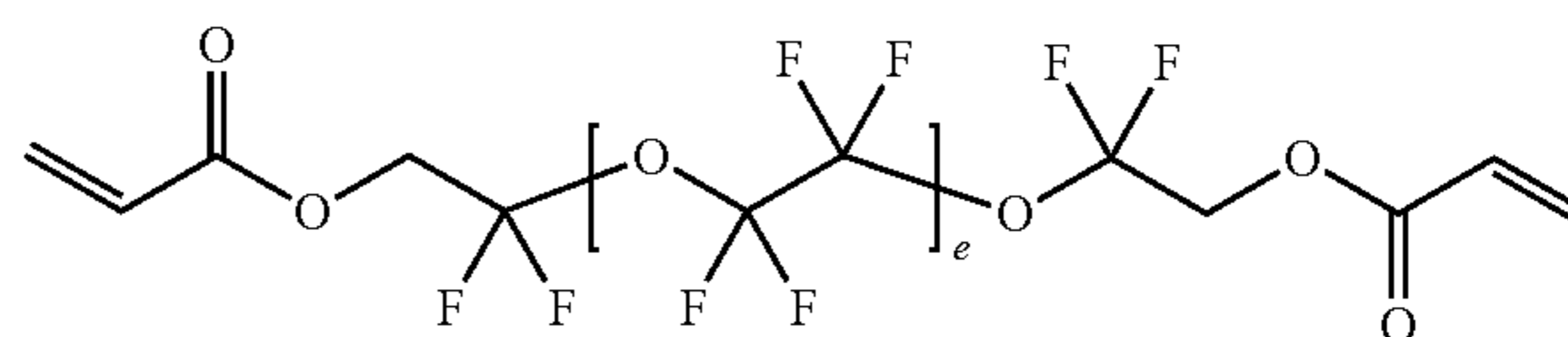
[Chemical Formula 4]
