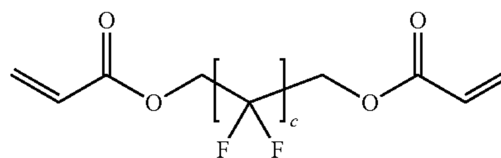
[Chemical Formula 2]
