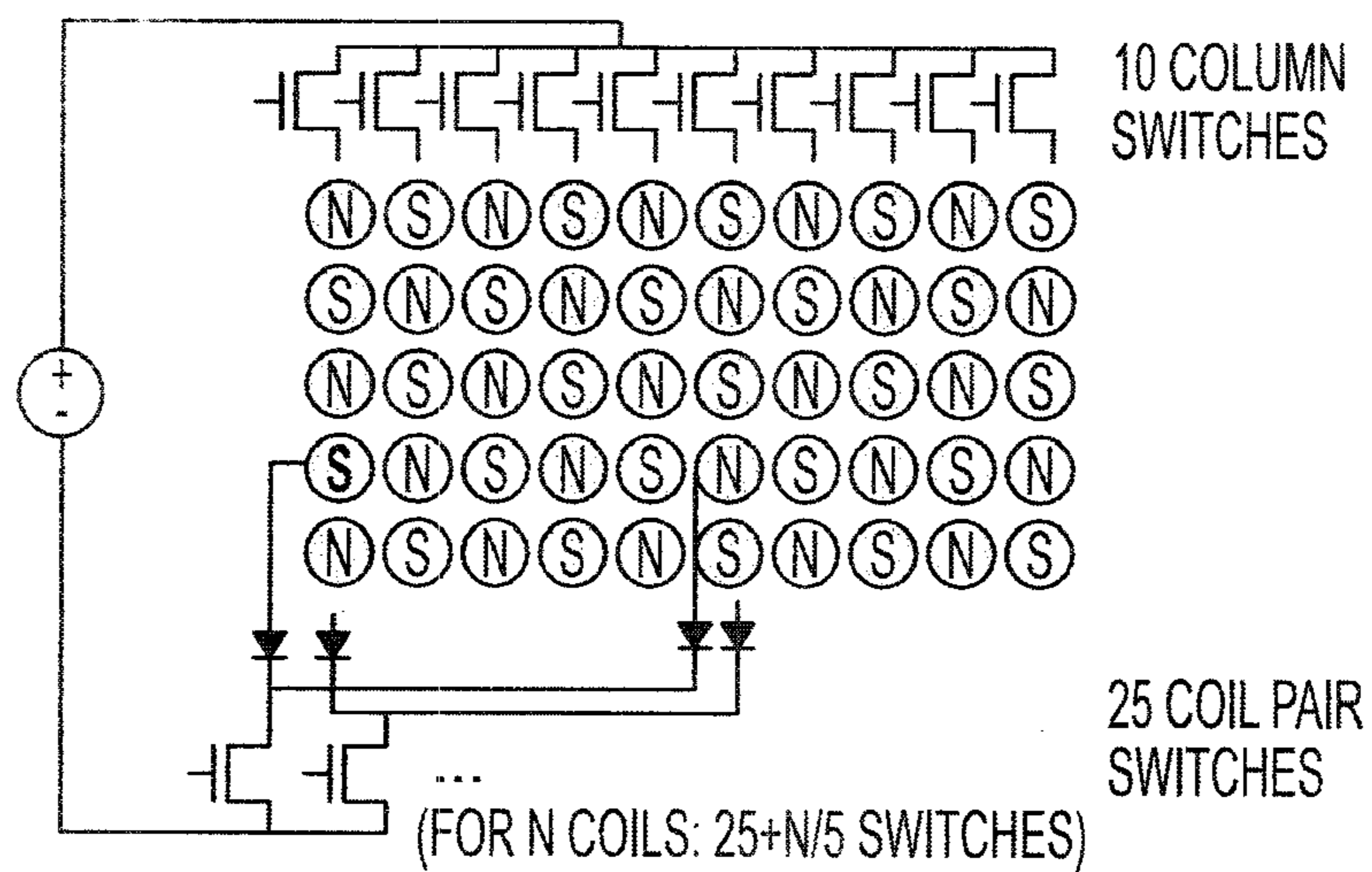
CIRCUIT DESIGN TO REDUCE # OF SWITCHES
