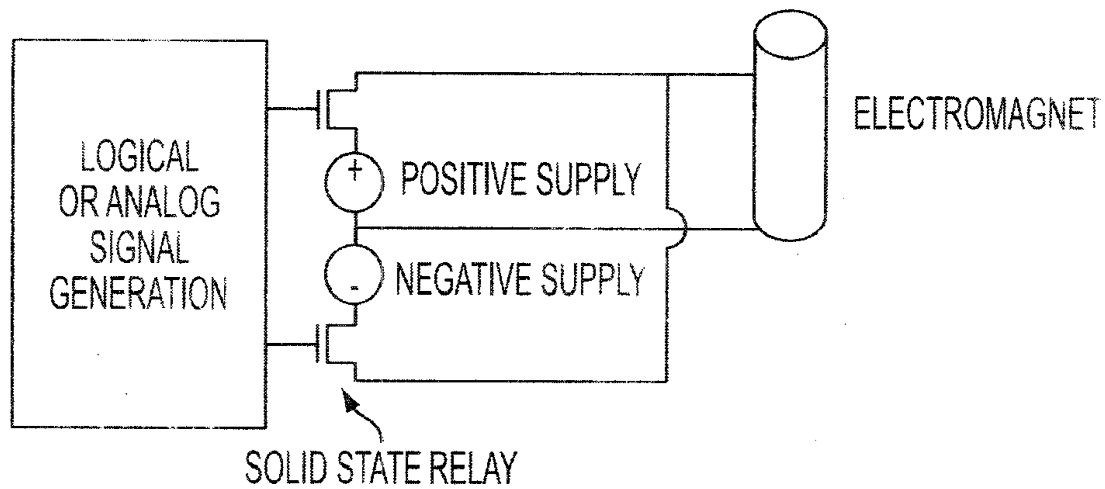
CIRCUIT DESIGN FOR REVERSIBLE MAGNETIC FIELD
