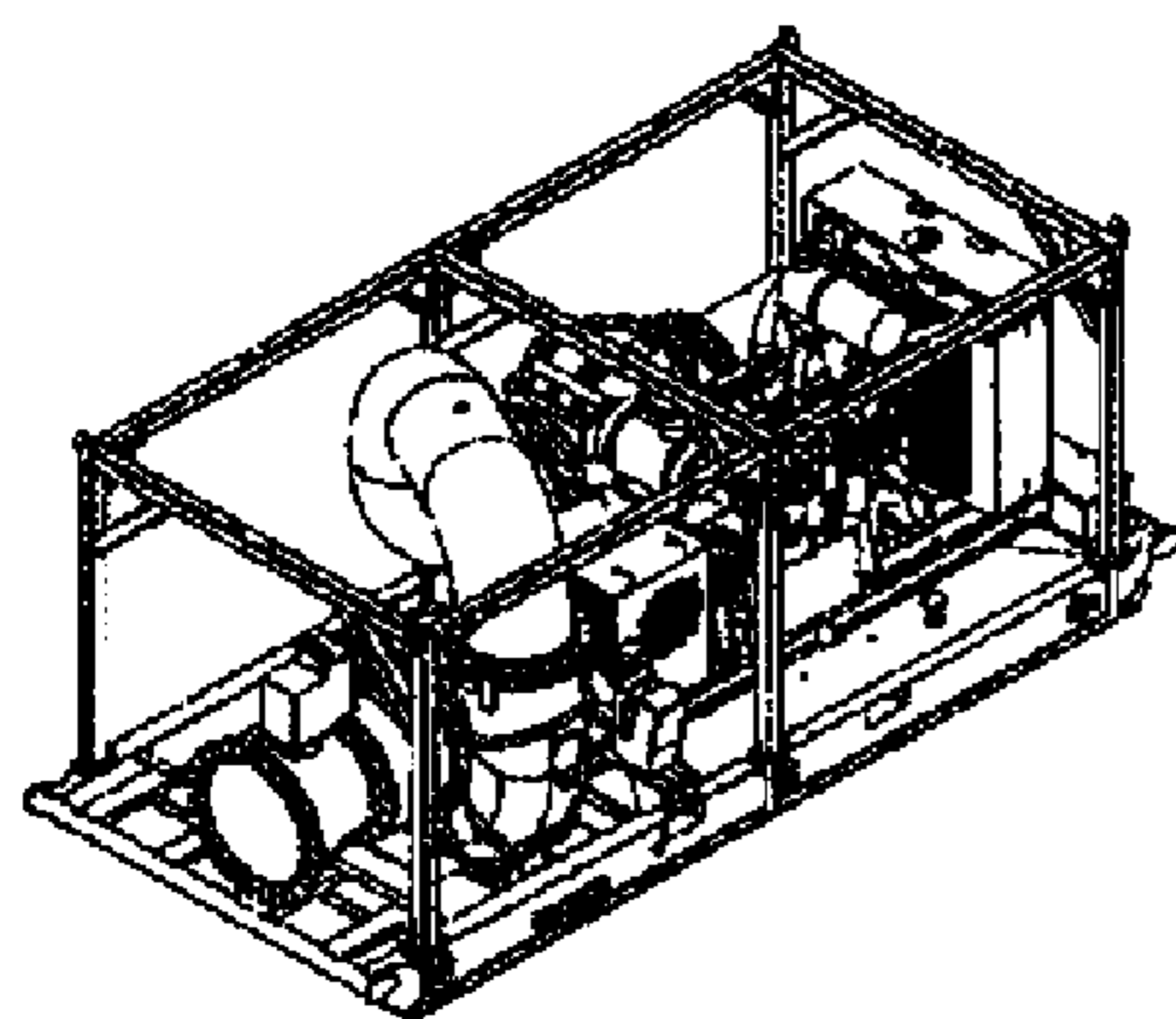
78,000 GPM Mobile liquid fire suppressant pump
