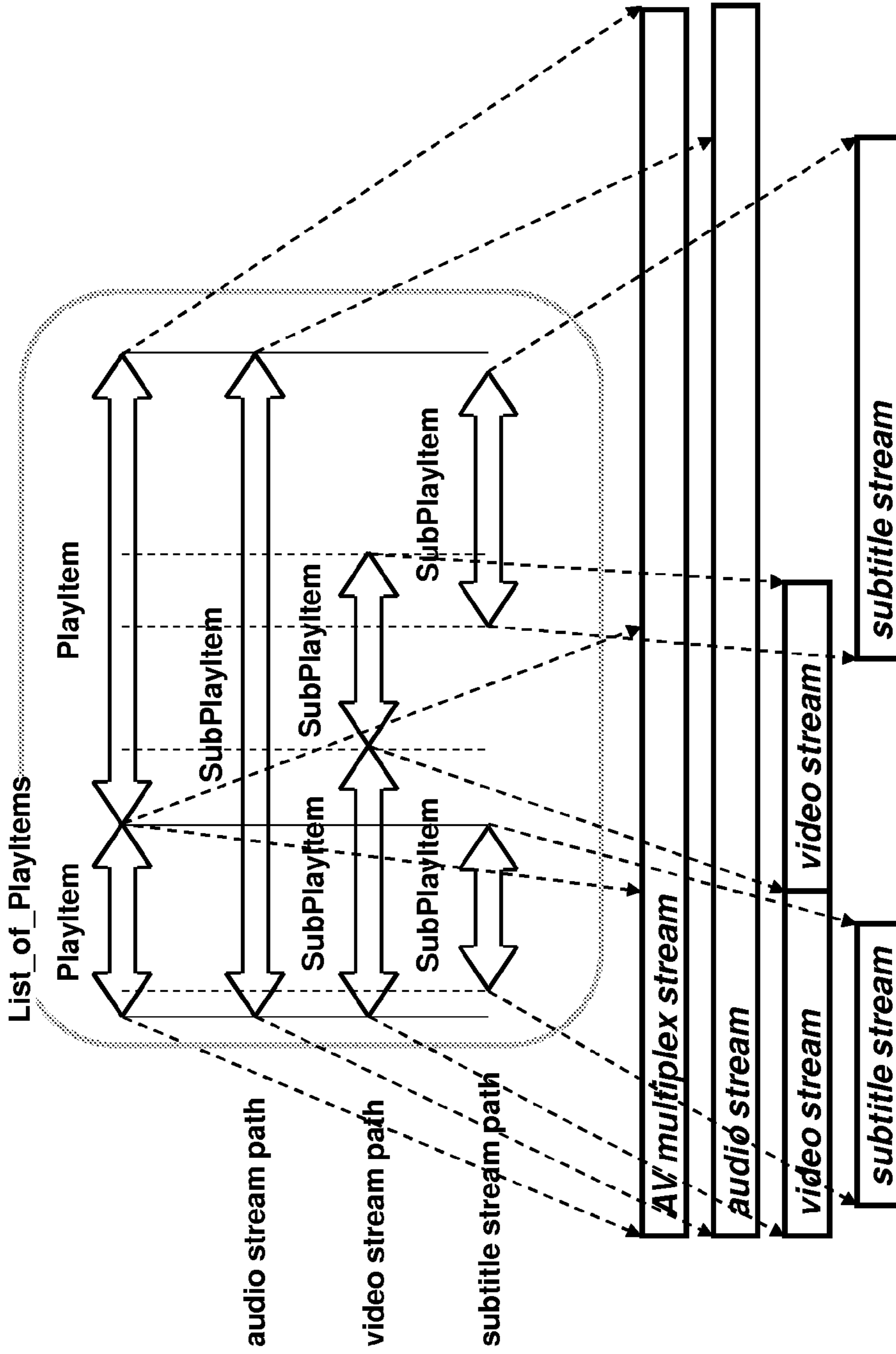
List_of_PlayItems Example
