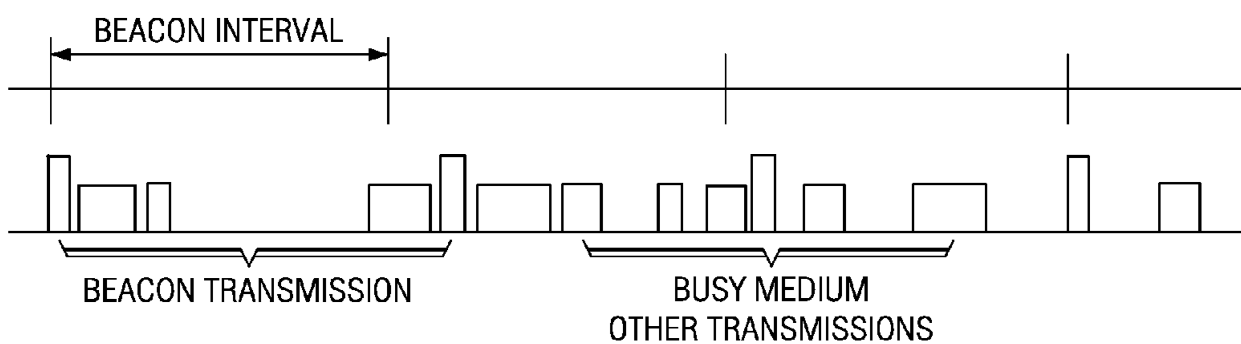
FIG. 3 (PRIOR ART)
