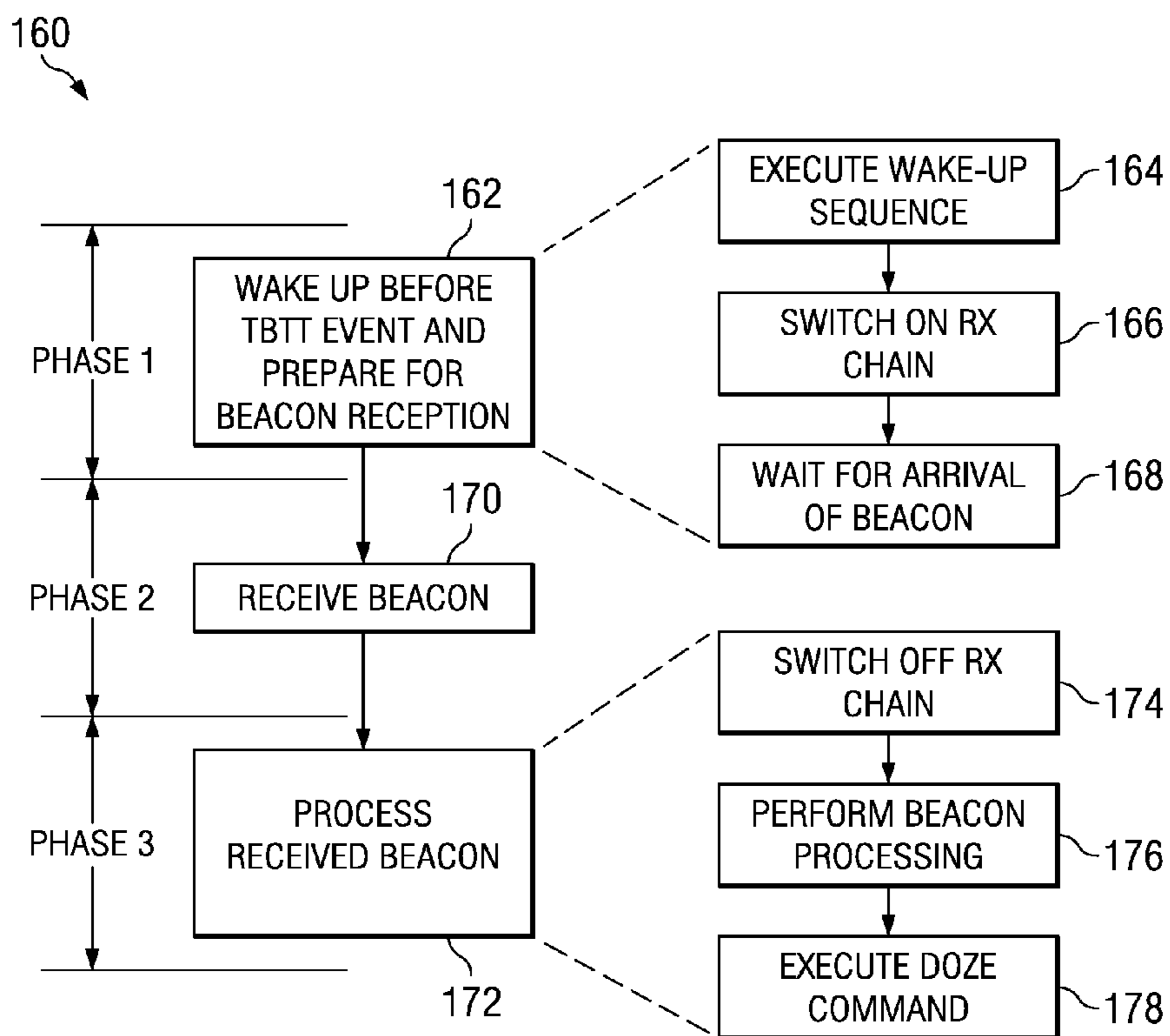
FIG. 4 (PRIOR ART)
