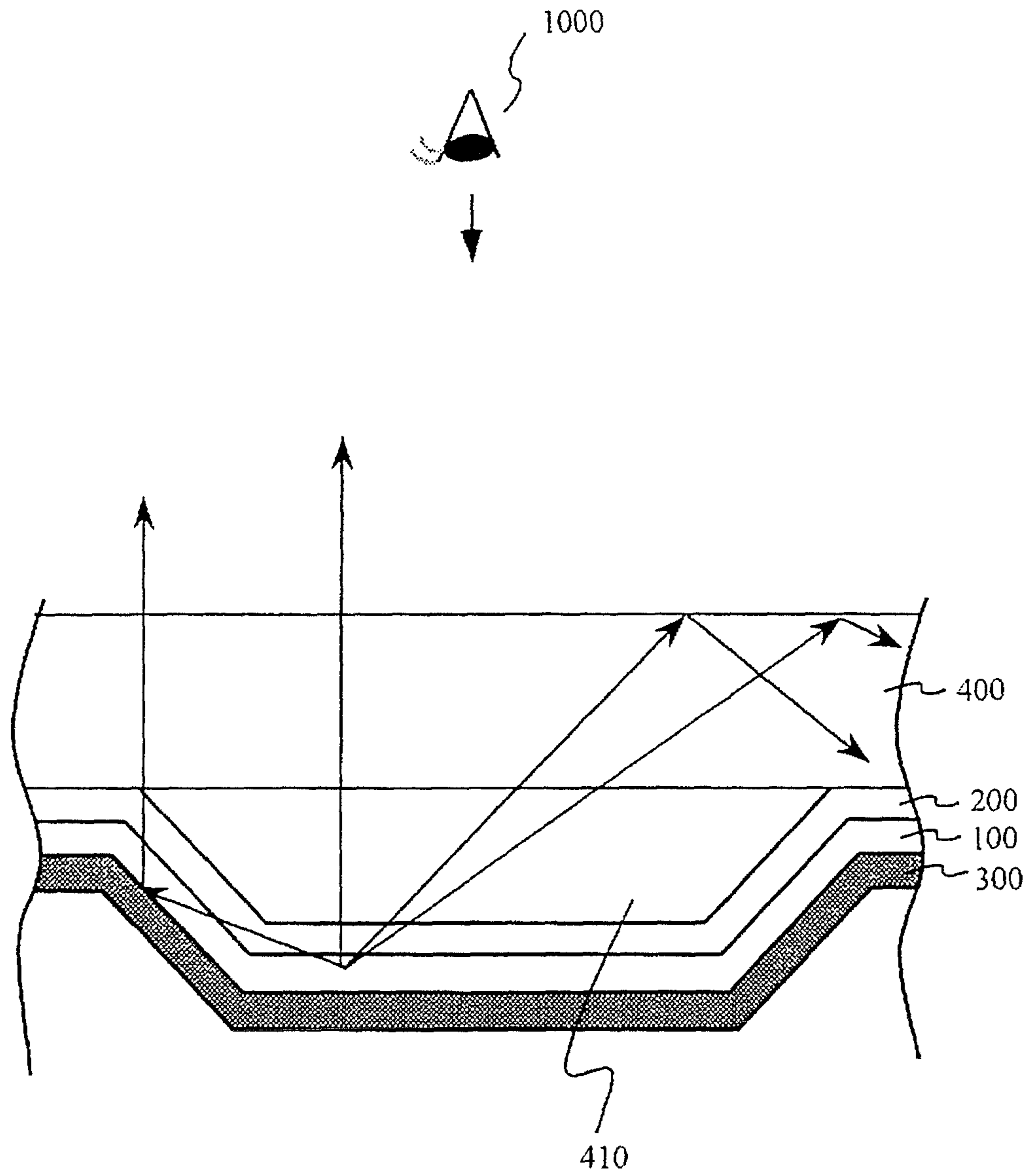
FIG. 34 PRIOR ART
