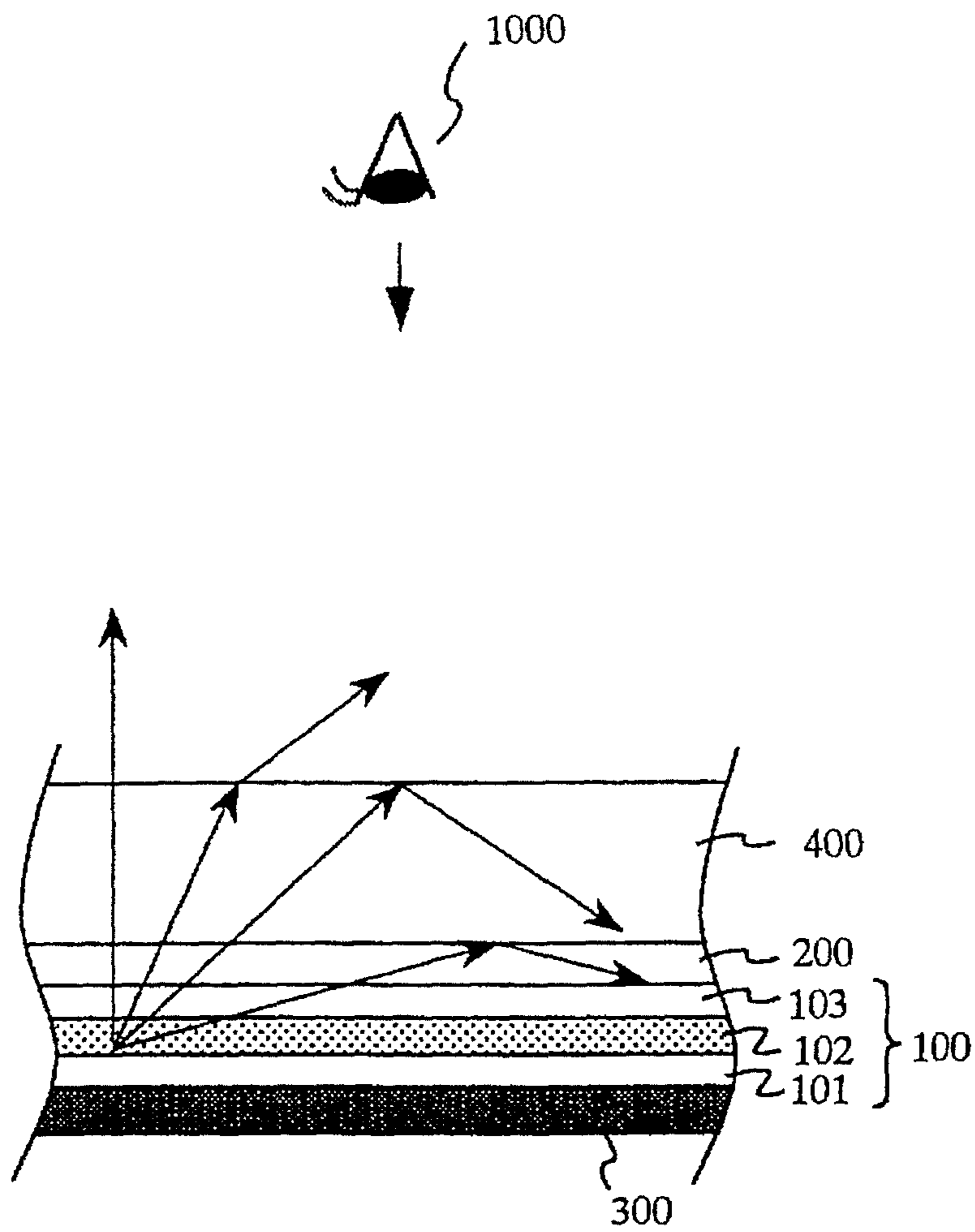
FIG. 33 PRIOR ART
