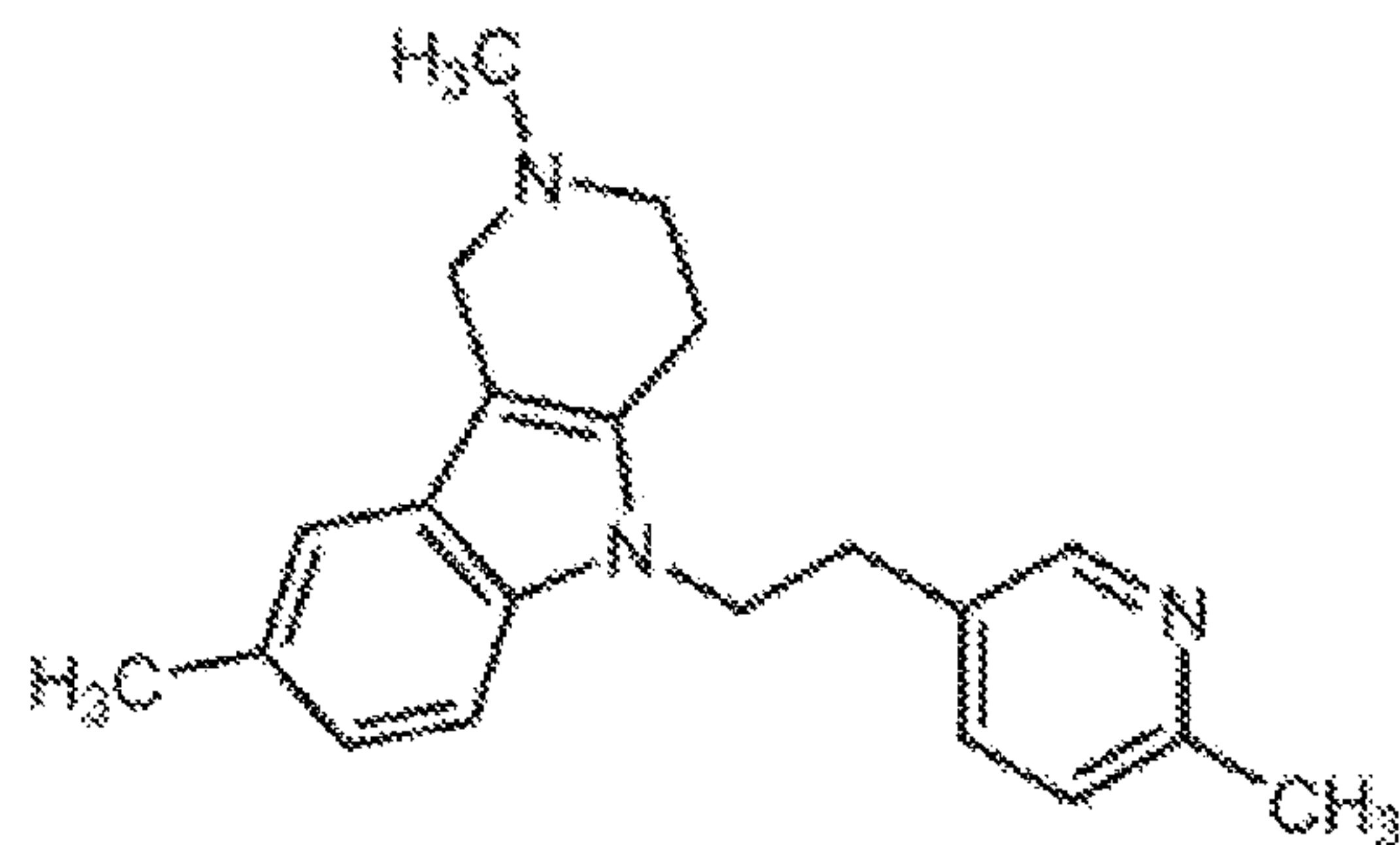
Dimebon
