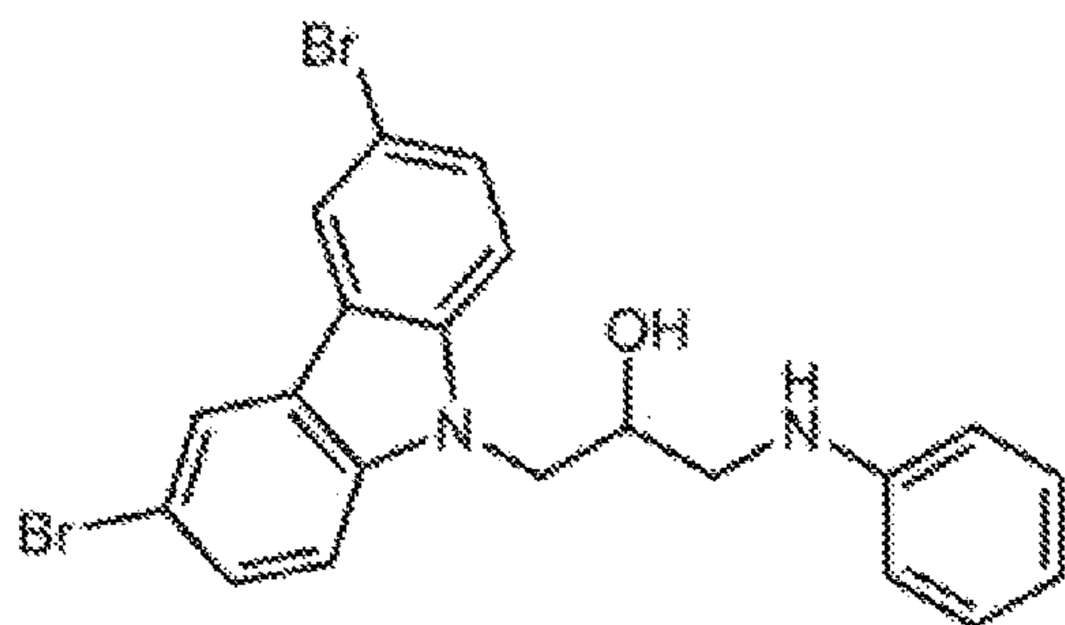
Example 45 Compound
