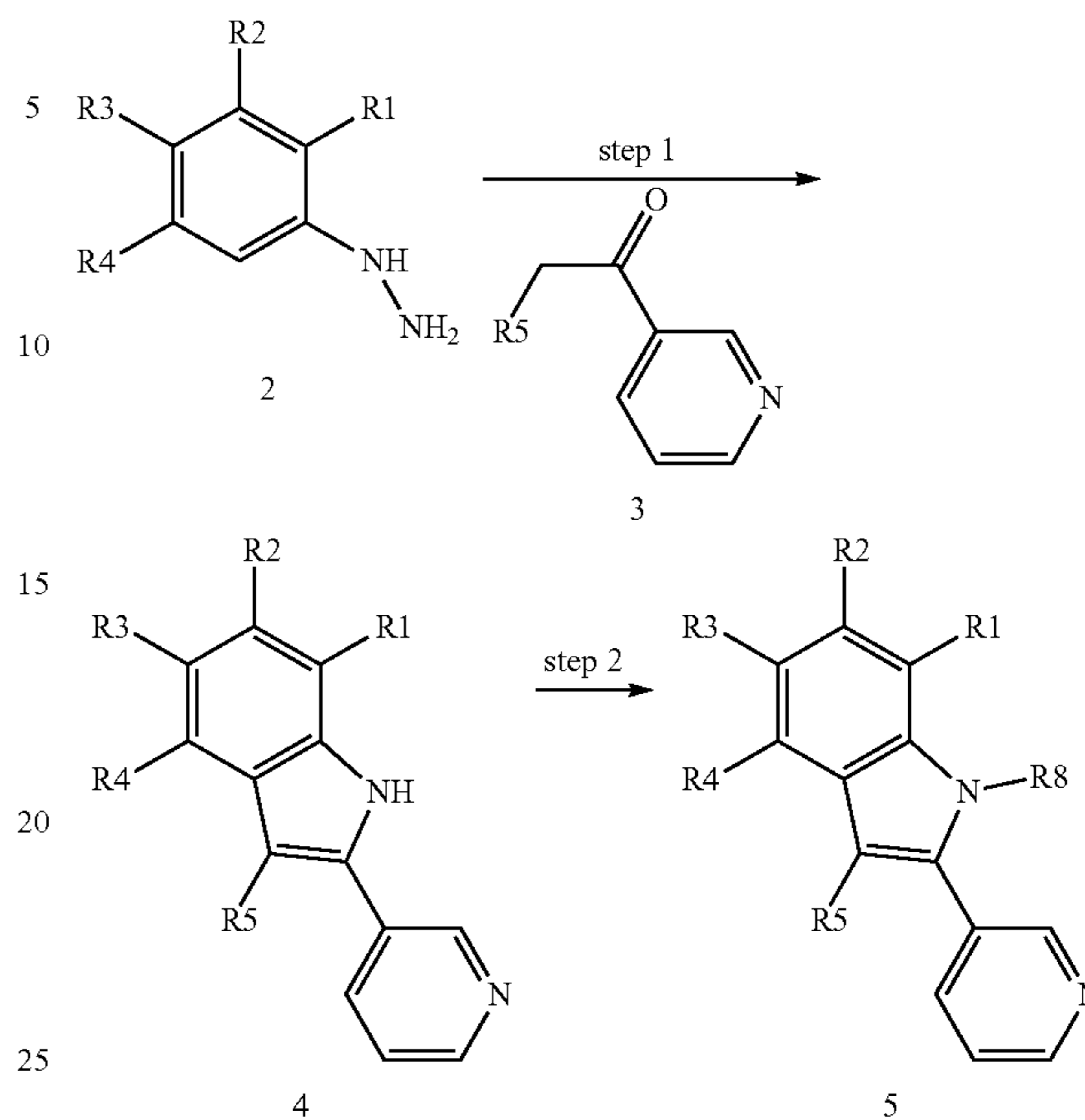
Scheme 1.
