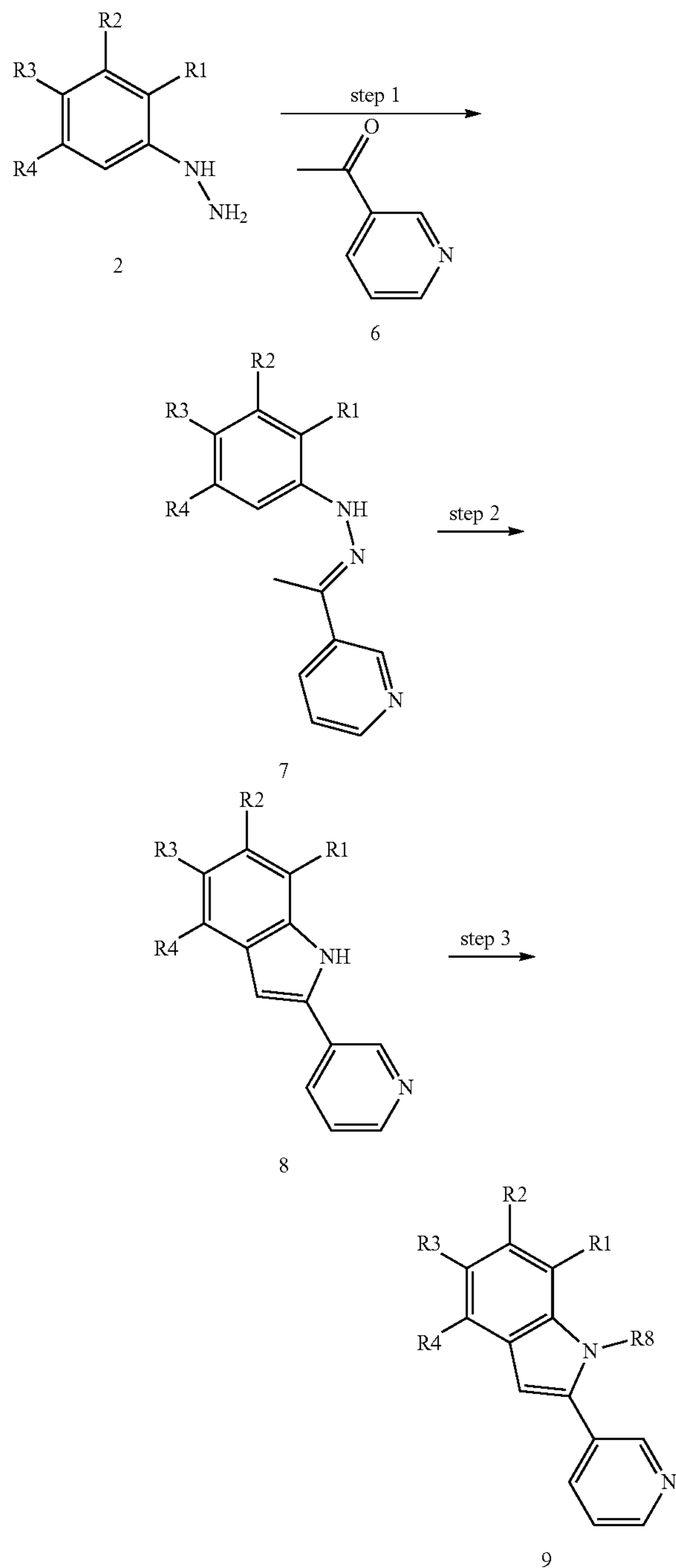
Scheme 2.
