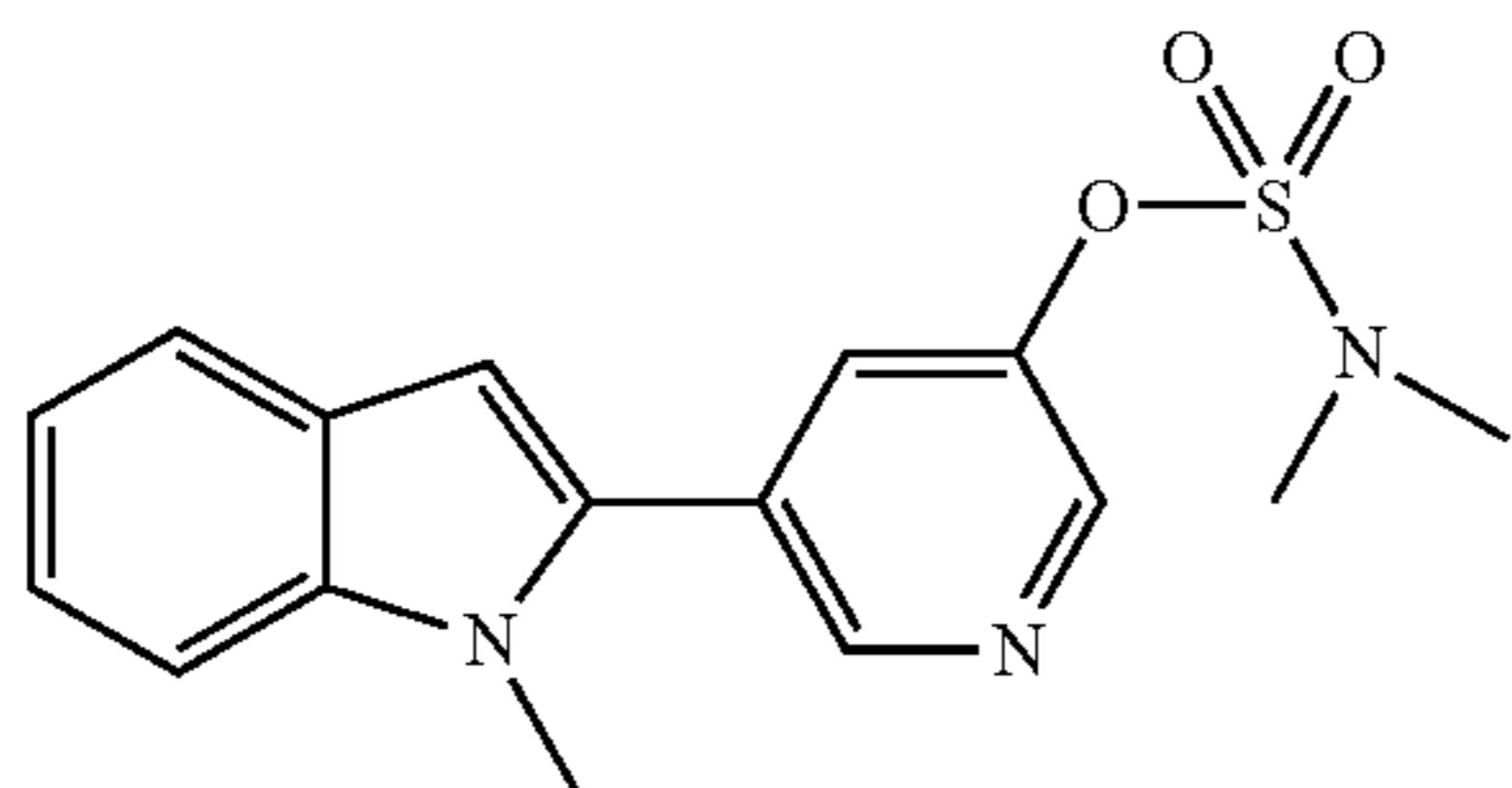
(b) Dimethyl-sulfamic acid 5-(1-methyl-1H-indol-2-yl)-pyridin-3-yl ester
