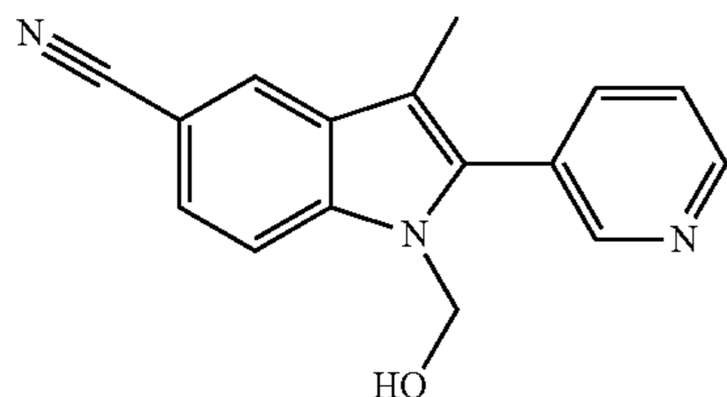
2-(5-Cyano-3-methyl-2-pyridin-3-yl-indol-1-yl)-methanol
