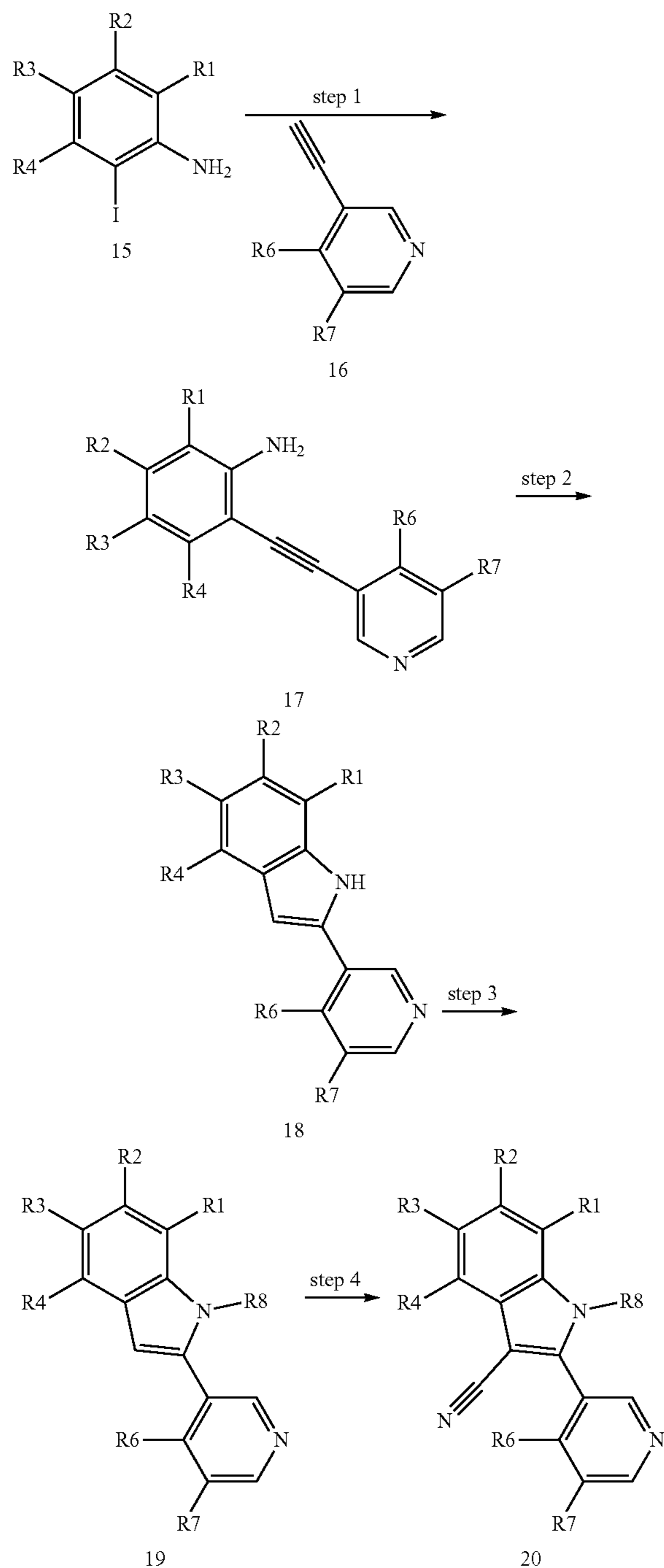
Scheme 4.
