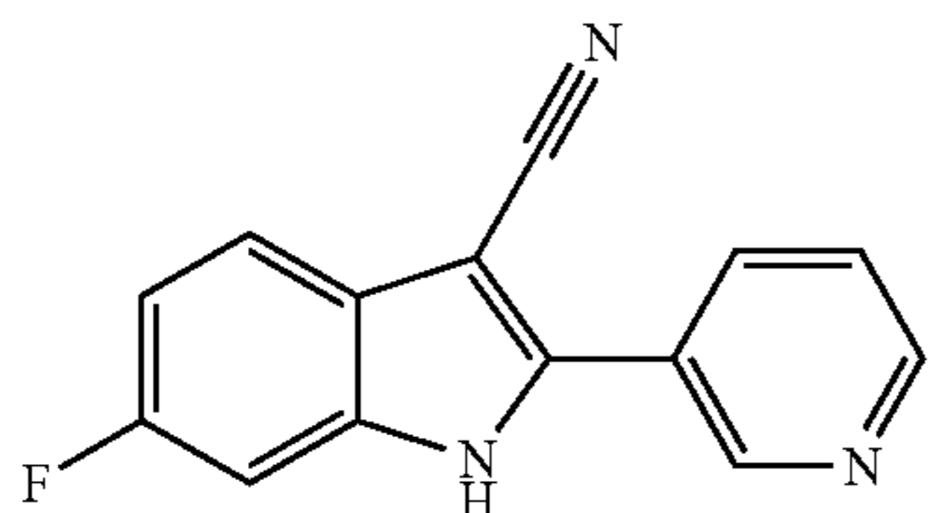
6-Fluoro-2-pyridin-3-yl-1H-indole-3-carbonitrile
