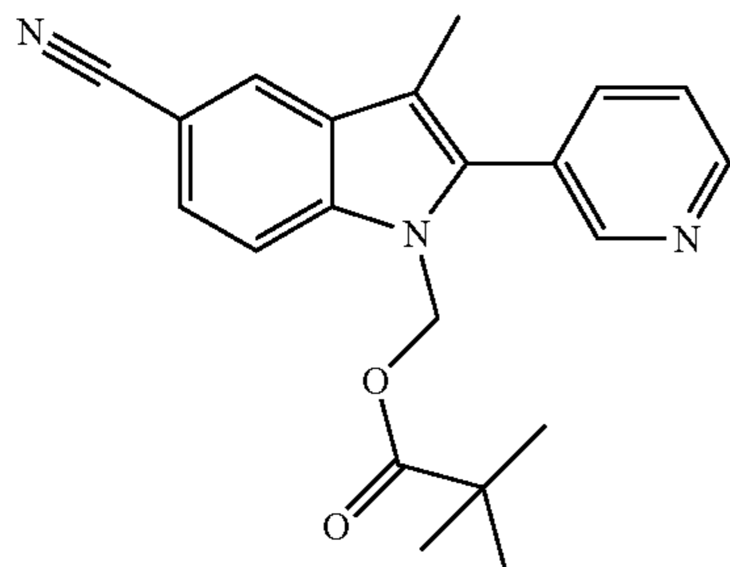
2,2-Dimethyl-propionic acid 5-cyano-3-methyl-2-pyridin-3-yl-indol-1-ylmethyl ester
