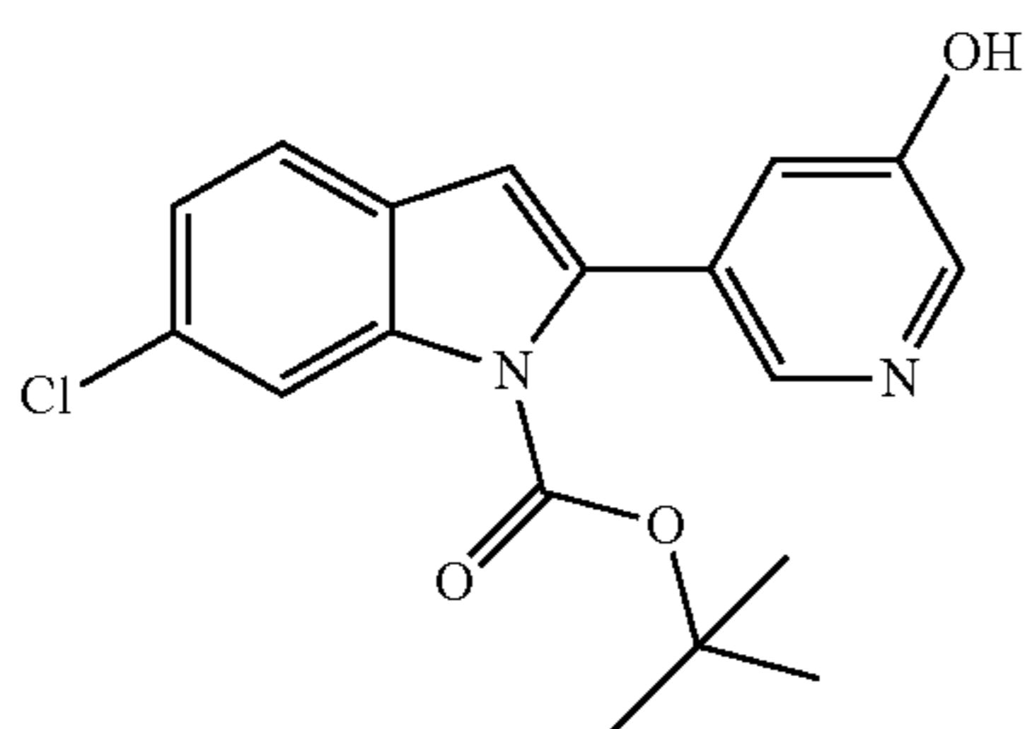
(a) 6-Chloro-2-(5-hydroxy-pyridin-3-yl)-indole-1-carboxylic acid tert-butyl ester
