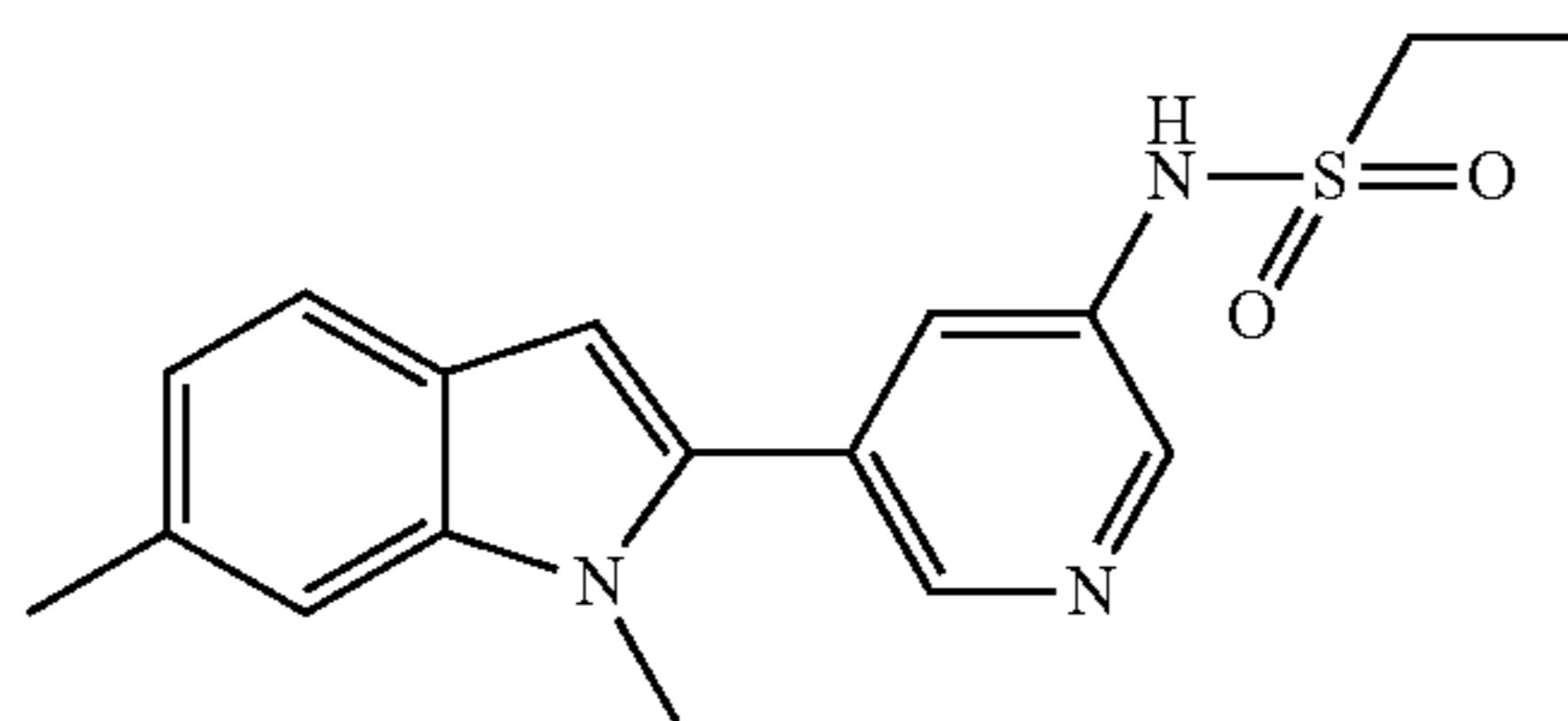
(e) Ethanesulfonic acid [5-(1,6-dimethyl-1H-indol-2-yl)-pyridin-3-yl]-amide
