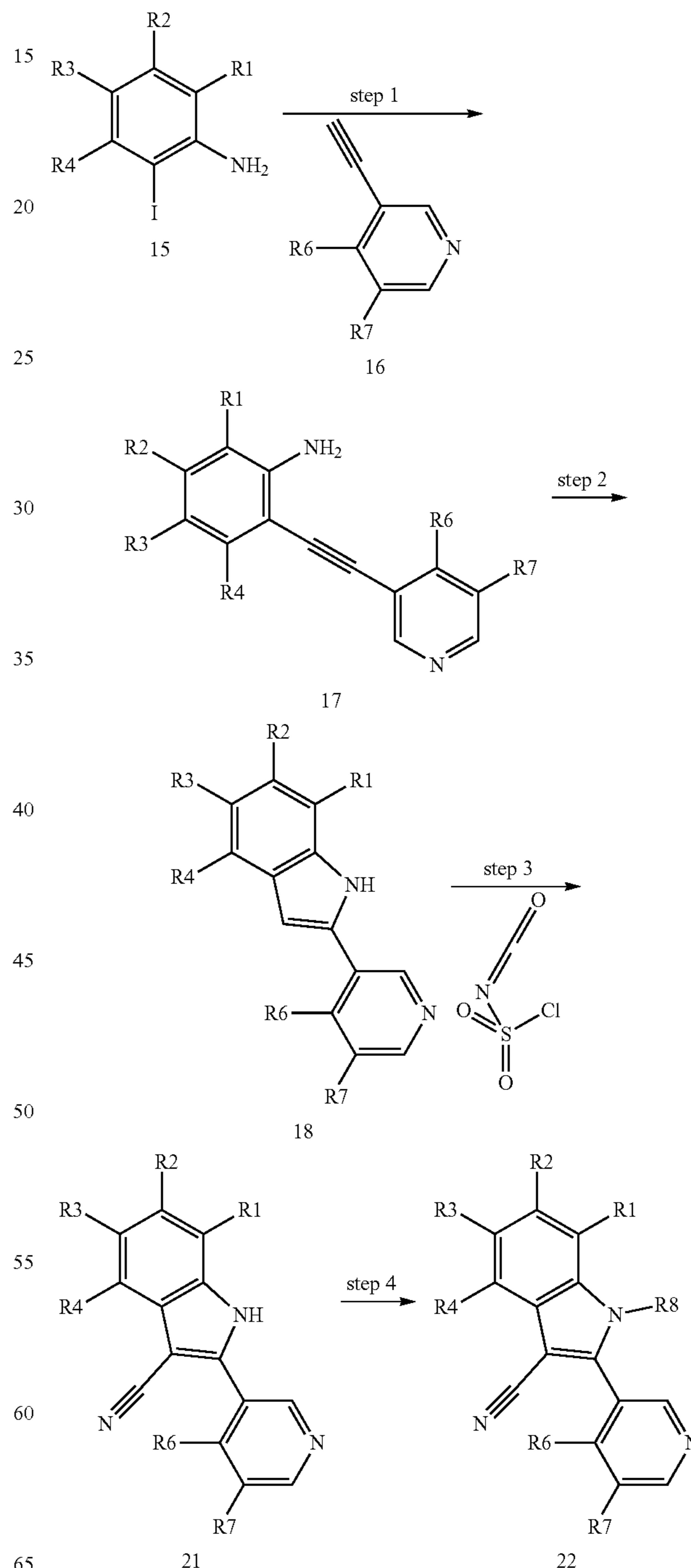
Scheme 5.
