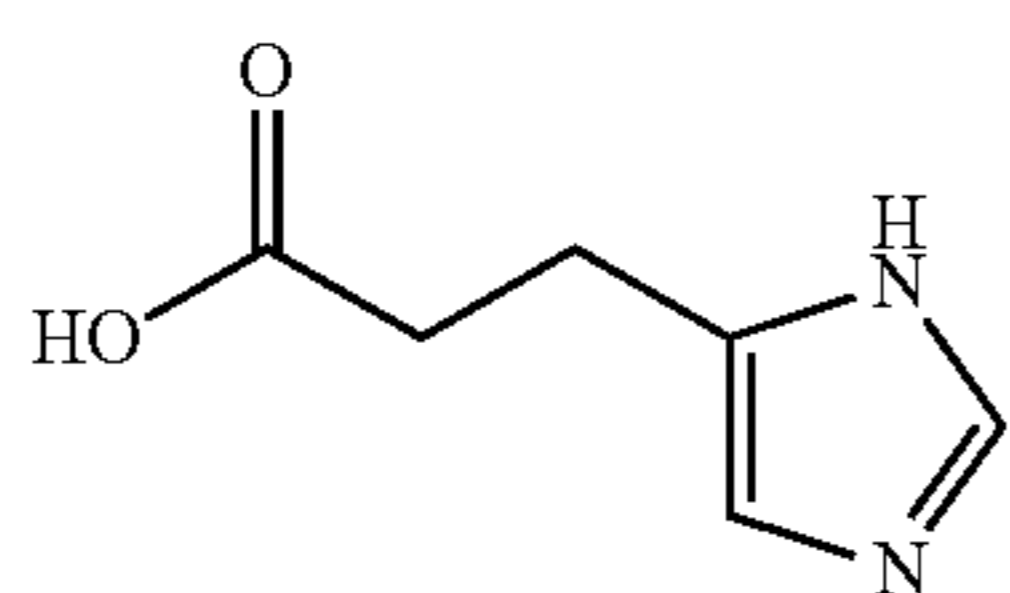
Chart 1: Representative acids for amination reactions.
