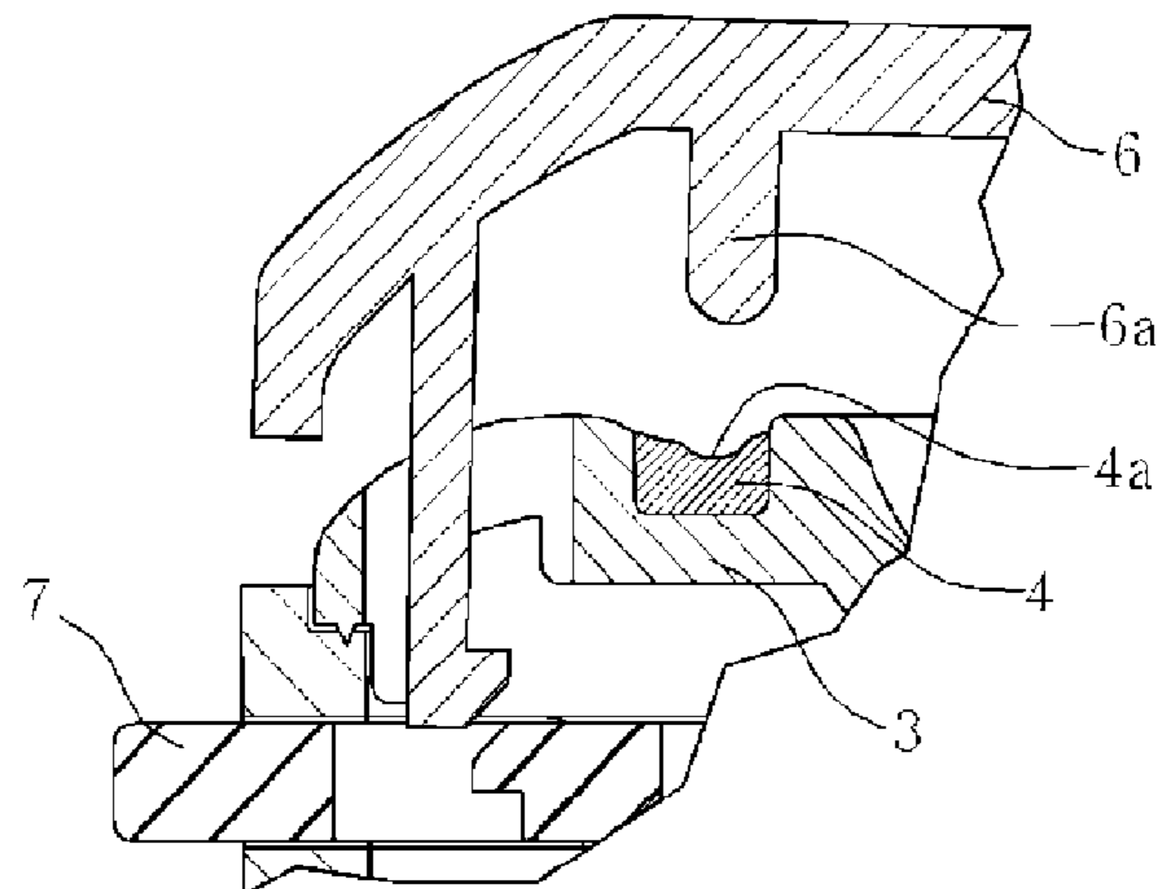
FIG. 1c (Prior Art)
