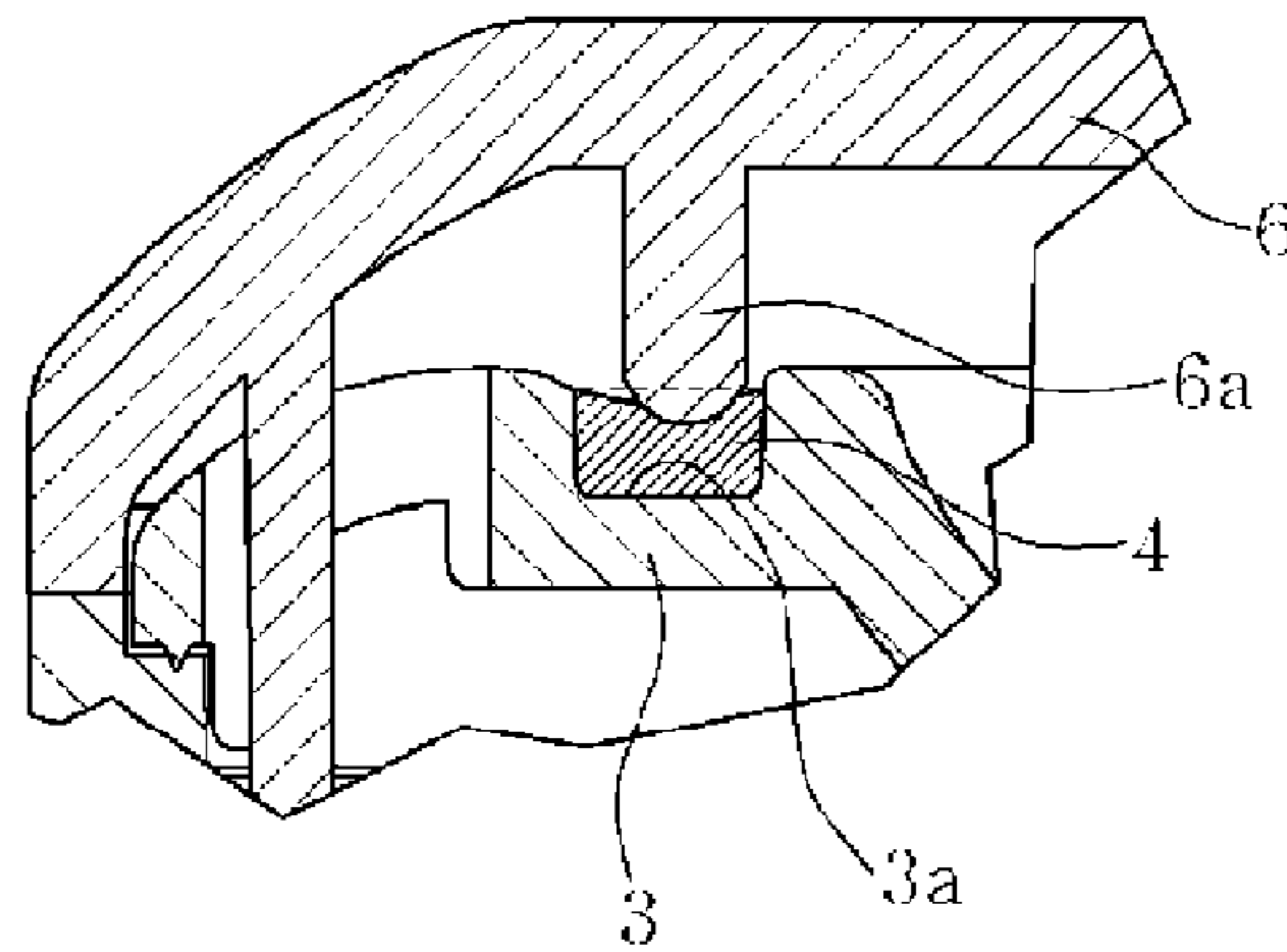
FIG. 1c (Prior Art)
