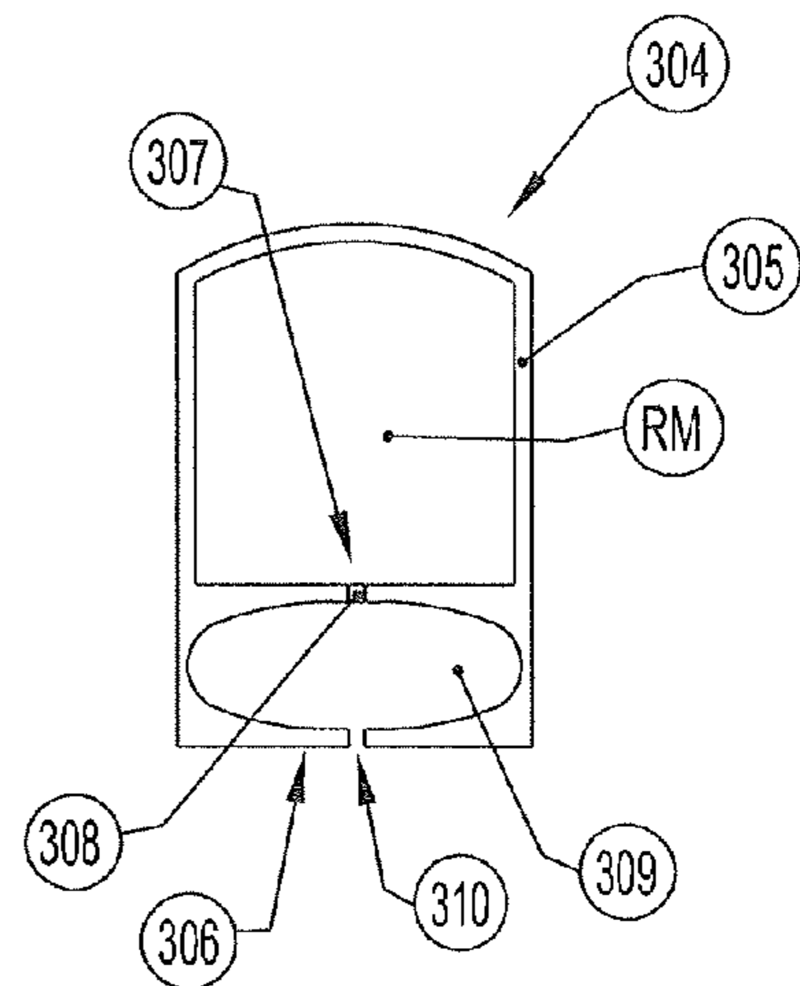
FIG 21
