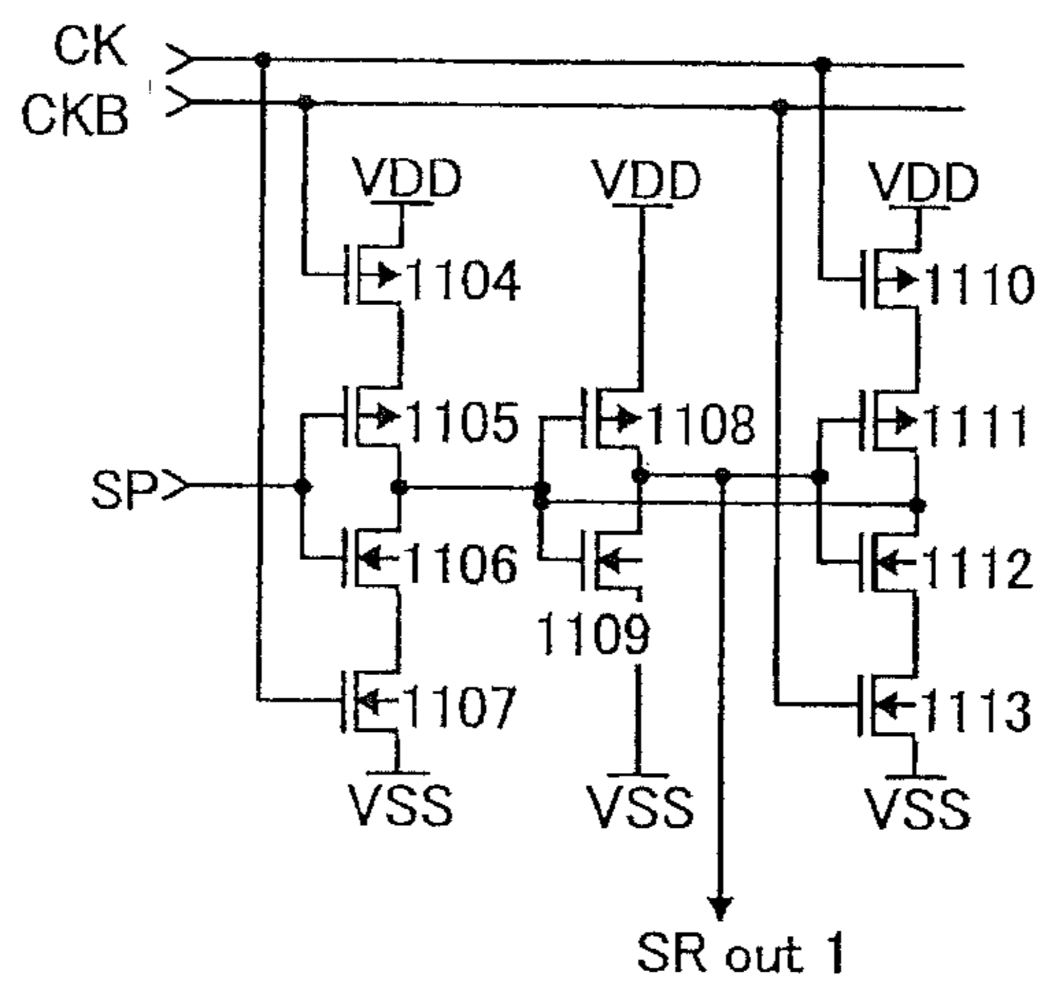
Fig. 11C Prior Art
