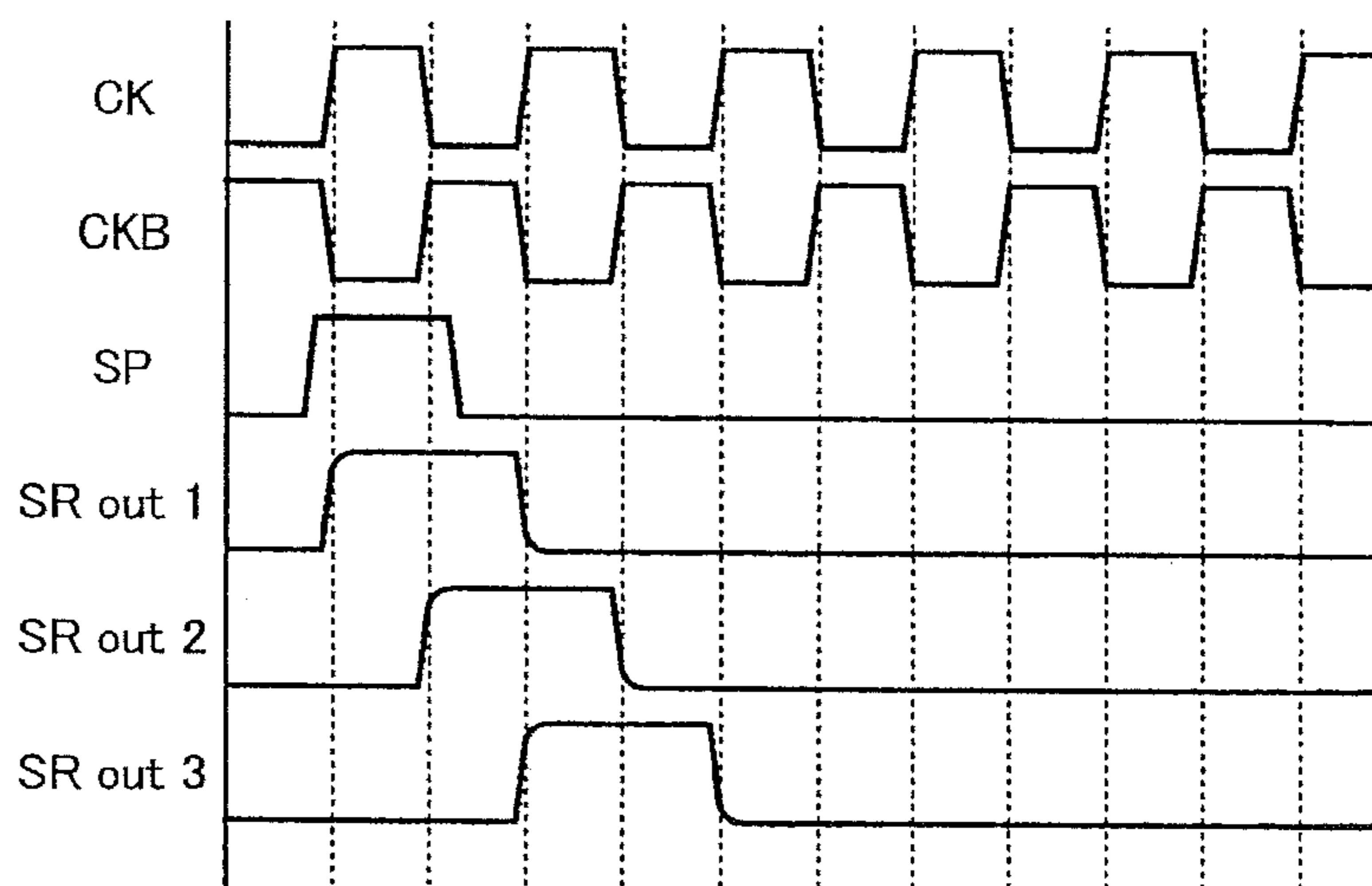
Fig. 11C Prior Art
