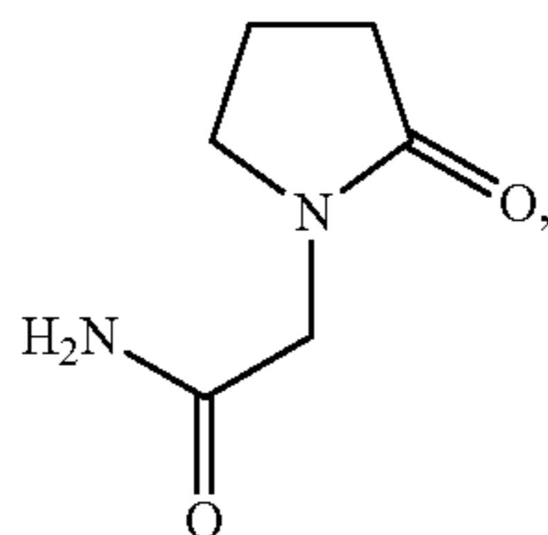
2-(2-oxo-pyrrolidino)-acetamide (also known as "piracetam");
