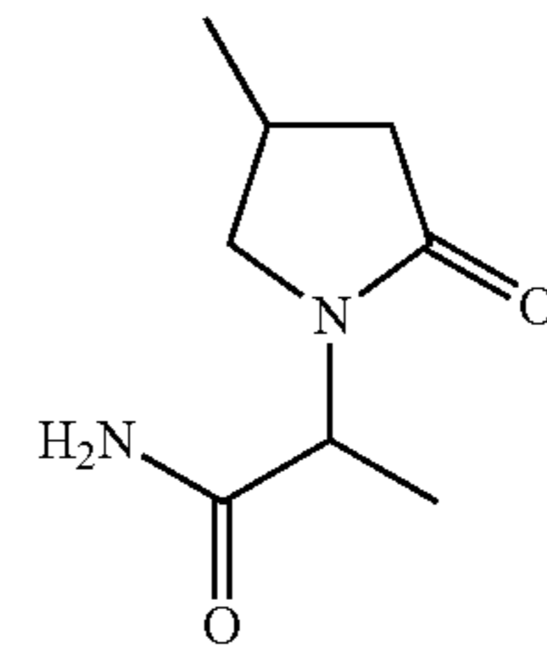
2-(4-methyl-2-oxo-pyrrolidino)-propionamide;
