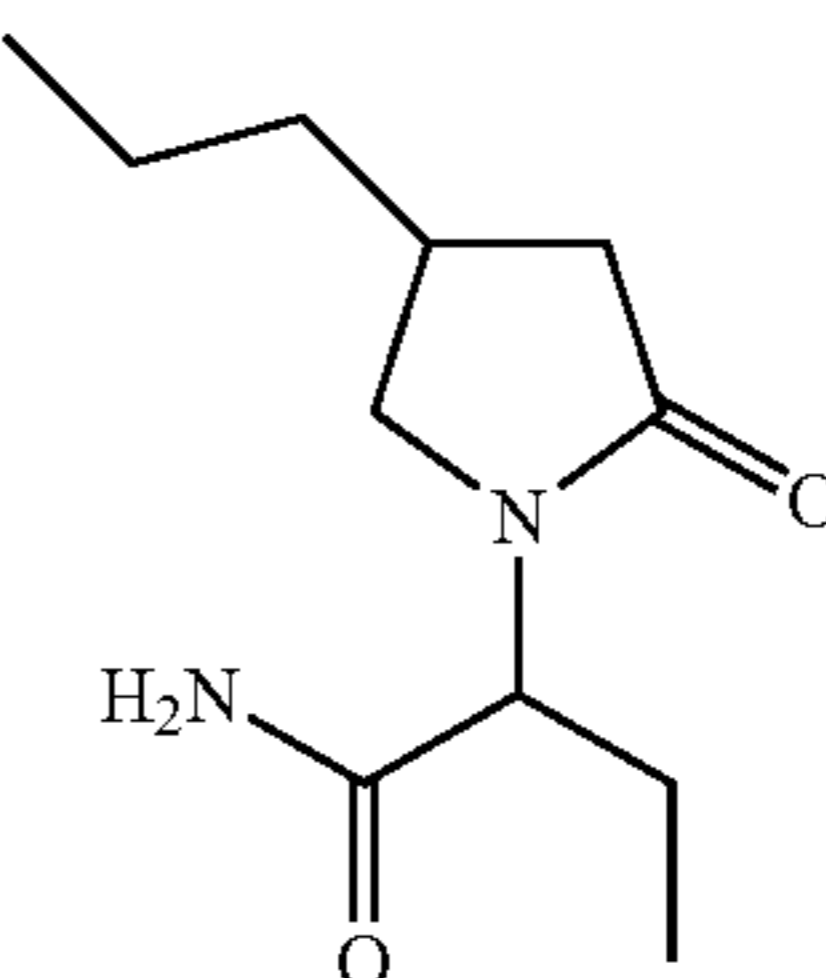
2-(4-propyl-2-oxo-pyrrolidino)-butylamide (also known as "brivaracetam");
