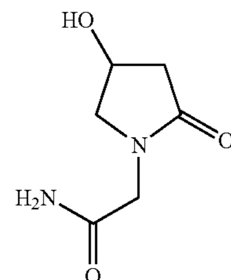
(4-hydroxy-2-oxo-pyrrolidino)-acetamide (also known as "oxiracetam");
