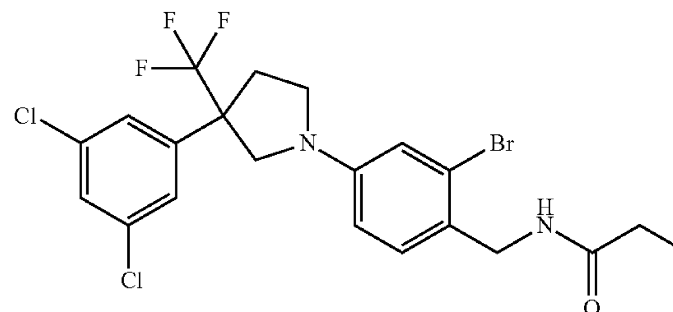
Compound No. 3-5 according to WO2008/128711
