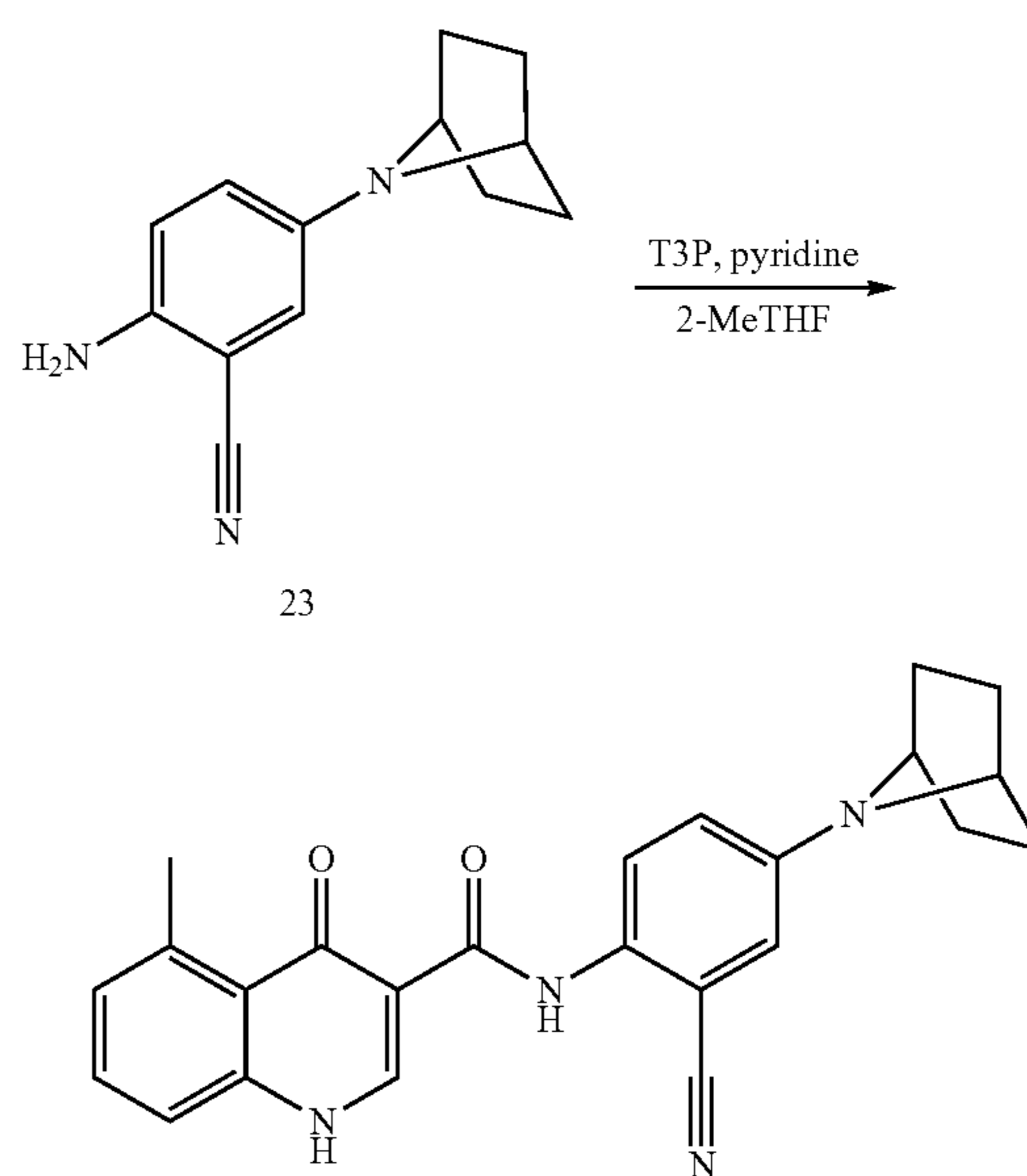
Example Compound 6
