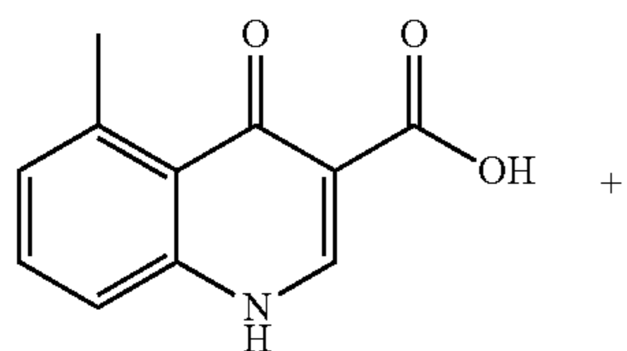
Scheme 11
