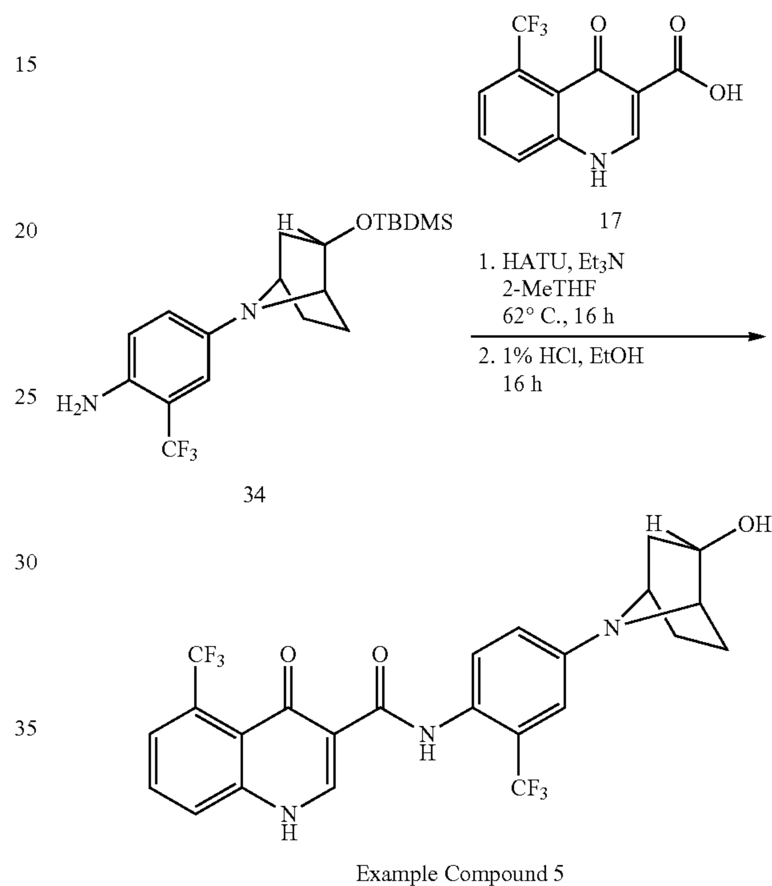
Scheme 13
