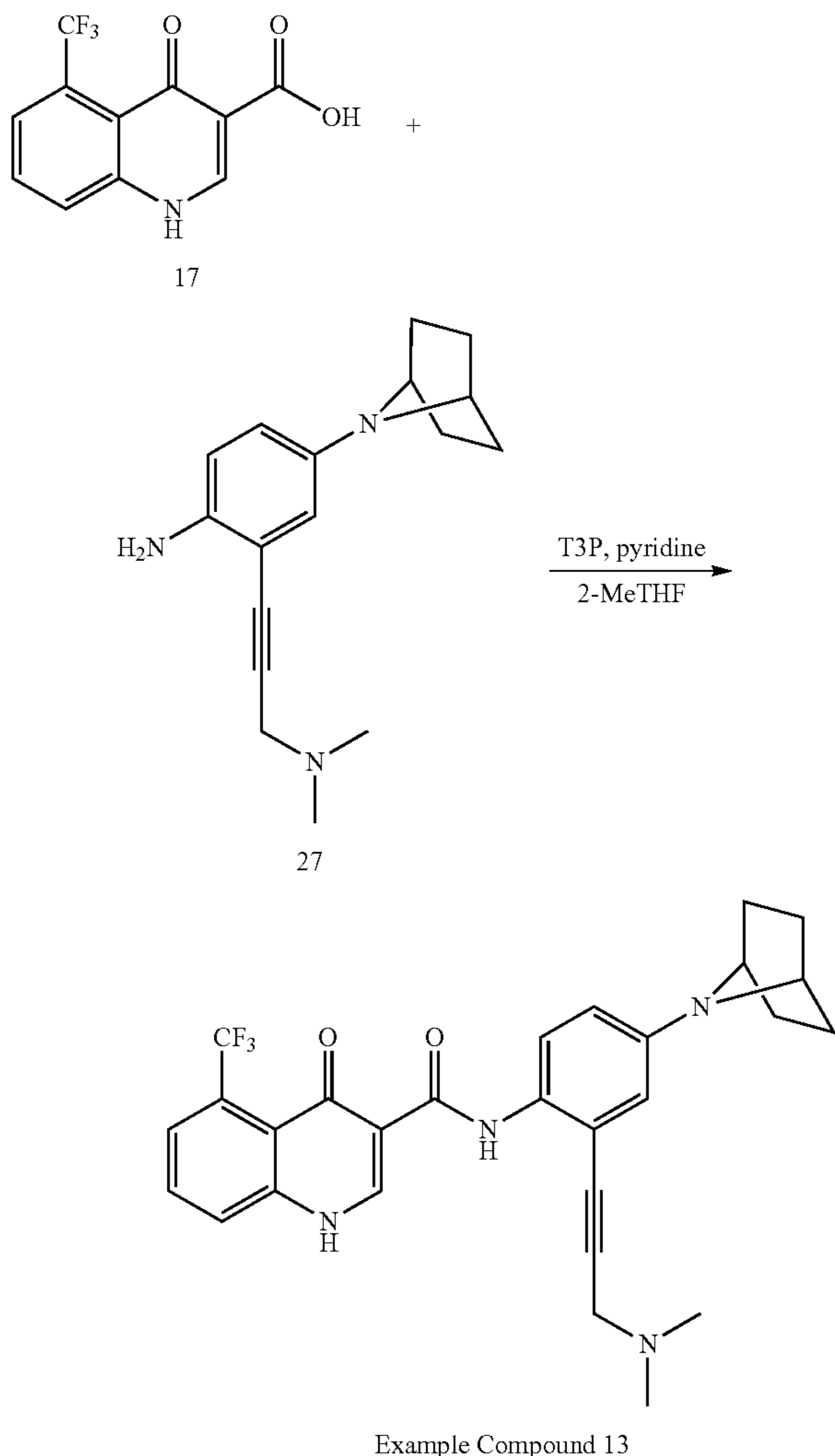
Scheme 12
