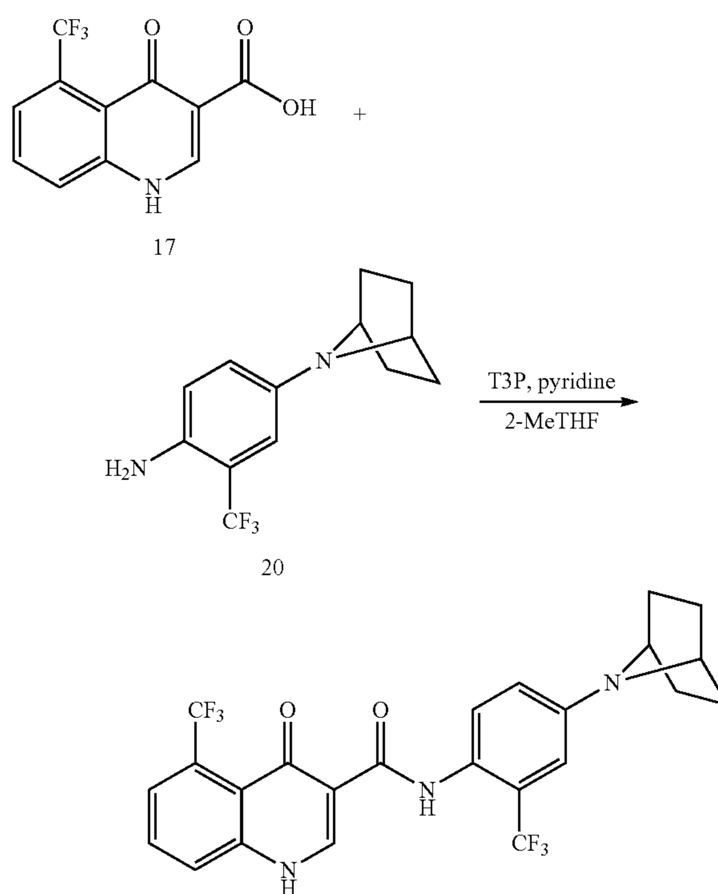
Example Compound 3
