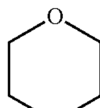
tetrahydropyran (tetrahydropyranly)
