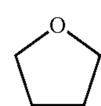
tetrahydrofuran (tetrahydrofuranlyl)
