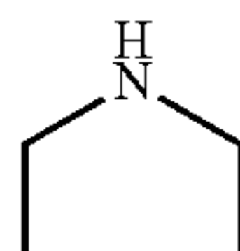
1,4-dioxane (1,4-dioxanyl)
