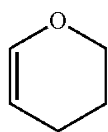
3,4-dihydro-2H-pyran (3,4-dihydro-2H-pyranlyl)
