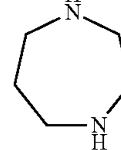
1,4-diazepepane (1,4-diazepepanyl)
