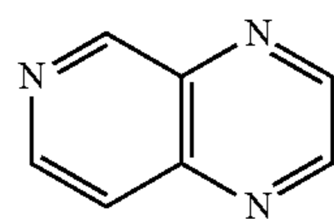
pyrido[3,4-b]pyrazine (pyrido[3,4-b]pyrazinyl)
