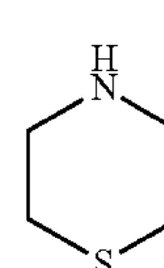
1,4-azathiane (1,4-azathianyl)
