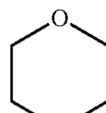
1,4-dioxane (1,4-dioxanyl)
