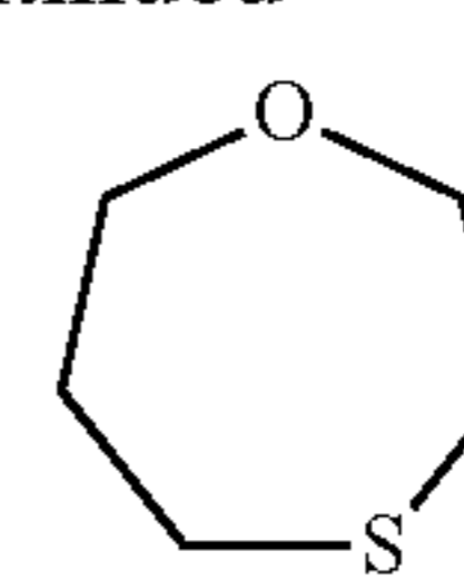
1,4-oxathiepane (1,4-oxathiepanyl)
