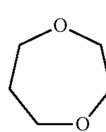
1,4-dioxepane (1,4-dioxepanyl)
