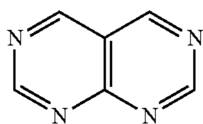
pyrimido[4,5-d]pyrimidine (pyrimido[4,5-d]pyrimidinyl)
