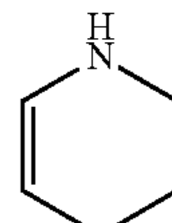
1,2,3,4-tetrahydropyridine (1,2,3,4-tetrahydropyridinyl)
