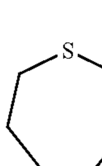
thiepane (thiepanyl)
