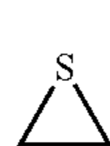
thiarane (thiaranyl)
