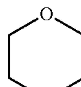
1,4-dioxane (1,4-dioxanyl)
