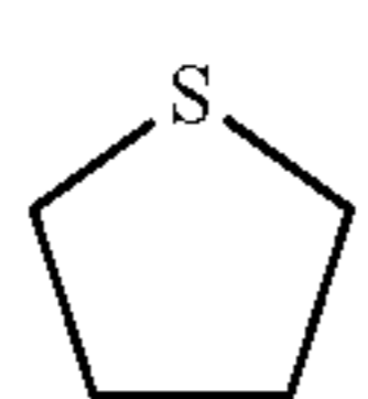
tetrahydrothiophane (tetrahydrothiophenyl)
