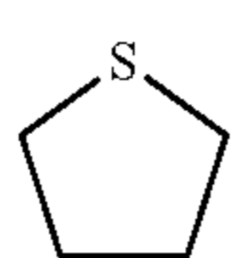
tetrahydrothiophane (tetrahydrothiophenyl)
