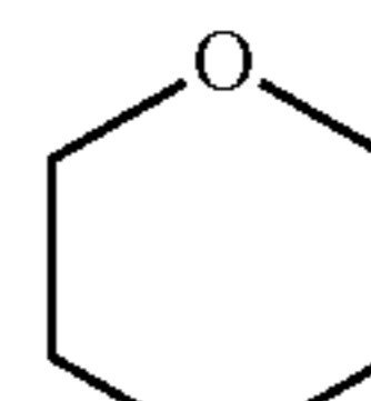
1,4-oxathiane (1,4-oxathianyl)
