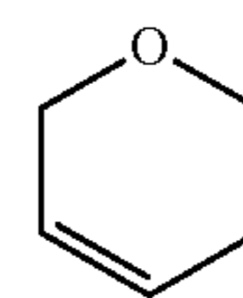
5,6-dihydro-2H-pyran (5,6-dihydro-2H-pyranlyl)
