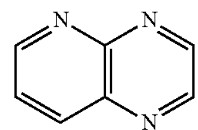
pyrido[2,3-b]pyrazine (pyrido[2,3-b]pyrazinyl)
