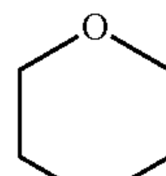
1,4-oxathiane (1,4-oxathianyl)
