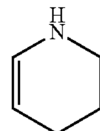
1,2,3,4-tetrahydropyridine (1,2,3,4-tetrahydropyridinyl)
