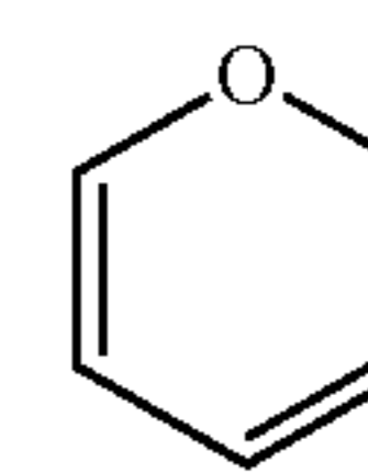
2H-pyran (2H-pyranly)
