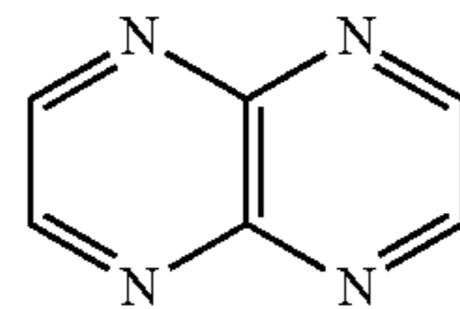
pyrazino[2,3-b]pyrazine (pyrazino[2,3-b]pyrazinyl)
