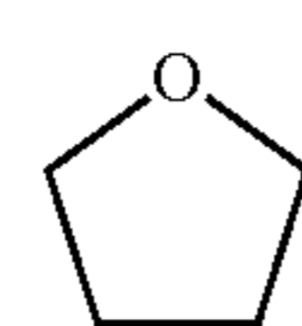
tetrahydrofuran (tetrahydrofuranly)
