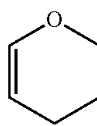
3,4-dihydro-2H-pyran (3,4-dihydro-2H-pyranly)
