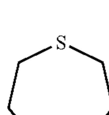
1,4-dioxepane (1,4-dioxepanyl)
