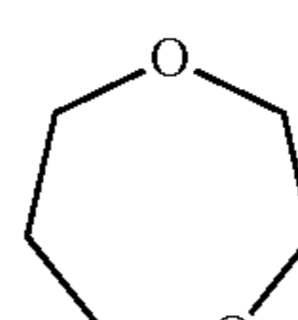
1,4-dioxepane (1,4-dioxepanyl)
