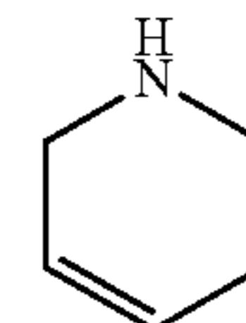
1,2,5,6-tetrahydropyridine (1,2,5,6-tetrahydropyridinyl)
