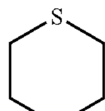
tetrahydrothiopyran (tetrahydrothiopyranlyl)
