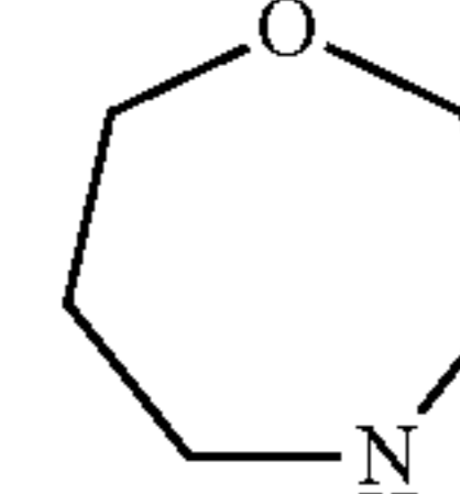
1,4-oxaazepane (1,4-oxaazepanyl)
