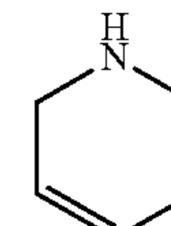
1,2,5,6-tetrahydropyridine (1,2,5,6-tetrahydropyridinyl)
