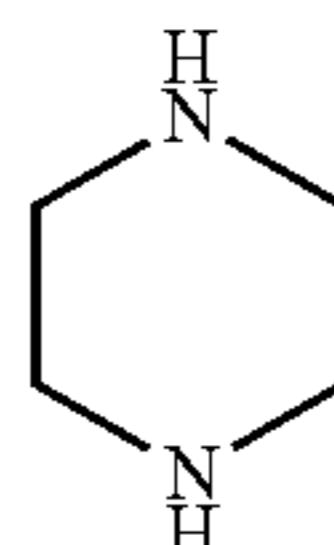
piperazine (piperazinyl)
