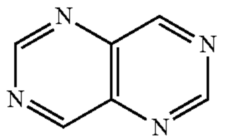
pyrimido[5,4-d]pyrimidine (pyrimido[5,4-d]pyrimidinyl)
