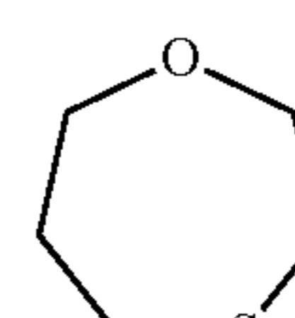
1,4-oxathiepane (1,4-oxathiepanyl)
