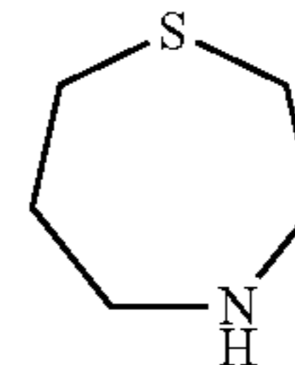
1,4-thieazepane (1,4-thieazepanyl)
