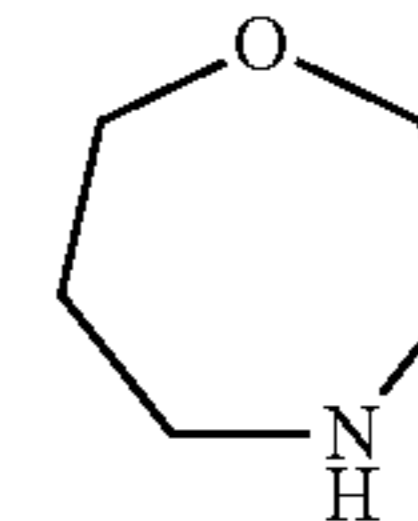
1,4-oxaazepane (1,4-oxaazepanyl)
