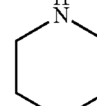
piperidine (piperidinyl)
