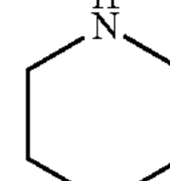
piperidine (piperidinyl)
