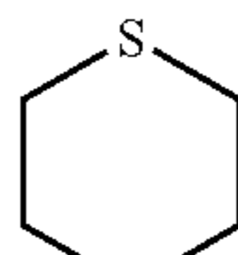
tetrahydrothiopyran (tetrahydrothiopyranly)
