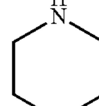
morpholine (morpholinyl)
