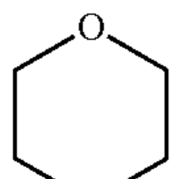
tetrahydropyran (tetrahydropyranlyl)
