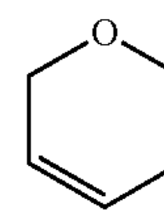
5,6-dihydro-2H-pyran (5,6-dihydro-2H-pyranly)
