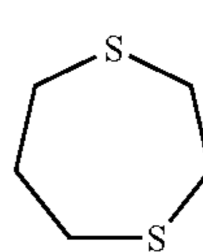
1,4-dithiepane (1,4-dithiepanyl)
