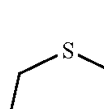
1,4-dithiane (1,4-dithianyl)
