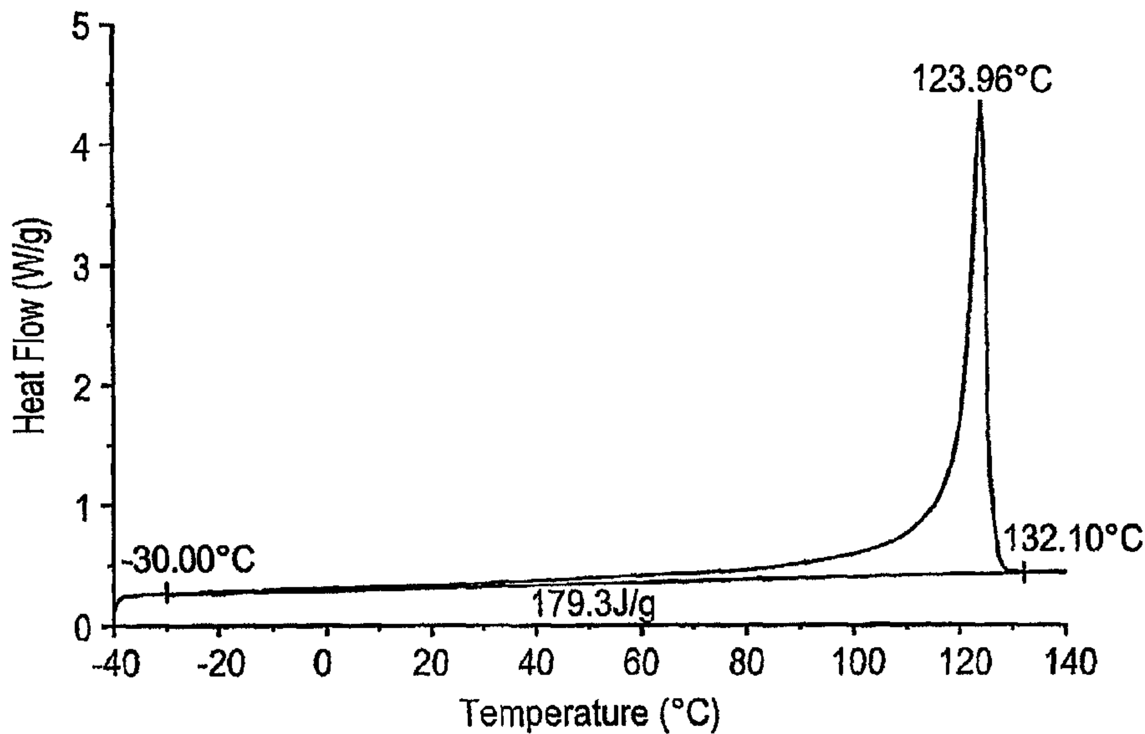
FIG. 26 DSC Comparative E*
