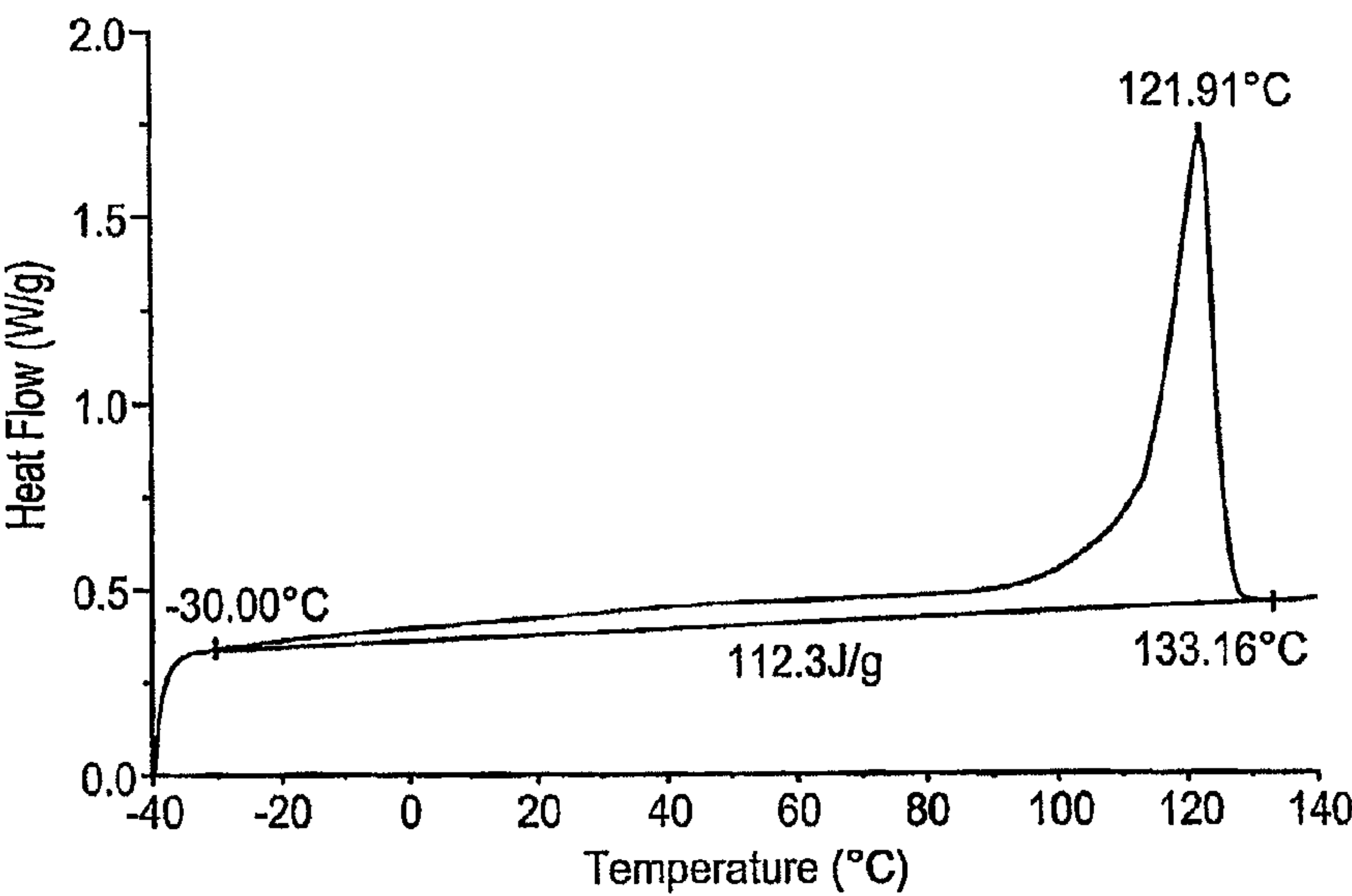
FIG. 46 DSC Comparative M*
