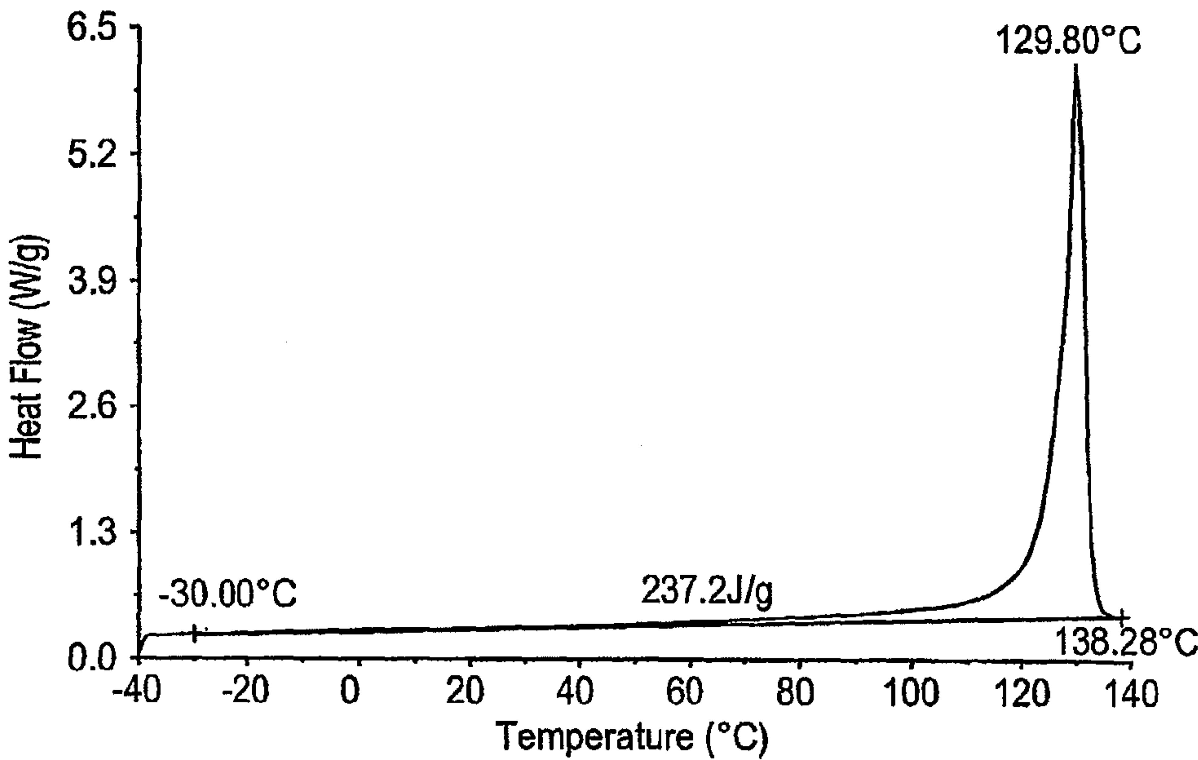
FIG. 23 DSC Comparative B*
