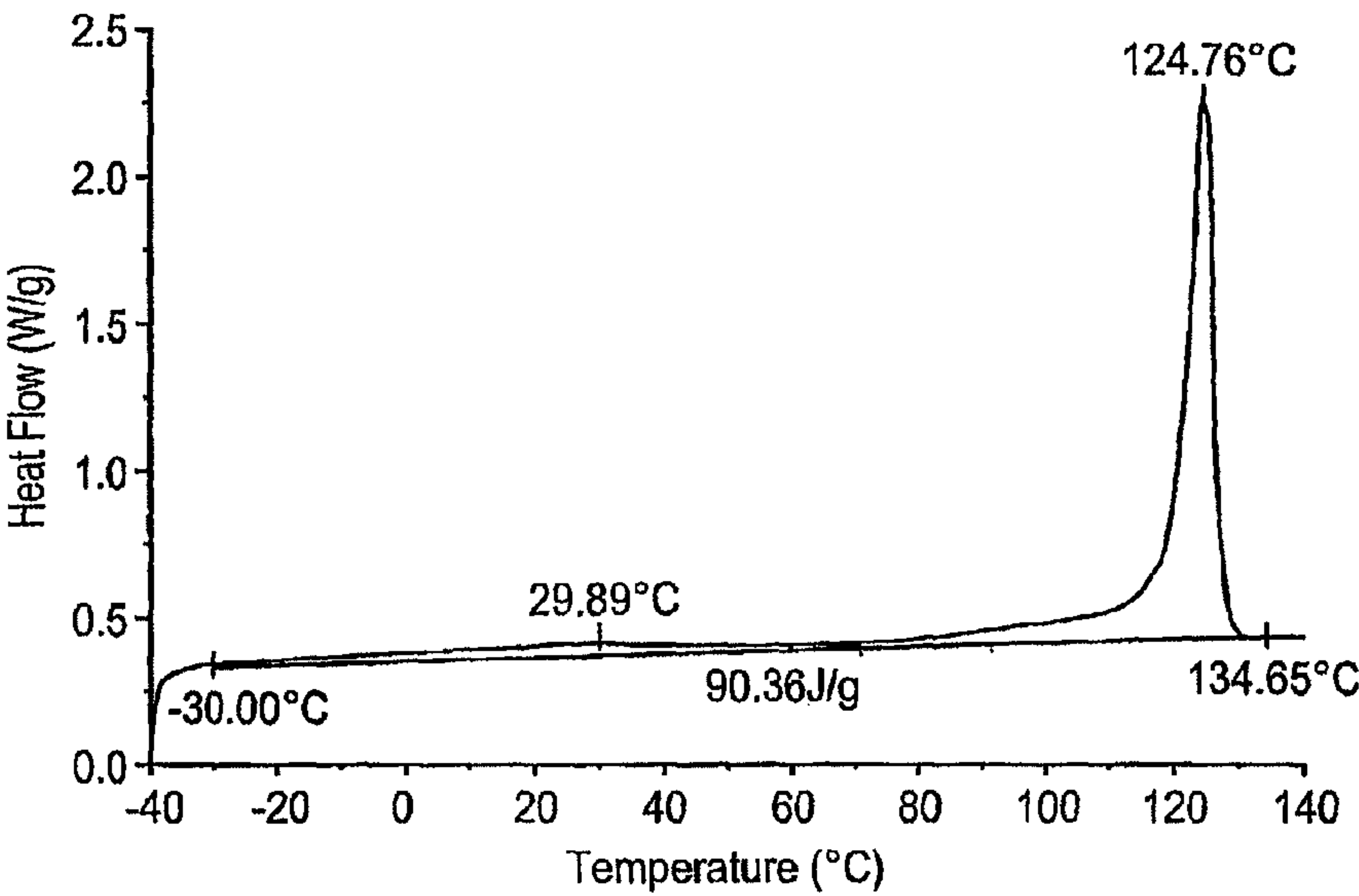
FIG. 27 DSC Comparative F*
