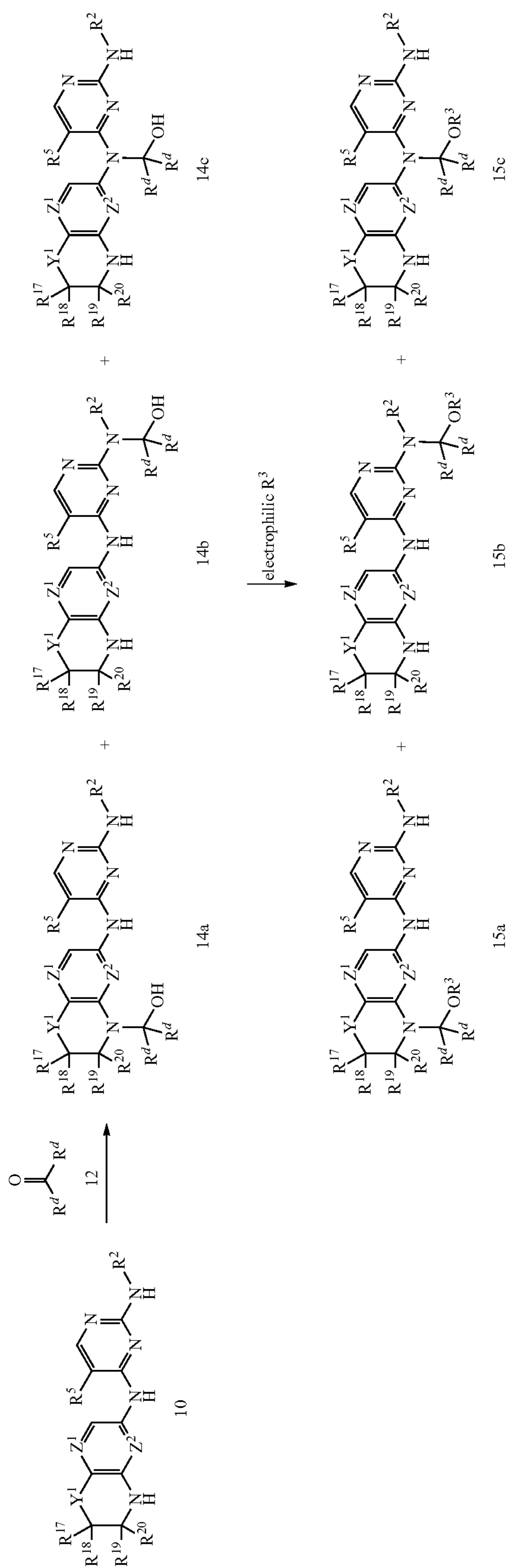
Scheme (I)
