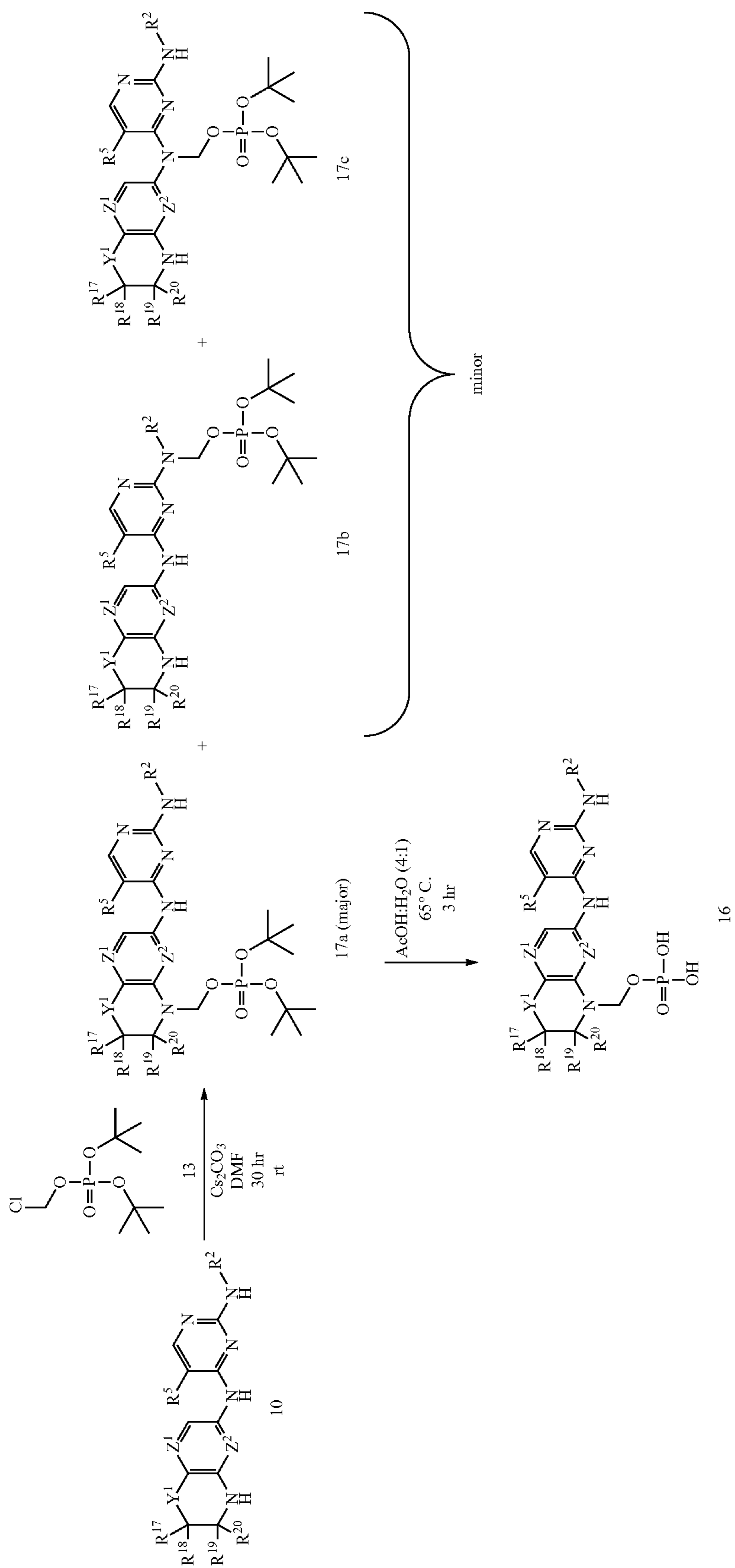
Scheme (V)
