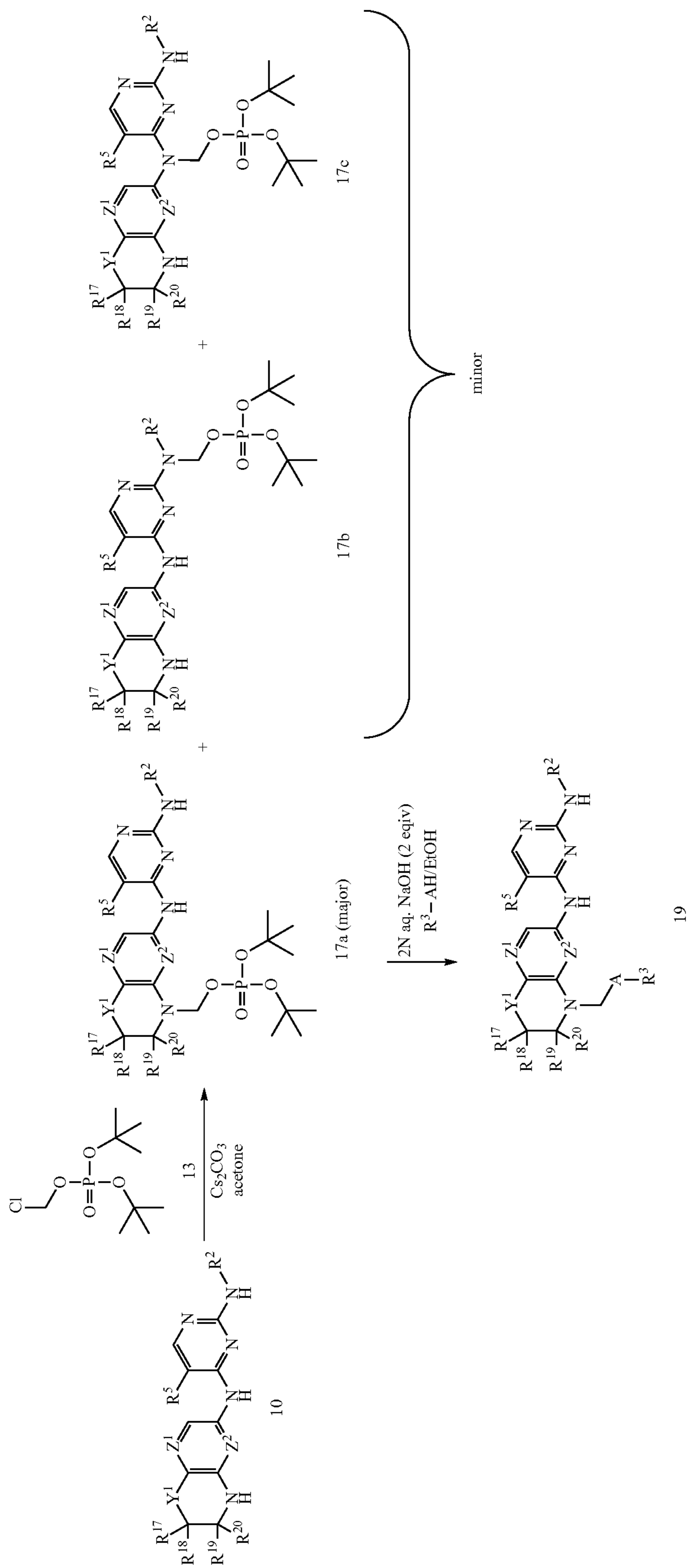
Scheme II
