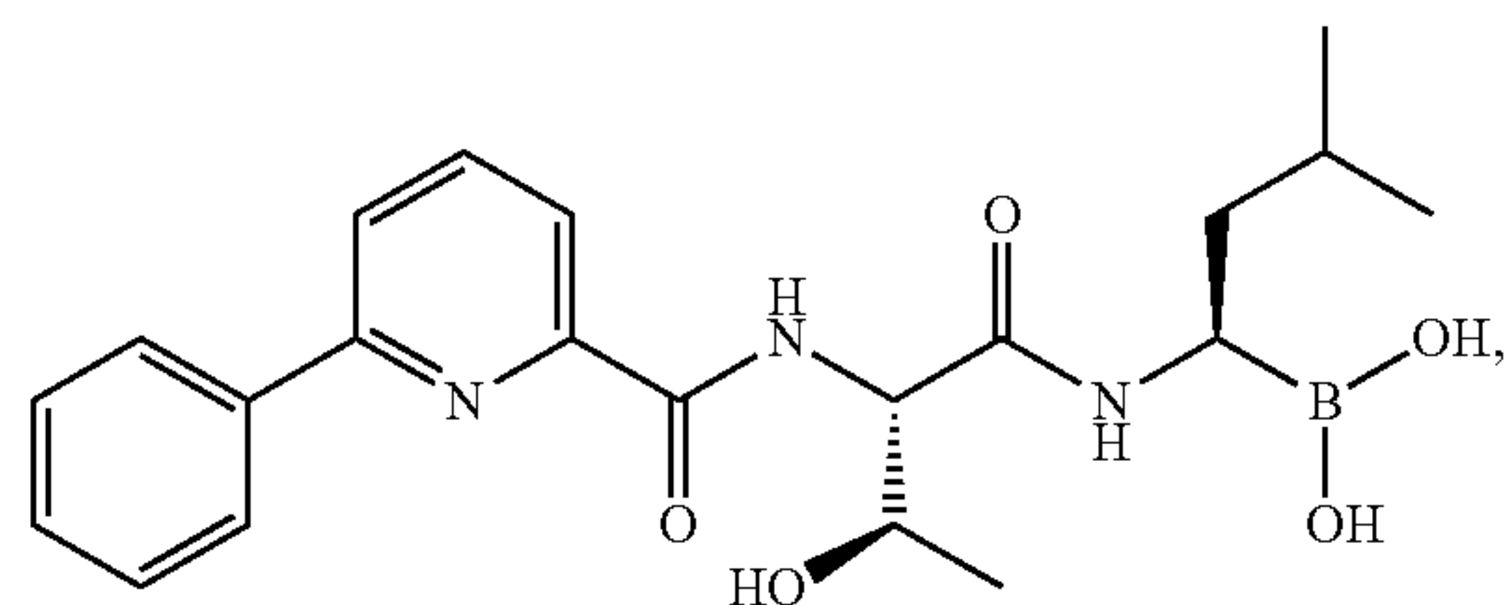
Compound 1
