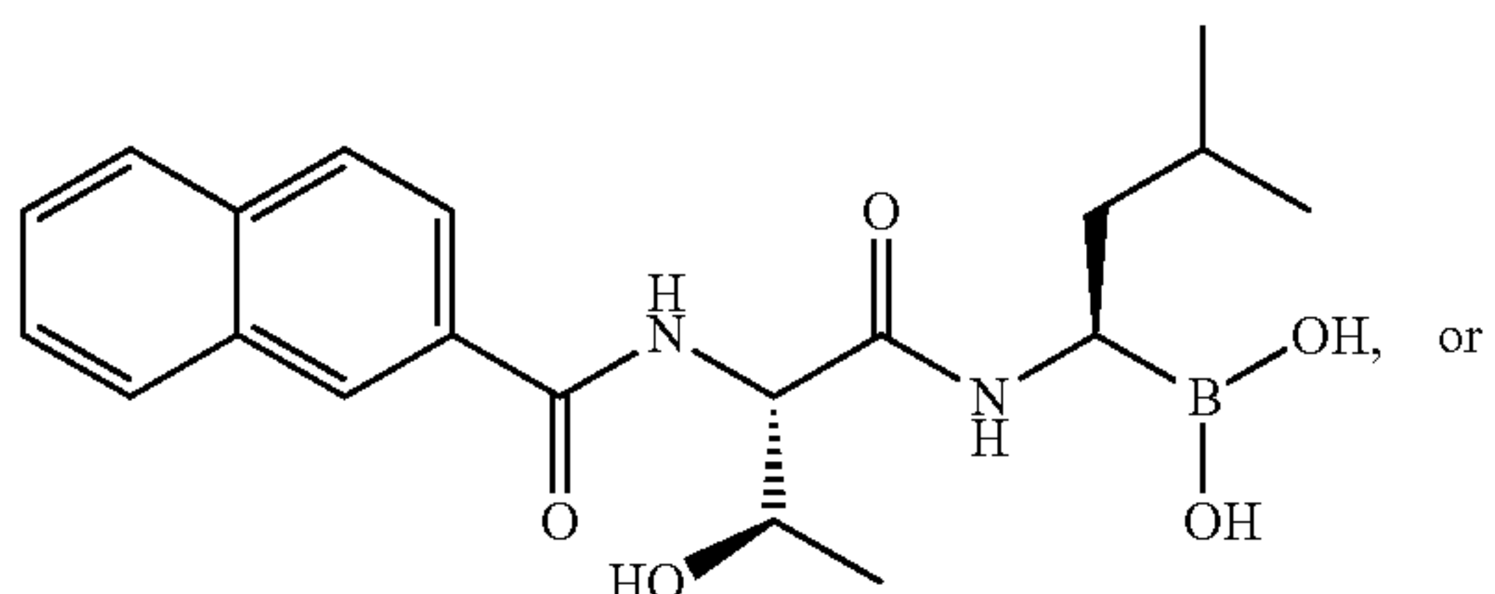
Compound 9
