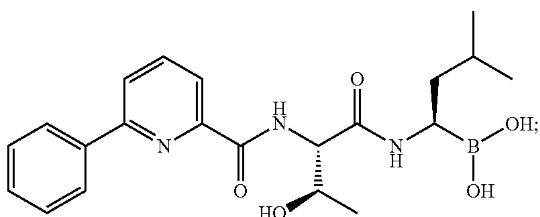
Compound 1
