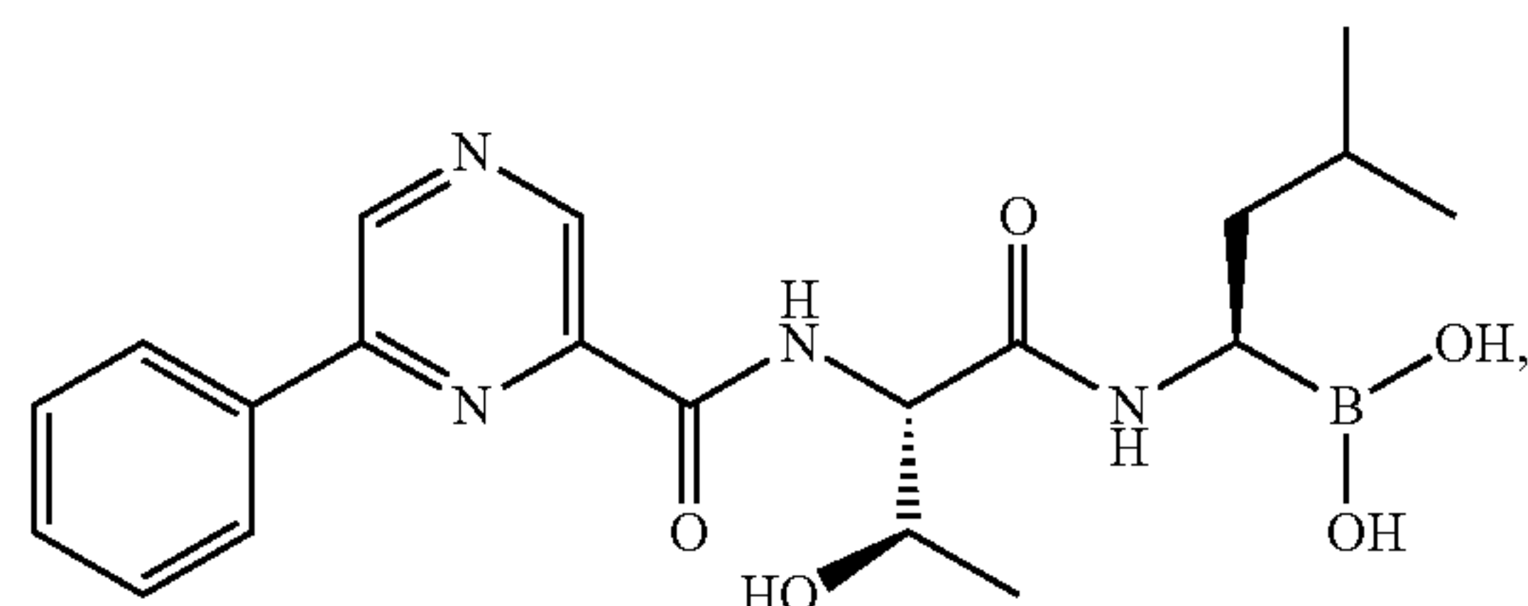
Compound 4
