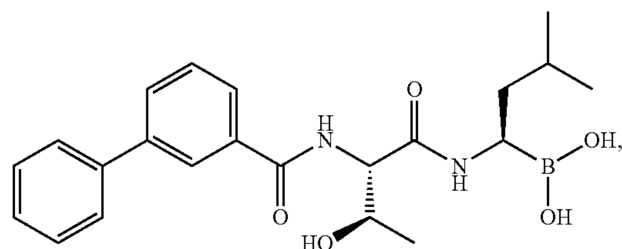
Compound 2
