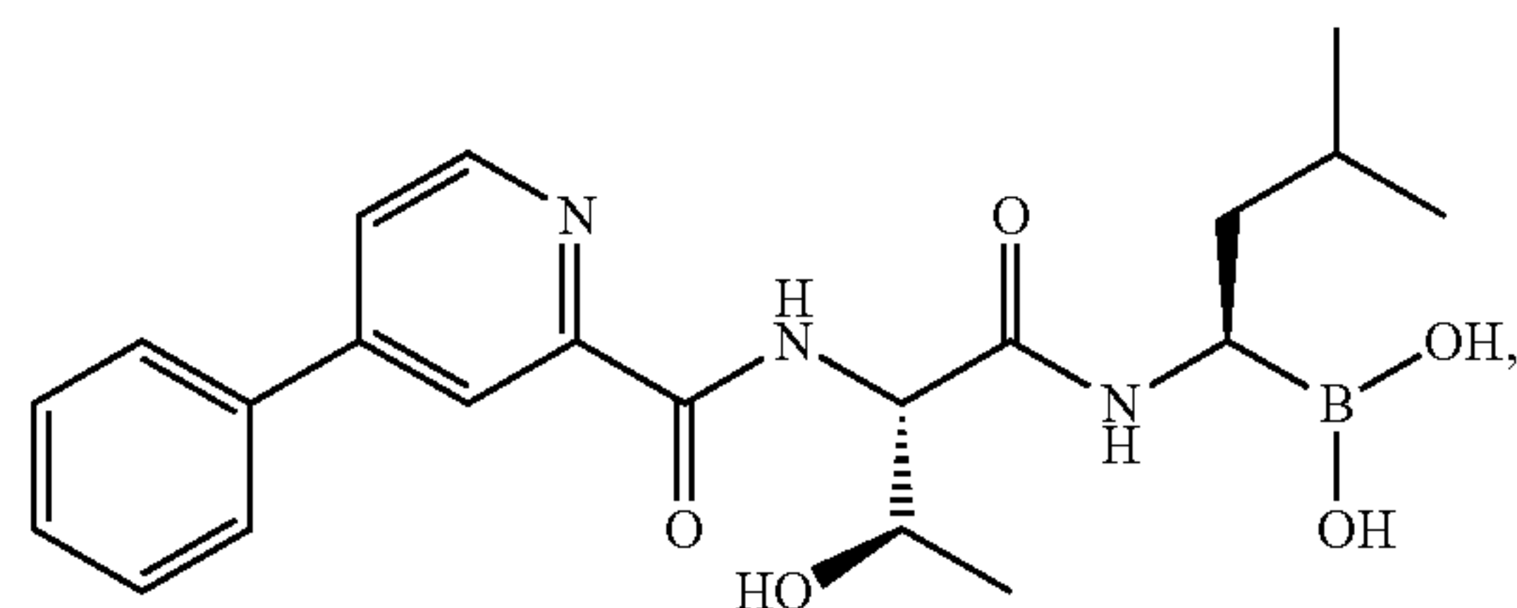
Compound 3
