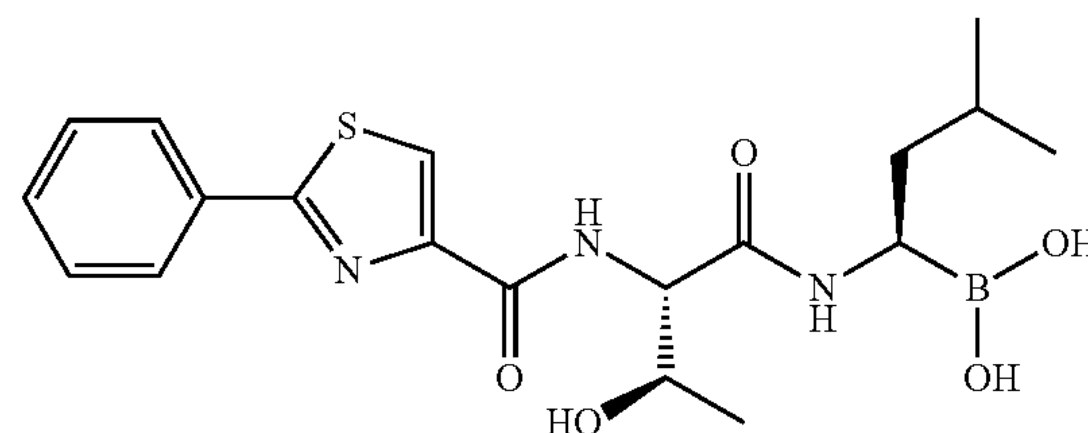
Compound 5
