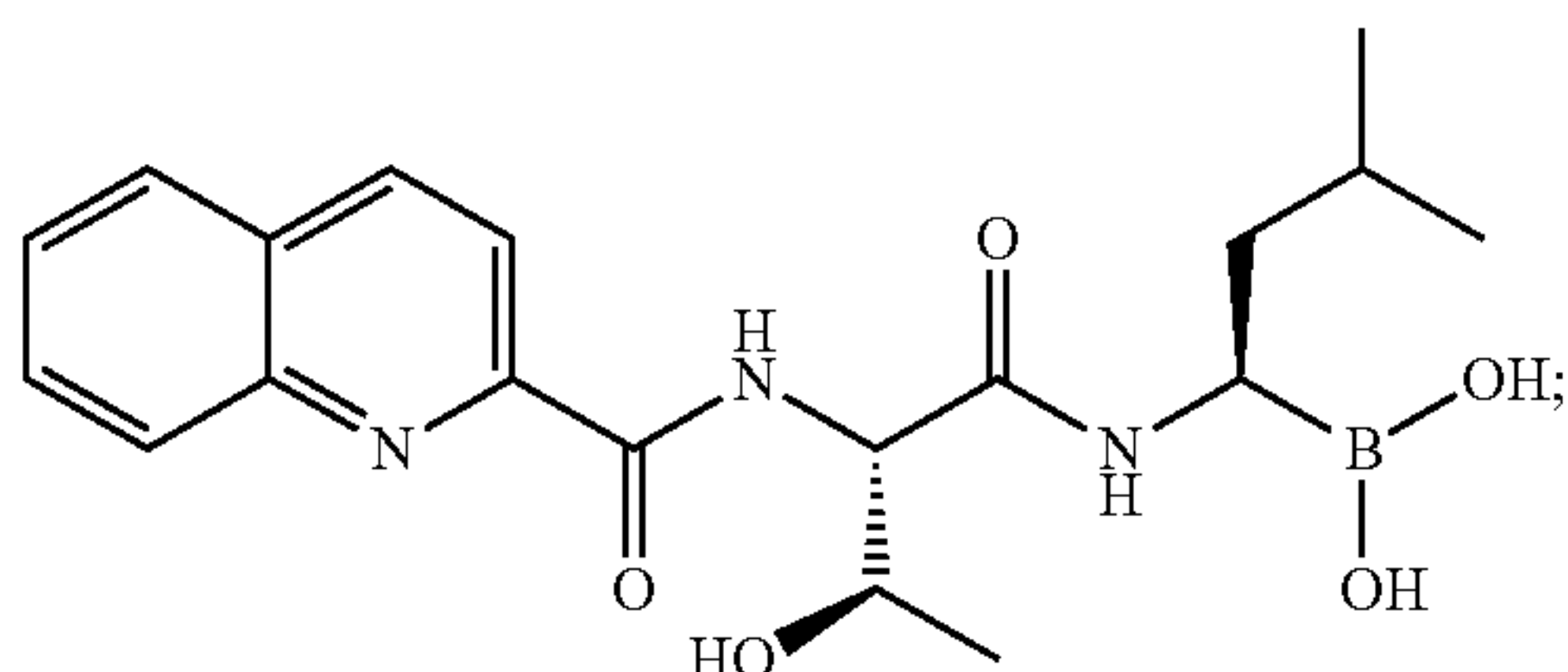
Compound 9
