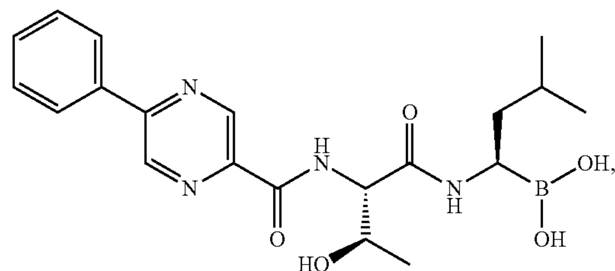
Compound 6
