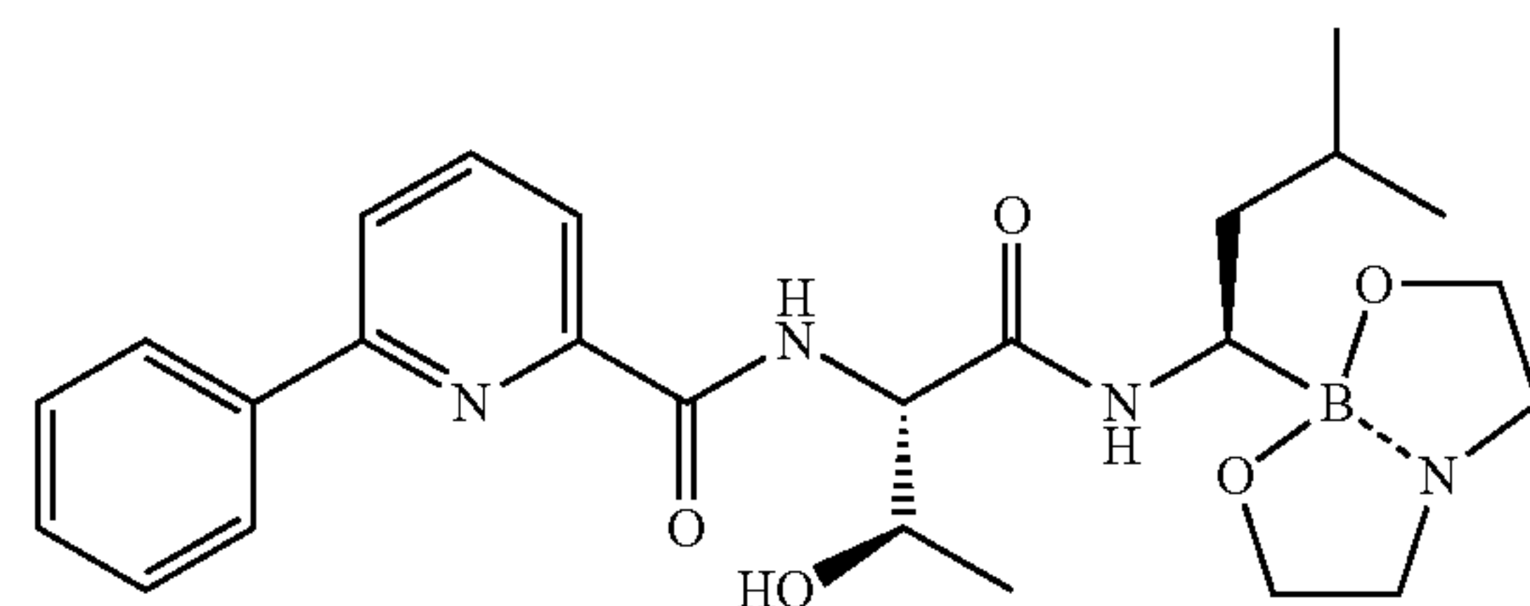
Compound 10
