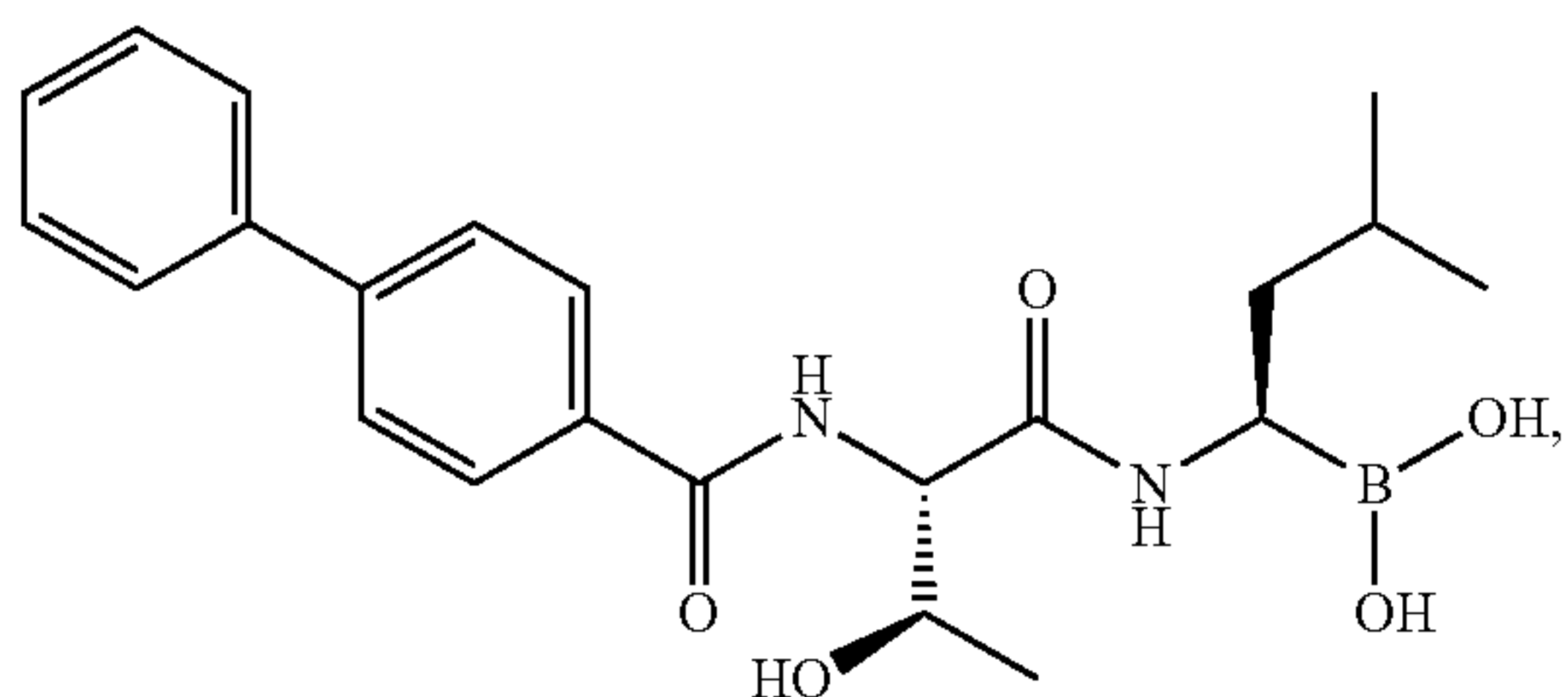
Compound 8
