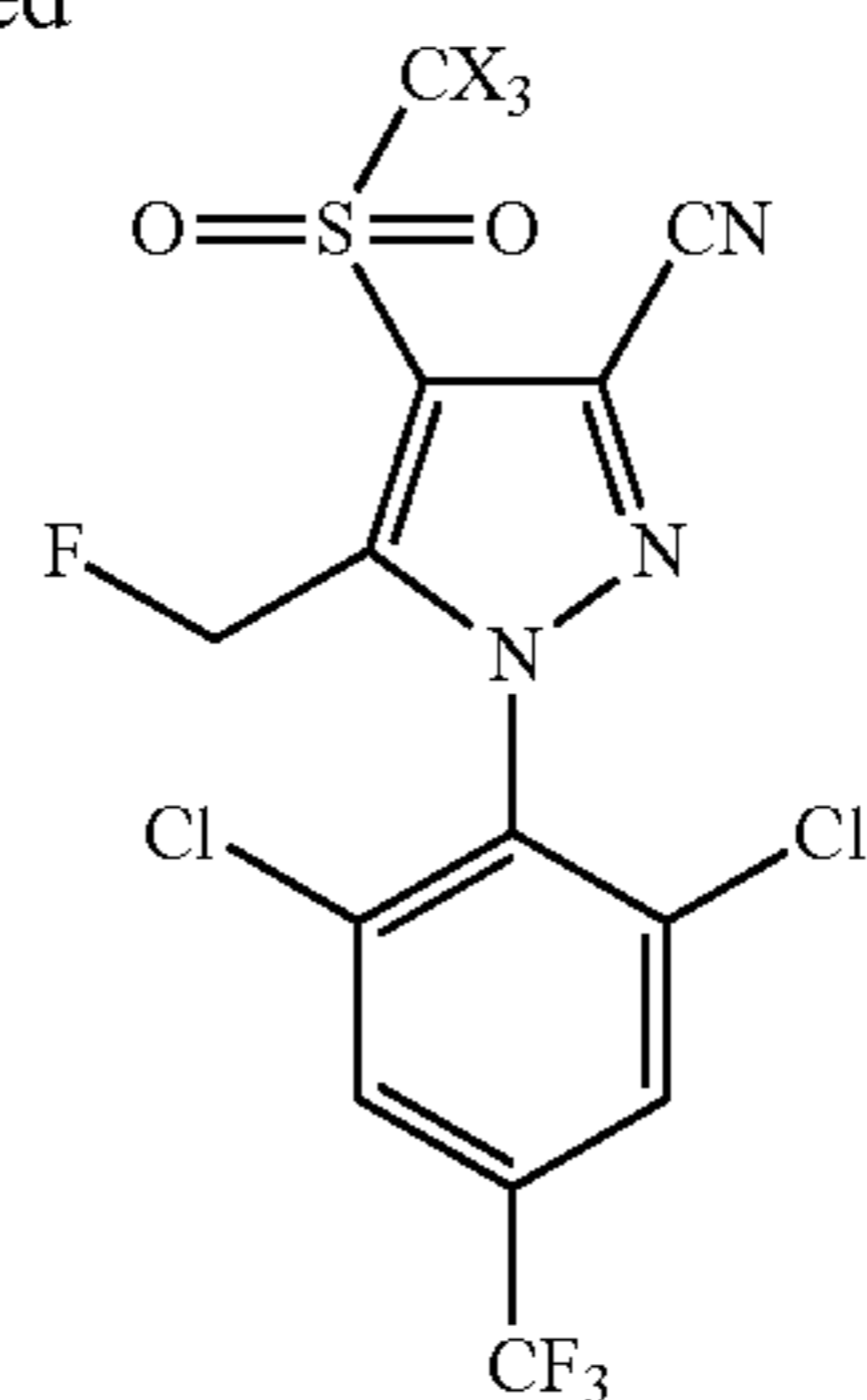
Example 43, CX 3 = CFCl 2
