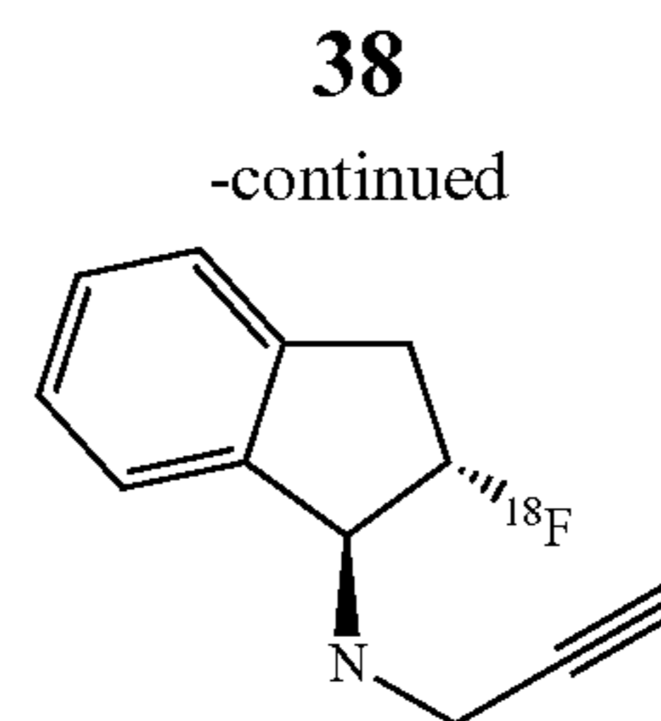
(1S,2S)-2-( 18 F)fluoro-N-(prop-2-yn-1-yl)-2,3-dihydro-1H-inden-1-amine
