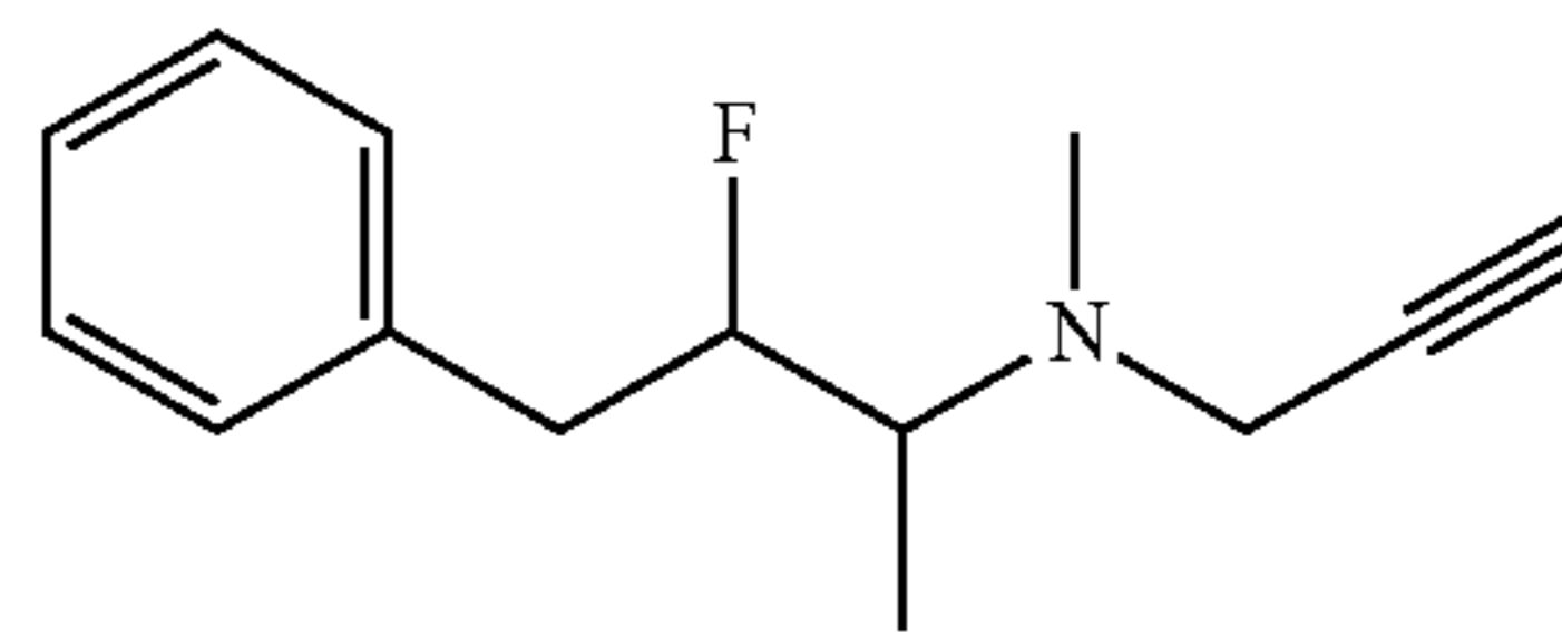
(2-Fluoro-1-methyl-3-phenyl-propyl)-methyl-prop-2-ynyl-amine
