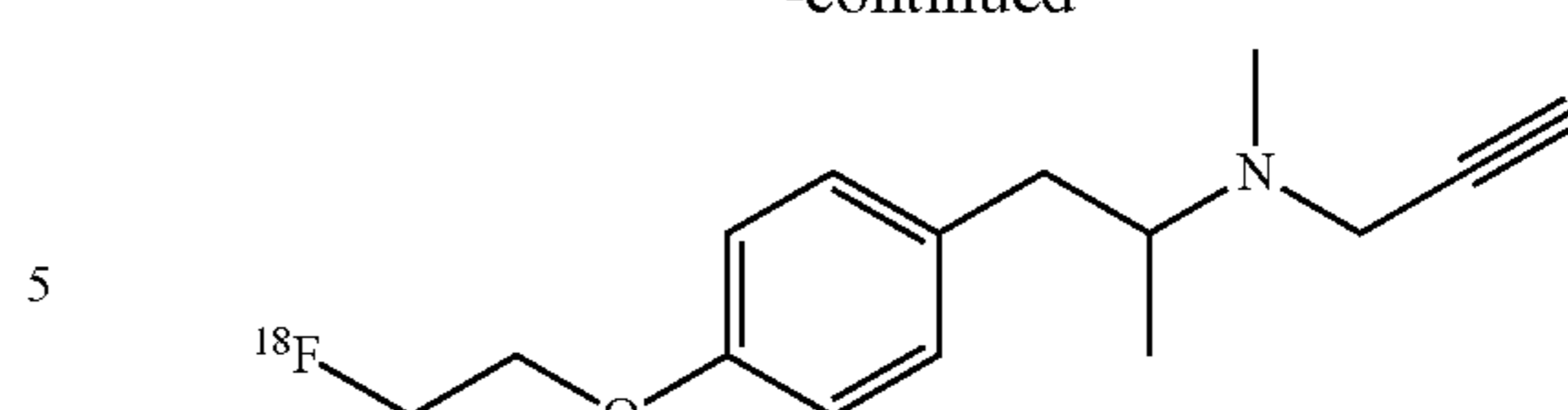
[F-18]-{2-[4-(2-Fluoro-ethoxy)-phenyl]-1-methyl-ethyl}-methyl-prop-2-ynyl-amine
