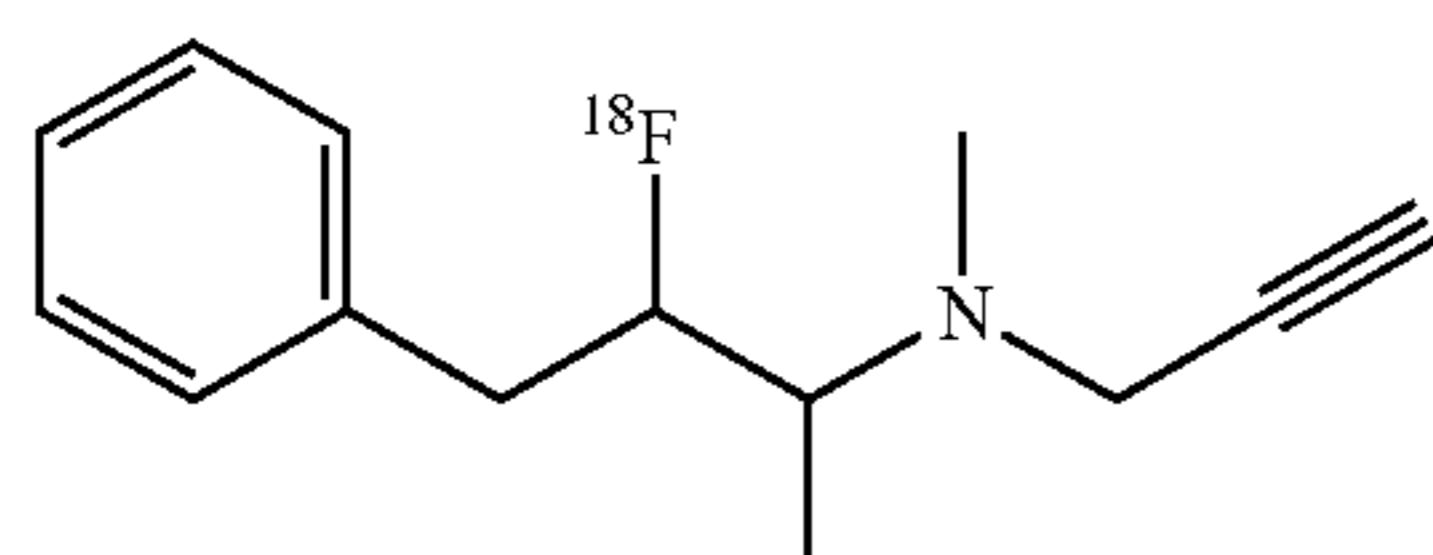
[F-18]-(2-Fluoro-1-methyl-3-phenyl-propyl)-methyl-prop-2-ynyl-amine
