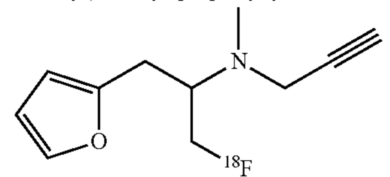
[F-18]-(1-Fluoromethyl-2-furan-2-yl-ethyl)-methyl-prop-2-ynyl-amine
