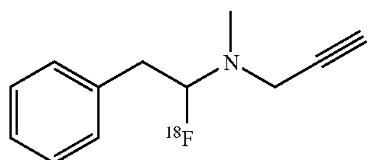
[F-18]-(1-Fluoro-2-phenyl-ethyl)-methyl-prop-2-ynyl-amine
