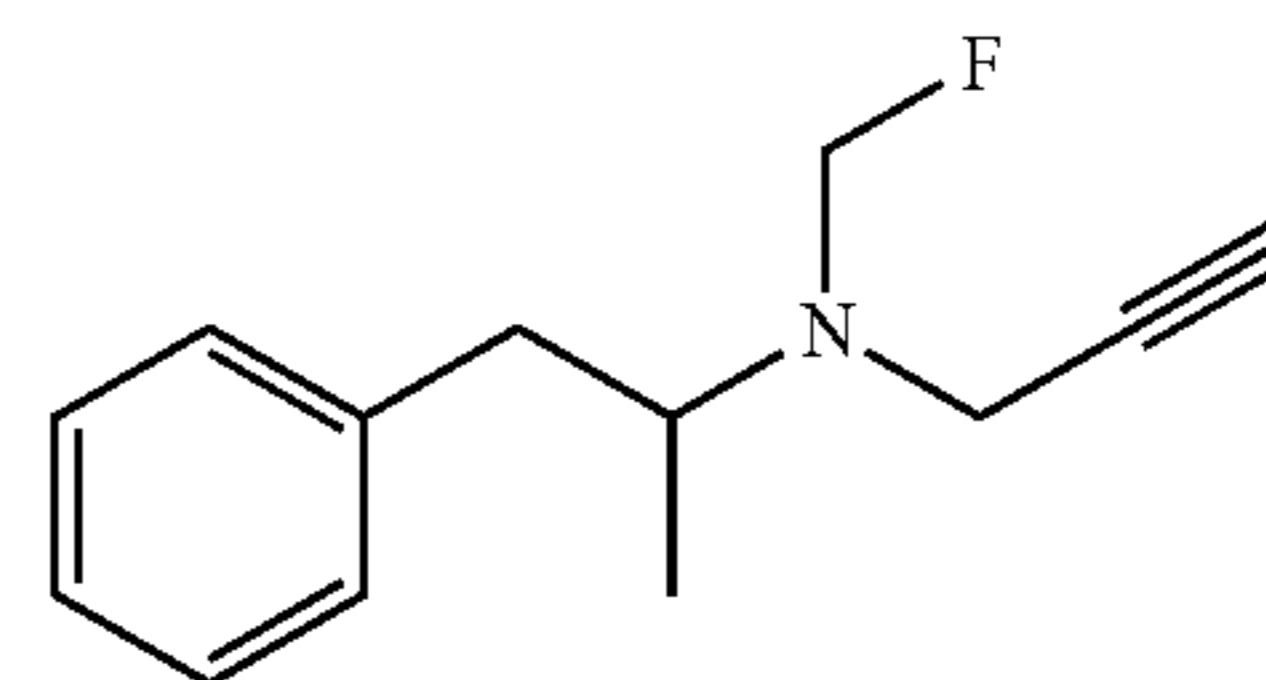
Fluoromethyl-(1-methyl-2-phenylethyl)-prop-2-ynyl-amine
