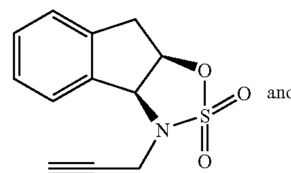
(3aS,8aR)-3-(prop-2-yn-1-yl)-3,3a,8,8a-tetrahydroindeno[1,2-d][1,2,3]oxathiazole 2,2-dioxide
