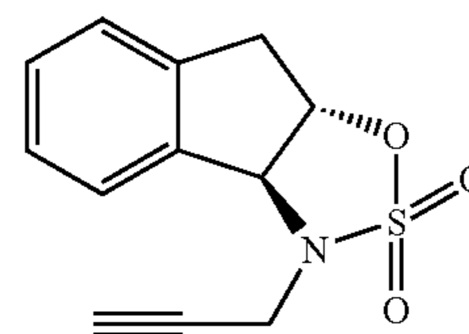
(3aS,8aS)-3-(prop-2-yn-1-yl)-3,3a,8,8a-tetrahydroindeno[1,2-d][1,2,3]oxathiazole 2,2-dioxide
