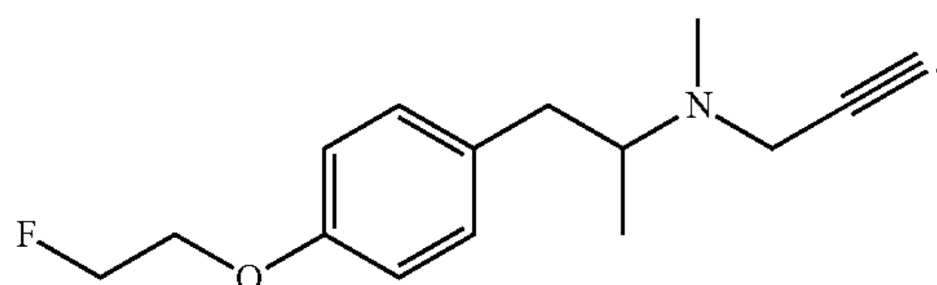
{2-[4-(2-Fluoro-ethoxy)-phenyl]-1-methyl-ethyl}-methyl-prop-2-ynyl-amine
