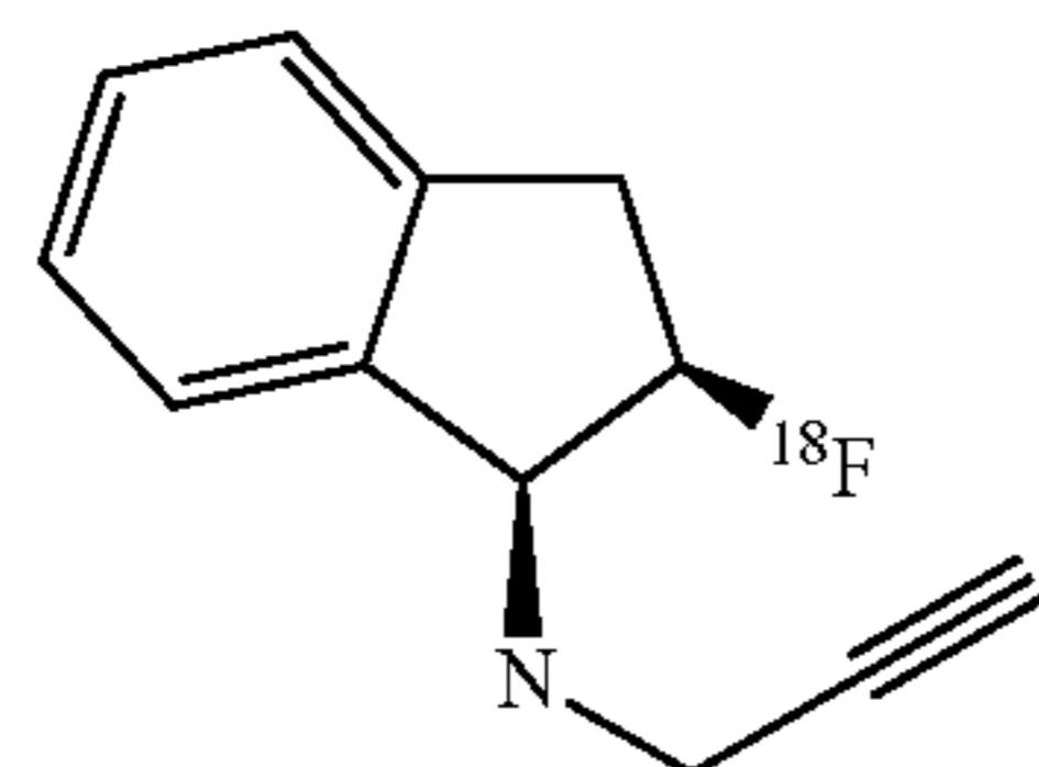
(1S,2R)-2-( 18 F)fluoro-N-(prop-2-yn-1-yl)-2,3-dihydro-1H-inden-1-amine
