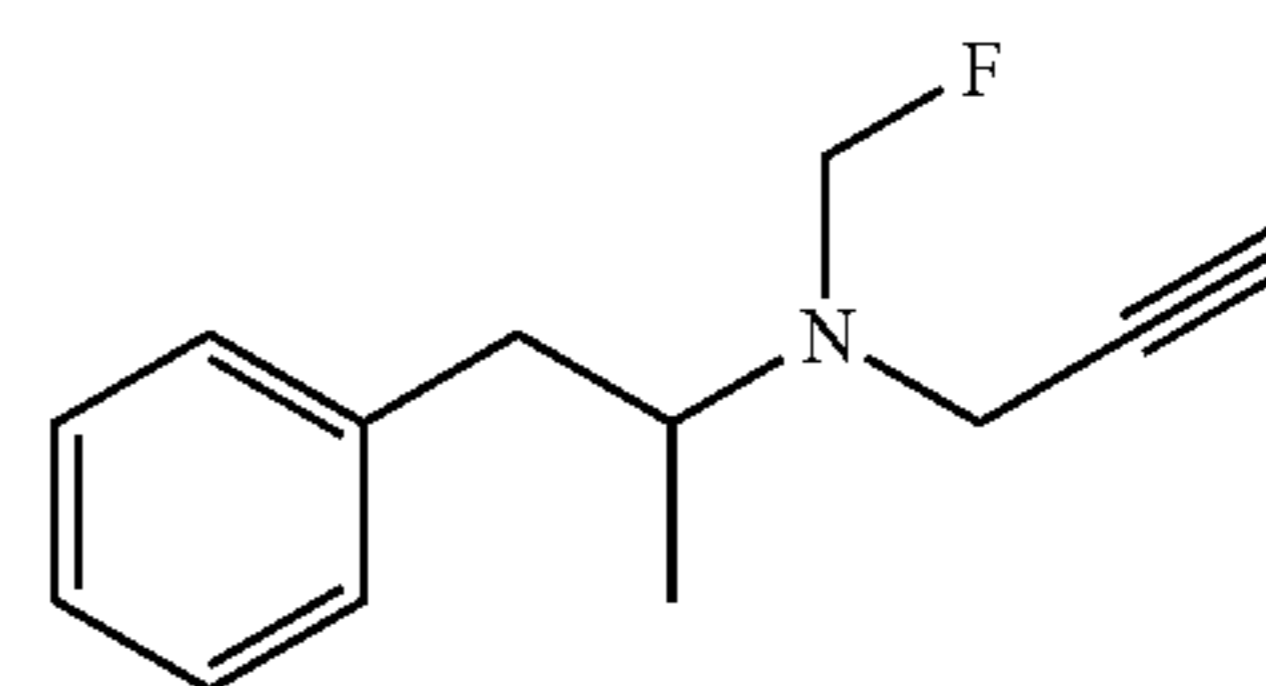
Fluoromethyl-(1-methyl-2-phenylethyl)-prop-2-ynyl-amine
