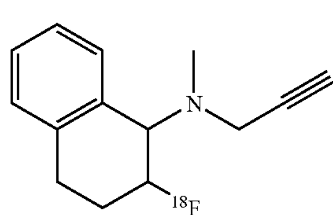
[F-18]-(2-Fluoro-1,2,3,4-tetrahydronaphthalen-1-yl)-methyl-prop-2-ynyl-amine
