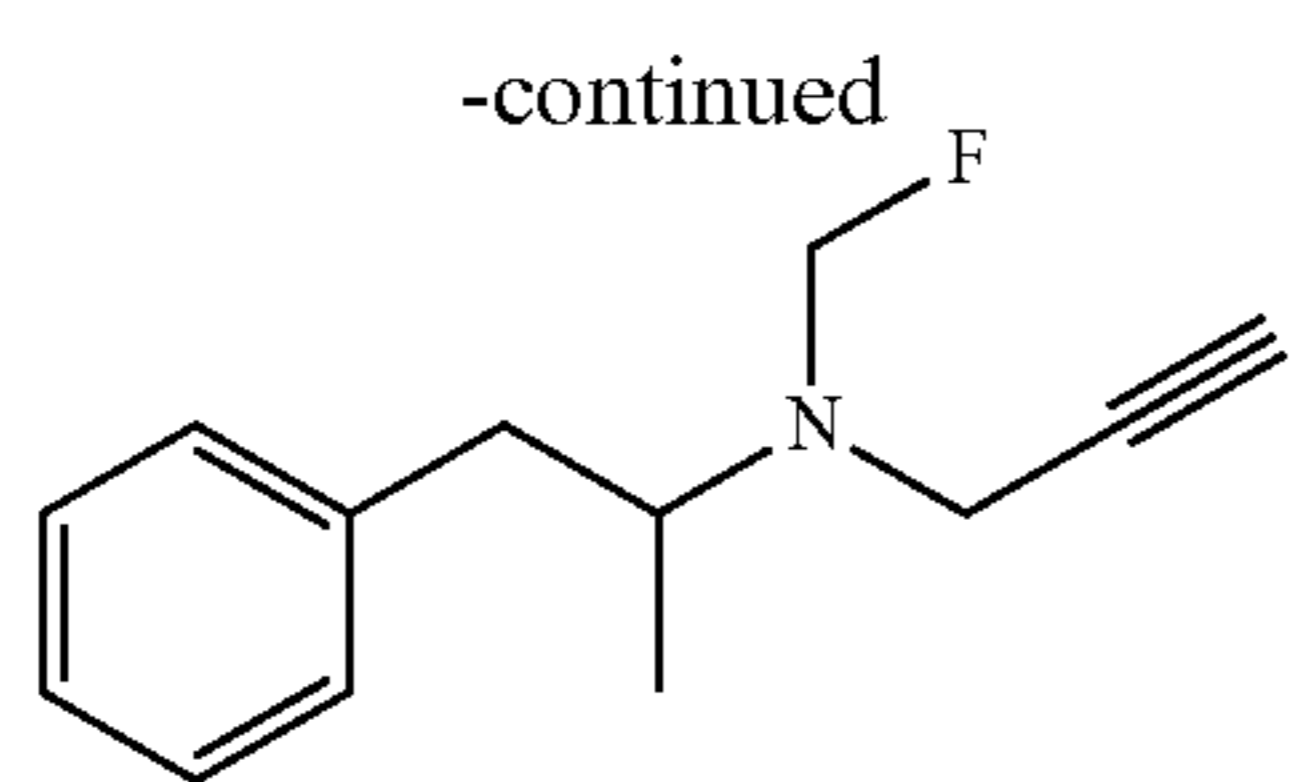
Fluoromethyl-(1-methyl-2-phenyl-ethyl)-prop-2-ynyl-amine
