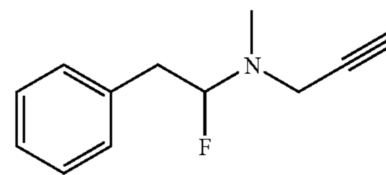
(1-Fluoro-2-phenylethyl)-methyl-prop-2-ynyl-amine
