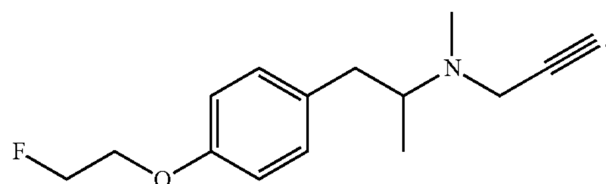
{2-[4-(2-Fluoro-ethoxy)-phenyl]-1-methyl-ethyl}-methyl-prop-2-ynyl-amine
