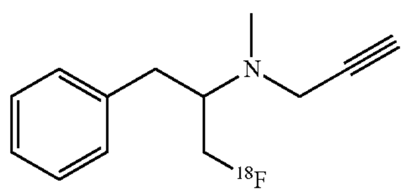
[F-18]-(1-Fluoromethyl-2-phenyl-ethyl)-methyl-prop-2-ynyl-amine
