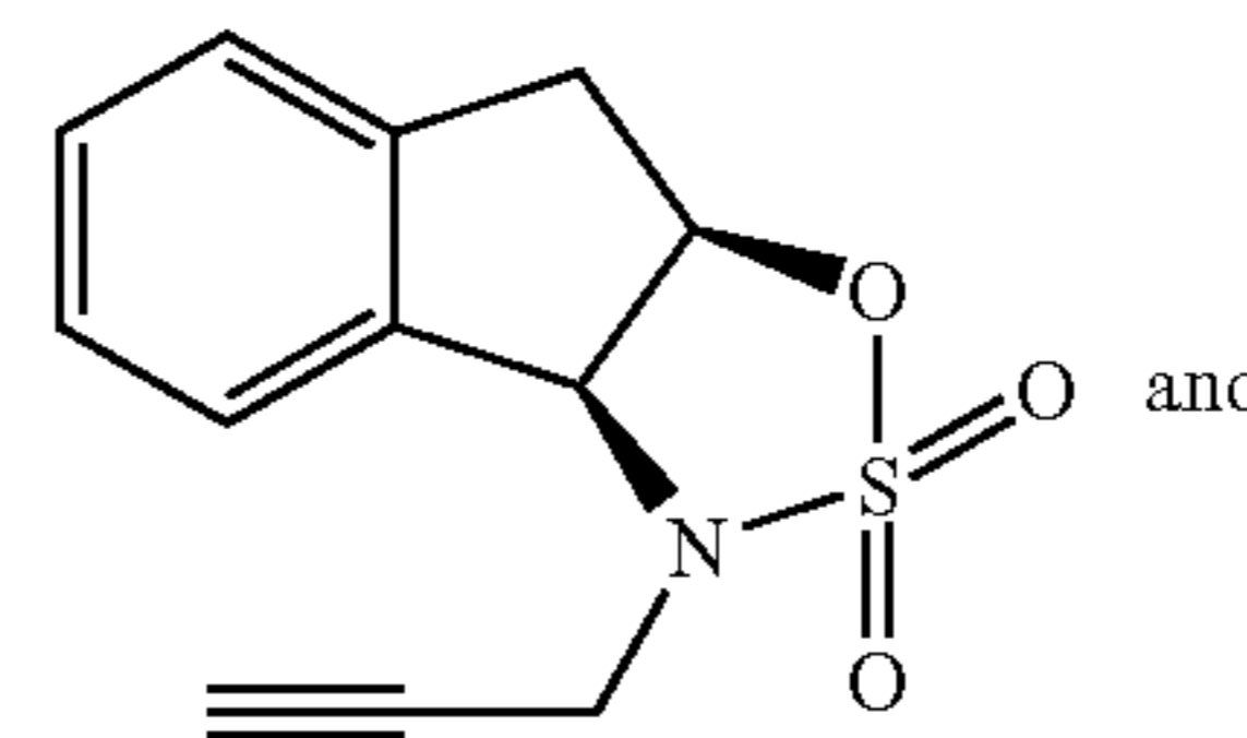
(3aS,8aR)-3-(prop-2-yn-1-yl)-3,3a,8,8a-tetrahydroindeno[1,2-d][1,2,3]oxathiazole 2,2-dioxide
