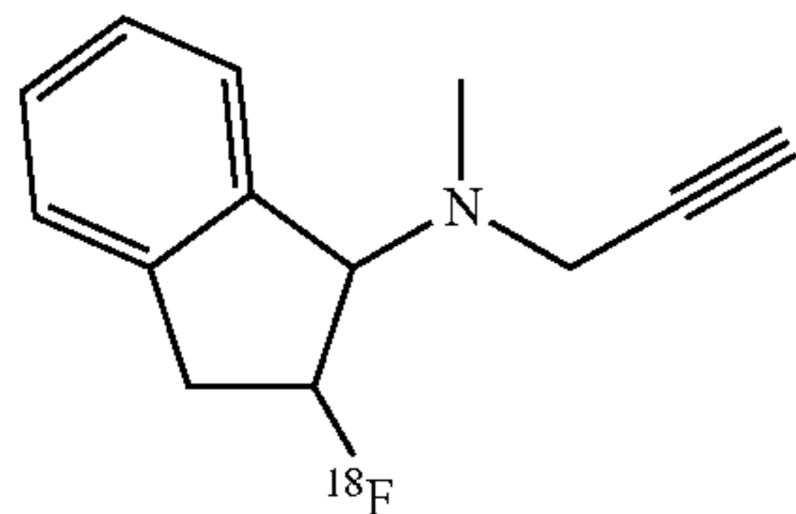
[F-18]-(2-Fluoro-indan-1-yl)-methyl-prop-2-ynyl-amine
