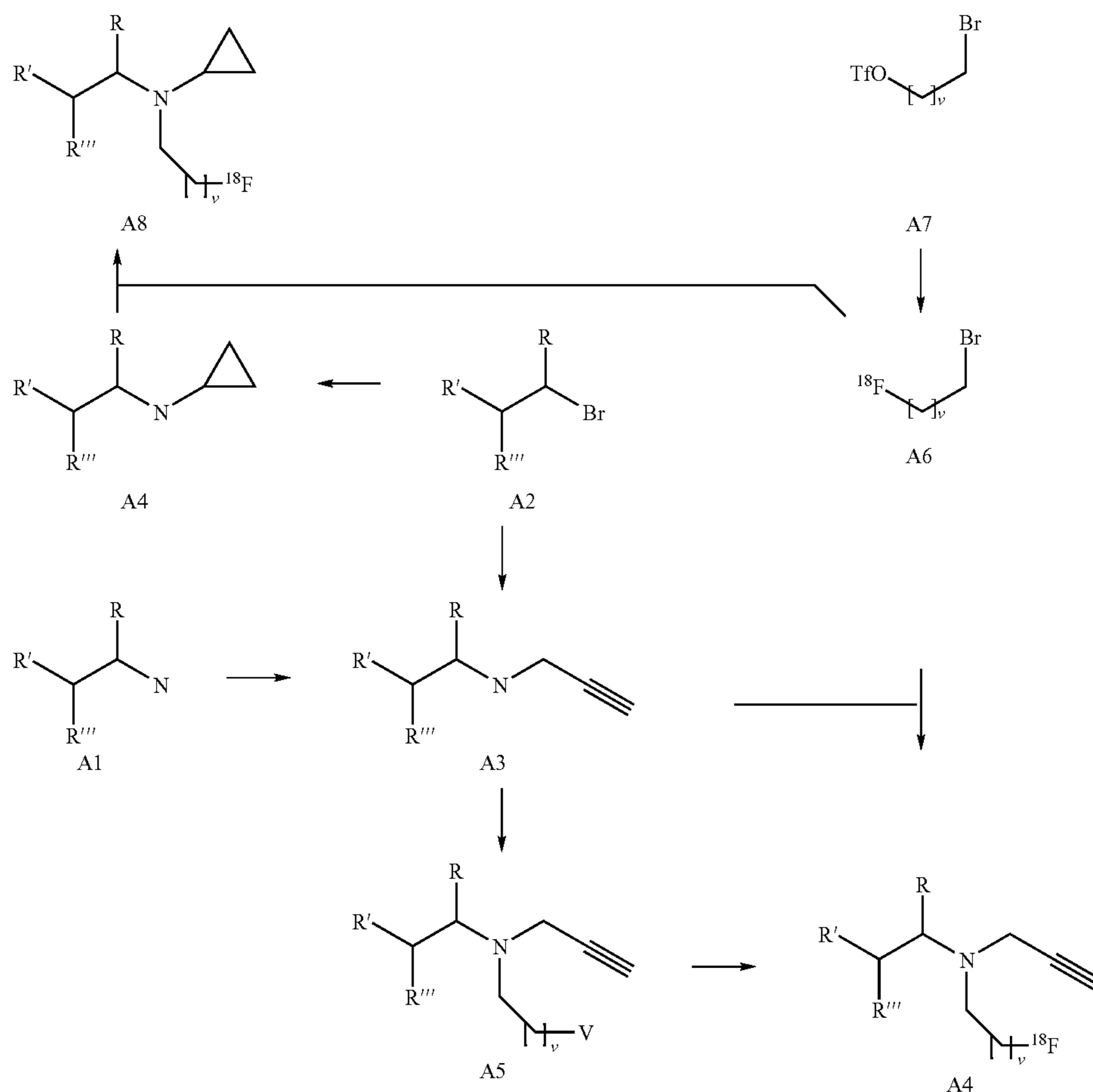
scheme 1
