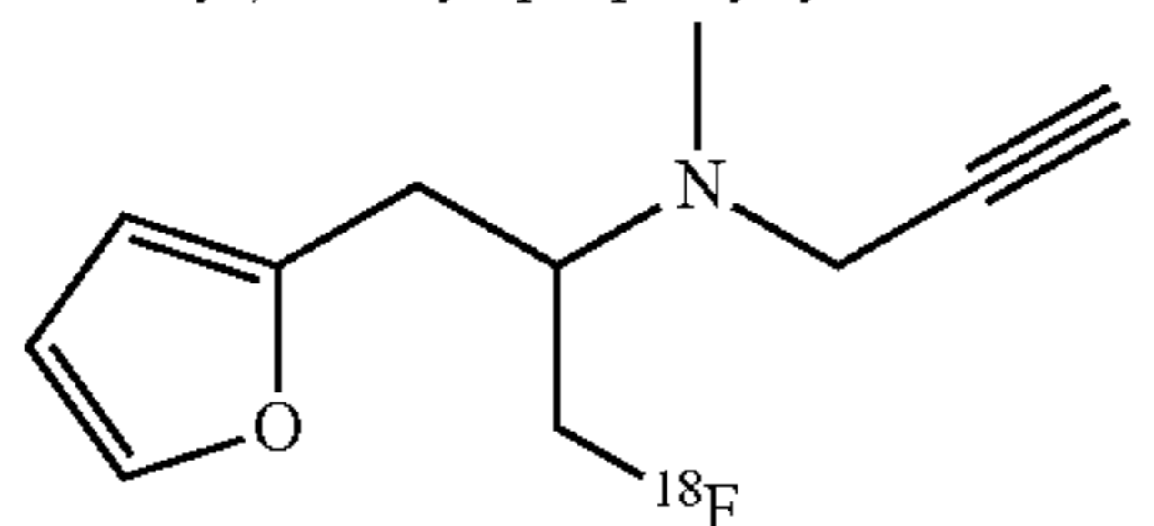
[F-18]-(1-Fluoromethyl-2-furan-2-yl-ethyl)-methyl-prop-2-ynyl-amine
