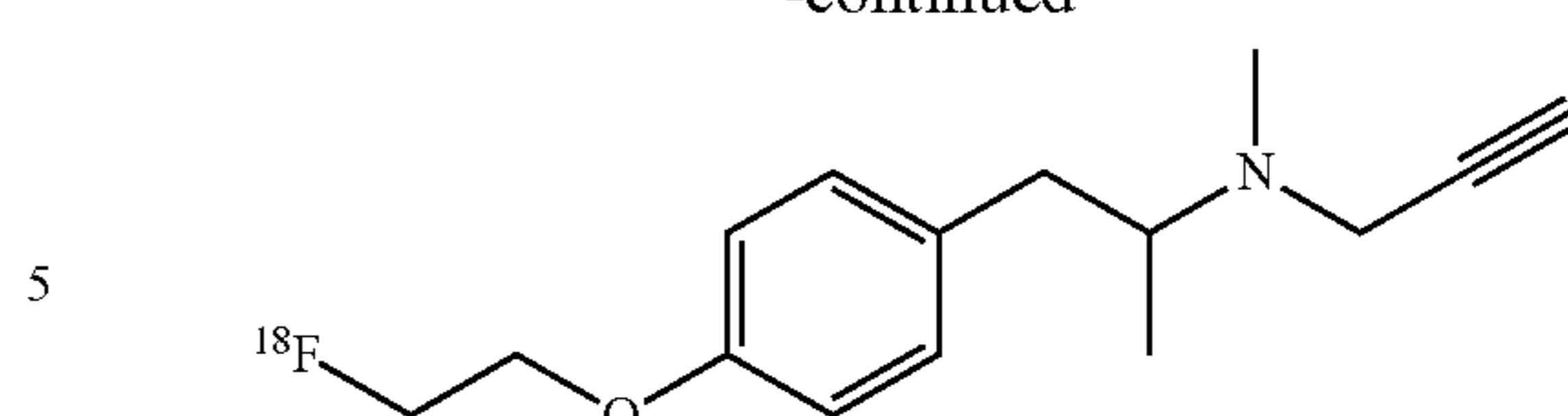
[F-18]-{2-[4-(2-Fluoro-ethoxy)-phenyl]-1-methyl-ethyl}-methyl-prop-2-ynyl-amine
