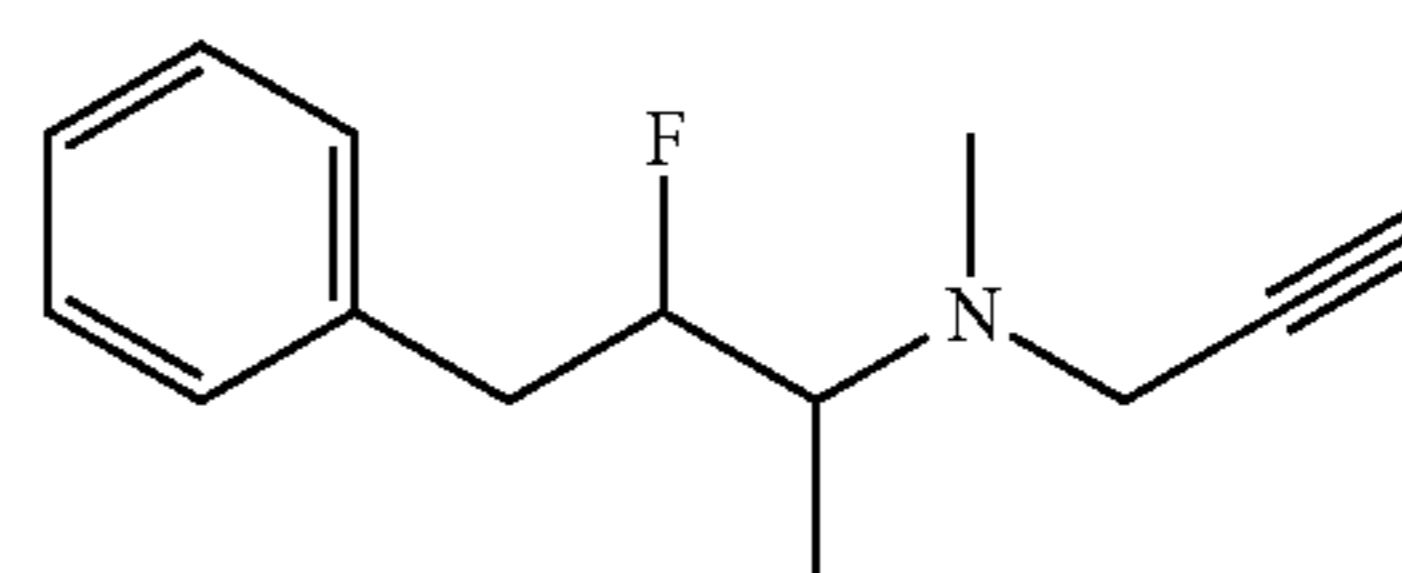
(2-Fluoro-1-methyl-3-phenylpropyl)-methyl-prop-2-ynyl-amine
