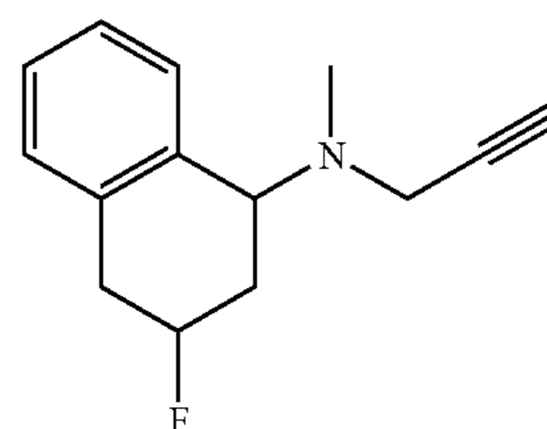
(3-Fluoro-1,2,3,4-tetrahydronaphthalen-1-yl)-methyl-prop-2-ynyl-amine
