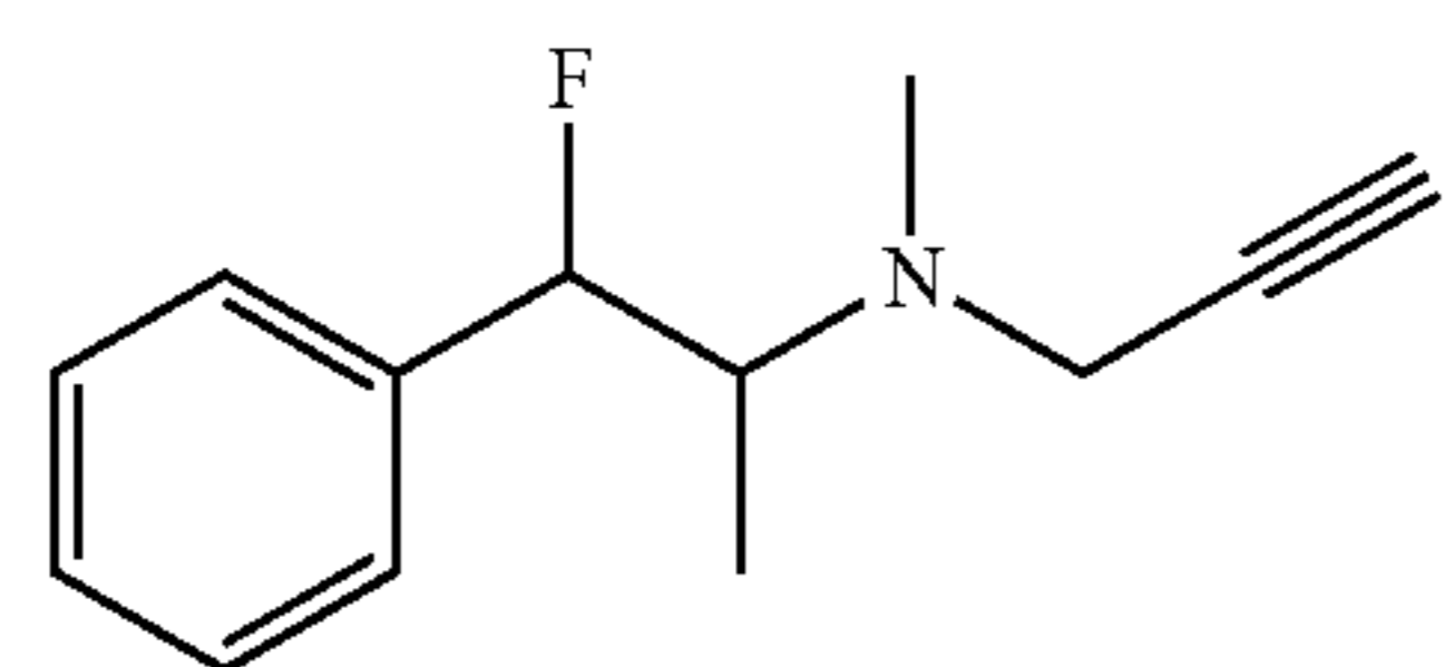
(2-Fluoro-1-methyl-2-phenylethyl)-methyl-prop-2-ynyl-amine
