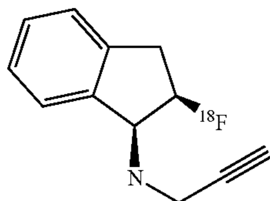
(1S,2R)-2-( 18 F)fluoro-N-(prop-2-yn-1-yl)-2,3-dihydro-1H-inden-1-amine
