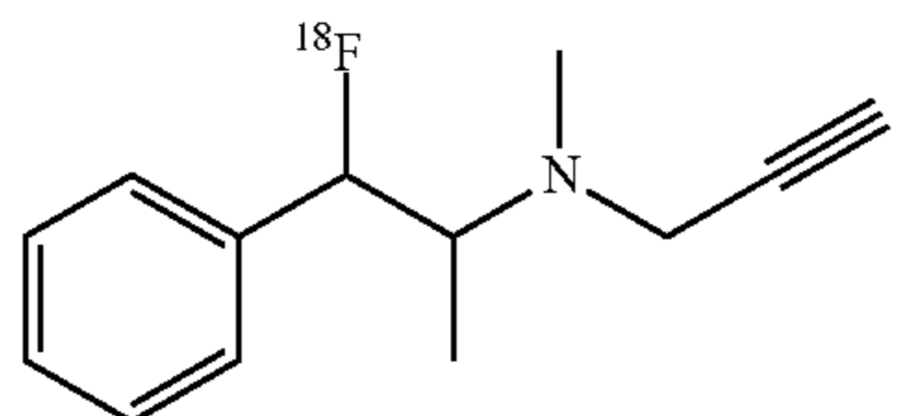
[F-18]-(2-Fluoro-1-methyl-2-phenyl-ethyl)-methyl-prop-2-ynyl-amine
