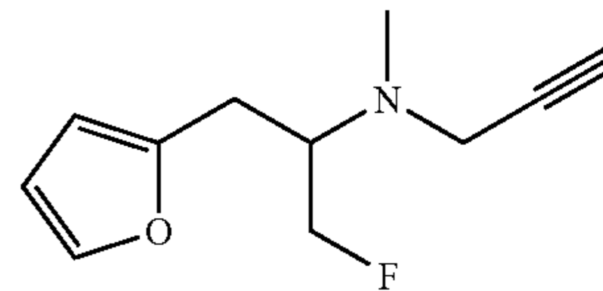
(1-Fluoromethyl-2-furan-2-ylethyl)-methyl-prop-2-ynyl-amine
