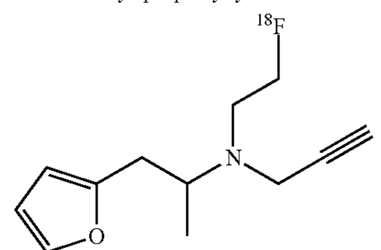
[F-18]-(2-Fluoro-ethyl)-(2-furan-2-yl-1-methyl-ethyl)-prop-2-ynyl-amine
