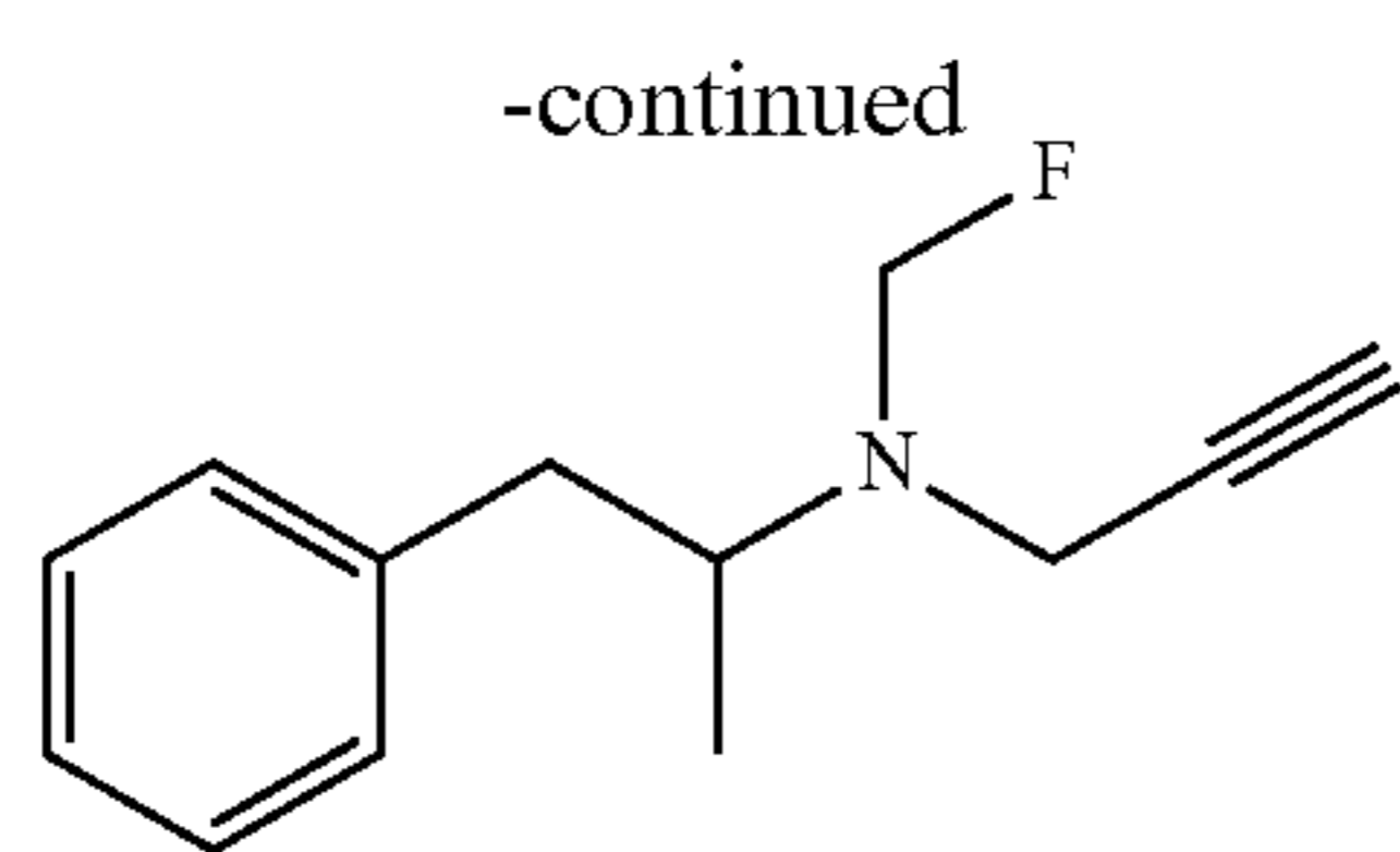
Fluoromethyl-(1-methyl-2-phenyl-ethyl)-prop-2-ynyl-amine
