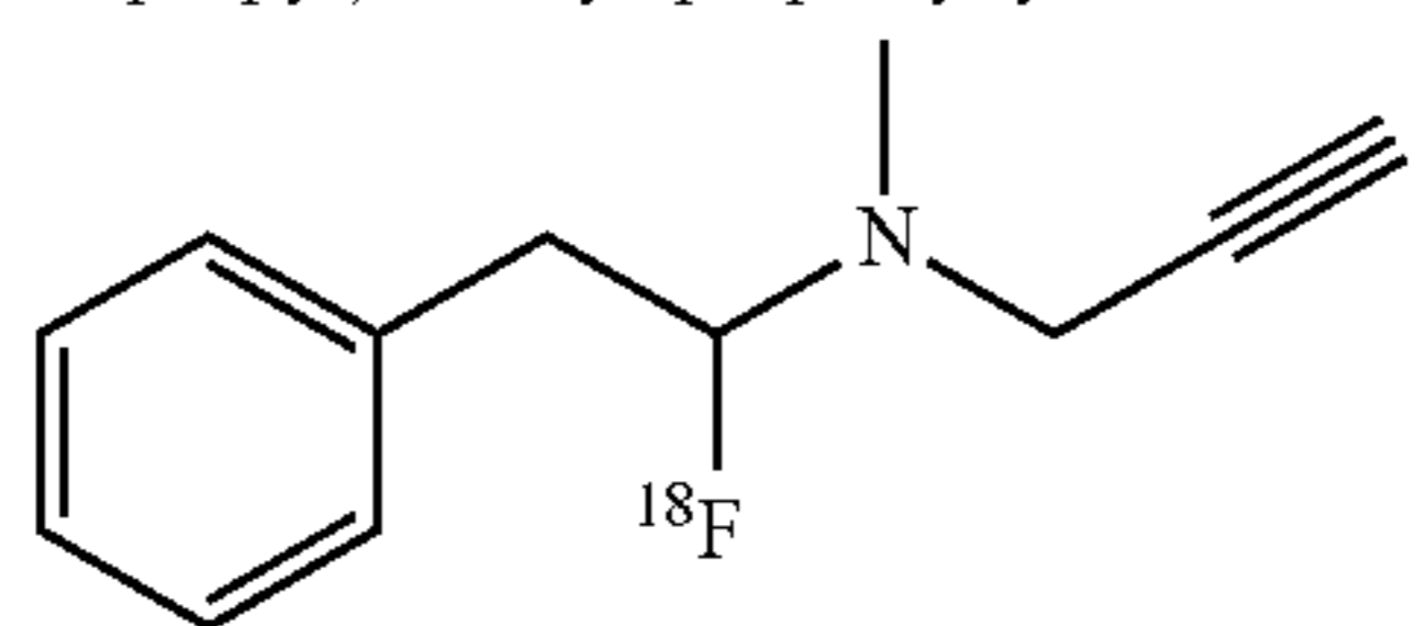
[F-18]-(1-Fluoro-2-phenyl-ethyl)-methyl-prop-2-ynyl-amine
