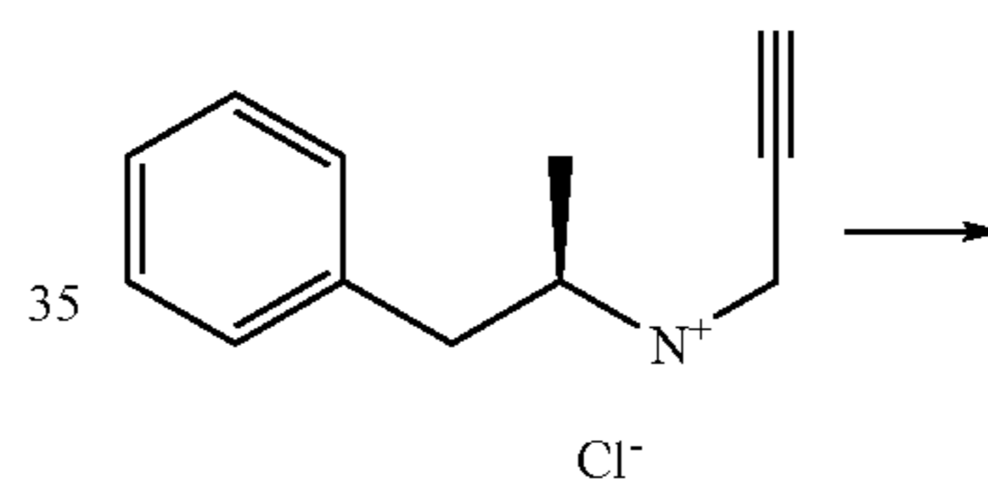
scheme 14
