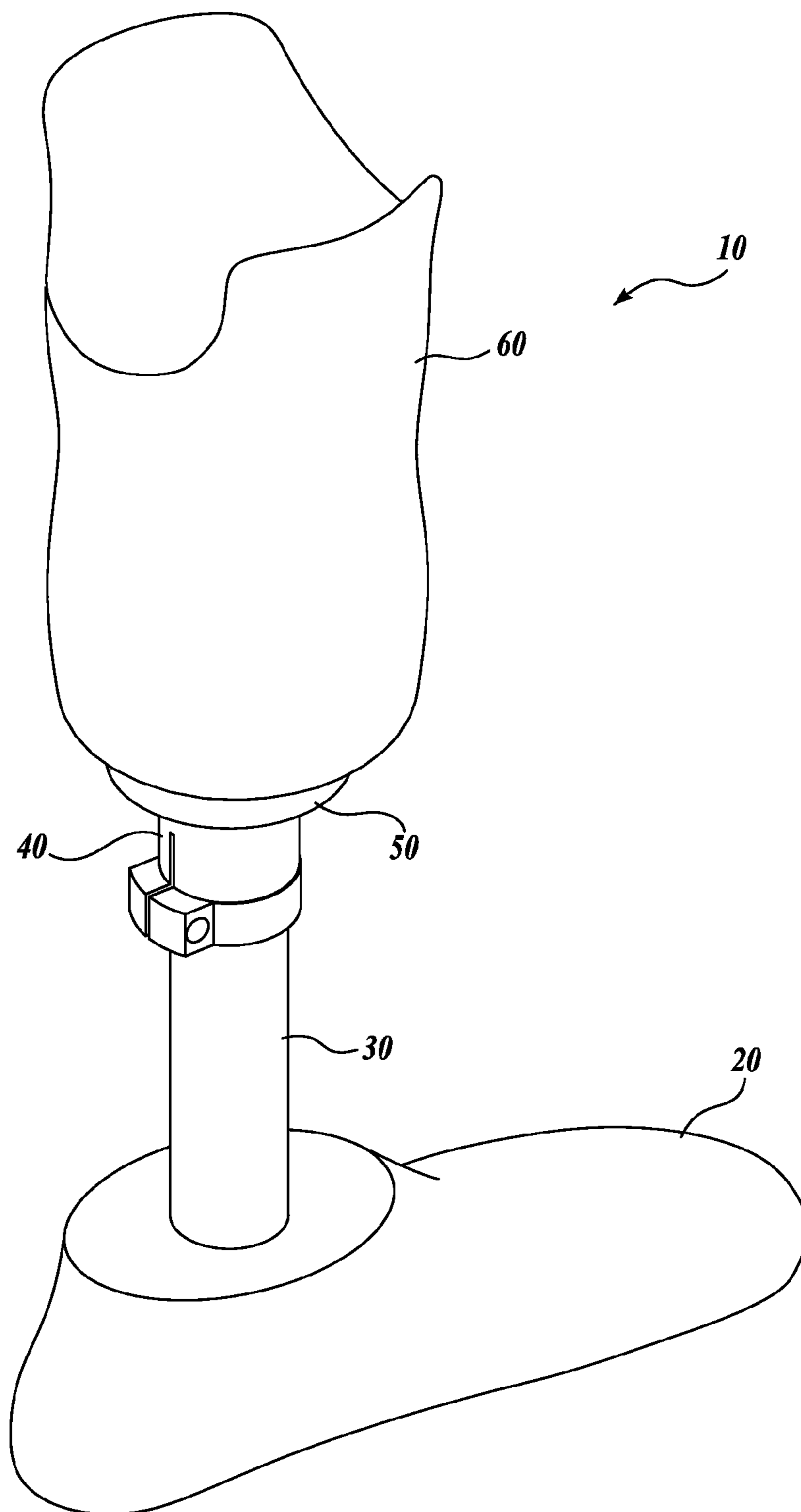
Fig. 1. (PRIOR ART)
