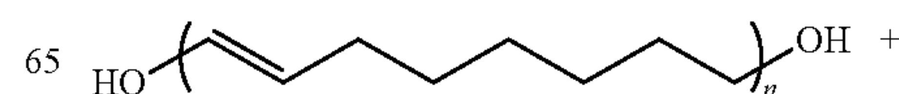
Scheme 3.
