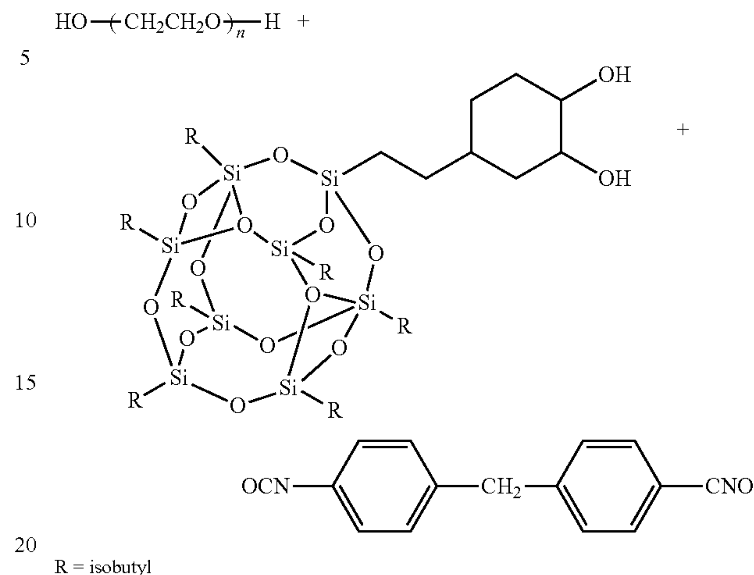
Scheme 1.
