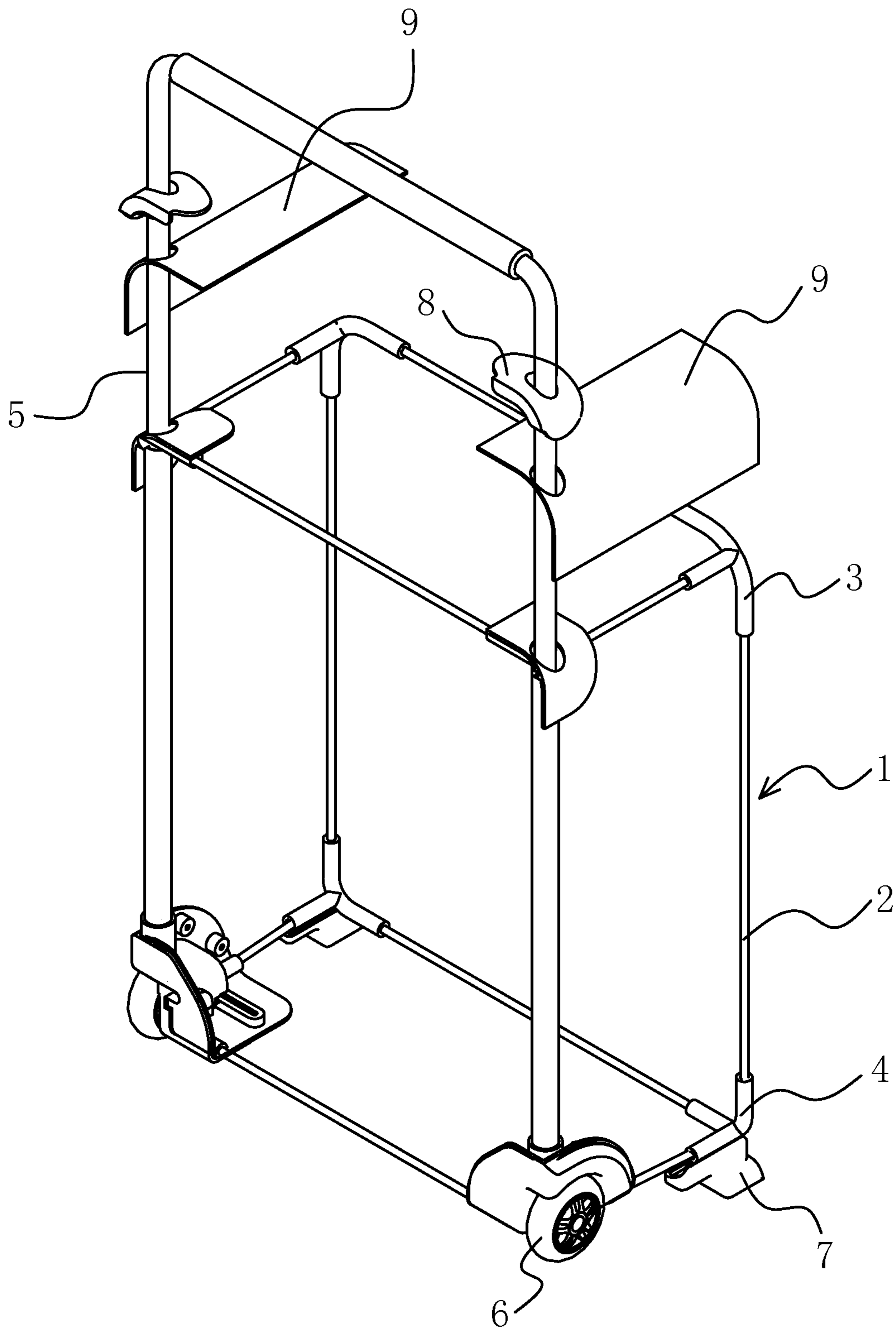
Figure 1 PRIOR ART
