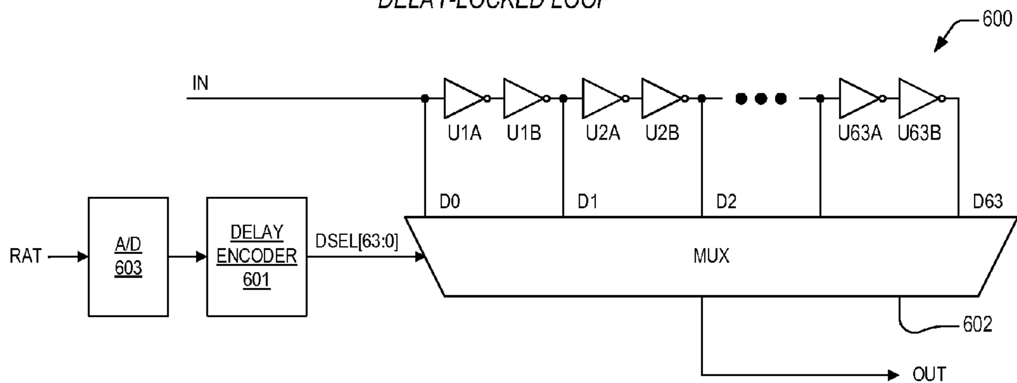
DELAY-LOCKED LOOP
