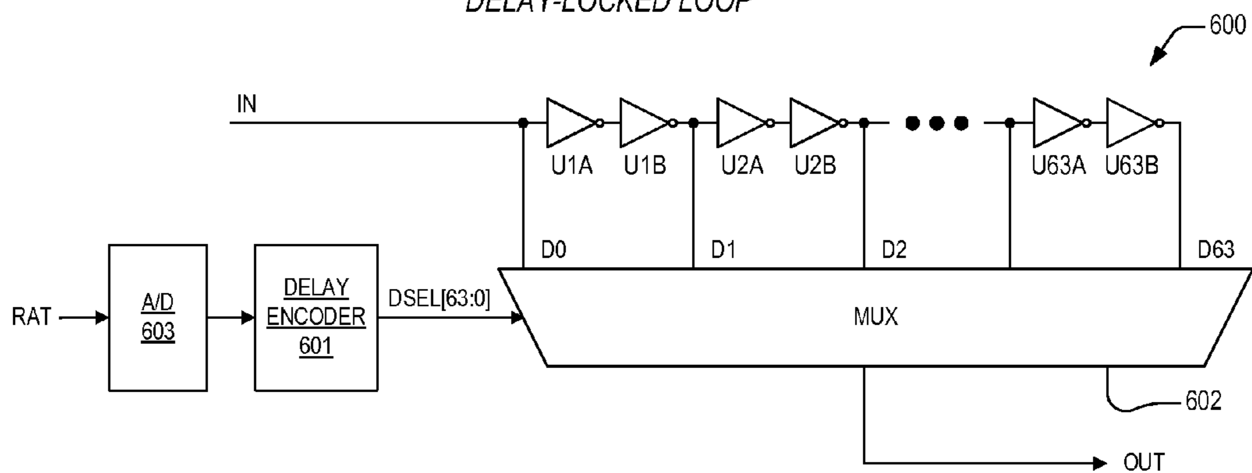
DELAY-LOCKED LOOP
