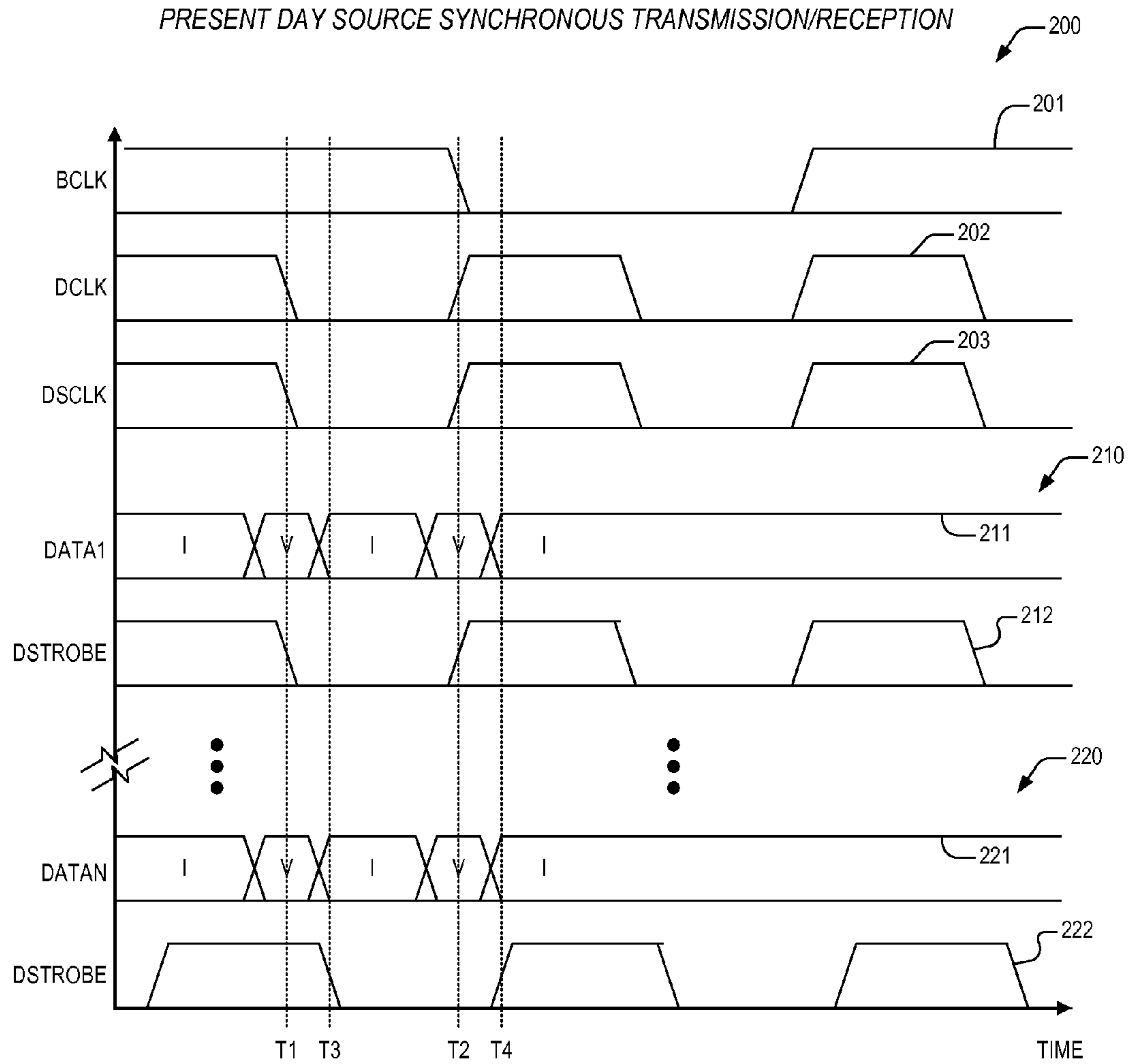
FIG. 2 (Prior Art)
