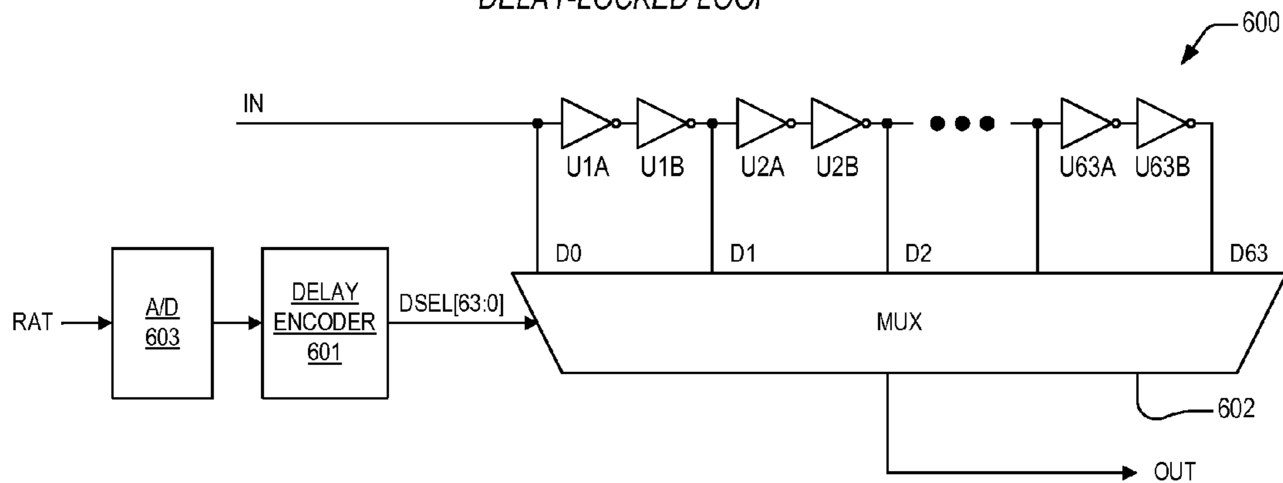
DELAY-LOCKED LOOP
