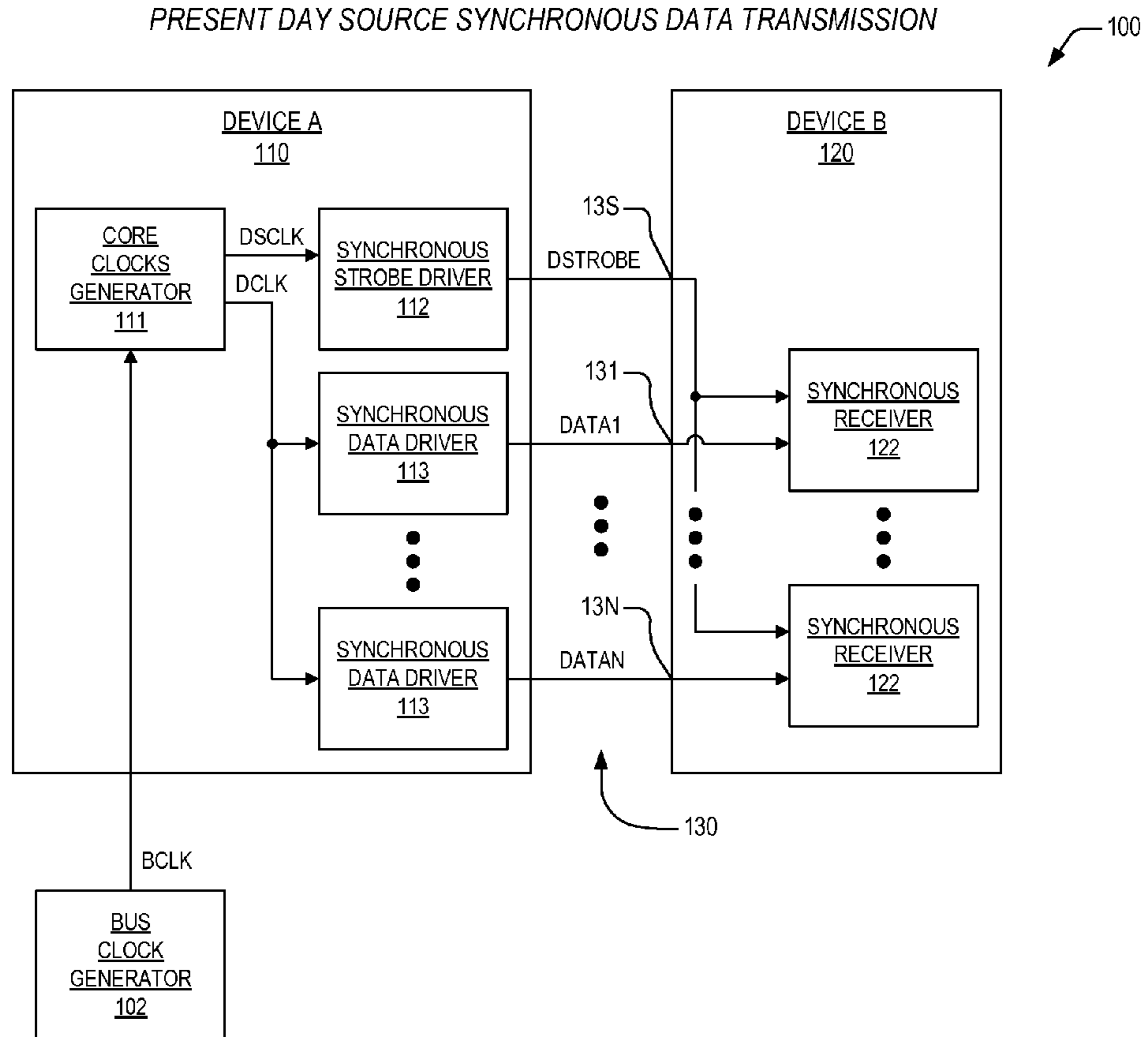
FIG. 1 (Prior Art)
