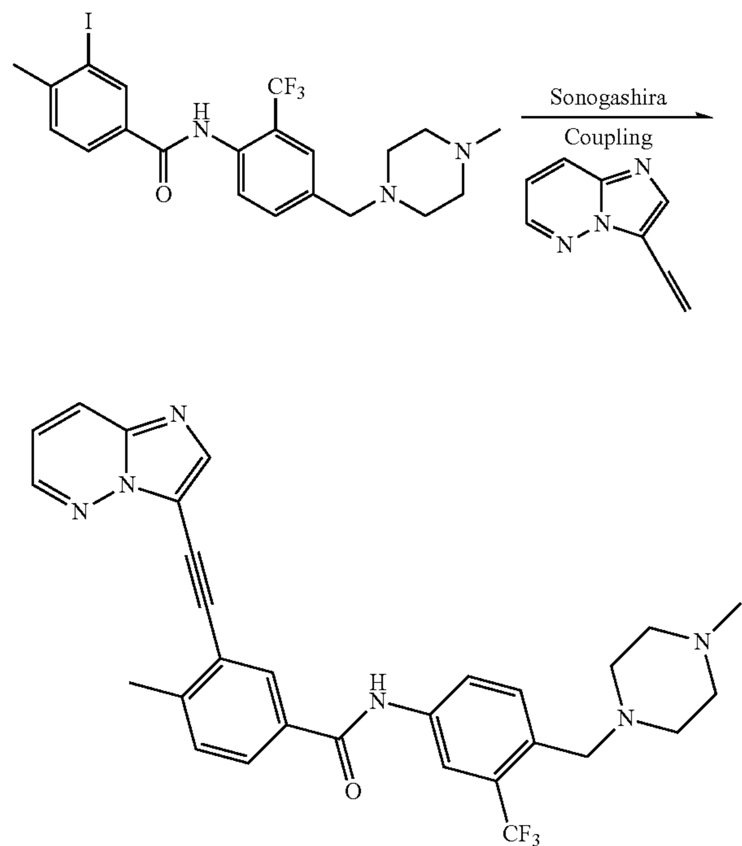
Scheme XIV
