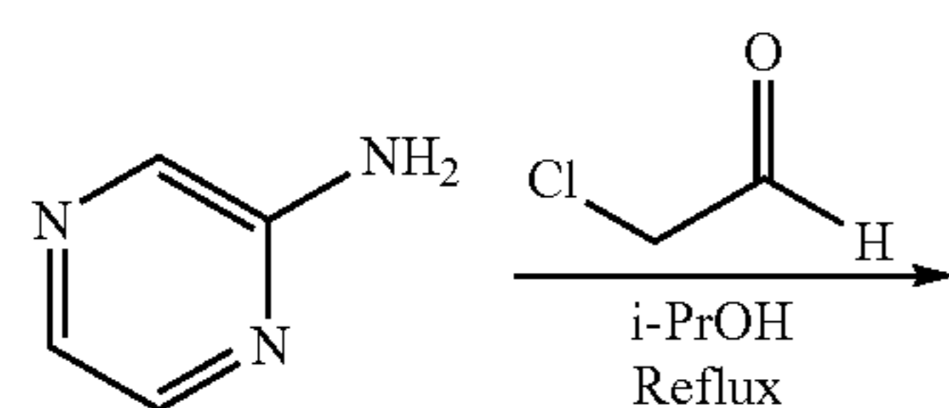
Scheme III: Preparation of 3-Ethynylimidazo[1,2-a]pyrazine
