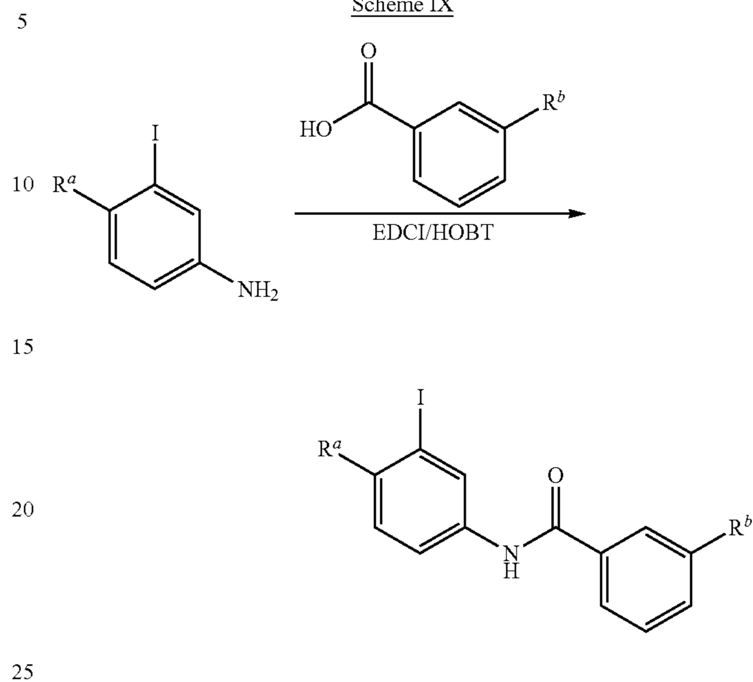
Scheme IX
