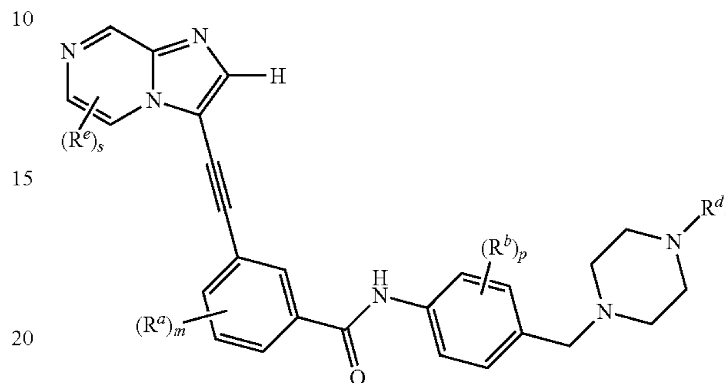
Formula IIIa
