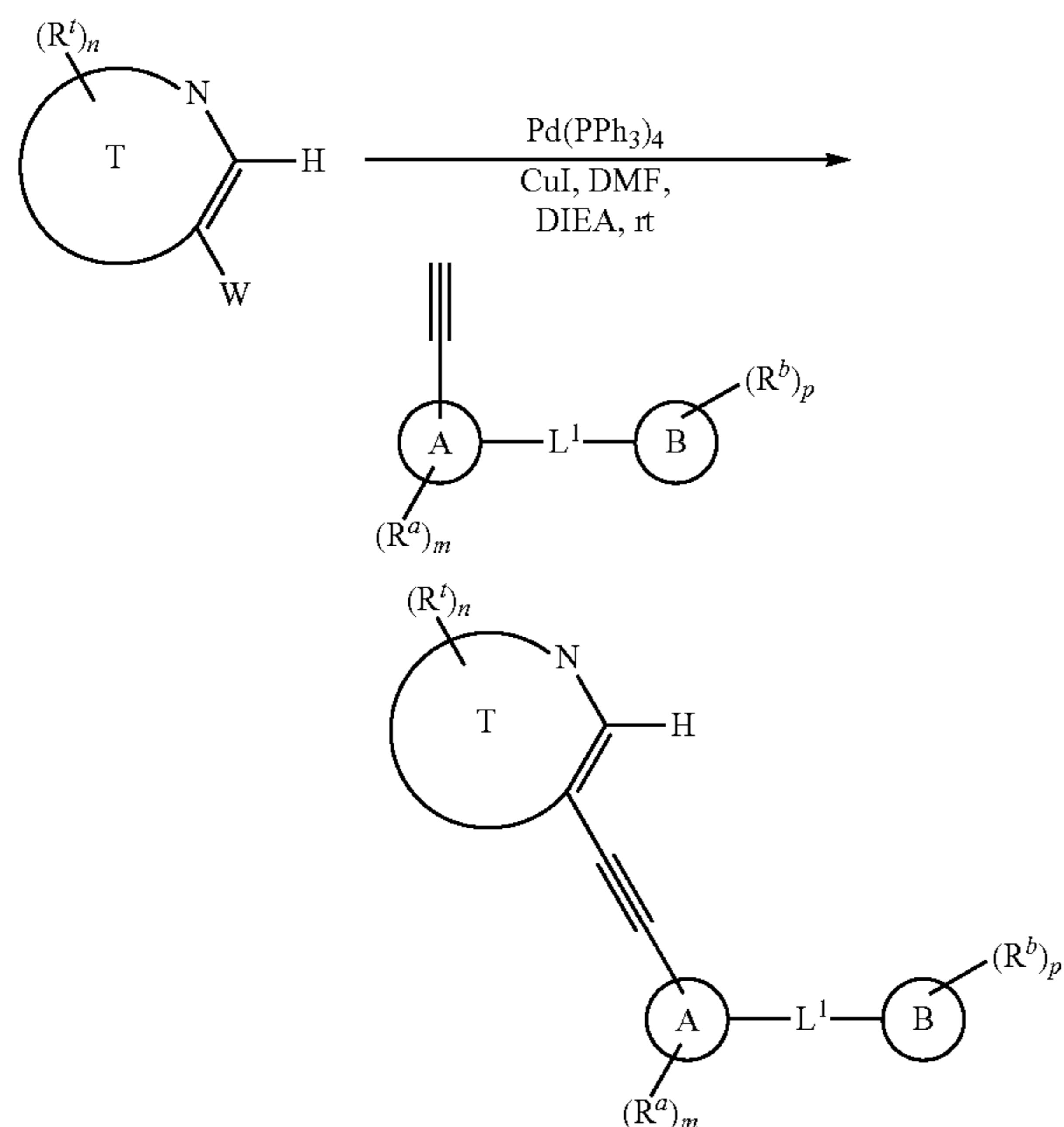
Scheme II: Alternative Sonogashira Coupling Reaction
