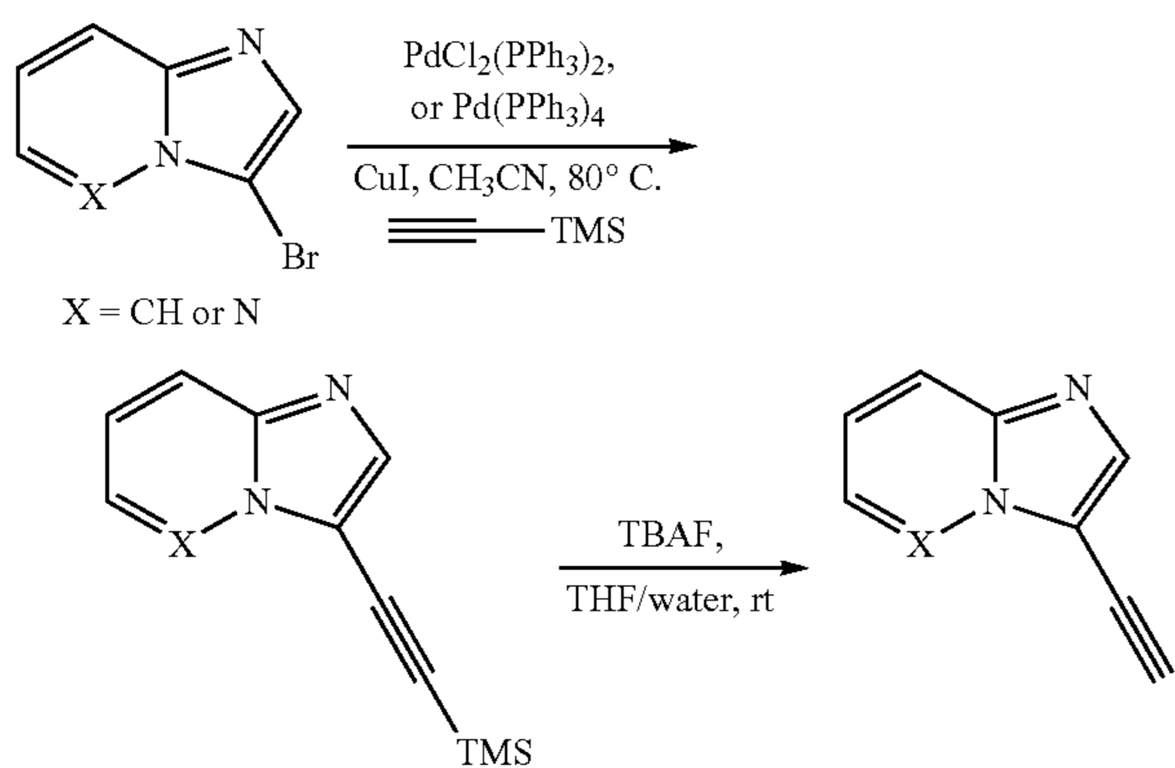
Scheme V: Preparation of 3-Ethynylimidazo[1,2-a]pyridine or 3-Ethynylimidazo[1,2-b]pyridazine
