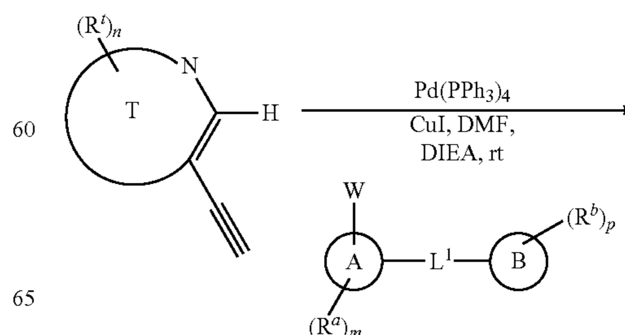
Scheme I: Sonogashira Coupling Reaction
