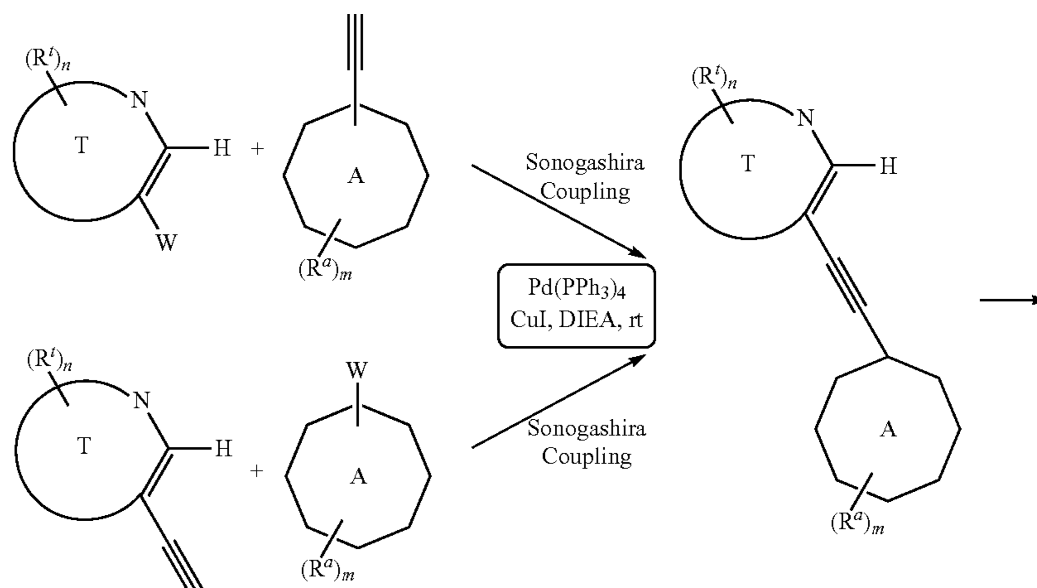
Scheme XVI
