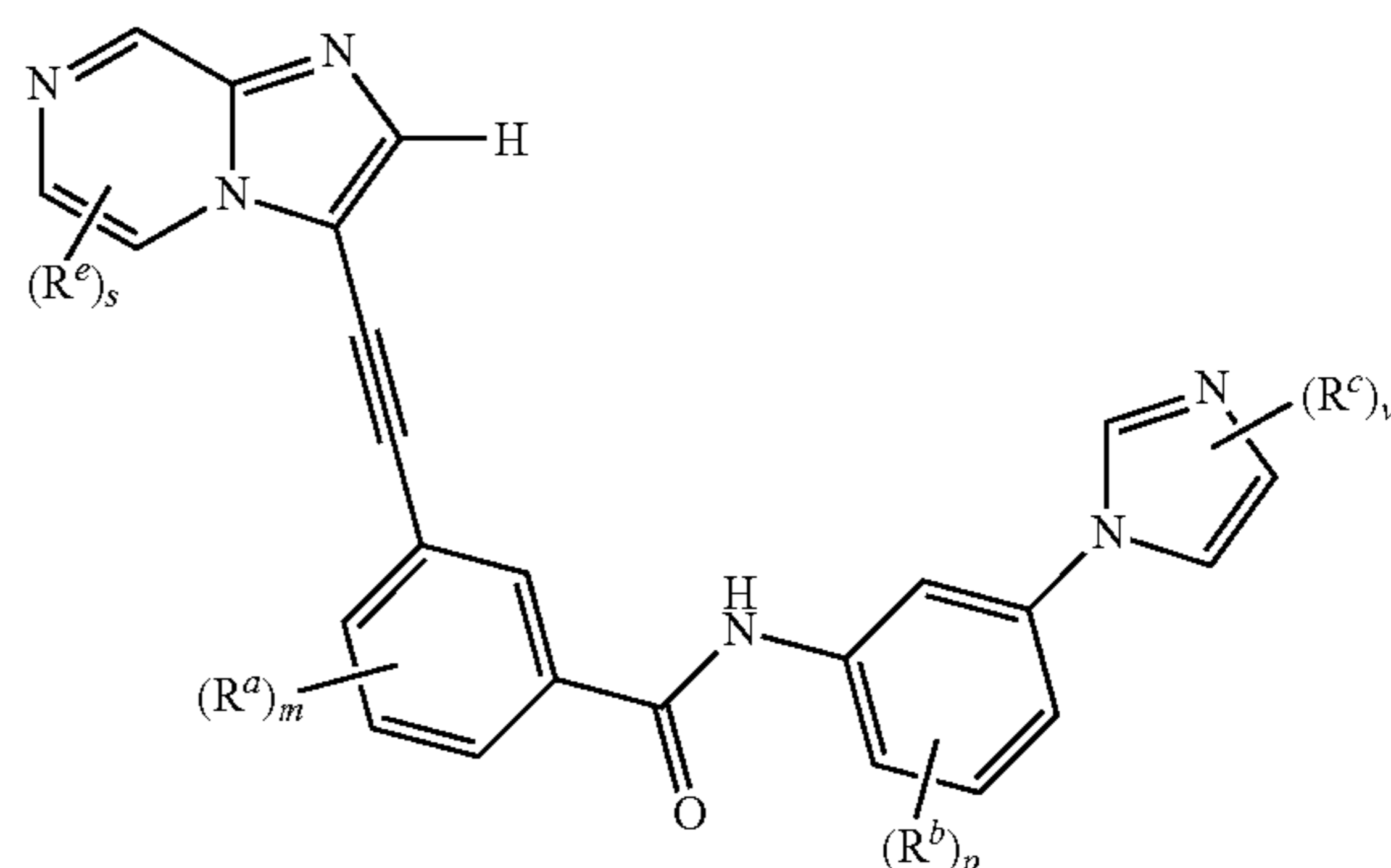
Formula IIa
