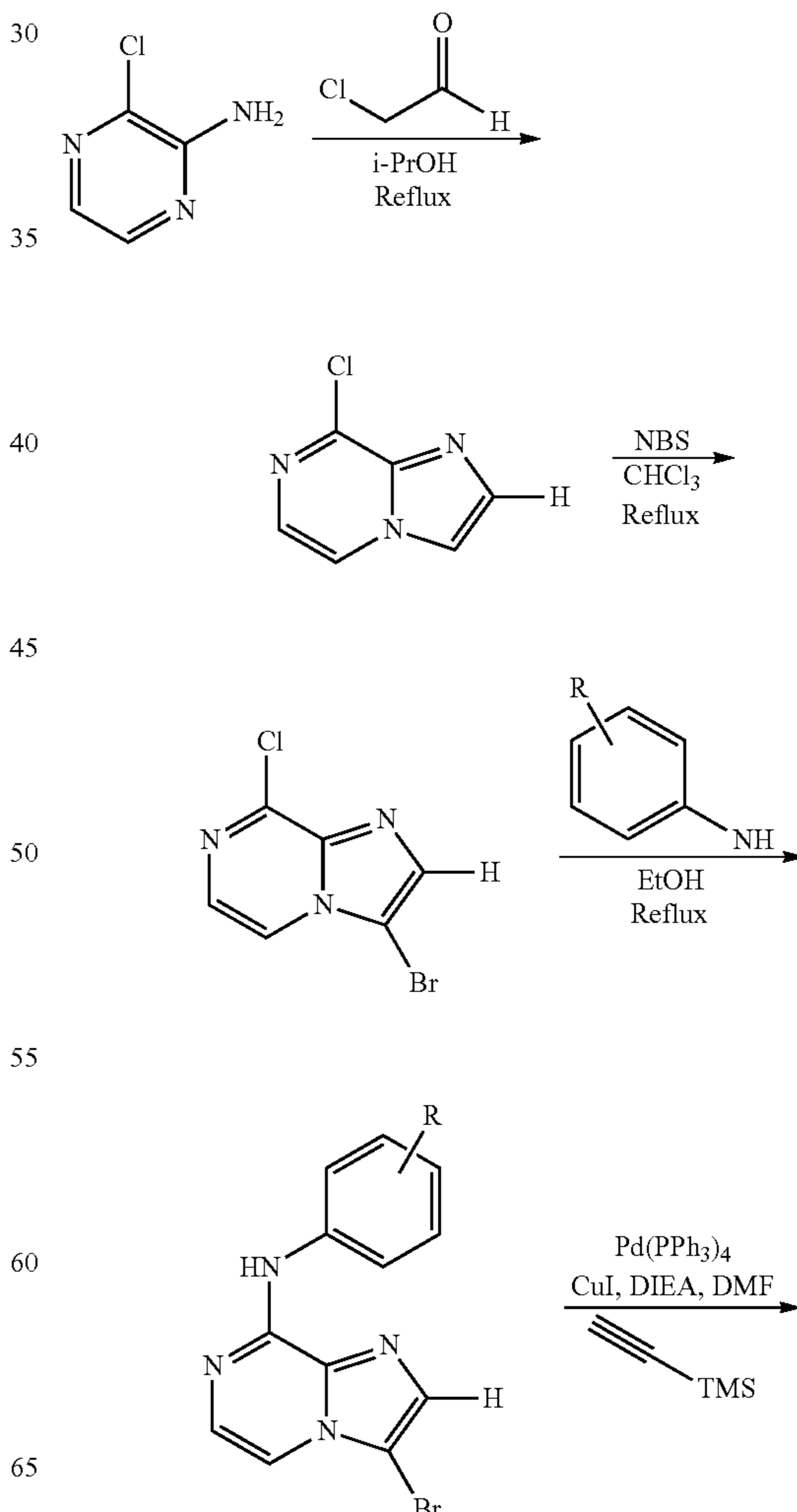
Scheme IV: Preparation of C-8 Substituted 3-Ethynylimidazo[1,2-a]pyrazines
