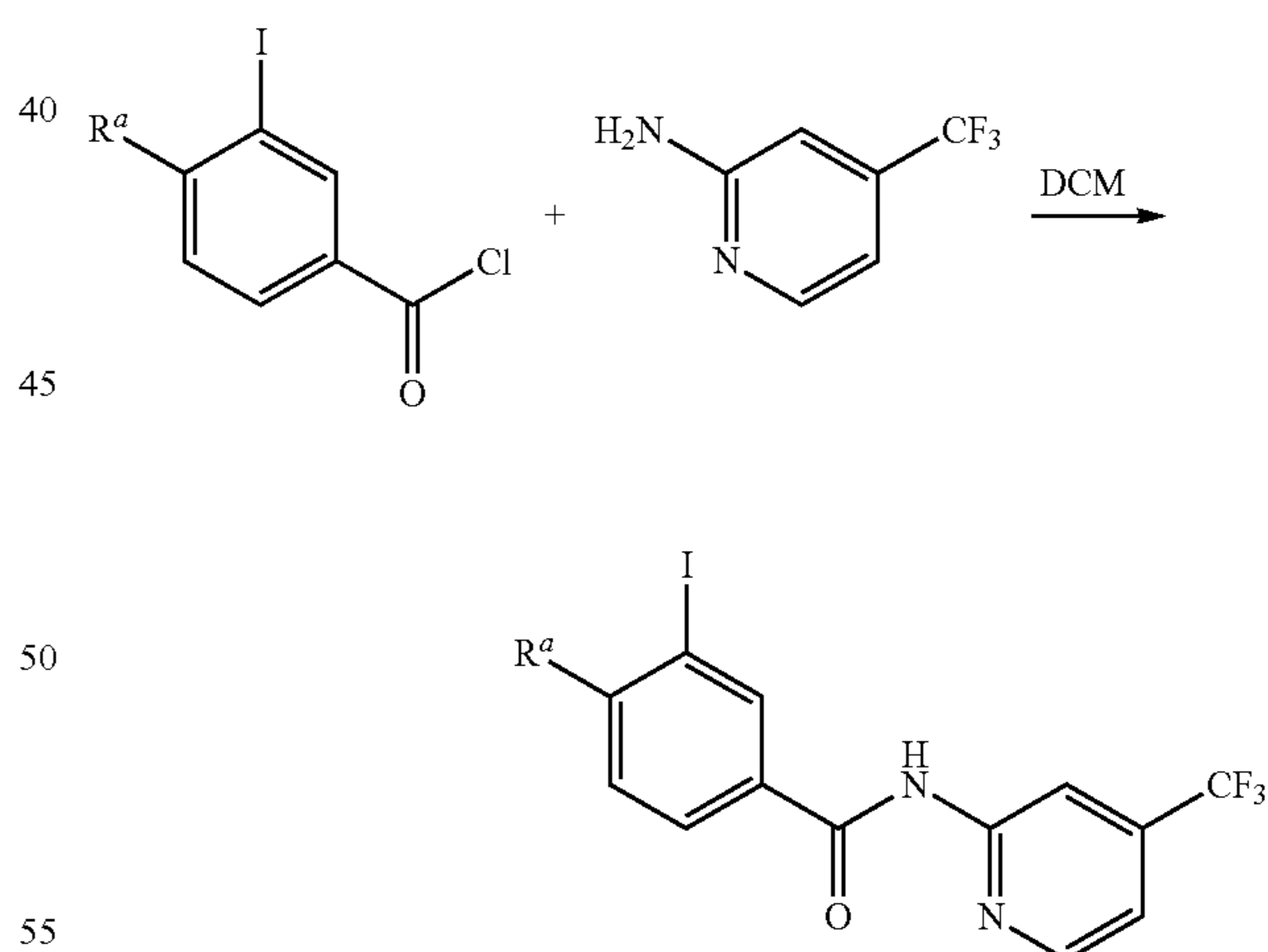
Scheme X
