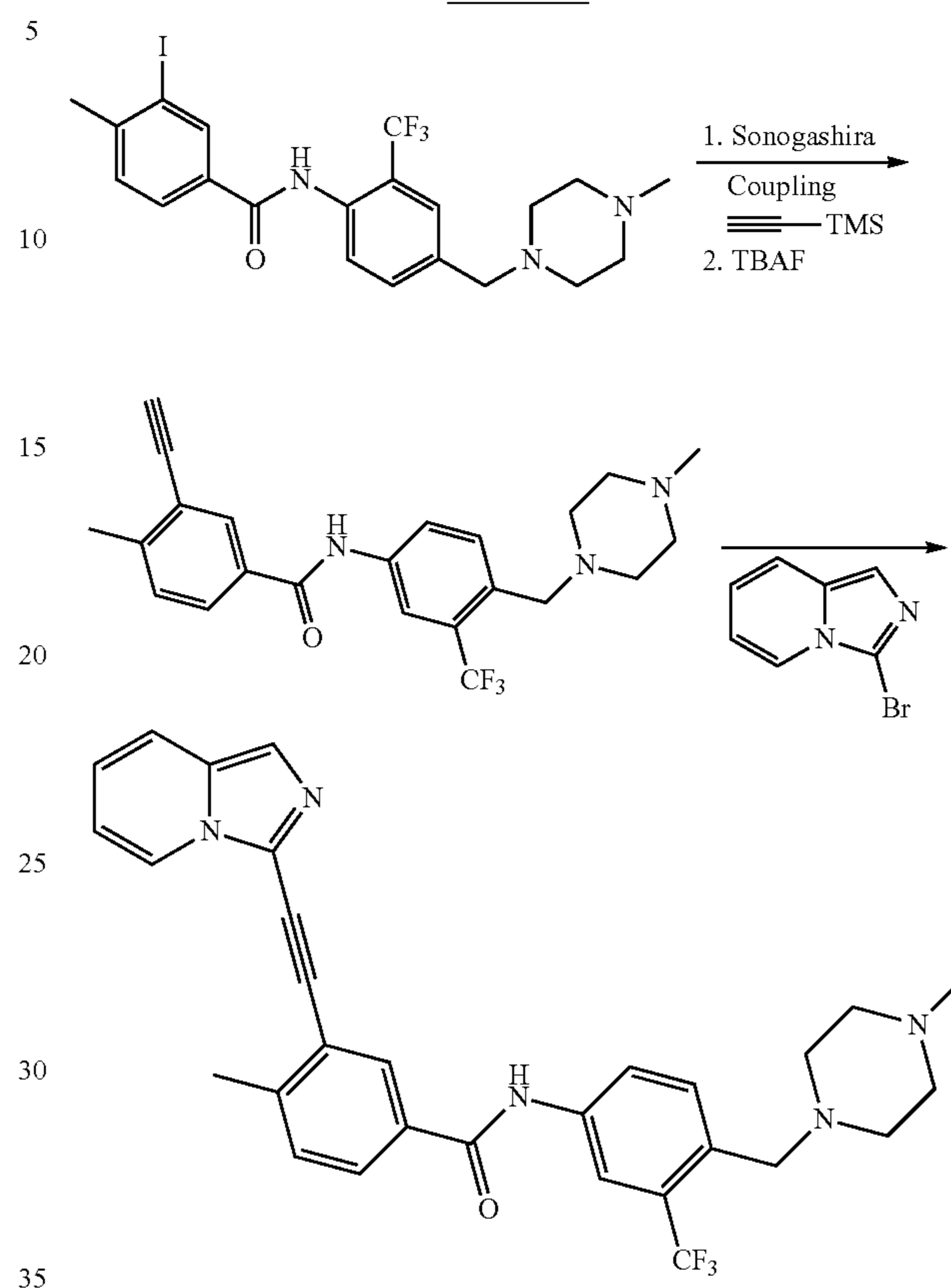
Scheme XV
