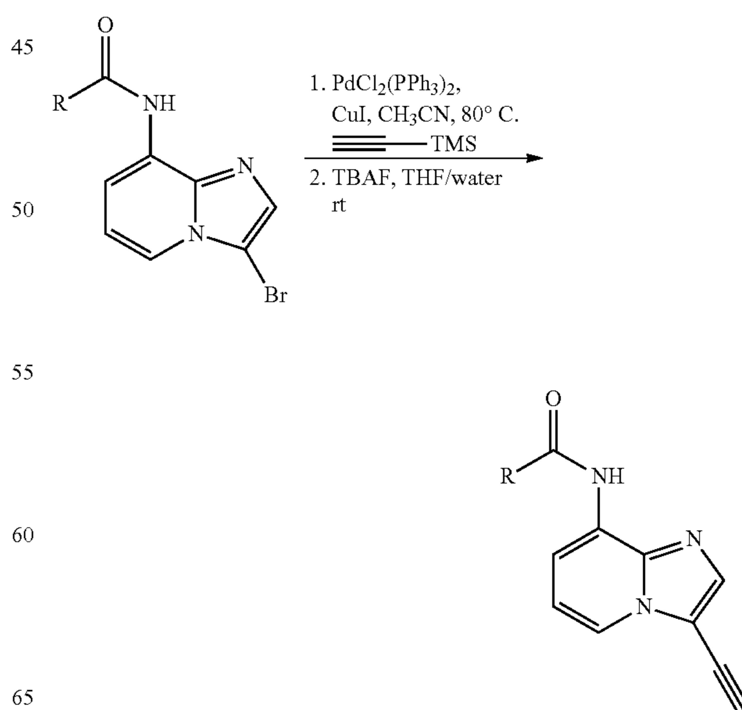
Scheme VII: Preparation of C-8 substituted 3-Ethynylimidazo[1,2-a]pyridines
