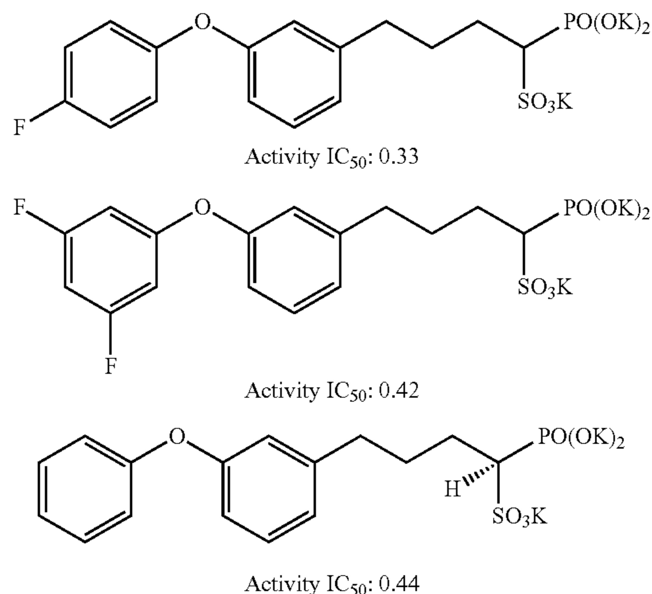
Structure of CrtM inhibitors and their inhibitory activity (iM)
