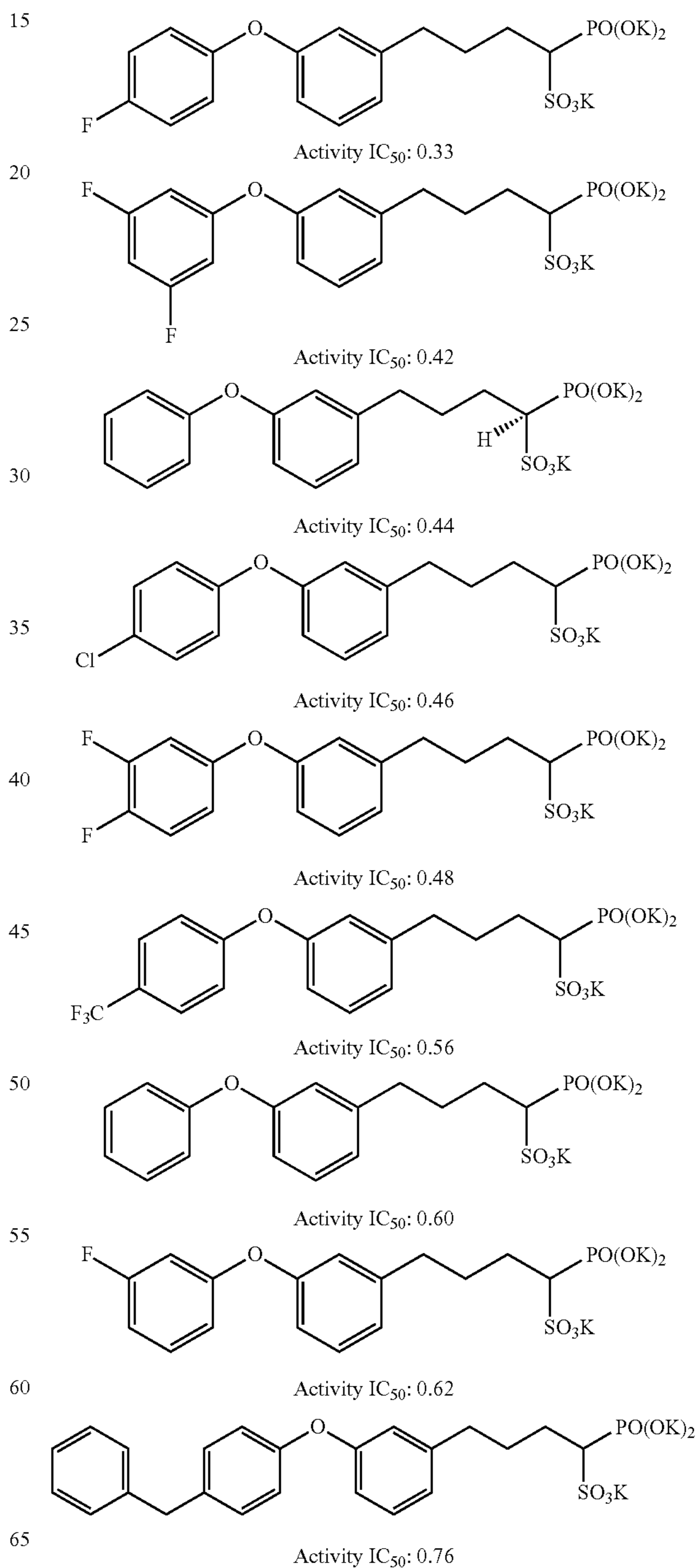
Structures of CrmM inhibitors and their inhibitory activity ( IC_{50} )
