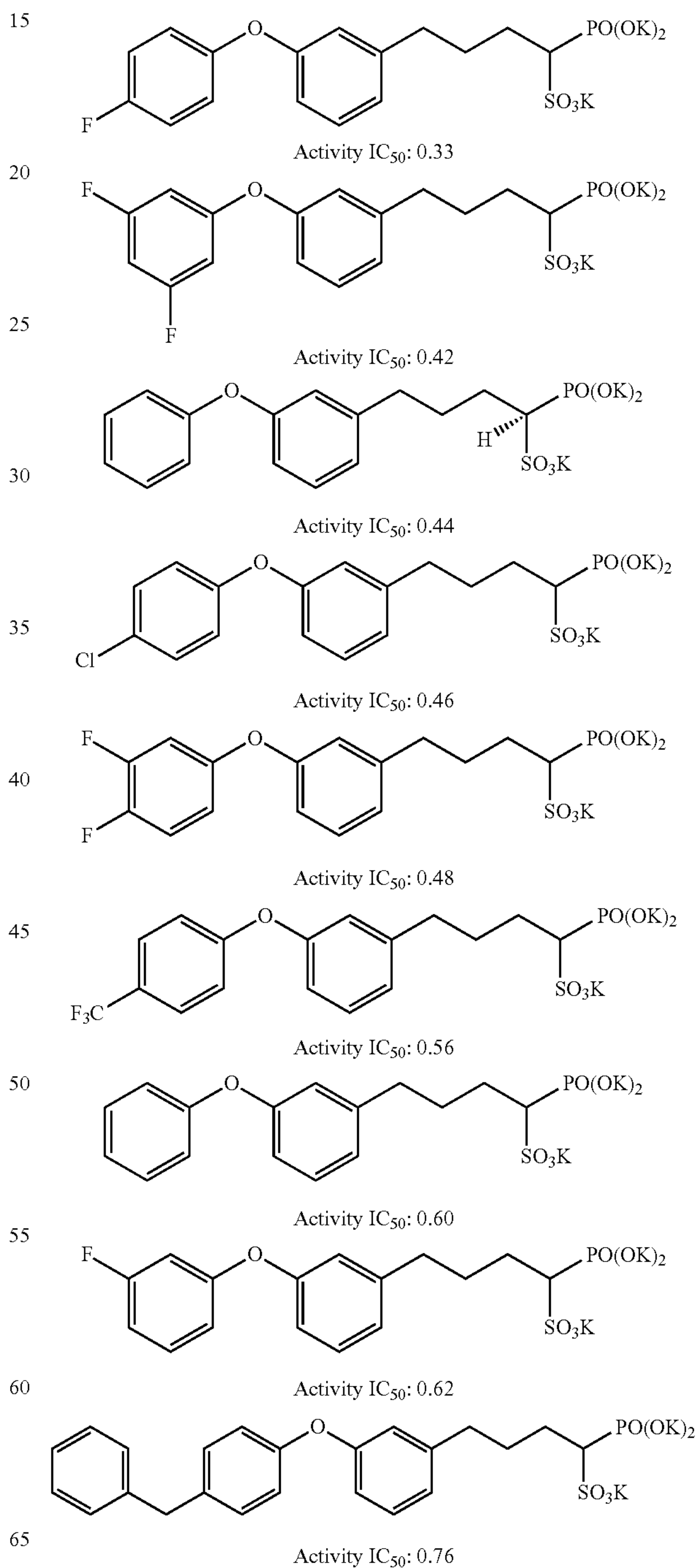
Structures of CrmM inhibitors and their inhibitory activity ( :\dot{\text{M}} )
