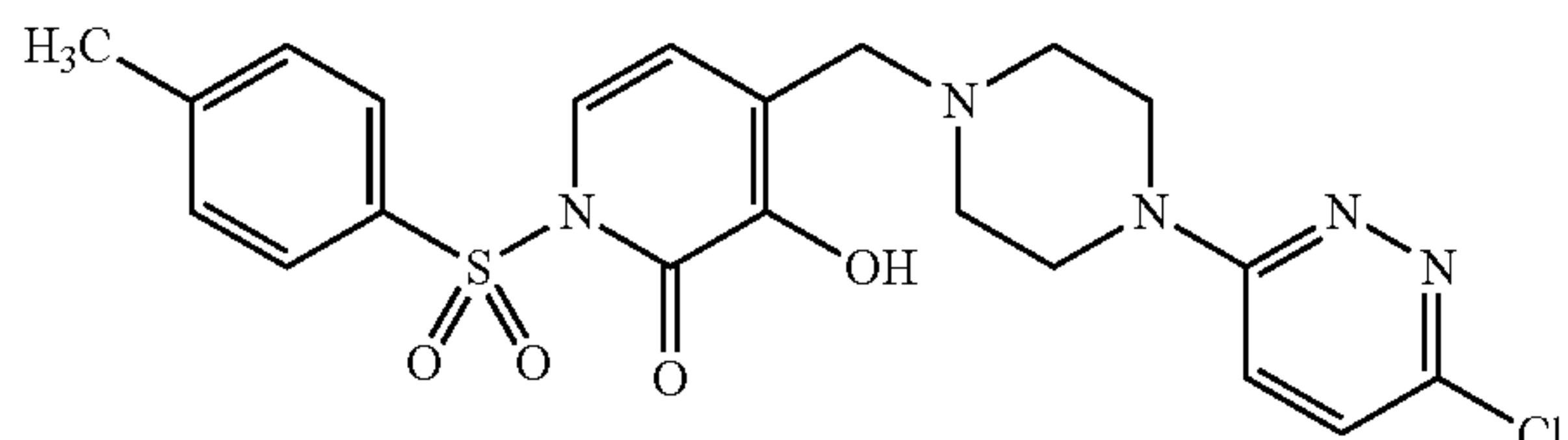
1-(4'-Methylbenzenesulfonyl)-3-hydroxy-4-[4-(6-chloropyridazin-3-yl)piperazin-1-ylmethyl]pyridin-2(1H)-one
