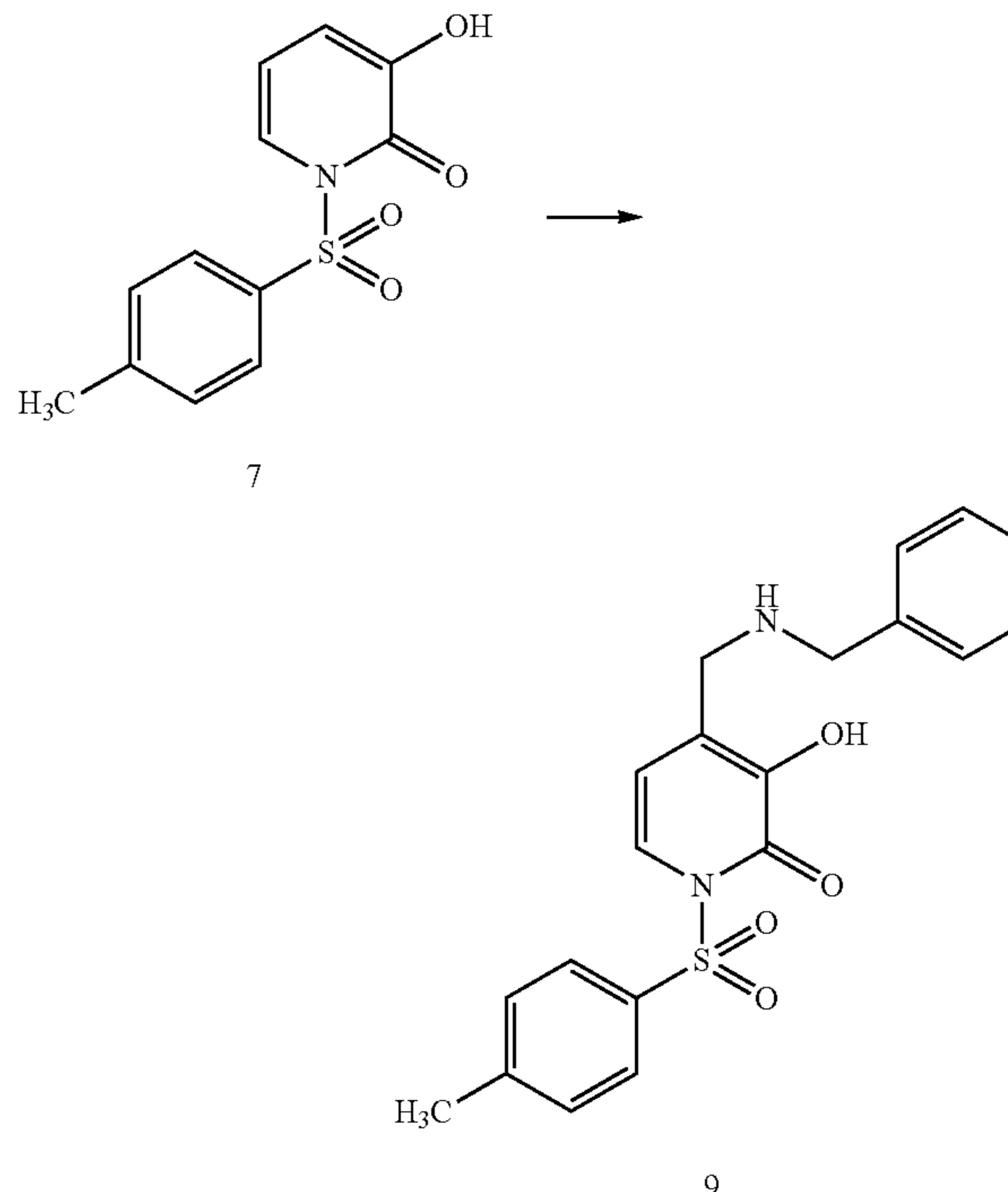
Scheme IV
