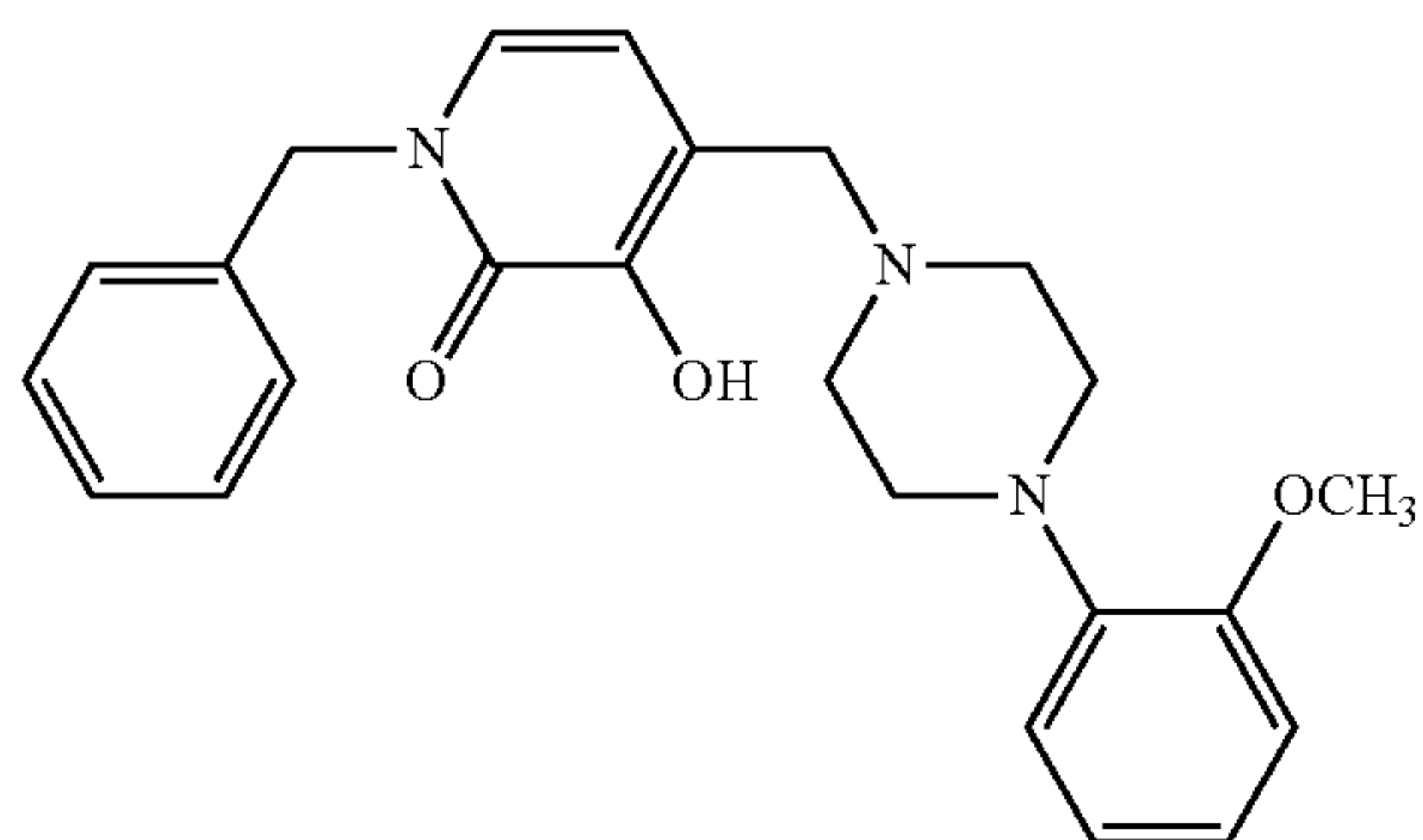
1-Benzyl-3-hydroxy-4-[4-(2-methoxyphenyl)piperazin-1-ylmethyl]pyridin-2(1H)-one
