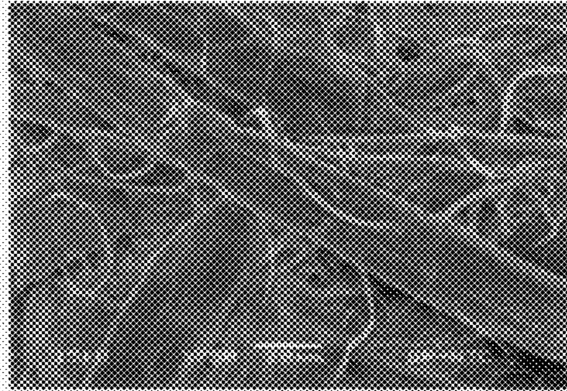
FIG. 2B 25% MICROFIBER, YANKEE SIDE
