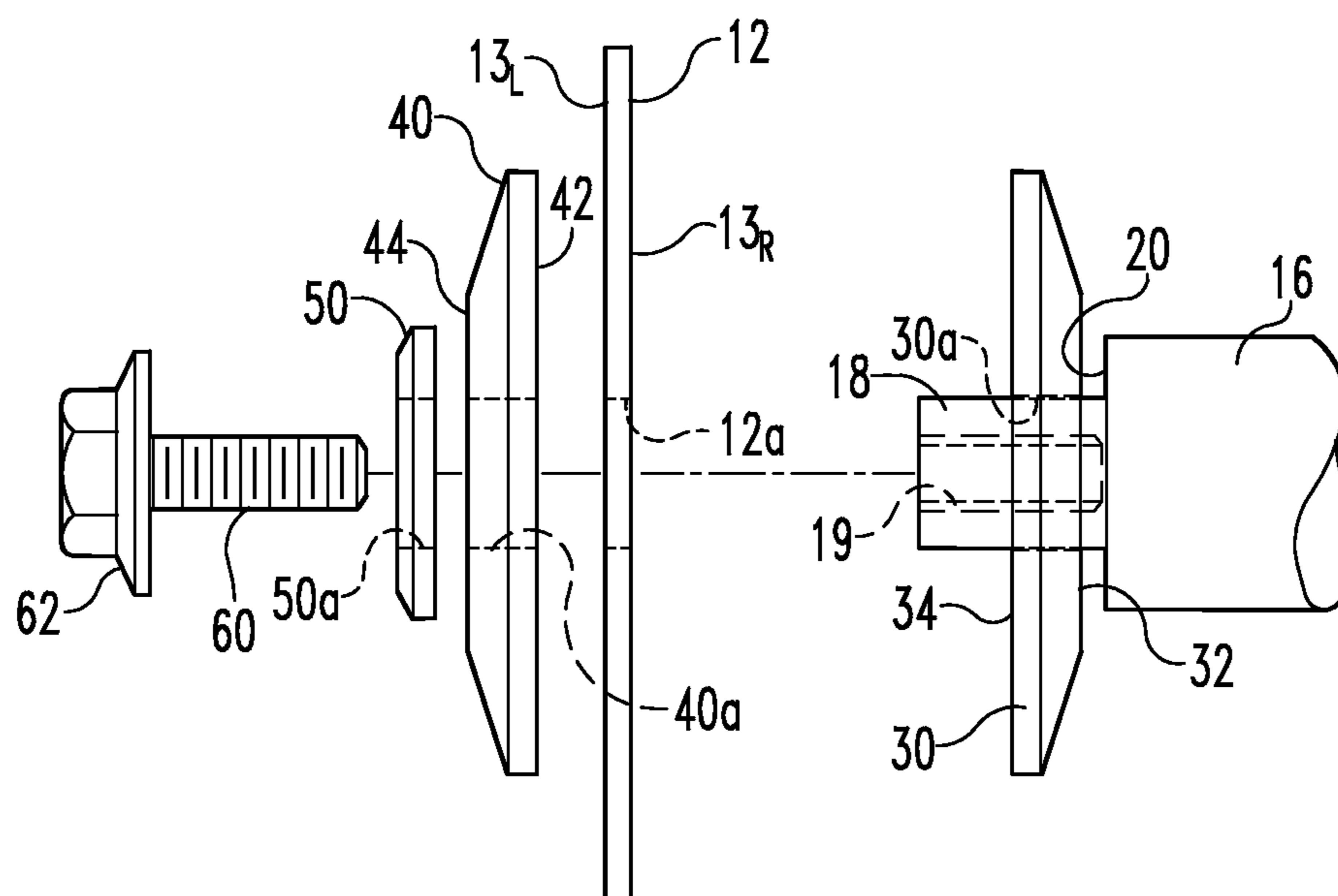
Fig. 2 (Prior Art)
