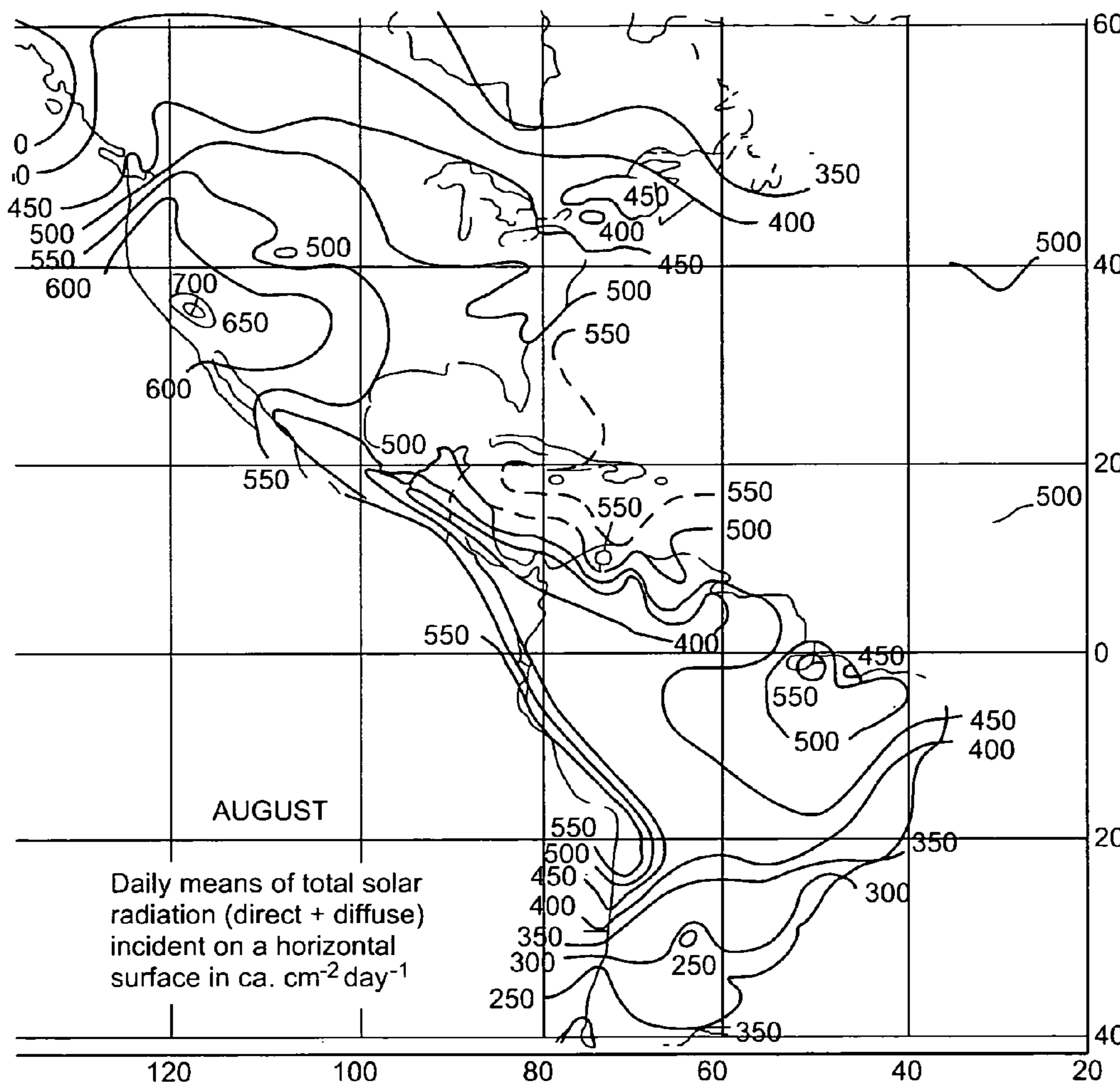
FIGURE 2.21 Average daily total horizontal solar radiation for the month of August in langleys per day. From dejong (2) with permission
