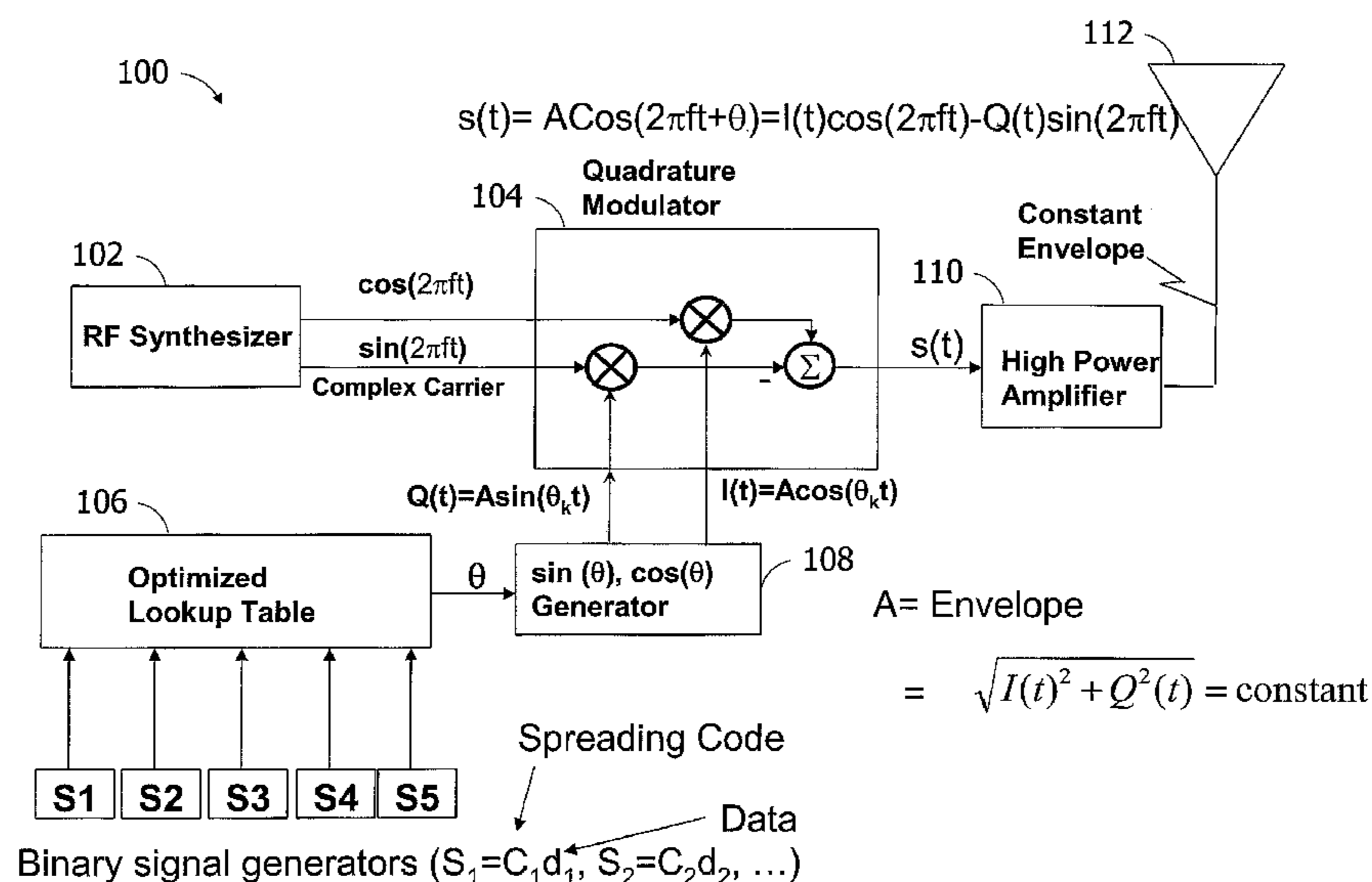
POCET System Combining 5 Signals
