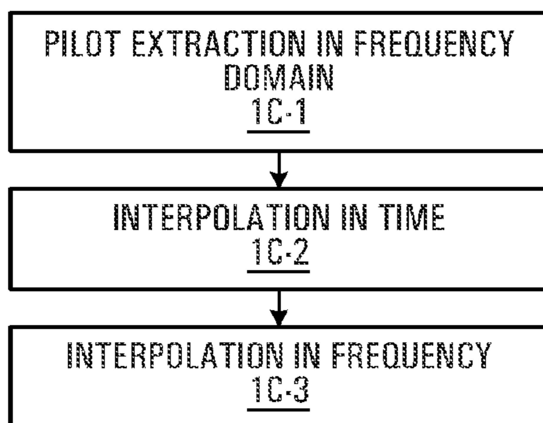
FIG. 1C (Prior Art)
