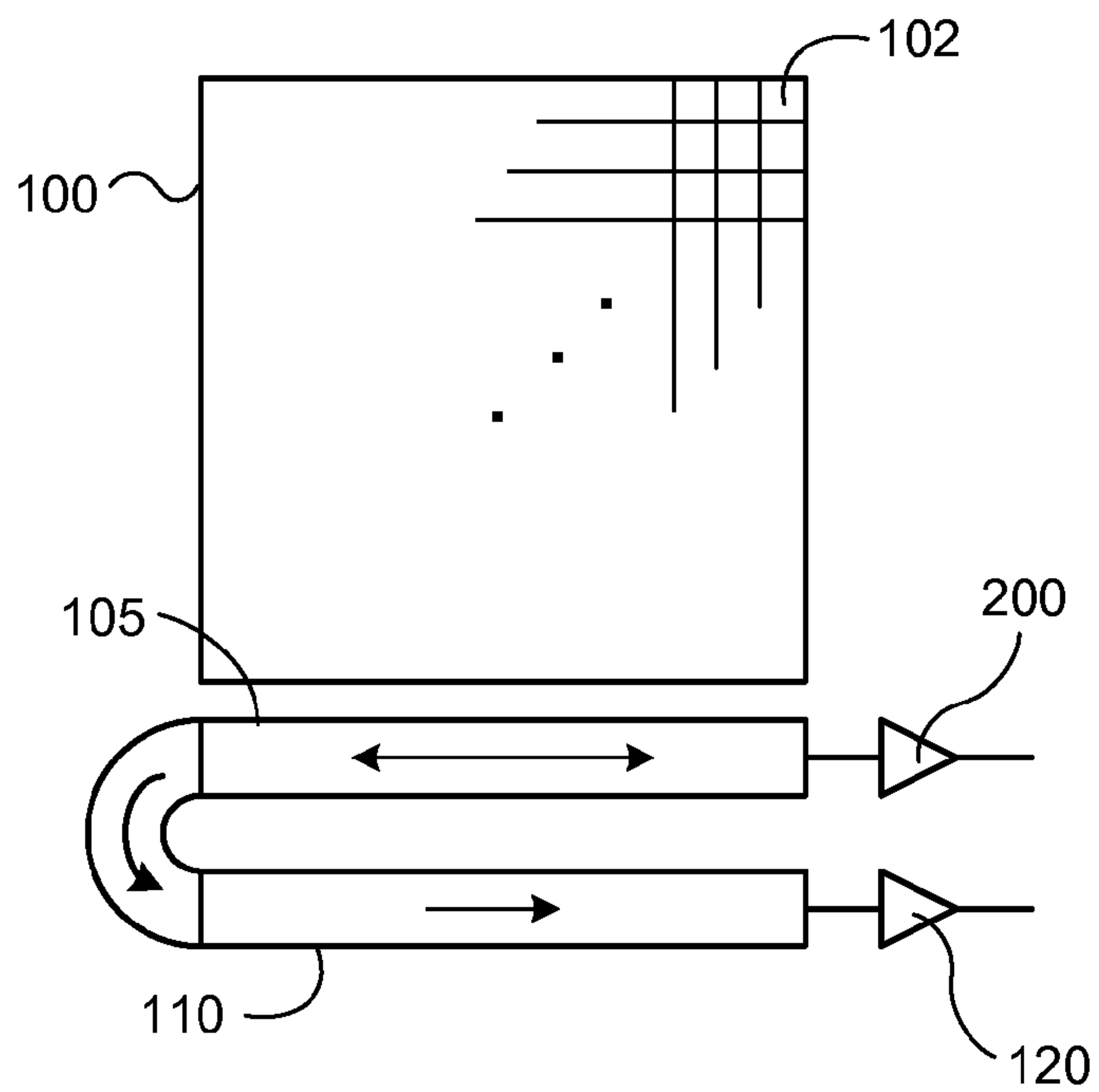
FIG. 2 (PRIOR ART)
