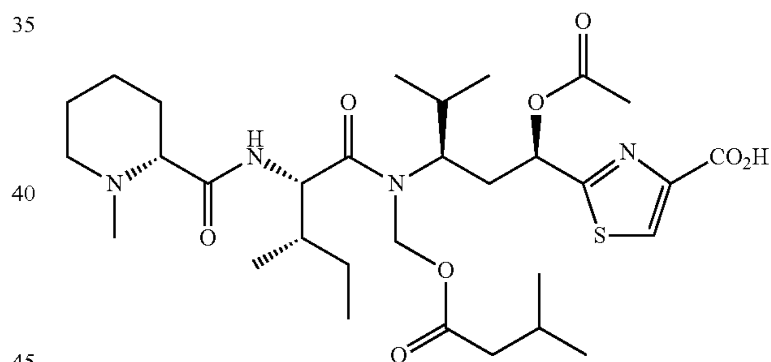
Acetate of Compound 27
