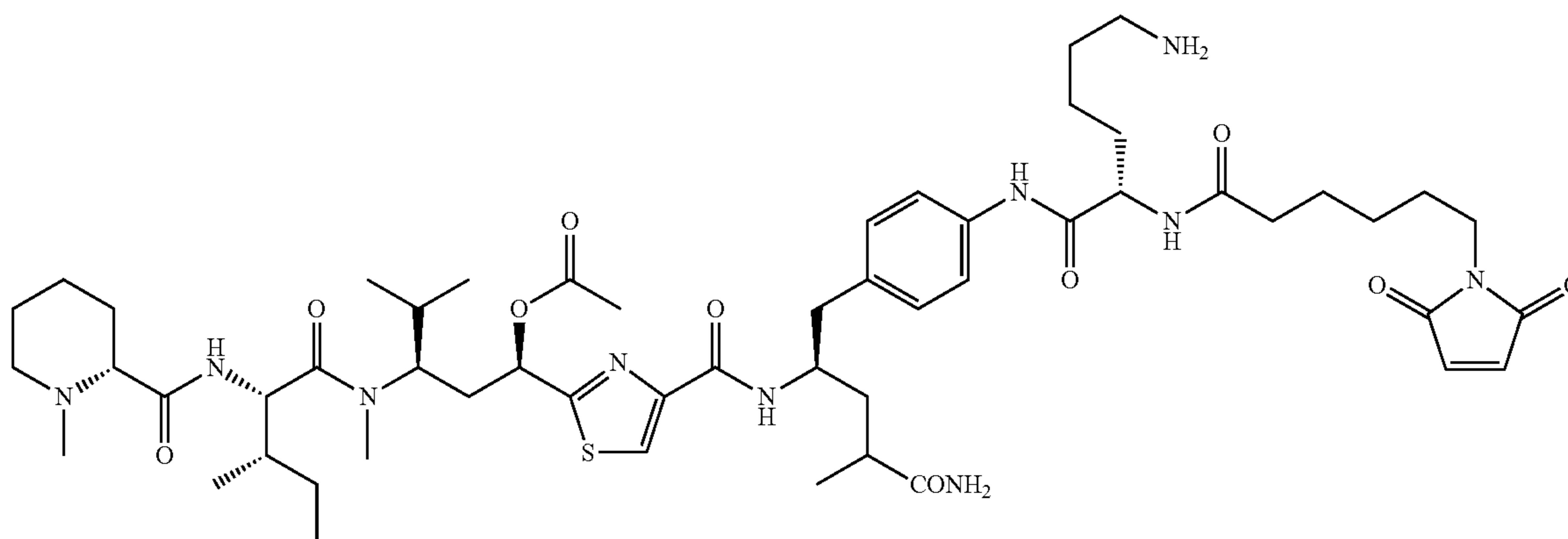
Amide of compound 39
