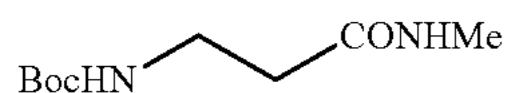
Methyl-3-(t-butoxycarbonylamino)propionic amide (14)
