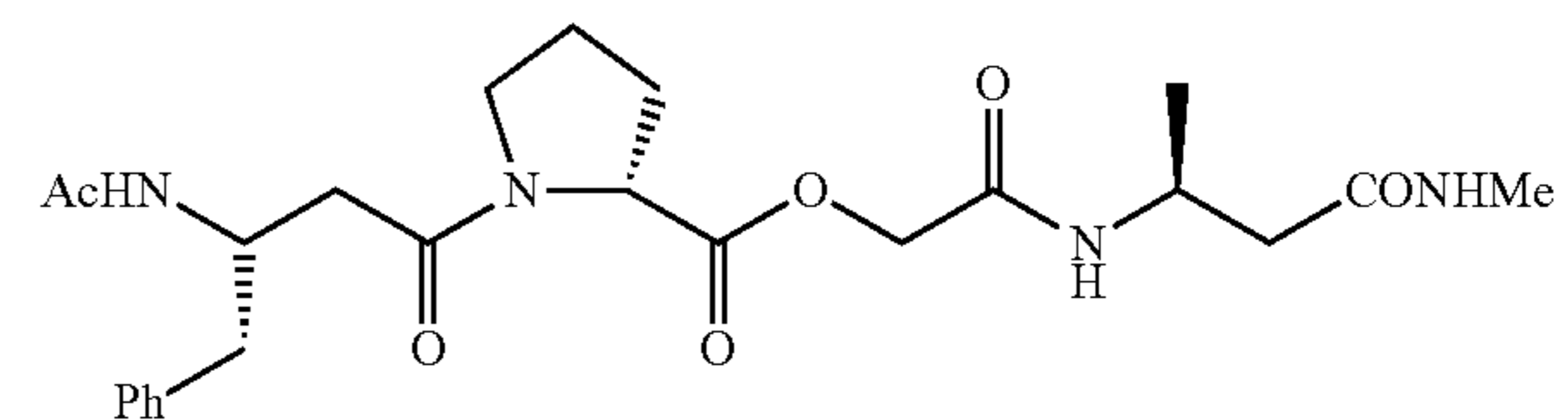
Compound 3.
