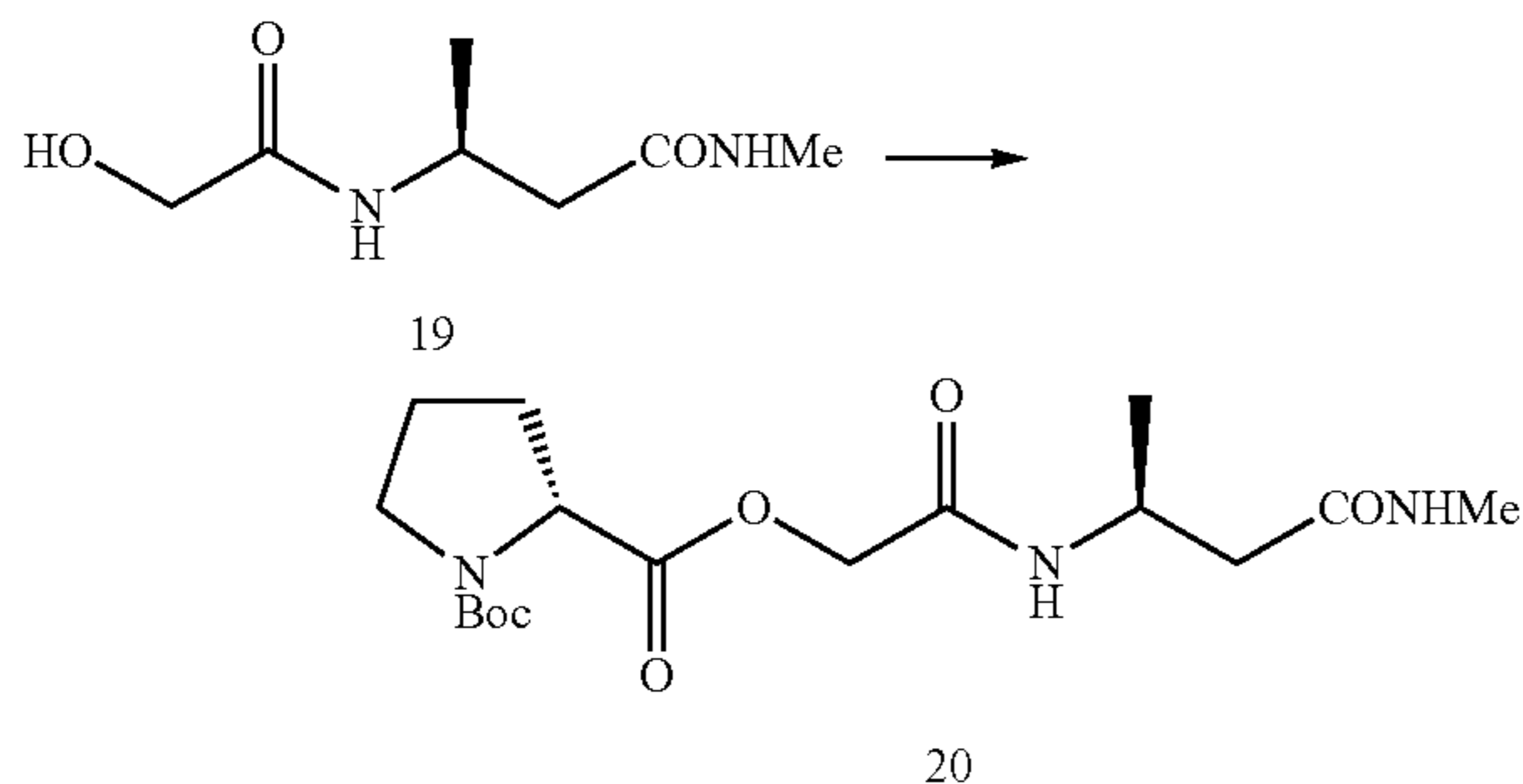
Compound 20.
