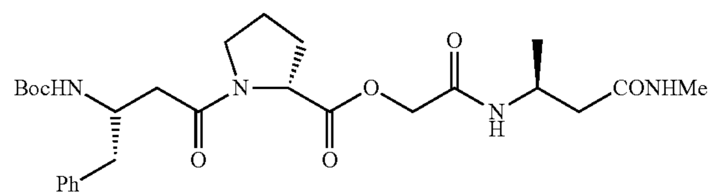
Compound 21.
