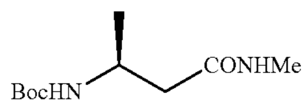
Methyl-(S)-3-(t-butoxycarbonylamino)butanoic amide (18)
