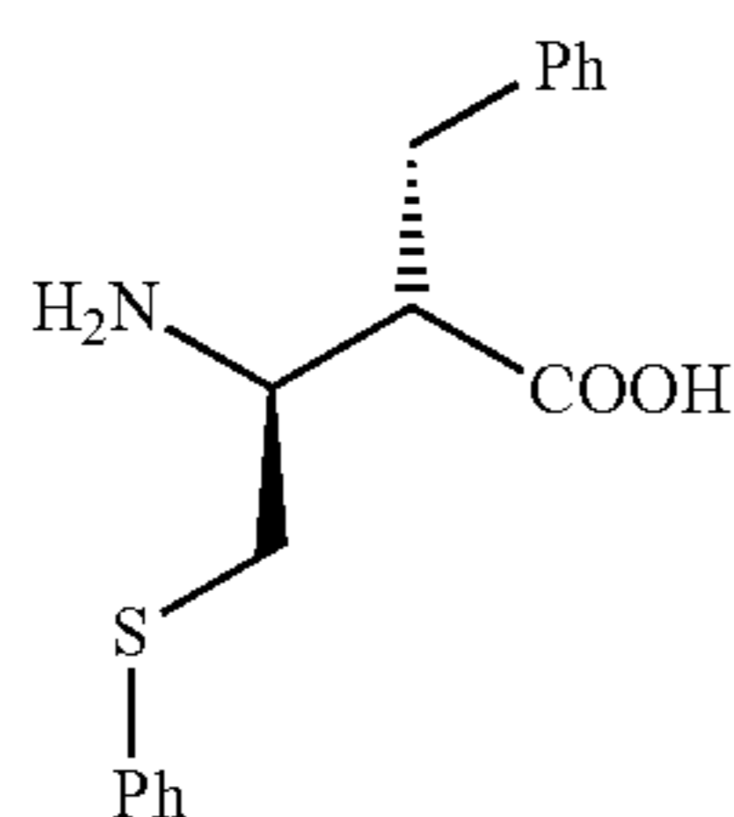
(2S,3S)-3-Amino-2-Benzyl-4-phenylthiobutanoic acid (8)
