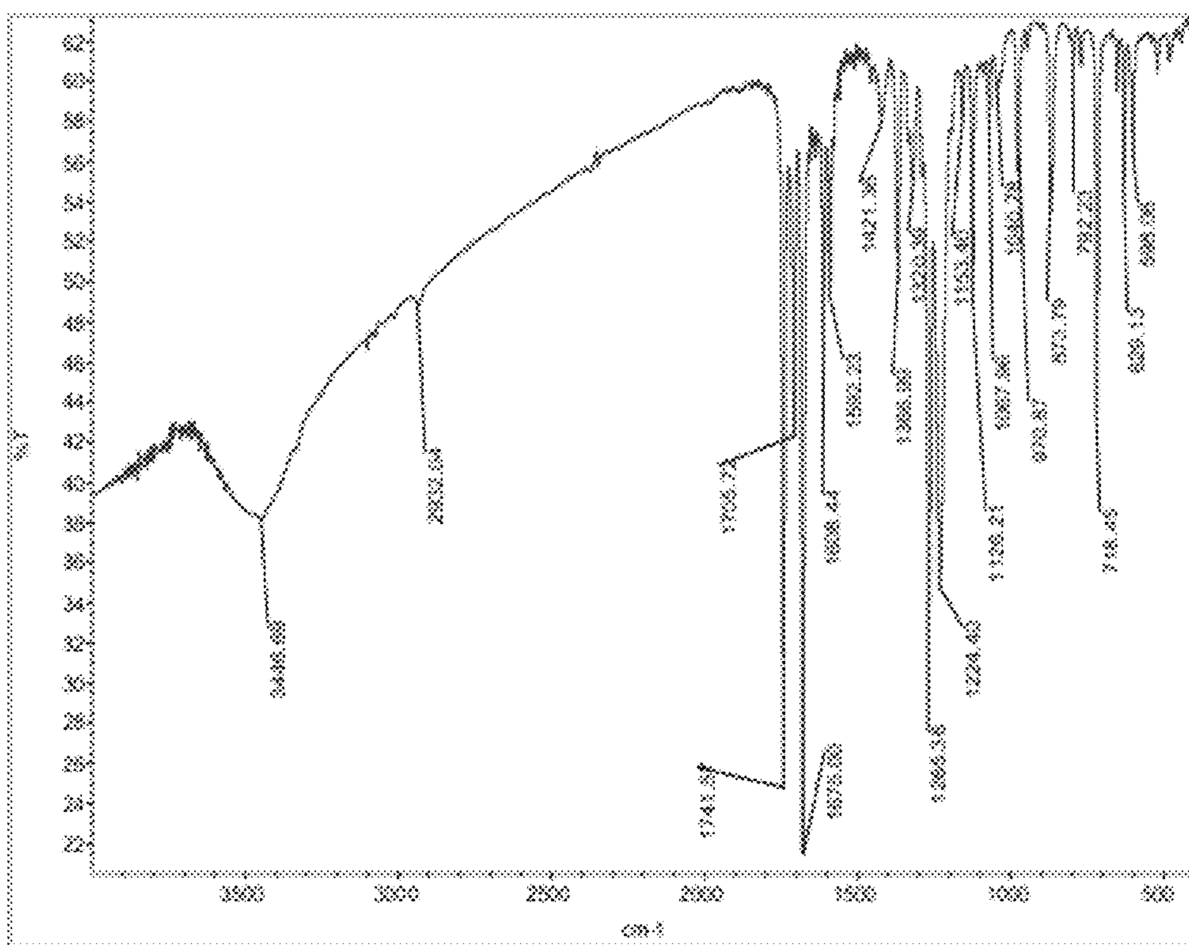
Figure 10 (IR spectrum of 2-chloro-3-diacylamino-1,4-naphthoquinone (zapp88).)
