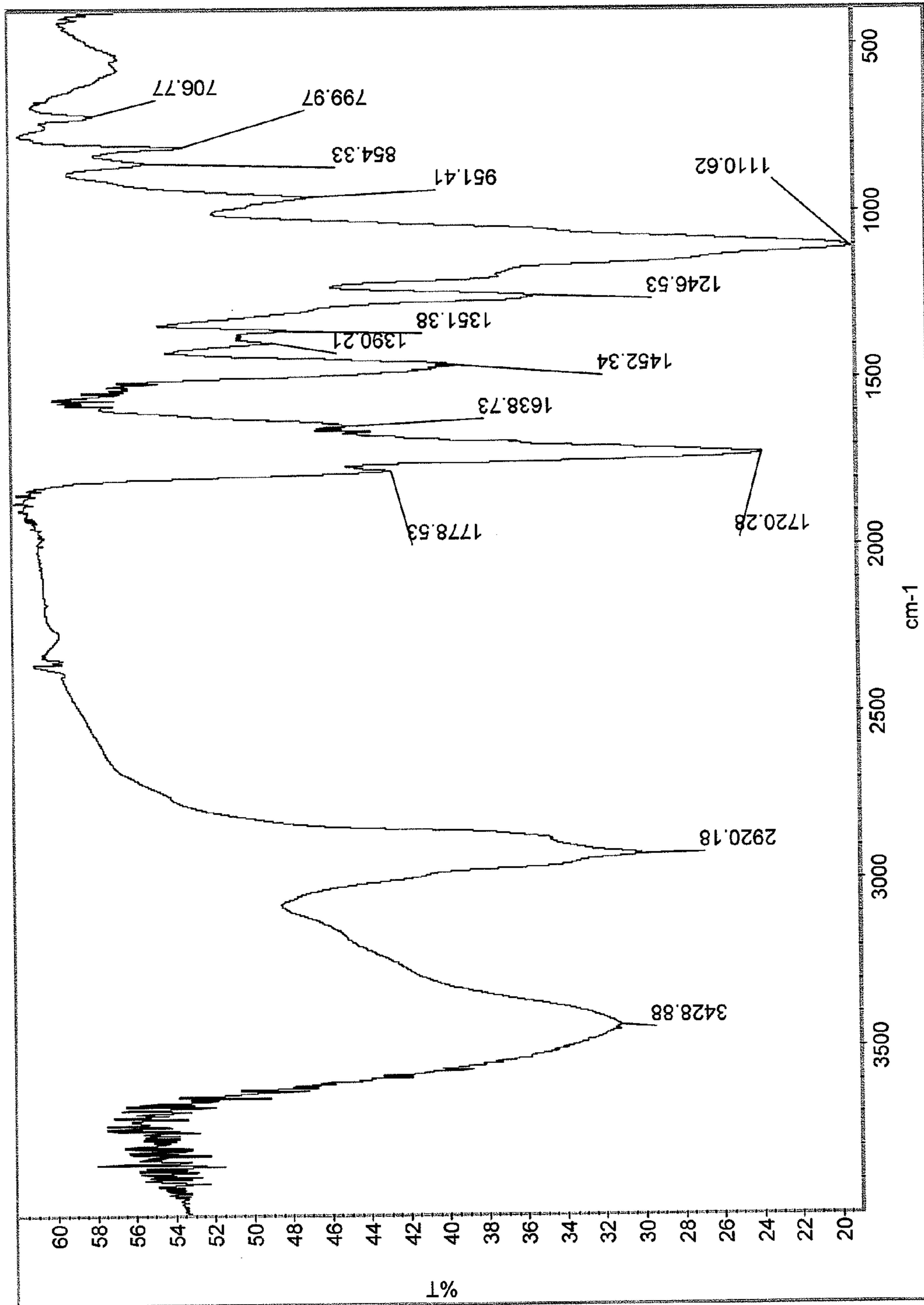
Figure 4 (IR spectrum of paclitaxel-loaded hydrolyzable PEG-MMA (PDL) nanospheres: fabricated with AIBN as an initiator)
