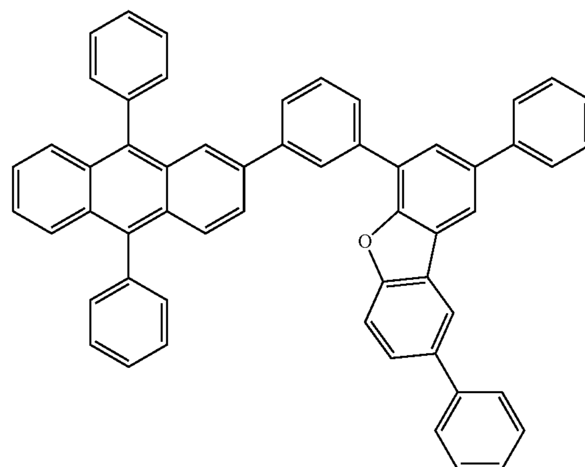
2mDBFPPA-III
