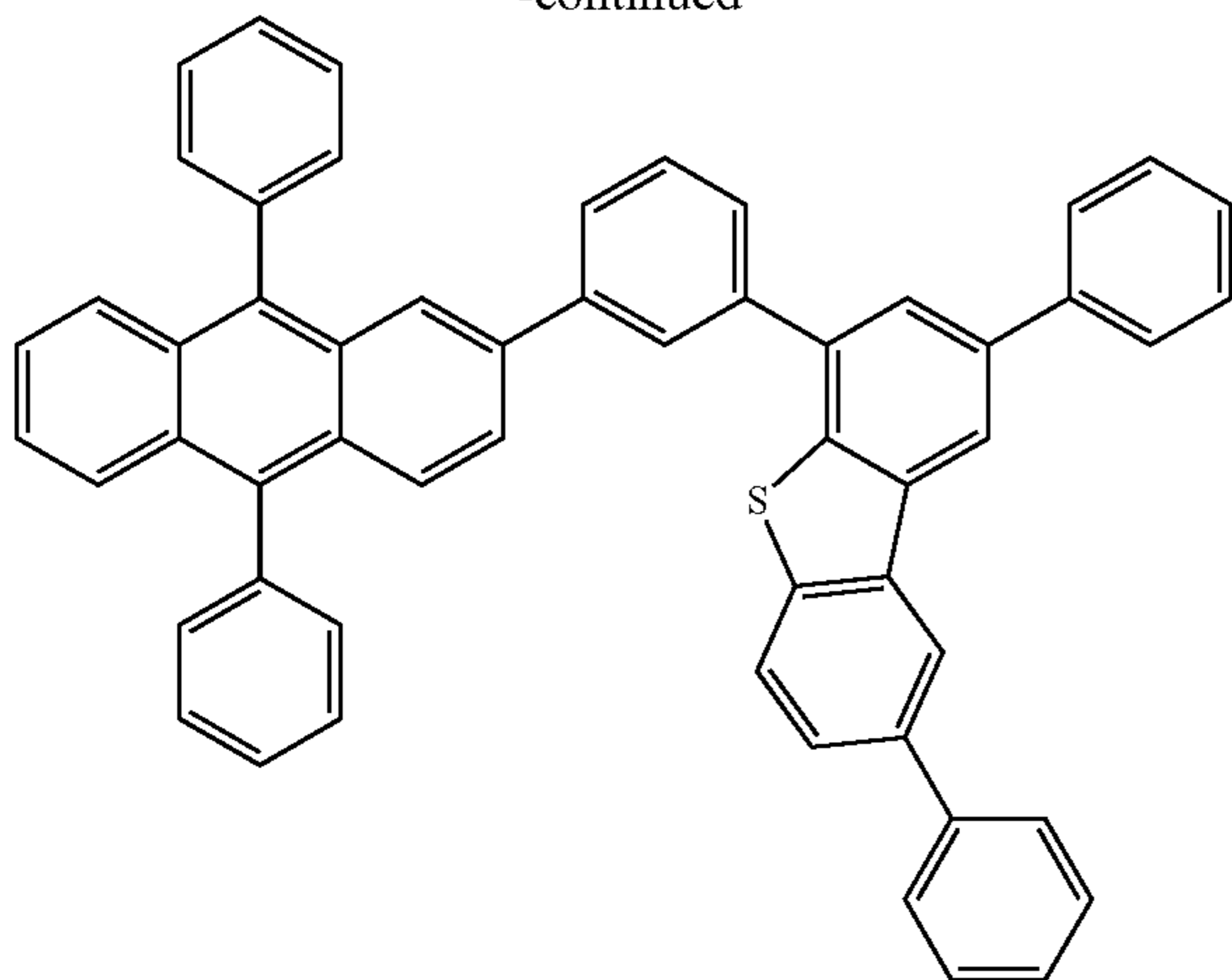
2mDBFPPA-III
