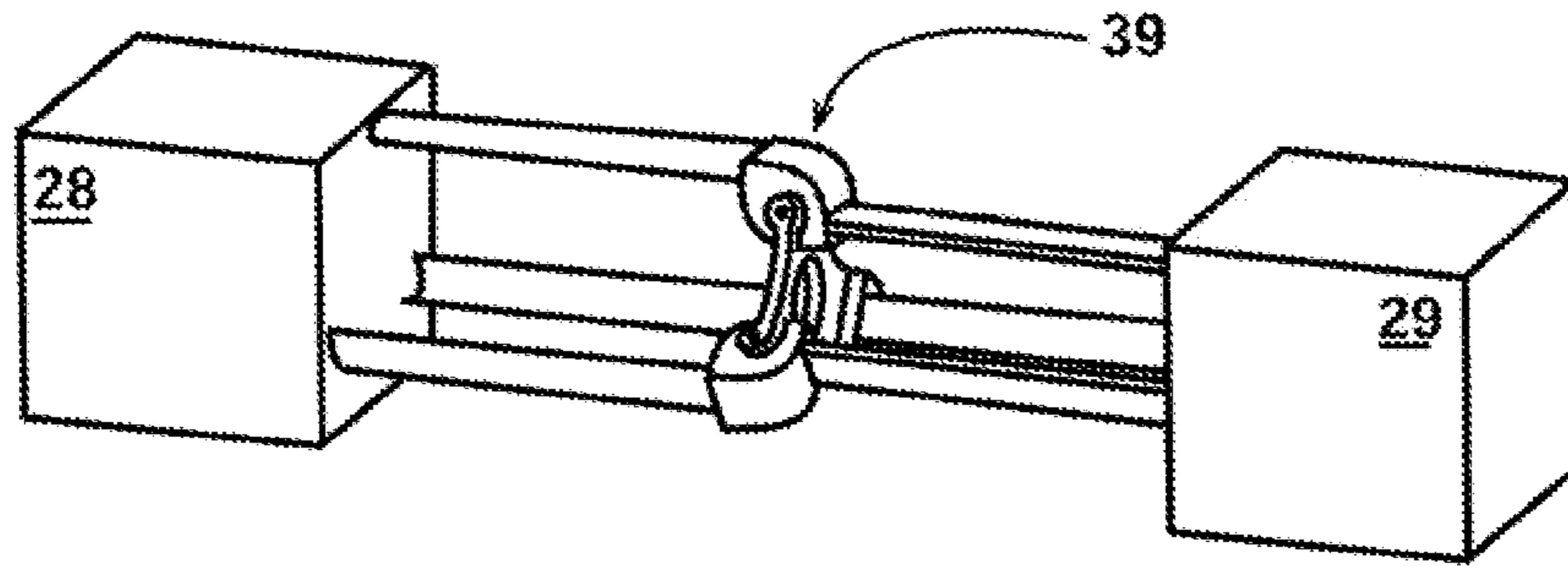
3-Beam Deployment Device Partial Deployment - Oblique View
