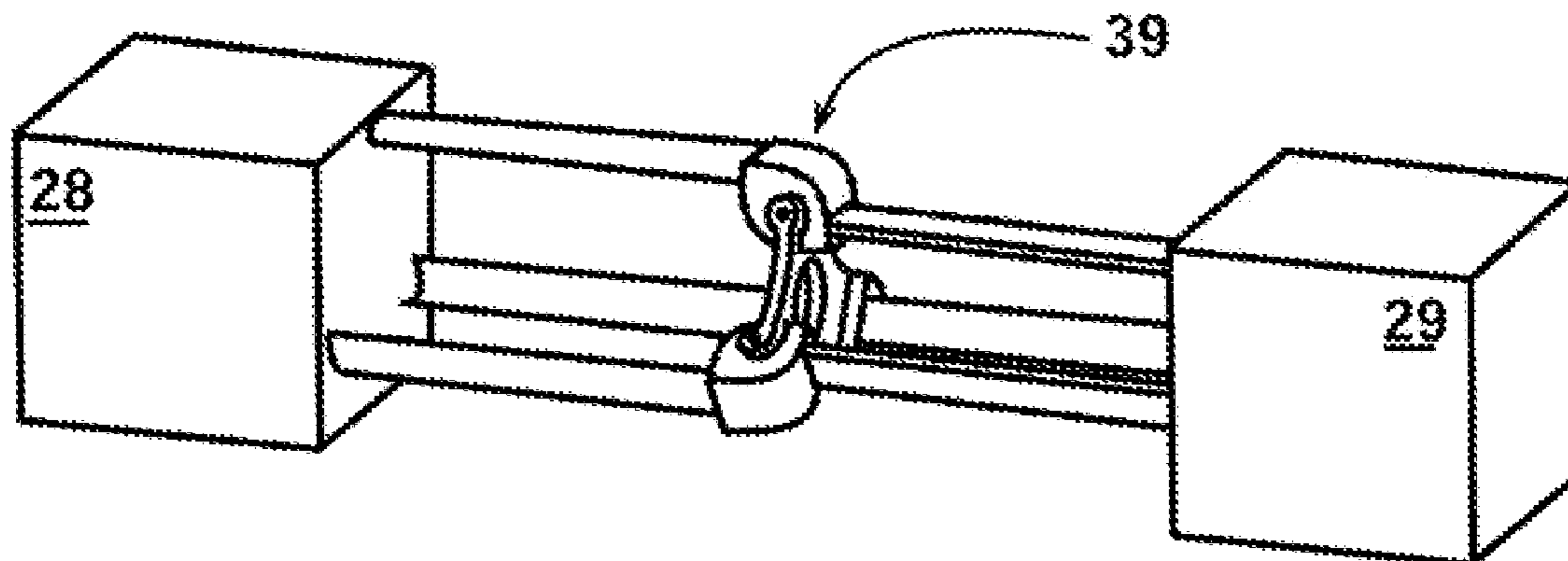
3-Beam Deployment Device Partial Deployment - Oblique View
