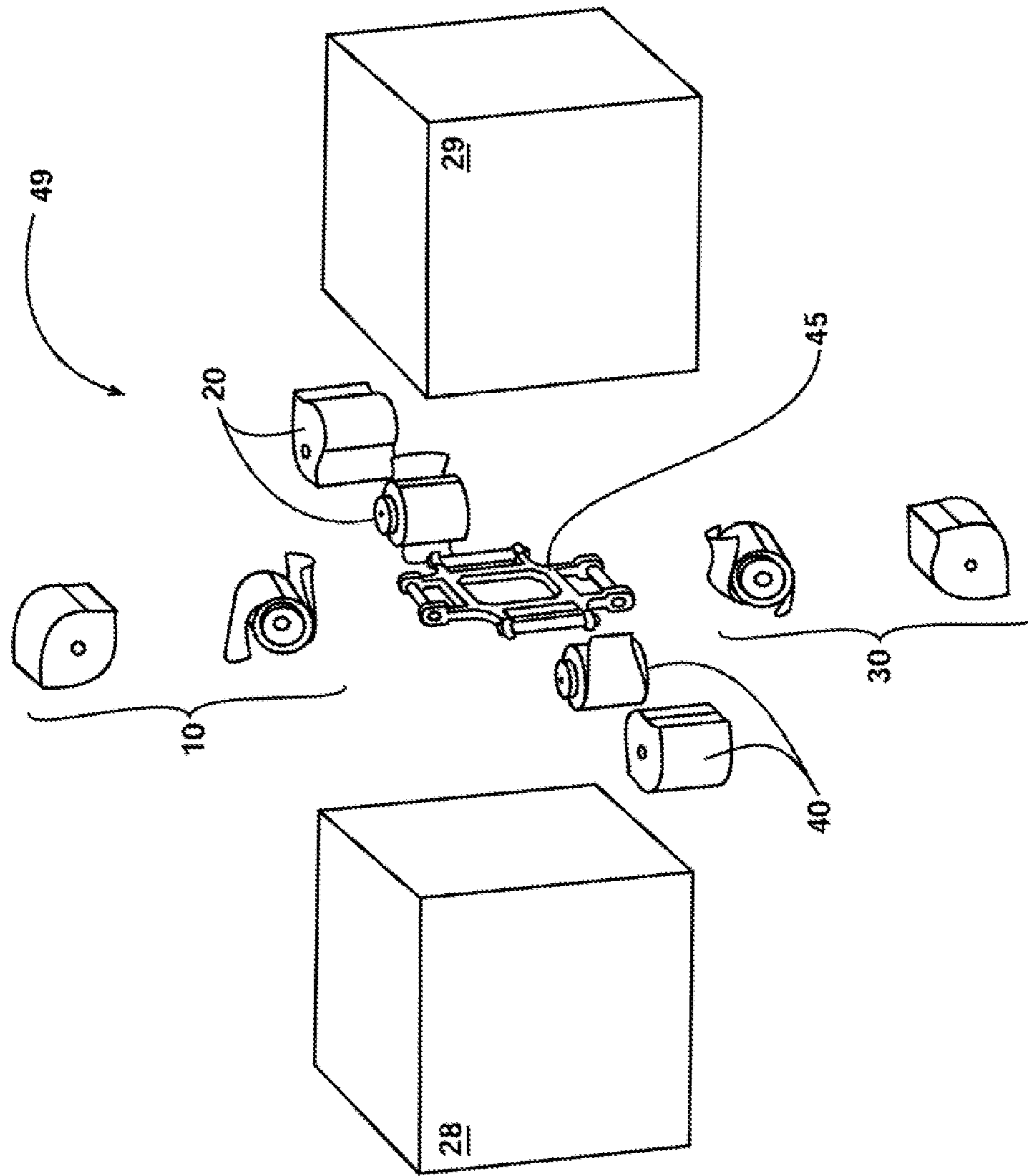
4-Beam Deployment Device - Expanded View
